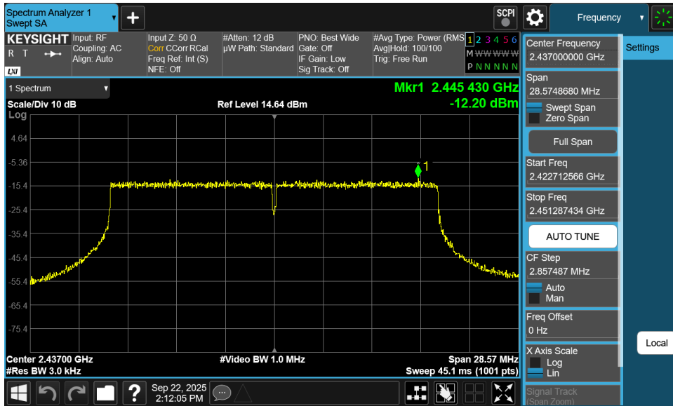
Plot 7-18. Power Spectral Density Plot Antenna 0 Common (802.11ax OFDMA – RU242 – Ch. 6)
