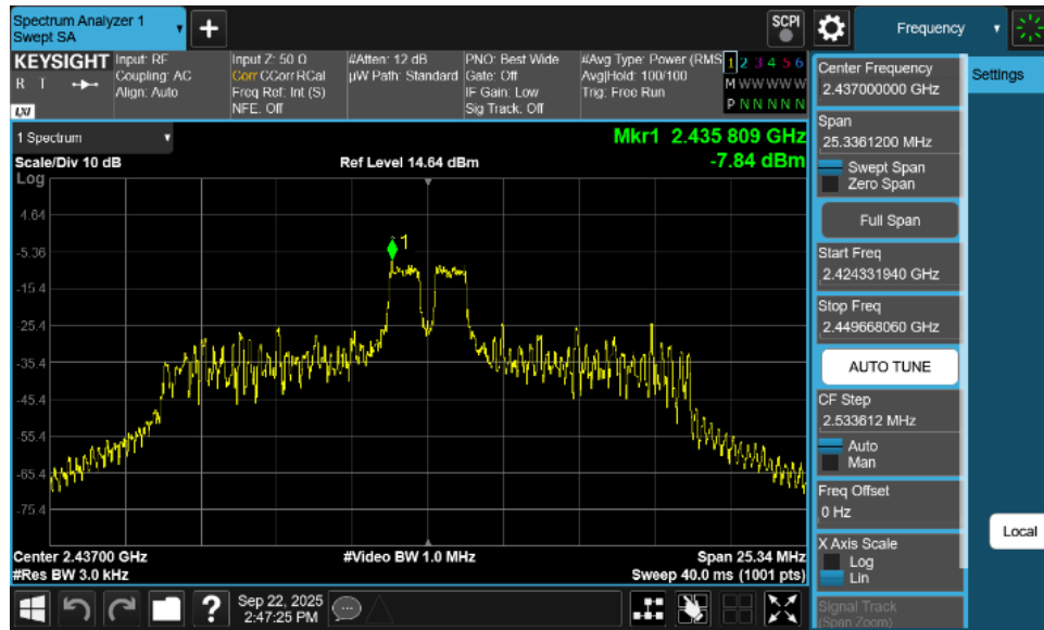
Plot 7-21. Power Spectral Density Plot Antenna 0 Common (802.11ax OFDMA – RU26 Index 4 – Ch. 6)
