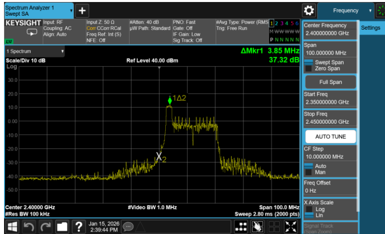
Plot 7-49. Band Edge Antenna 1 Common (802.11ax OFDMA – RU26 Index 0 – Ch. 1)
