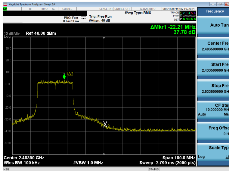
Plot 7-46. Band Edge Antenna 0 Common (802.11ax OFDMA – RU242 – Ch. 10)
