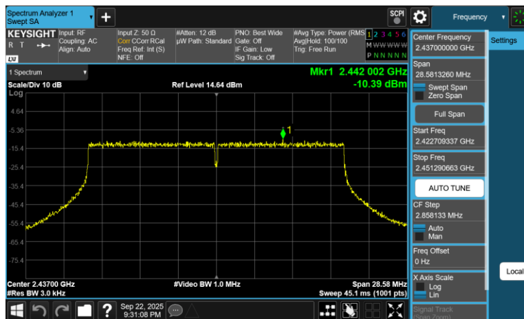
Plot 7-32. Power Spectral Density Plot Antenna 1 Dedicated (802.11ax OFDMA – RU242 – Ch. 6)
