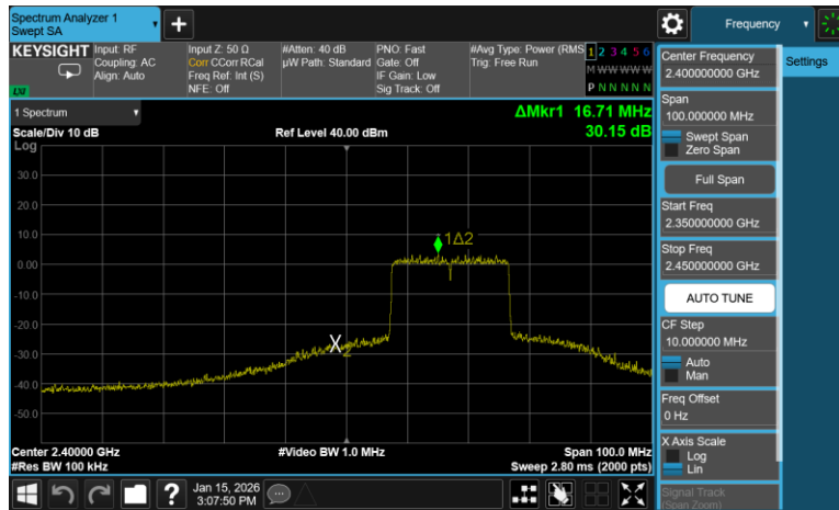
Plot 7-53. Band Edge Antenna 1 Common (802.11ax OFDMA – RU242 – Ch. 2)
