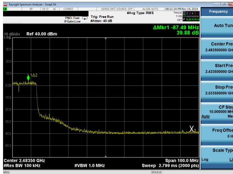
Plot 7-42. Band Edge Antenna 0 Common (802.11ax OFDMA – RU242 – Ch. 6(High Channel))
