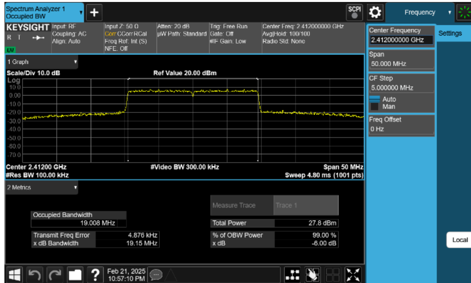
Plot 7-16. 6dB BW Plot Antenna 1 Dedicated (802.11ax OFDMA – RU242 – Ch. 1)
