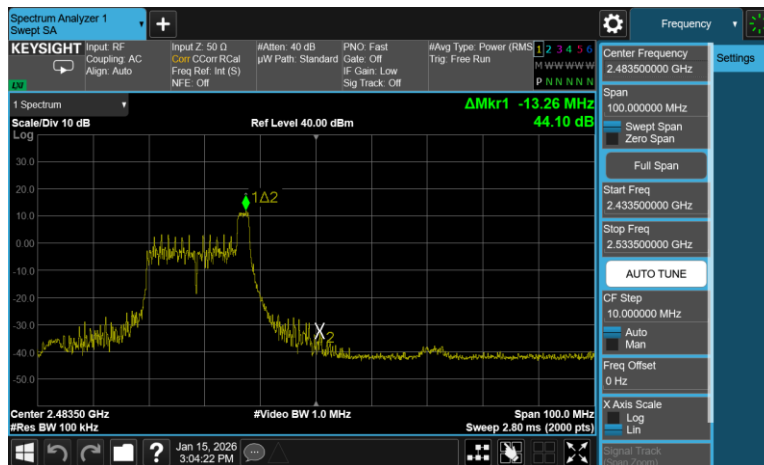
Plot 7-50. Band Edge Antenna 1 Common (802.11ax OFDMA – RU26 Index 8 – Ch. 11)
