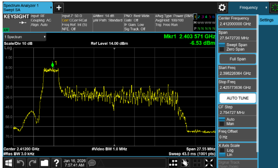
Plot 7-25. Power Spectral Density Plot Antenna 0 Dedicated (802.11ax OFDMA – RU26 Index 0 – Ch. 1)
