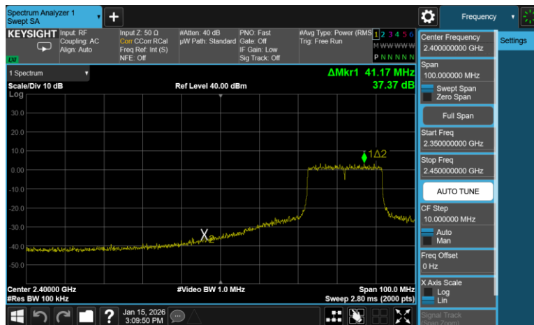
Plot 7-56. Band Edge Antenna 1 Common (802.11ax OFDMA – RU242 – Ch. 5)
