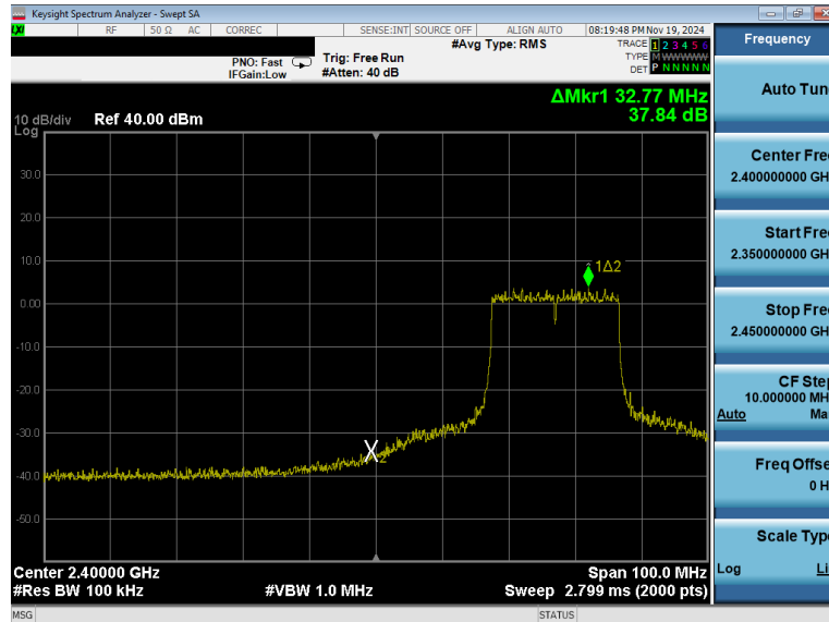
Plot 7-39. Band Edge Antenna 0 Common (802.11ax OFDMA – RU242 – Ch. 4)
