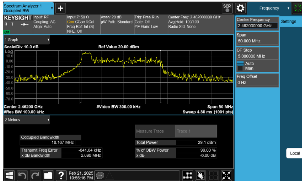
Plot 7-15. 6dB BW Antenna 1 Dedicated (802.11ax OFDMA – RU26 Index 0 – Ch. 11)
