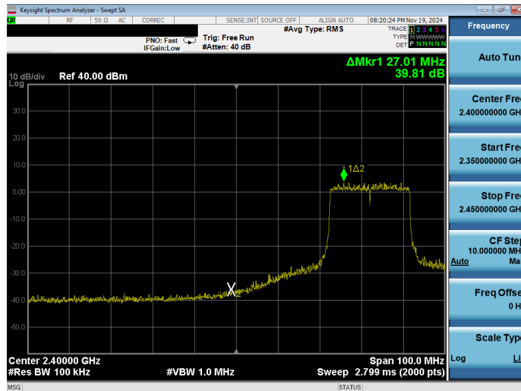
Plot 7-40. Band Edge Antenna 0 Common (802.11ax OFDMA – RU242 – Ch. 5)
