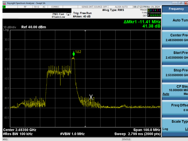
Plot 7-35. Band Edge Antenna 0 Common (802.11ax OFDMA – RU26 Index 8 – Ch. 12)
