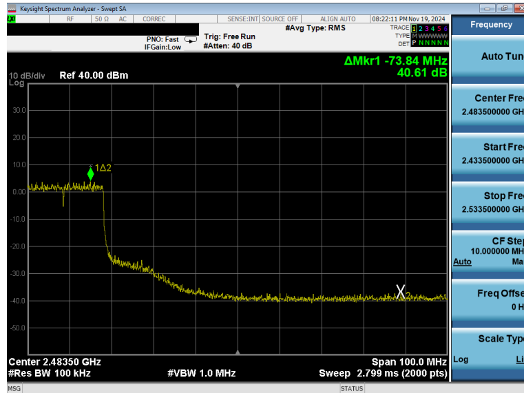
Plot 7-43. Band Edge Antenna 0 Common (802.11ax OFDMA – RU242 – Ch. 7)
