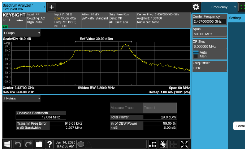
Plot 7-5. 99% OBW Plot Antenna 0 Dedicated (802.11ax OFDMA – RU26 Index 8 – Ch. 6)
