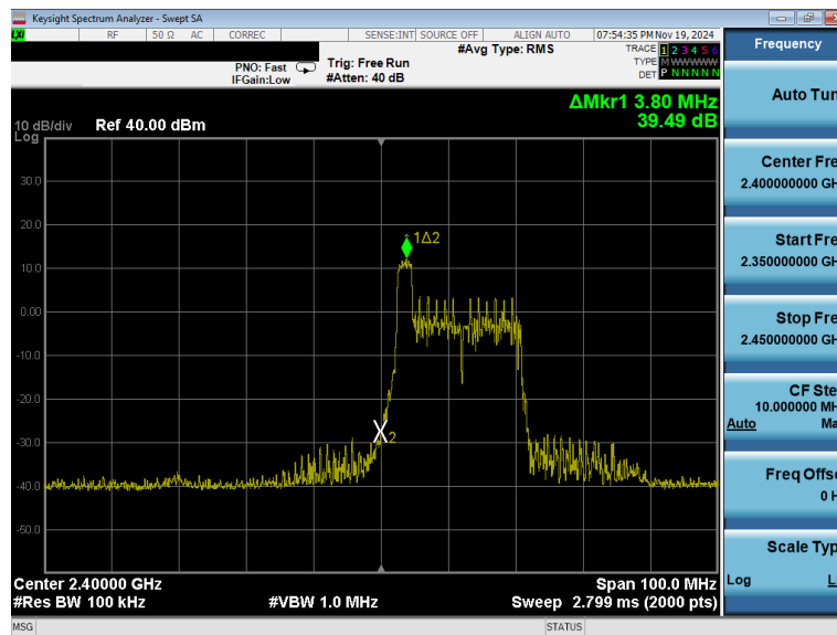
Plot 7-33. Band Edge Antenna 0 Common (802.11ax OFDMA – RU26 Index 0 – Ch. 1)
