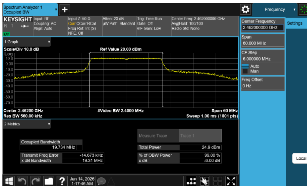
Plot 7-4. 99% OBW Plot Antenna 1 Common (802.11ax OFDMA – RU242 – Ch. 11)
