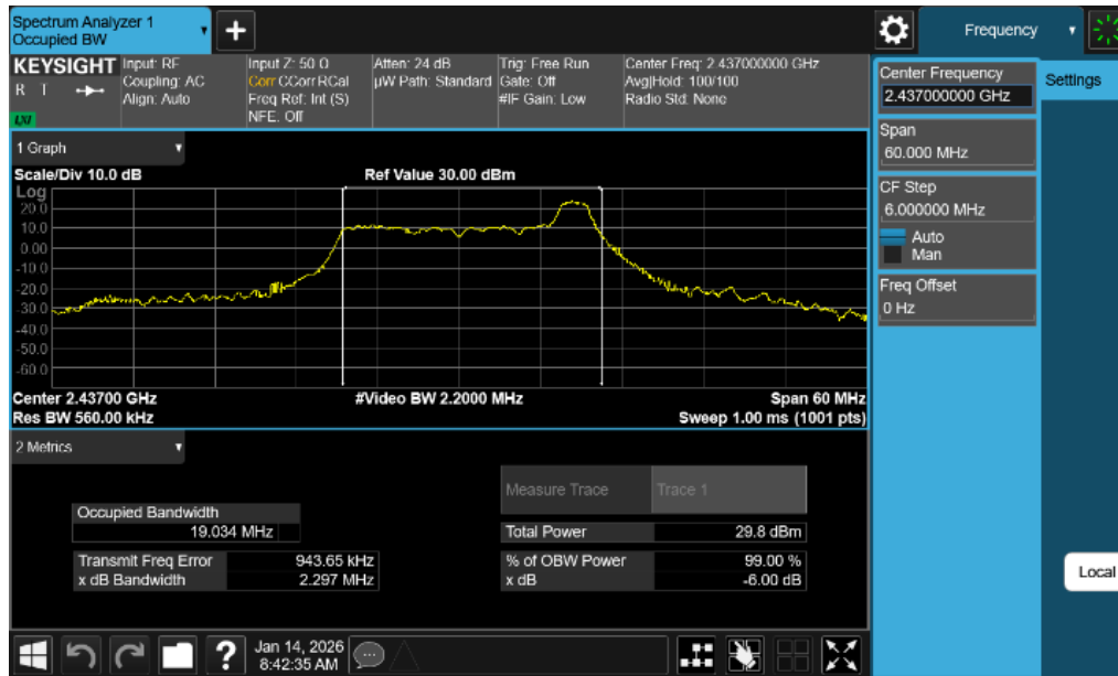
Plot 7-7. 99% OBW Antenna 1 Dedicated (802.11ax OFDMA – RU26 Index 8 – Ch. 6)
