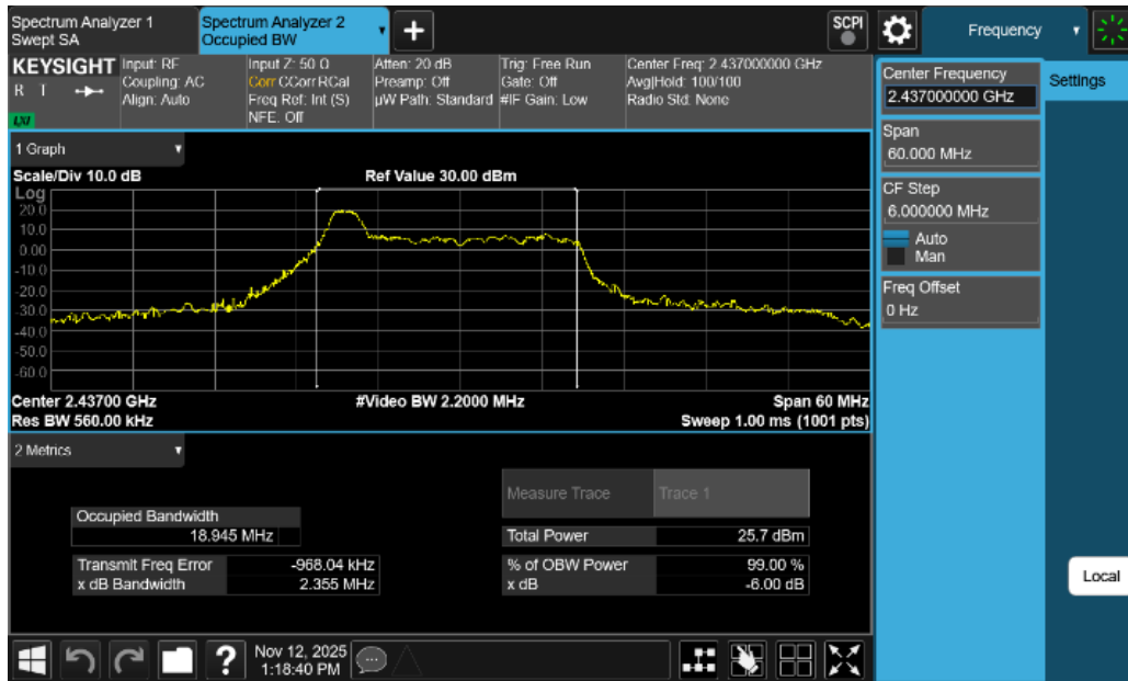
Plot 7-1. 99% OBW Plot Antenna 0 Common (802.11ax OFDMA – RU26 Index 0 – Ch. 6)
