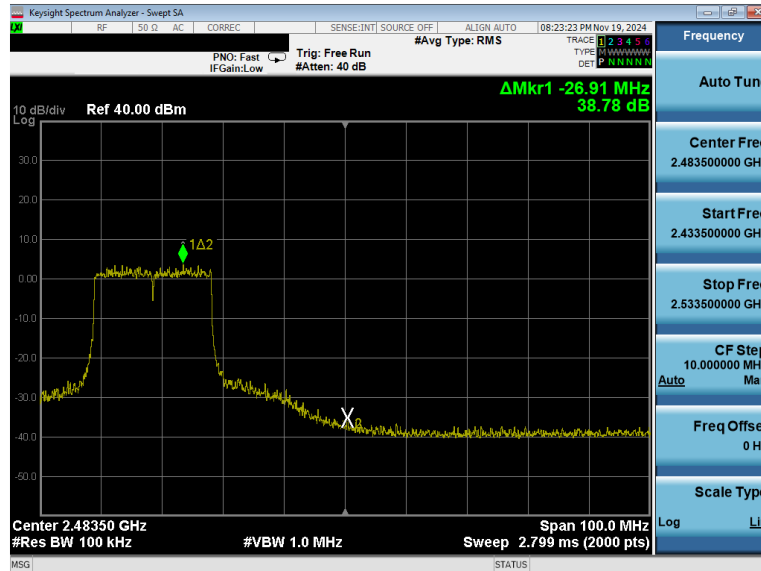
Plot 7-45. Band Edge Antenna 0 Common (802.11ax OFDMA – RU242 – Ch. 9)
