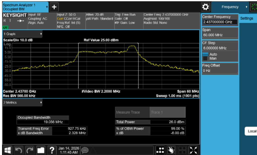
Plot 7-3. 99% OBW Antenna 1 Common (802.11ax OFDMA – RU26 Index 8 – Ch. 6)
