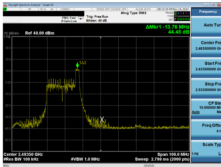
Plot 7-34. Band Edge Antenna 0 Common (802.11ax OFDMA – RU26 Index 8 – Ch. 11)
