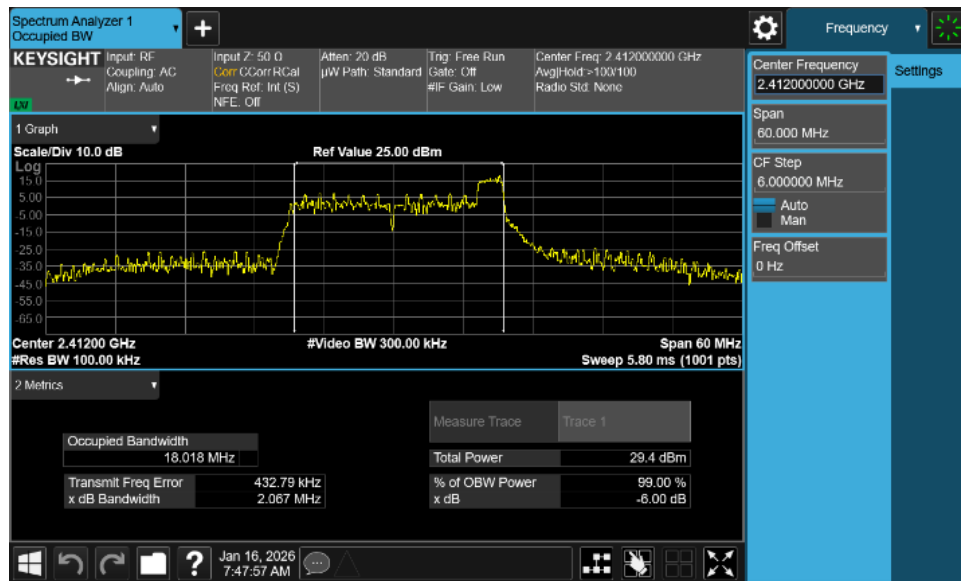
Plot 7-13. 6dB BW Plot Antenna 0 Dedicated (802.11ax OFDMA – RU26 Index 8 – Ch. 1)
