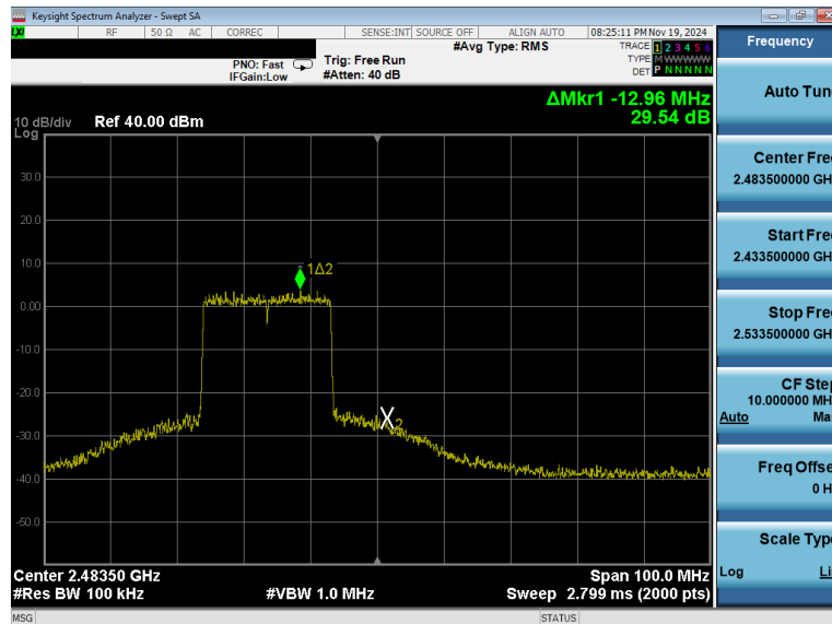
Plot 7-48. Band Edge Antenna 0 Common (802.11ax OFDMA – RU242 – Ch. 12)
