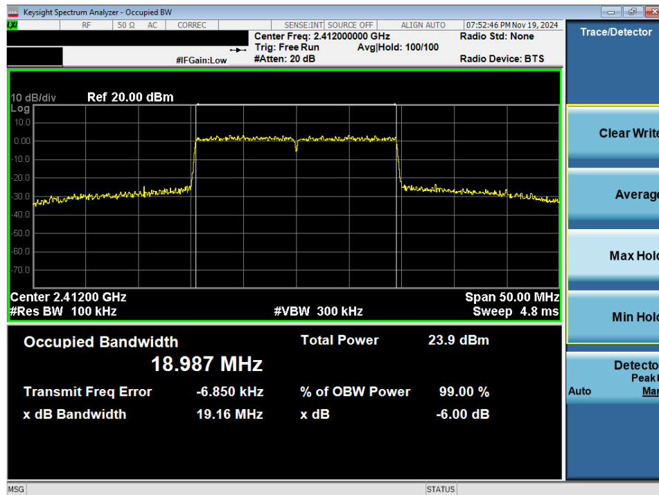
Plot 7-10. 6dB BW Plot Antenna 0 Common (802.11ax OFDMA – RU242 – Ch. 1)
