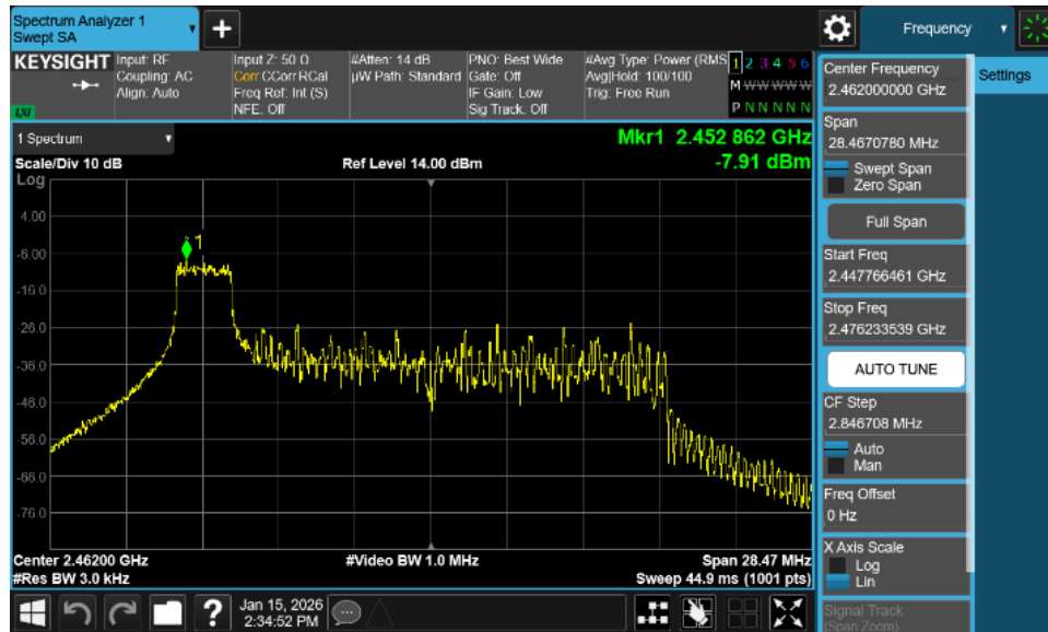
Plot 7-19. Power Spectral Density Plot Antenna 1 Common (802.11ax OFDMA – RU26 Index 4 – Ch. 11)
