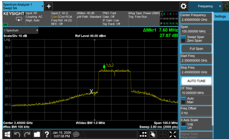
Plot 7-52. Band Edge Antenna 1 Common (802.11ax OFDMA – RU242 – Ch. 1)
