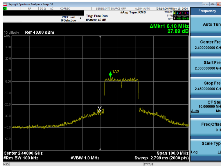
Plot 7-36. Band Edge Antenna 0 Common (802.11ax OFDMA – RU242 – Ch. 1)
