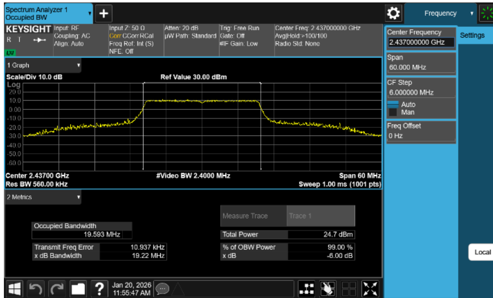
Plot 7-2. 99% OBW Plot Antenna 0 Common (802.11ax OFDMA – RU242 – Ch. 6)
