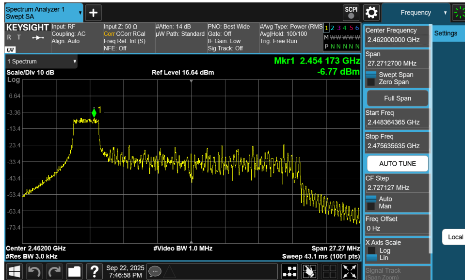
Plot 7-27. Power Spectral Density Plot Antenna 1 Dedicated (802.11ax OFDMA – RU26 Index 0 – Ch. 11)
