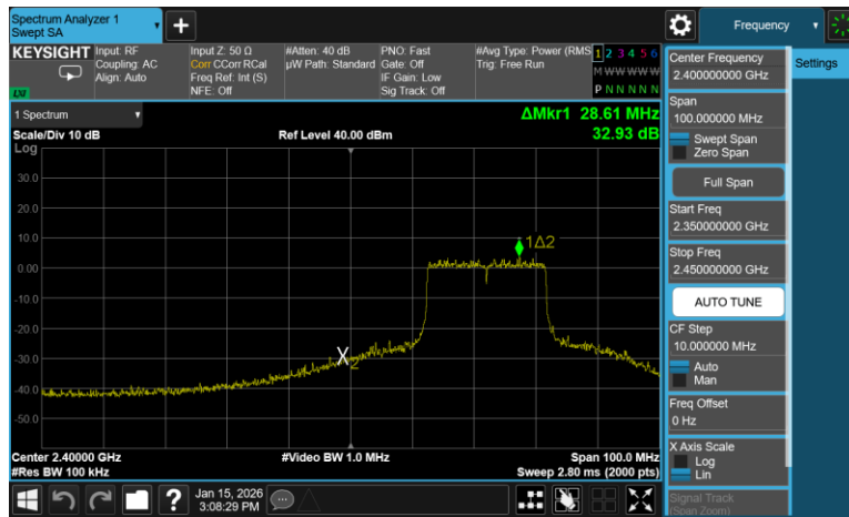
Plot 7-54. Band Edge Antenna 1 Common (802.11ax OFDMA – RU242 – Ch. 3)
