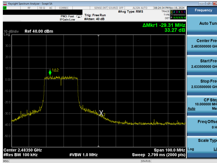
Plot 7-47. Band Edge Antenna 0 Common (802.11ax OFDMA – RU242 – Ch. 11)
