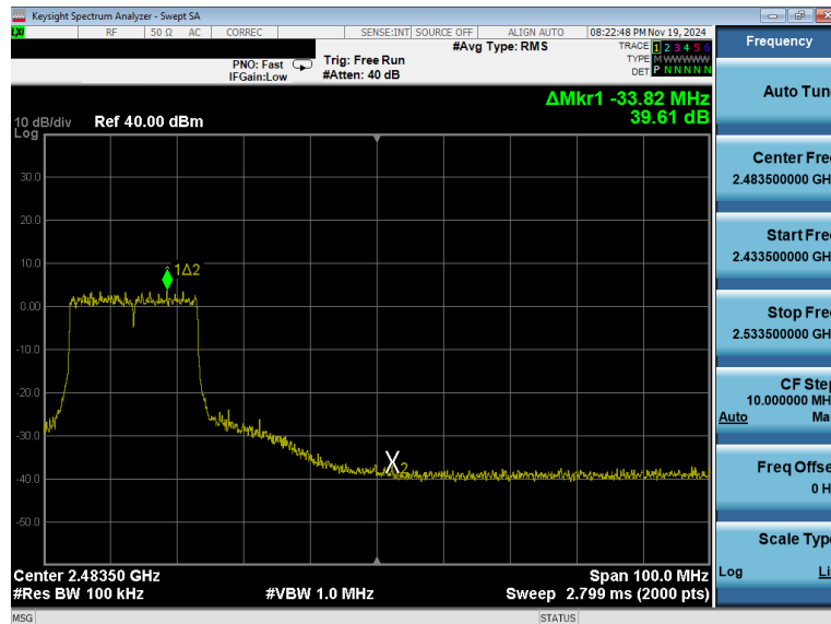
Plot 7-44. Band Edge Antenna 0 Common (802.11ax OFDMA – RU242 – Ch. 8)
