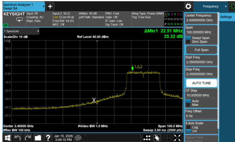
Plot 7-55. Band Edge Antenna 1 Common (802.11ax OFDMA – RU242 – Ch. 4)
