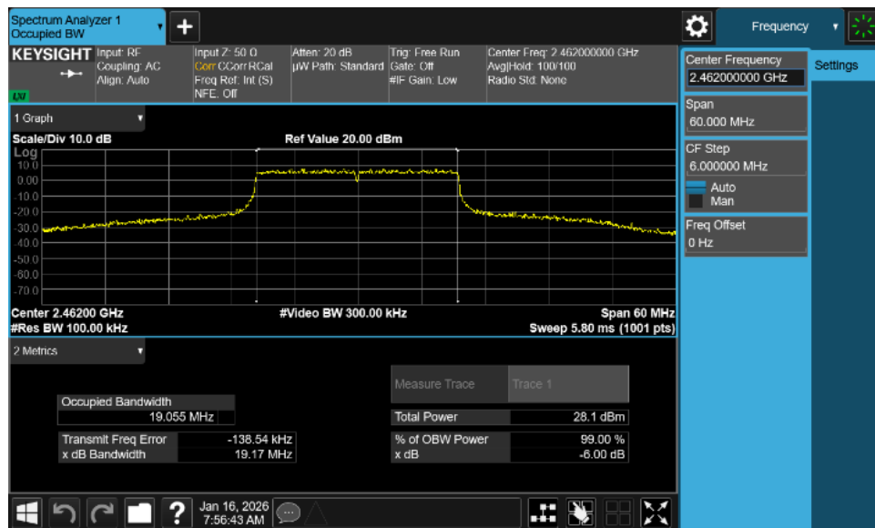
Plot 7-14. 6dB BW Plot Antenna 0 Dedicated (802.11ax OFDMA – RU242 – Ch. 11)
