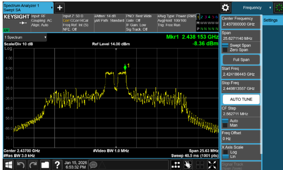
Plot 7-23. Power Spectral Density Plot Antenna 1 Common (802.11ax OFDMA – RU26 Index 4 – Ch. 6)
