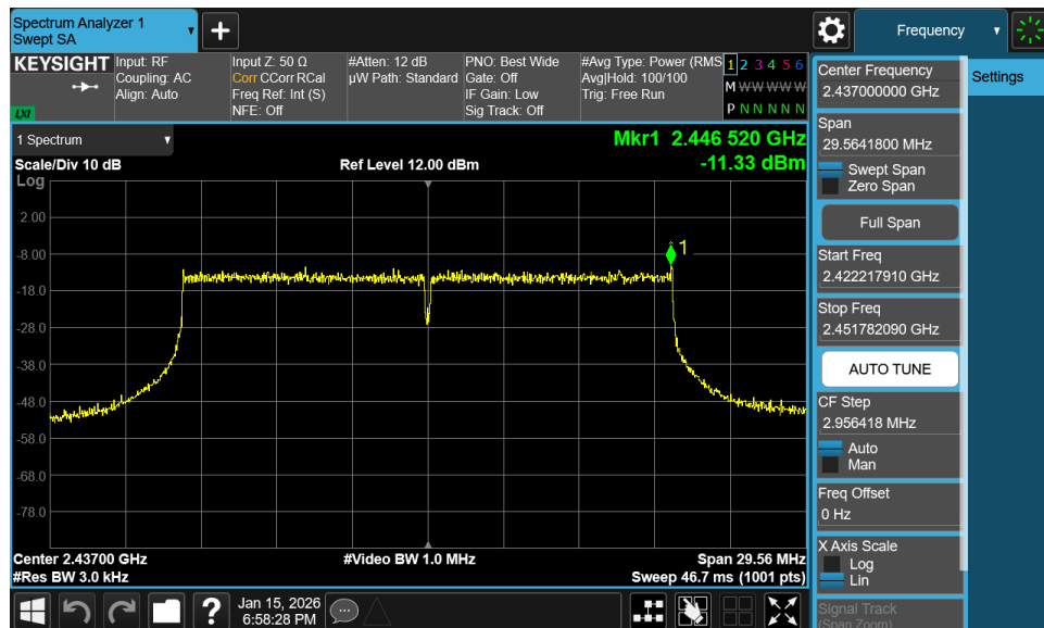
Plot 7-24. Power Spectral Density Plot Antenna 1 Common (802.11ax OFDMA – RU242 – Ch. 6)
