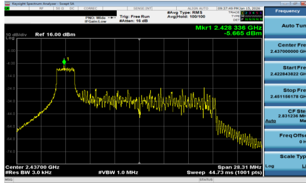
Plot 7-29. Power Spectral Density Plot Antenna 0 Dedicated (802.11ax OFDMA – RU26 Index 0 – Ch. 6)
