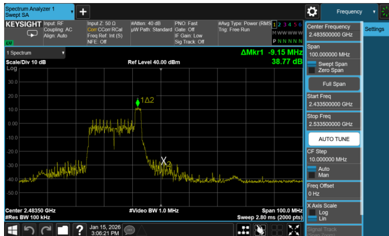
Plot 7-51. Band Edge Antenna 1 Common (802.11ax OFDMA – RU26 Index 8 – Ch. 12)
