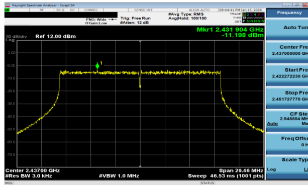
Plot 7-30. Power Spectral Density Plot Antenna 0 Dedicated (802.11ax OFDMA – RU242 – Ch. 6)
