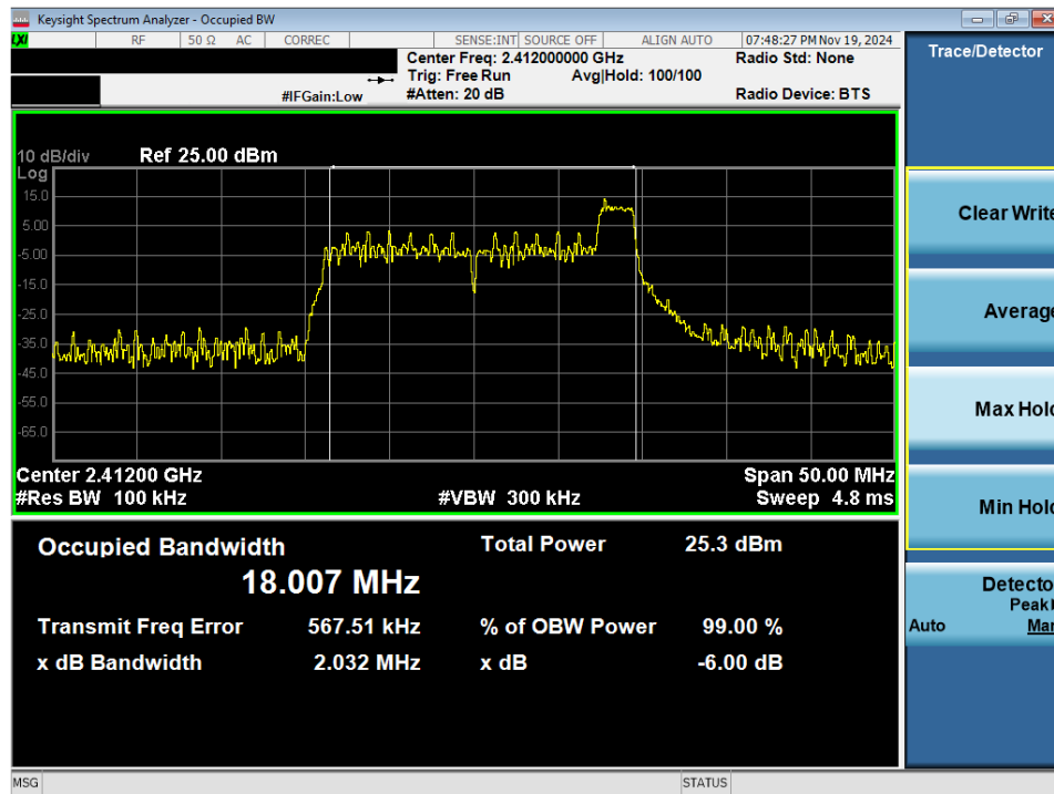
Plot 7-9. 6dB BW Plot Antenna 0 Common (802.11ax OFDMA – RU26 Index 8 – Ch. 1)
