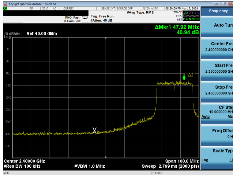
Plot 7-41. Band Edge Antenna 0 Common (802.11ax OFDMA – RU242 – Ch. 6(Low Channel))
