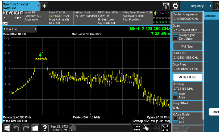
Plot 7-31. Power Spectral Density Plot Antenna 1 Dedicated (802.11ax OFDMA – RU26 Index 0 – Ch. 6)
