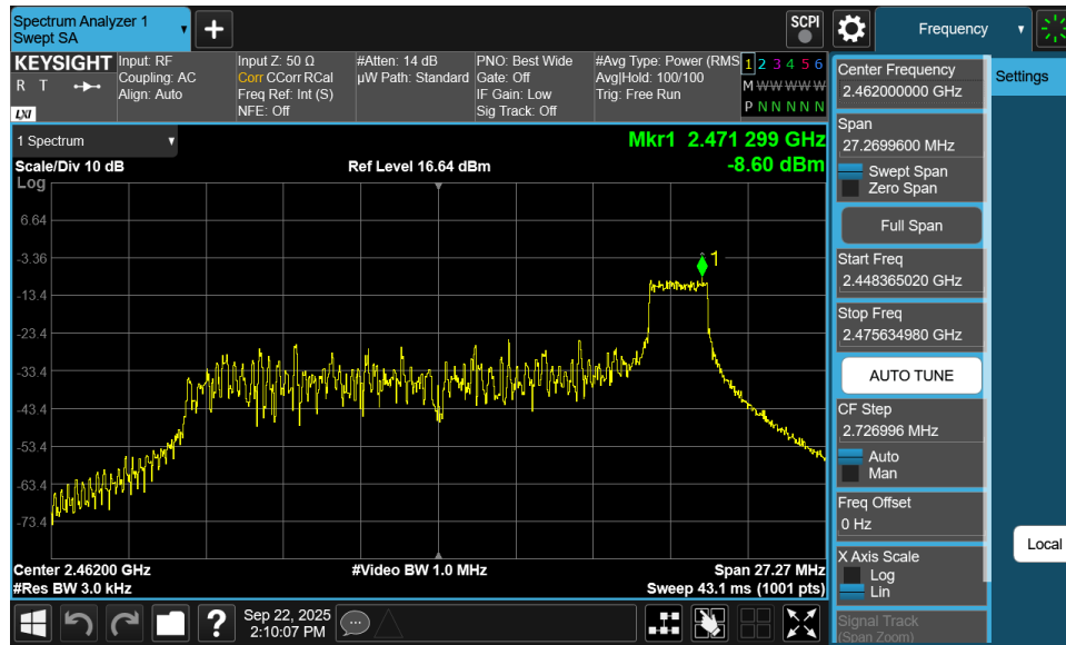
Plot 7-17. Power Spectral Density Plot Antenna 0 Common (802.11ax OFDMA – RU26 Index 8 – Ch. 11)
