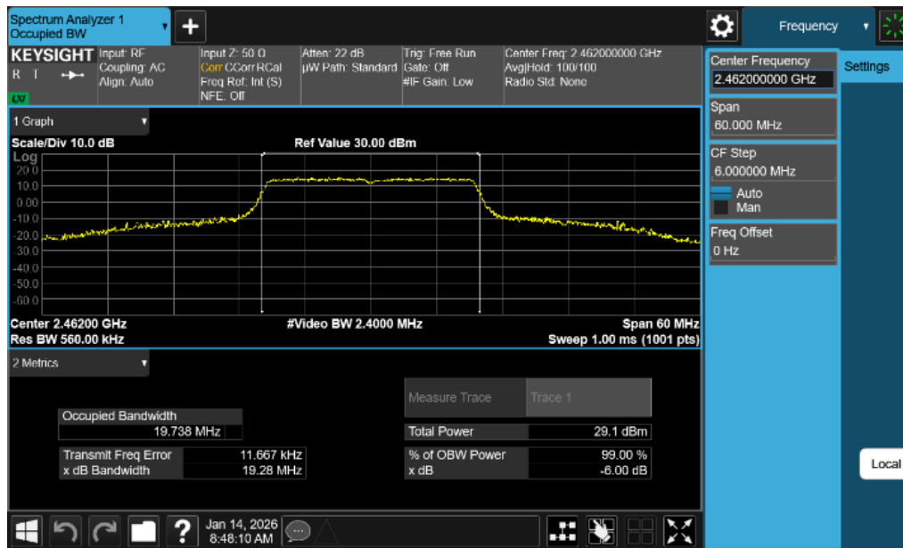
Plot 7-6. 99% OBW Plot Antenna 0 Dedicated (802.11ax OFDMA – RU242 – Ch. 11)
