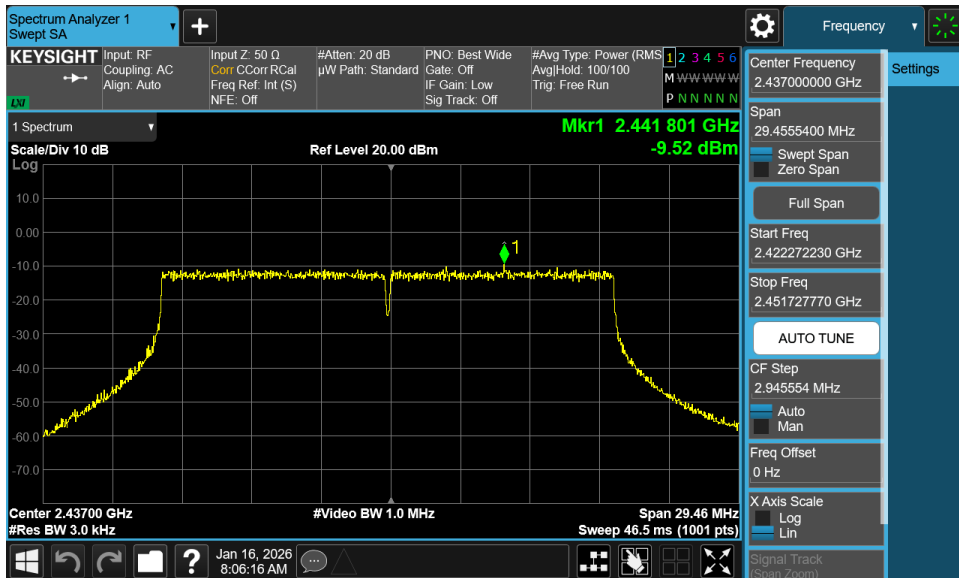
Plot 7-26. Power Spectral Density Plot Antenna 0 Dedicated (802.11ax OFDMA – RU242 – Ch. 6)
