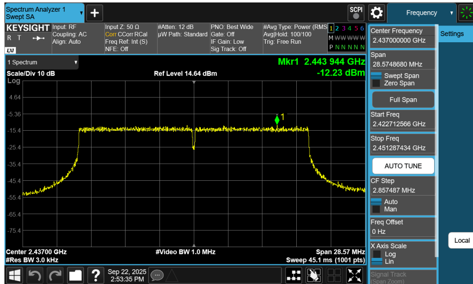
Plot 7-22. Power Spectral Density Plot Antenna 0 Common (802.11ax OFDMA – RU242 – Ch. 6)
