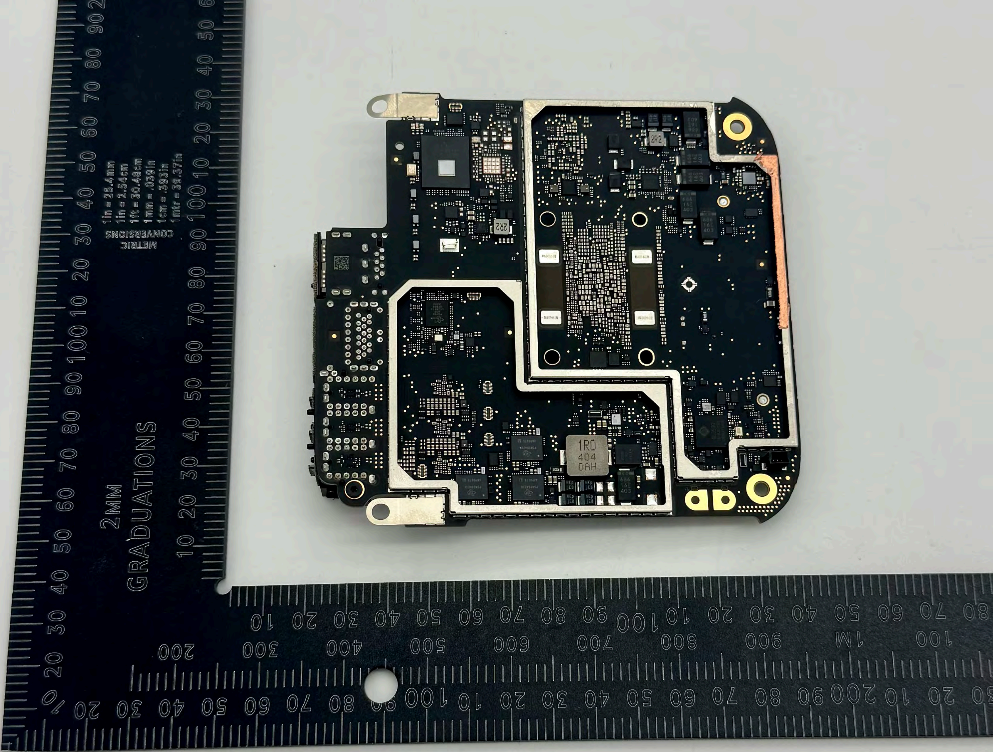
A3238 MLB with shield removed - Back
