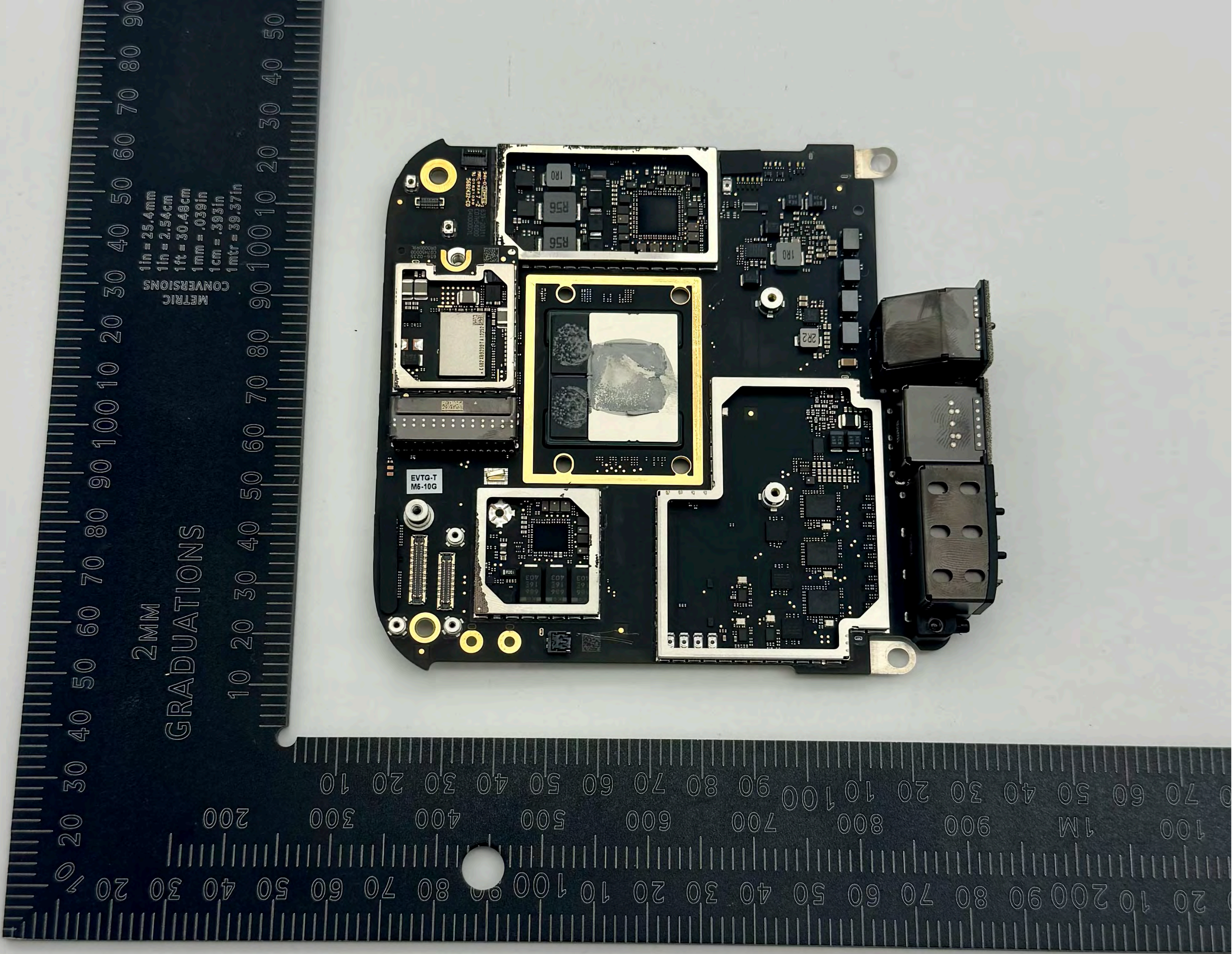
A3238 MLB with shield removed - Front
