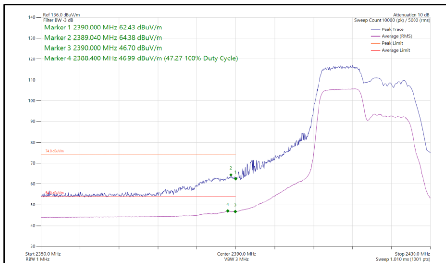
Figure 57 - 802.11ax HE20, RU 106-53, SISO, Core 1 - 2417 MHz Band Edge Frequency 2390 MHz
