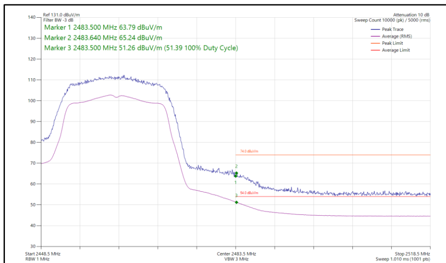
Figure 30 - 802.11n HT20, SISO, Core 0 - 2462 MHz Band Edge Frequency 2483.5 MHz
