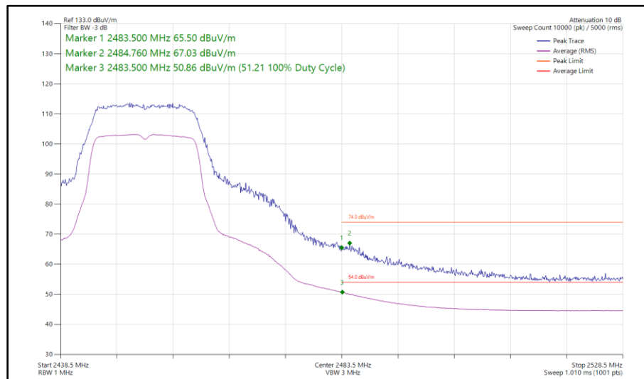
Figure 21 - 802.11g, SISO, Core 0 - 2452 MHz Band Edge Frequency 2483.5 MHz
