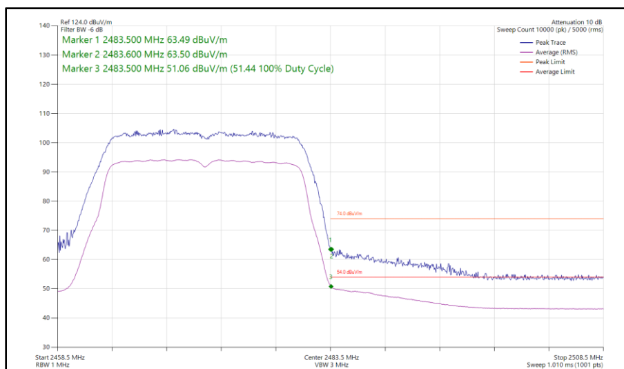
Figure 32 - 802.11n HT20, SISO, Core 0 - 2472 MHz Band Edge Frequency 2483.5 MHz
