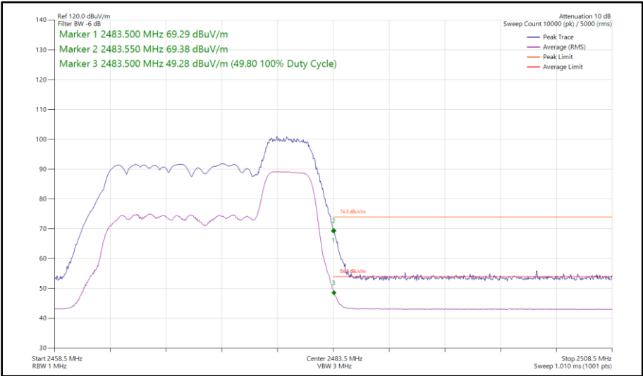
Figure 43 - 802.11ax HE20, RU 52-40, SISO, Core 0 - 2472 MHz Band Edge Frequency 2483.5 MHz
