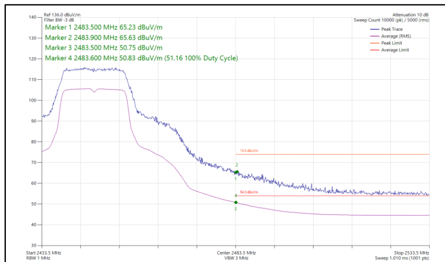
Figure 20 - 802.11g, SISO, Core 0 - 2447 MHz Band Edge Frequency 2483.5 MHz
