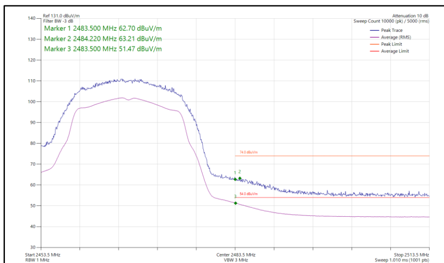
Figure 24 - 802.11g, SISO, Core 0 - 2467 MHz Band Edge Frequency 2483.5 MHz
