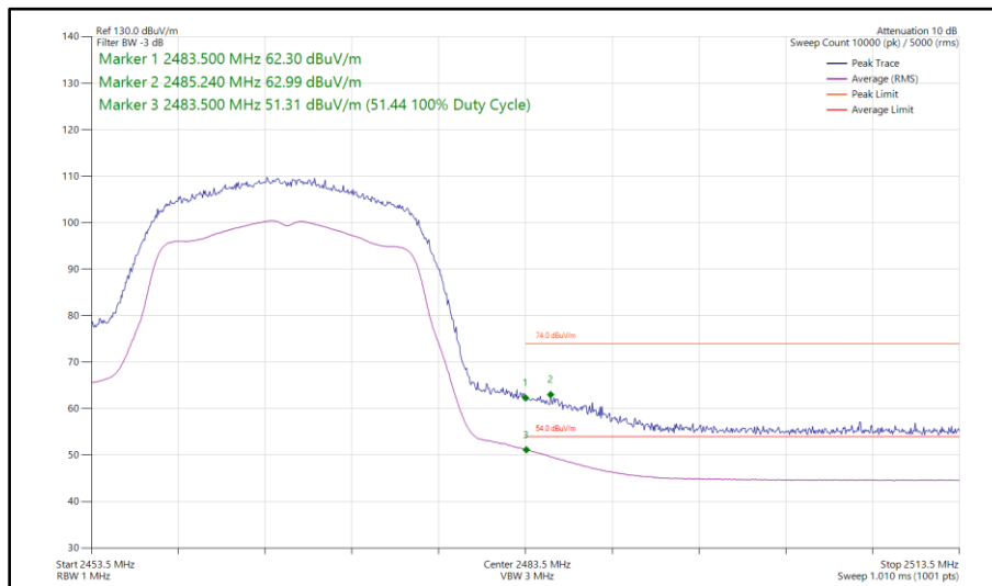
Figure 31 - 802.11n HT20, SISO, Core 0 - 2467 MHz Band Edge Frequency 2483.5 MHz
