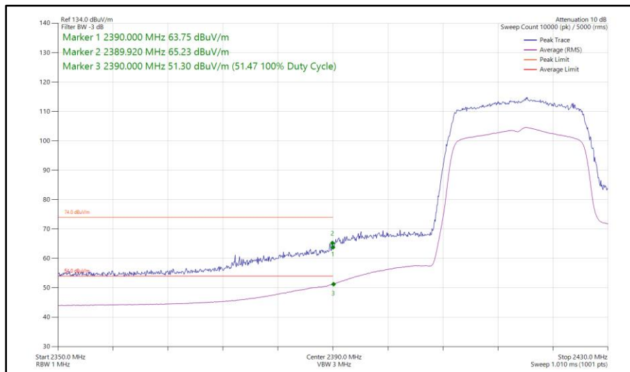
Figure 56 - 802.11ax HE20, SU, SISO, Core 1 - 2417 MHz Band Edge Frequency 2390 MHz
