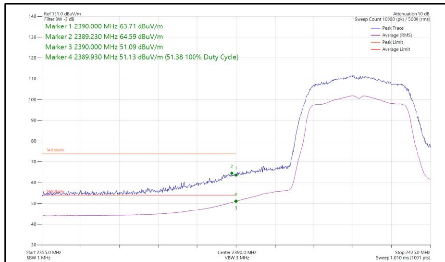
Figure 50 - 802.11n HT20, SISO, Core 1 - 2412 MHz Band Edge Frequency 2390 MHz
