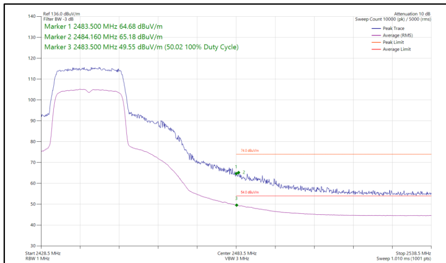
Figure 33 - 802.11ax HE20, SU, SISO, Core 0 - 2442 MHz Band Edge Frequency 2483.5 MHz
