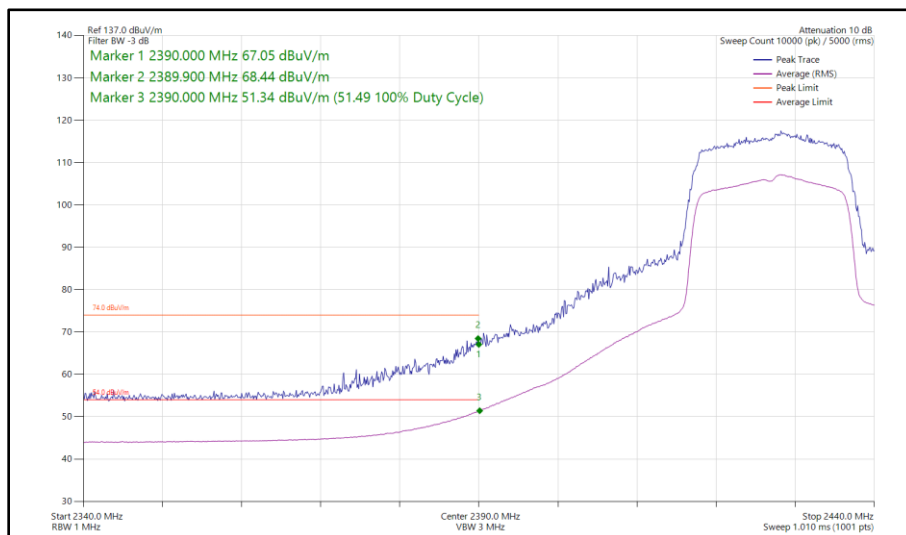
Figure 59 - 802.11ax HE20, SU, SISO, Core 1 - 2427 MHz Band Edge Frequency 2390 MHz
