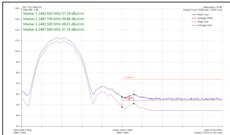
Figure 60 - 802.11b, SISO, Core 1 - 2462 MHz Band Edge Frequency 2483.5 MHz
