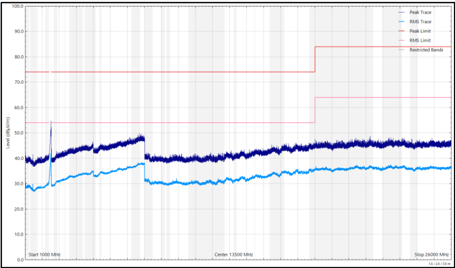
Figure 217 - 2472 MHz (CH13), 802.11g, Core 1, 1 GHz to 26 GHz, Horizontal
