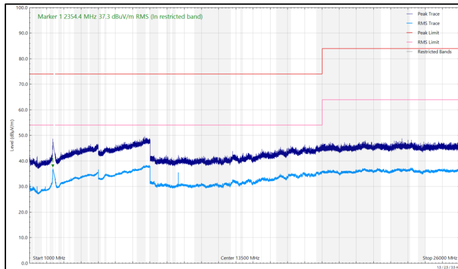
Figure 220 - 2412 MHz (CH1), HT20, CDD, Core 0 + Core 1, 1 GHz to 26 GHz, Vertical
