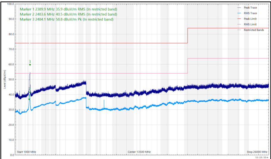
Figure 216 - 2442 MHz (CH7), 802.11g, Core 1, 1 GHz to 26 GHz, Vertical
