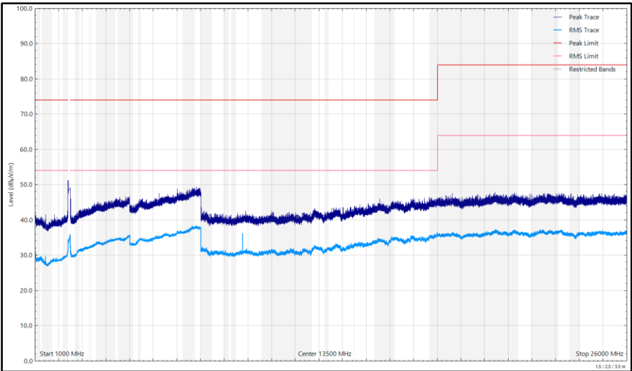
Figure 232 - 2442 MHz (CH7), HE20, RU26-0, CDD, Core 0 + Core 1, 1 GHz to 26 GHz, Vertical
