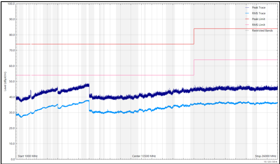
Figure 199 - 2442 MHz (CH7), 802.11b, Core 1, 1 GHz to 26 GHz, Horizontal
