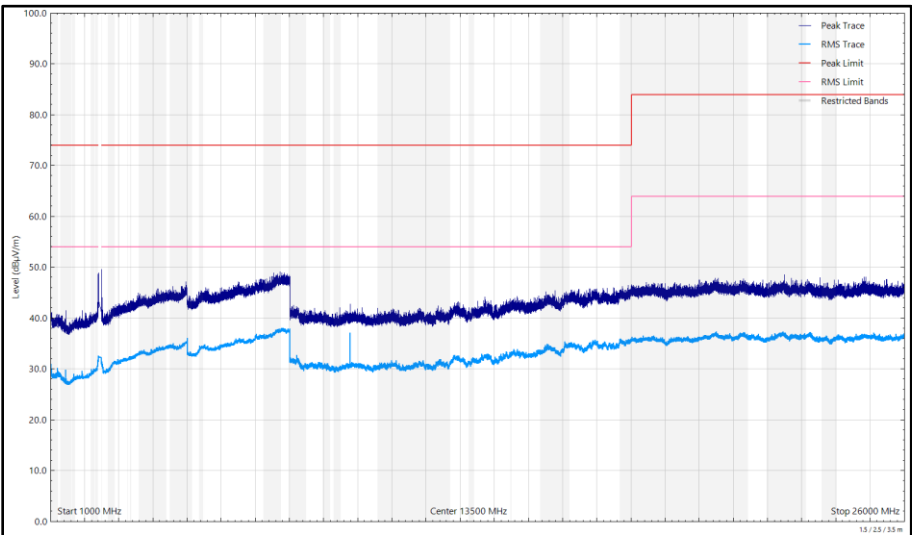
Figure 192 - 2442 MHz (CH7), 802.11b, Core 0, 1 GHz to 26 GHz, Vertical
