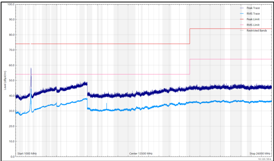
Figure 234 - 2472 MHz (CH13), HE20, RU26-0, CDD, Core 0 + Core 1, 1 GHz to 26 GHz, Vertical
