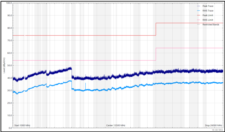
Figure 196 - 2412 MHz (CH1), 802.11b, Core 1, 1 GHz to 26 GHz, Vertical
