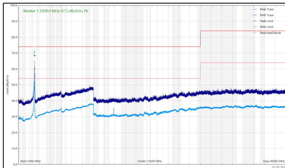
Figure 226 - 2472 MHz (CH13), HT20, CDD, Core 0 + Core 1, 1 GHz to 26 GHz, Vertical
