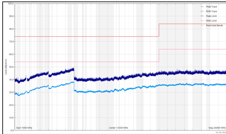
Figure 227 - 2412 MHz (CH1), HE20, RU26-0, CDD, Core 0 + Core 1, 1 GHz to 26 GHz, Horizontal
