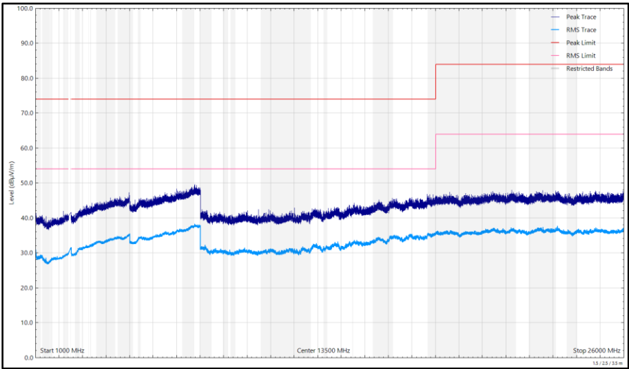
Figure 201 - 2472 MHz (CH13), 802.11b, Core 1, 1 GHz to 26 GHz, Horizontal
