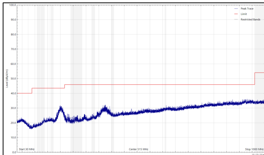
Figure 214 - 2442 MHz (CH7), 802.11g, Core 1, 30 MHz to 1 GHz, Vertical (Peak)
