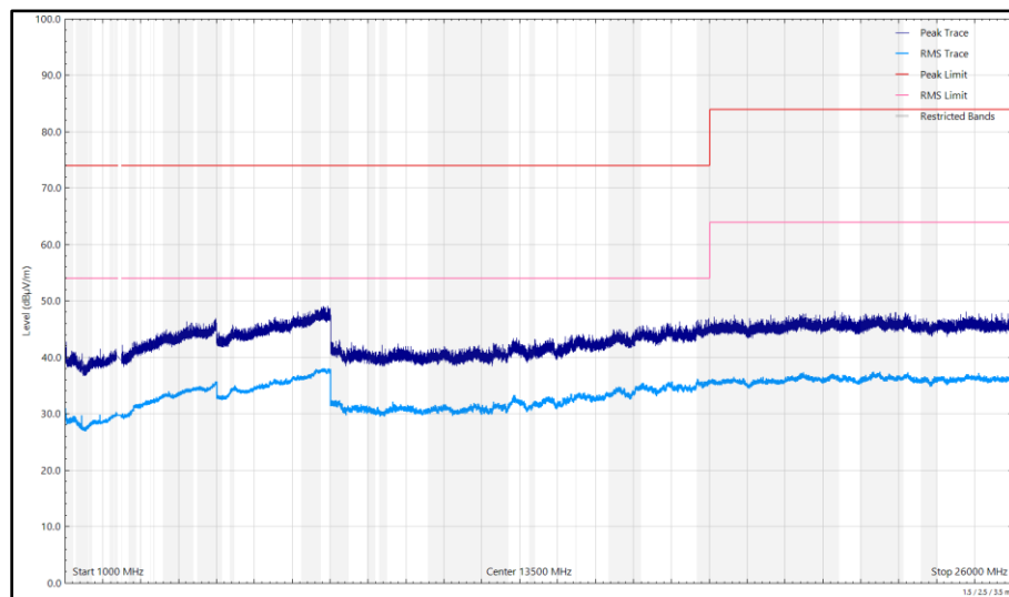
Figure 187 - 2412 MHz (CH1), 802.11b, Core 0, 1 GHz to 26 GHz, Horizontal
