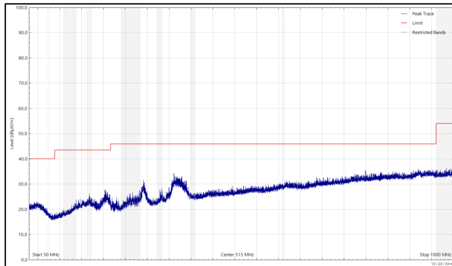
Figure 213 - 2442 MHz (CH7), 802.11g, Core 1, 30 MHz to 1 GHz, Horizontal (Peak)
