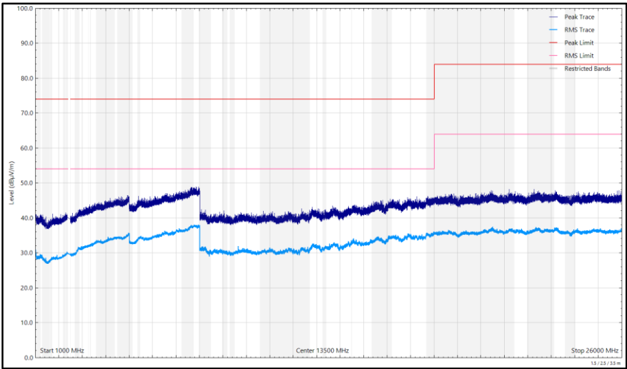
Figure 195 - 2412 MHz (CH1), 802.11b, Core 1, 1 GHz to 26 GHz, Horizontal
