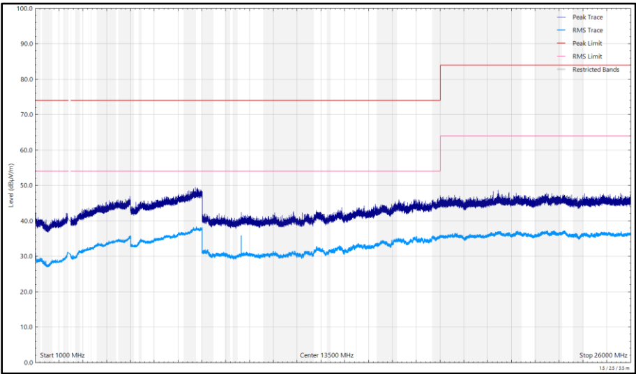
Figure 204 - 2412 MHz (CH1), 802.11g, Core 0, 1 GHz to 26 GHz, Vertical
