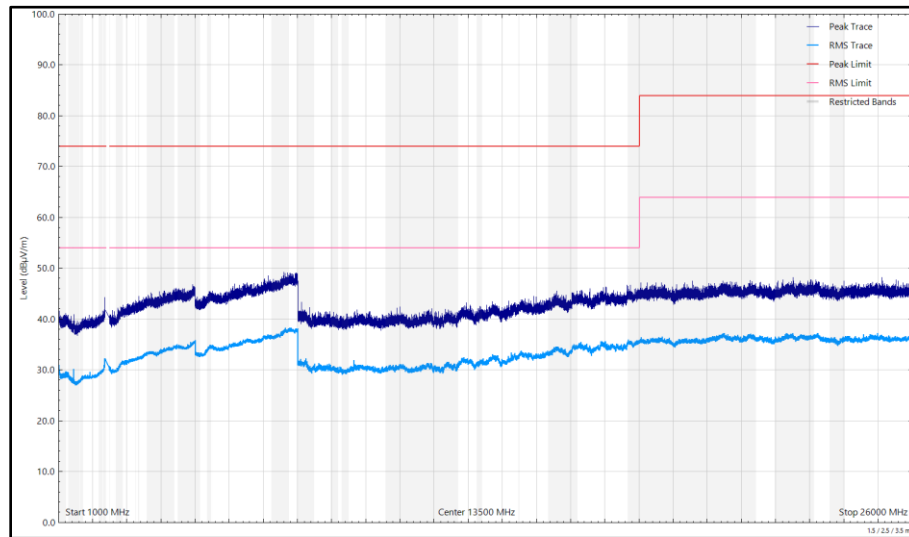
Figure 219 - 2412 MHz (CH1), HT20, CDD, Core 0 + Core 1, 1 GHz to 26 GHz, Horizontal
