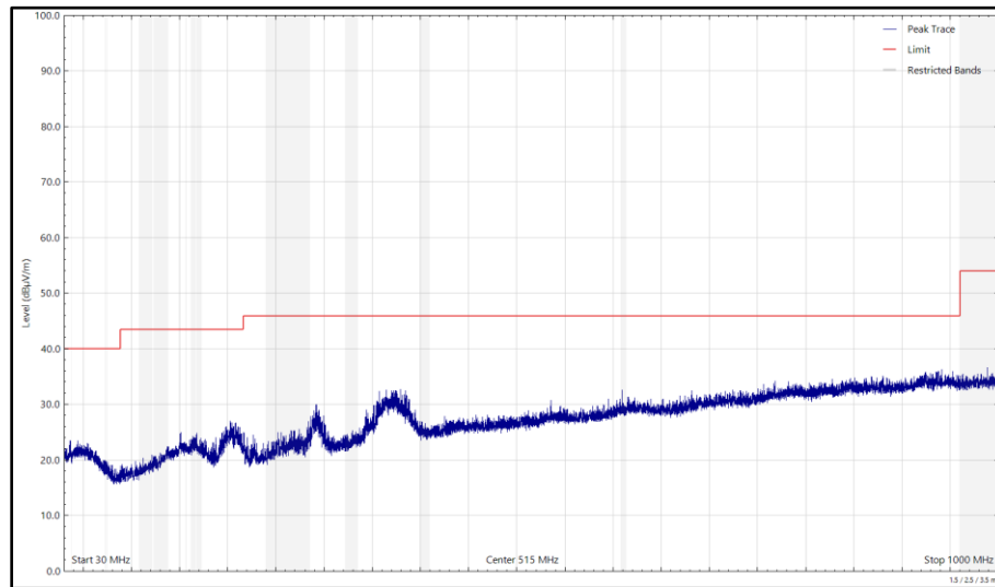
Figure 189 - 2442 MHz (CH7), 802.11b, Core 0, 30 MHz to 1 GHz, Horizontal (Peak)
