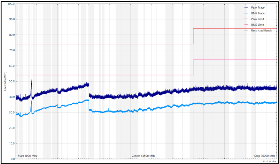
Figure 233 - 2472 MHz (CH13), HE20, RU26-0, CDD, Core 0 + Core 1, 1 GHz to 26 GHz, Horizontal
