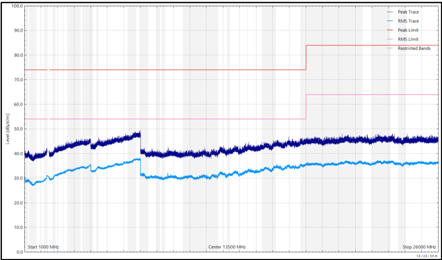
Figure 203 - 2412 MHz (CH1), 802.11g, Core 0, 1 GHz to 26 GHz, Horizontal
