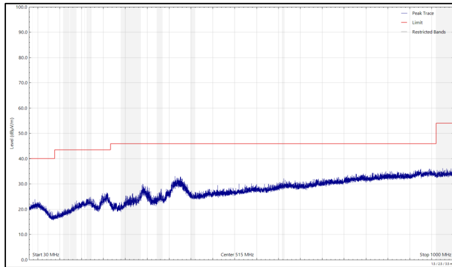
Figure 197 - 2442 MHz (CH7), 802.11b, Core 1, 30 MHz to 1 GHz, Horizontal (Peak)
