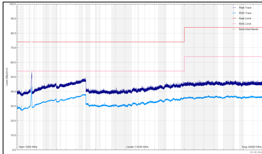
Figure 209 - 2472 MHz (CH13), 802.11g, Core 0, 1 GHz to 26 GHz, Horizontal
