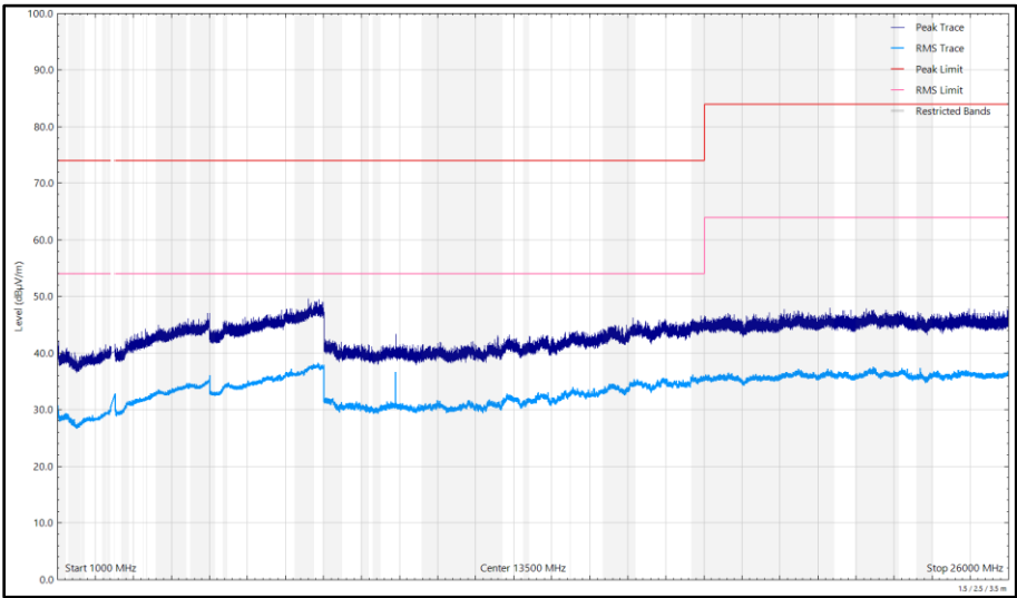
Figure 194 - 2472 MHz (CH13), 802.11b, Core 0, 1 GHz to 26 GHz, Vertical
