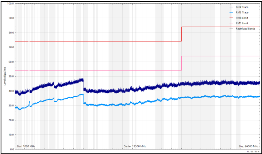
Figure 193 - 2472 MHz (CH13), 802.11b, Core 0, 1 GHz to 26 GHz, Horizontal
