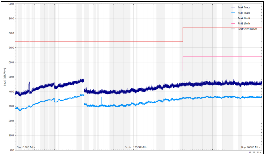
Figure 200 - 2442 MHz (CH7), 802.11b, Core 1, 1 GHz to 26 GHz, Vertical
