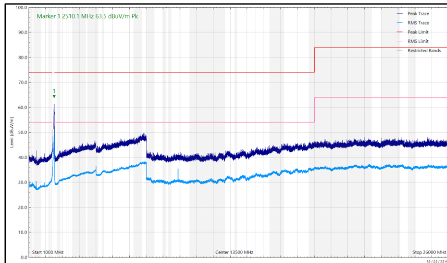
Figure 210 - 2472 MHz (CH13), 802.11g, Core 0, 1 GHz to 26 GHz, Vertical
