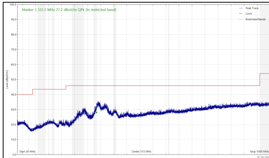
Figure 229 - 2442 MHz (CH7), HE20, RU26-0, CDD, Core 0 + Core 1, 30 MHz to 1 GHz, Horizontal (Peak)
