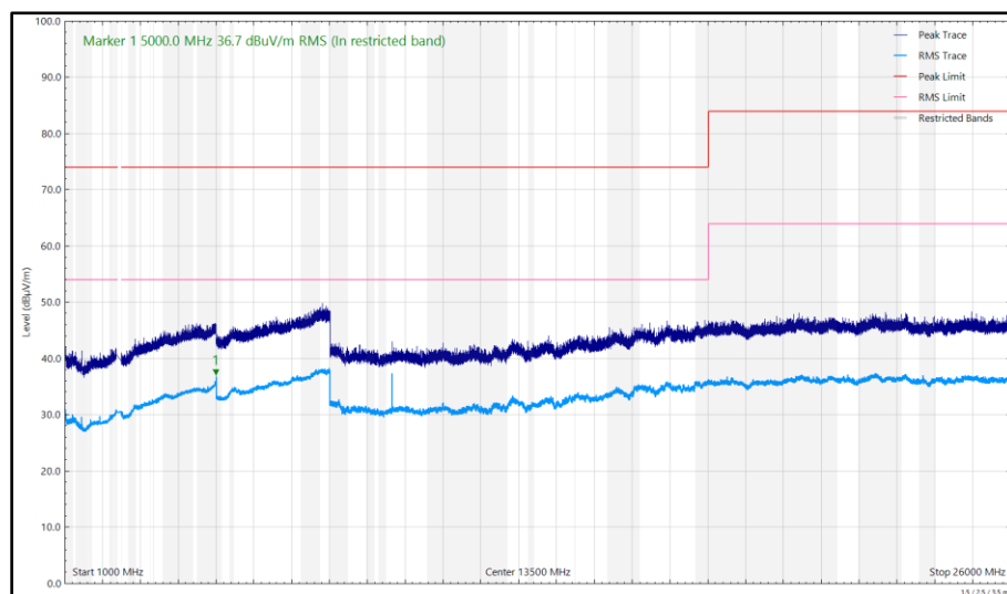
Figure 188 - 2412 MHz (CH1), 802.11b, Core 0, 1 GHz to 26 GHz, Vertical
