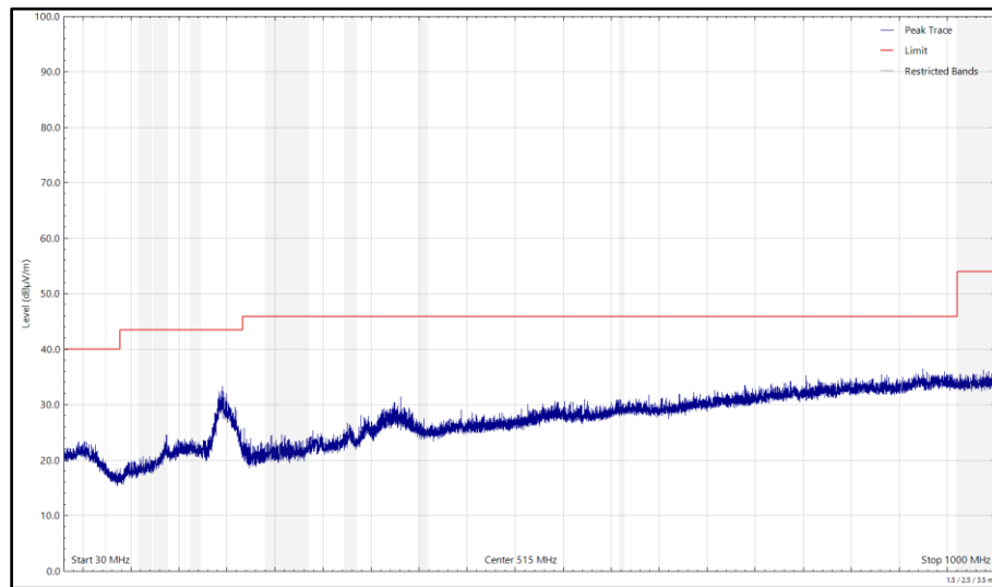
Figure 190 - 2442 MHz (CH7), 802.11b, Core 0, 30 MHz to 1 GHz, Vertical (Peak)
