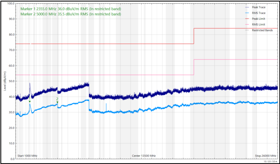
Figure 212 - 2412 MHz (CH1), 802.11g, Core 1, 1 GHz to 26 GHz, Vertical
