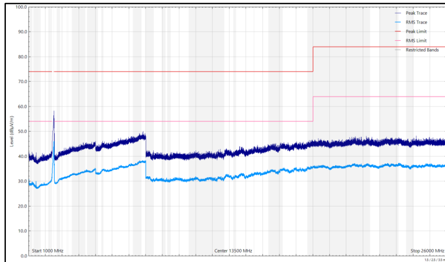
Figure 225 - 2472 MHz (CH13), HT20, CDD, Core 0 + Core 1, 1 GHz to 26 GHz, Horizontal
