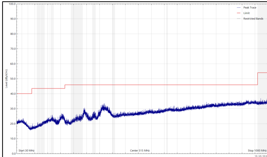
Figure 205 - 2442 MHz (CH7), 802.11g, Core 0, 30 MHz to 1 GHz, Horizontal (Peak)
