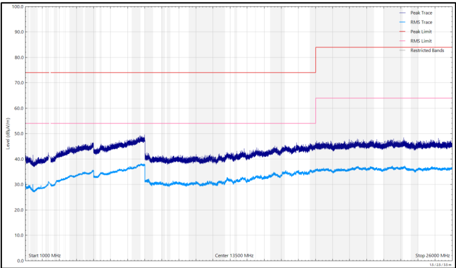
Figure 211 - 2412 MHz (CH1), 802.11g, Core 1, 1 GHz to 26 GHz, Horizontal
