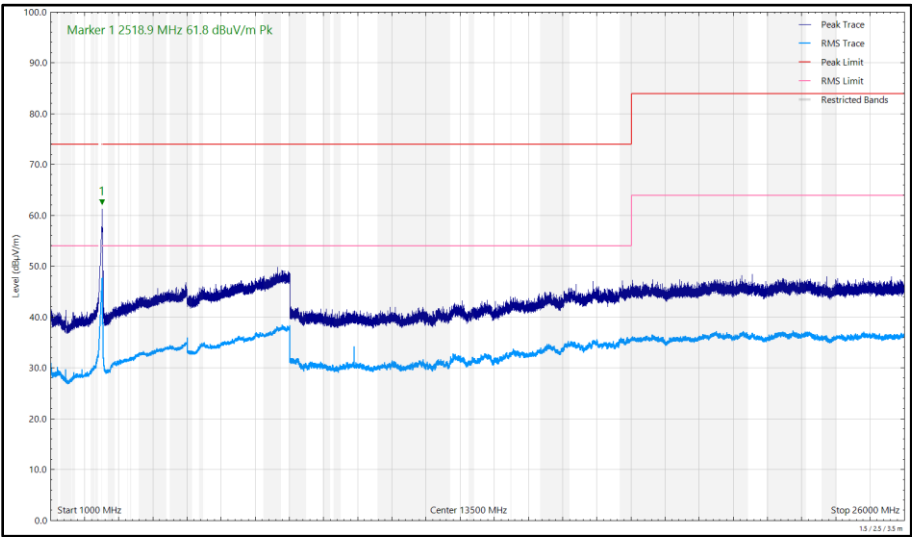
Figure 218 - 2472 MHz (CH13), 802.11g, Core 1, 1 GHz to 26 GHz, Vertical
