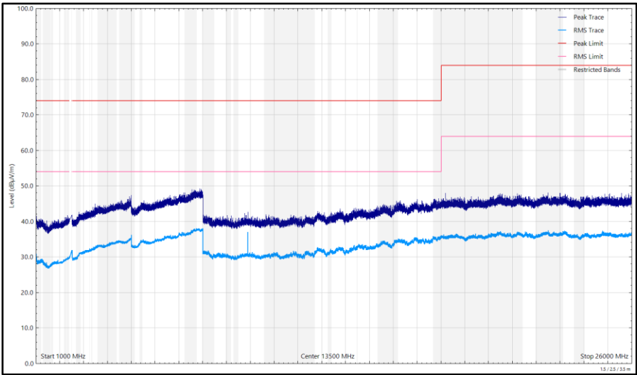
Figure 202 - 2472 MHz (CH13), 802.11b, Core 1, 1 GHz to 26 GHz, Vertical
