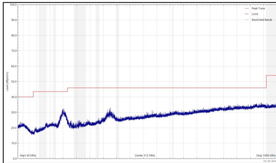
Figure 198 - 2442 MHz (CH7), 802.11b, Core 1, 30 MHz to 1 GHz, Vertical (Peak)
