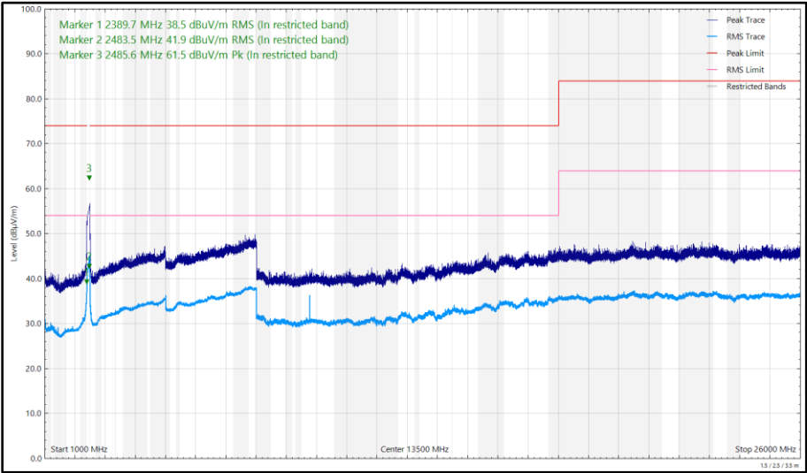
Figure 224 - 2442 MHz (CH7), HT20, CDD, Core 0 + Core 1, 1 GHz to 26 GHz, Vertical
