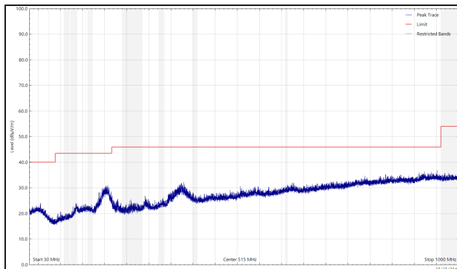
Figure 222 - 2442 MHz (CH7), HT20, CDD, Core 0 + Core 1, 30 MHz to 1 GHz, Vertical (Peak)
