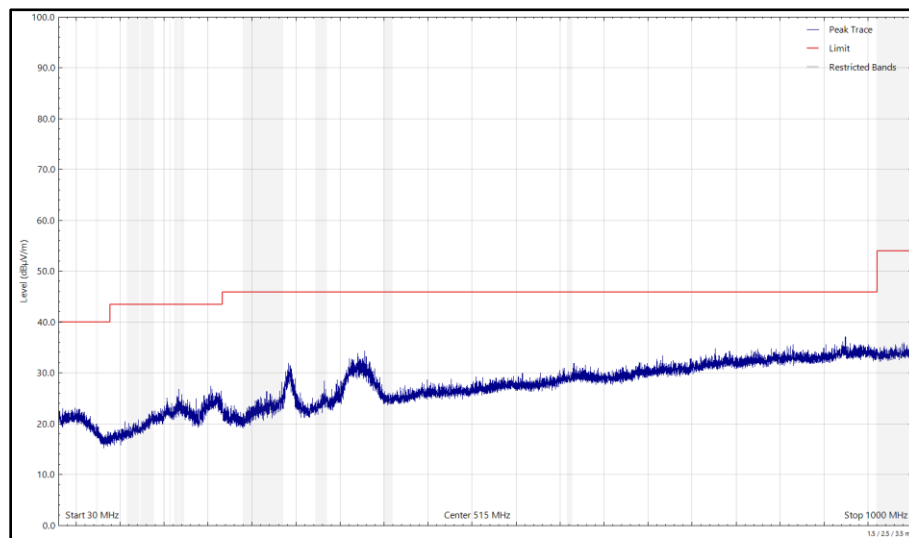
Figure 221 - 2442 MHz (CH7), HT20, CDD, Core 0 + Core 1, 30 MHz to 1 GHz, Horizontal (Peak)
