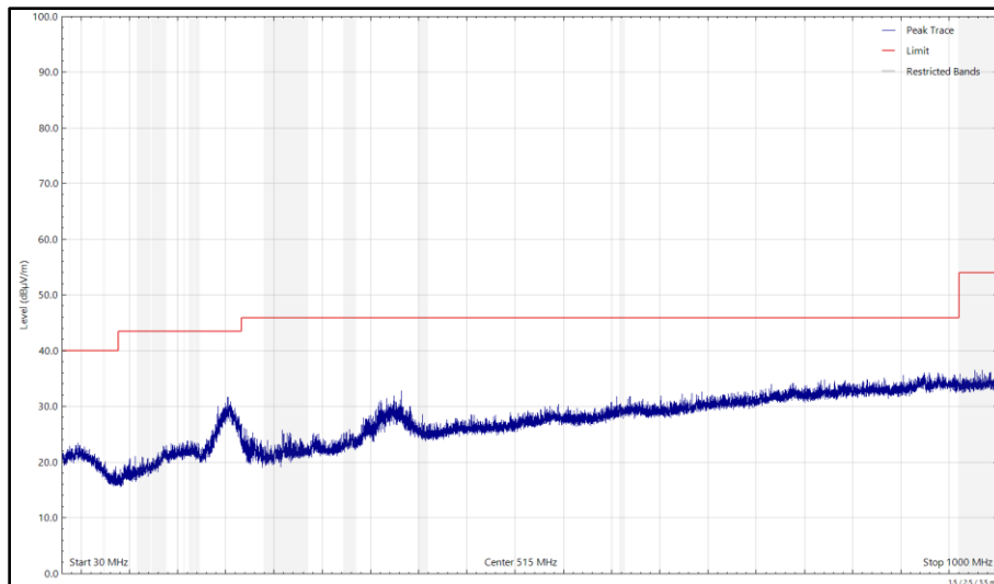
Figure 206 - 2442 MHz (CH7), 802.11g, Core 0, 30 MHz to 1 GHz, Vertical (Peak)
