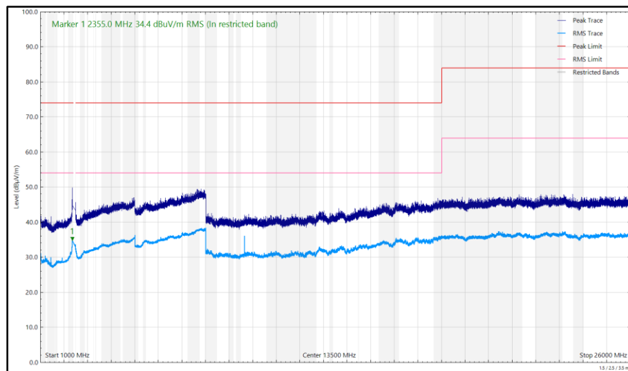
Figure 228 - 2412 MHz (CH1), HE20, RU26-0, CDD, Core 0 + Core 1, 1 GHz to 26 GHz, Vertical
