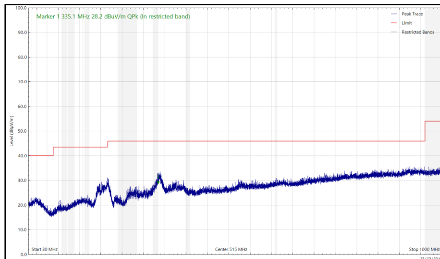
Figure 230 - 2442 MHz (CH7), HE20, RU26-0, CDD, Core 0 + Core 1, 30 MHz to 1 GHz, Vertical (Peak)
