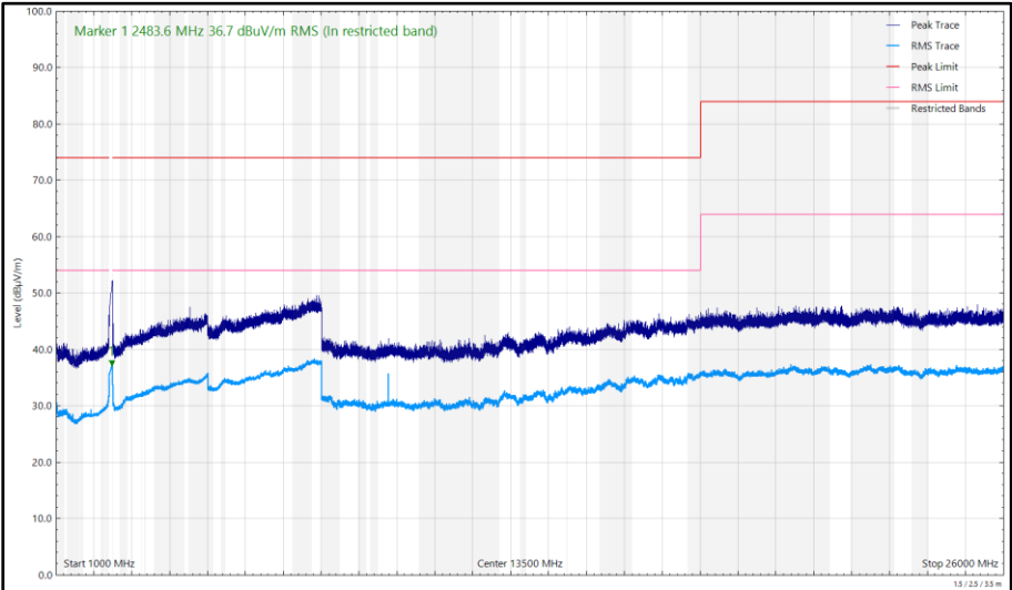
Figure 208 - 2442 MHz (CH7), 802.11g, Core 0, 1 GHz to 26 GHz, Vertical
