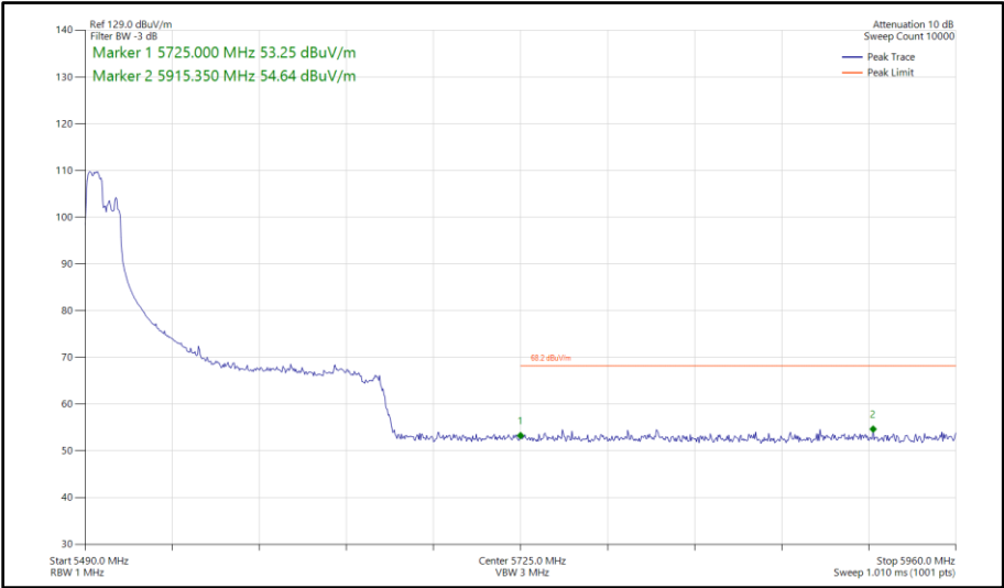
Figure 640 - 802.11ax HE160, RU 106-53P, SISO, Core 0 - 5570 MHz Band Edge Frequency 5725 MHz
