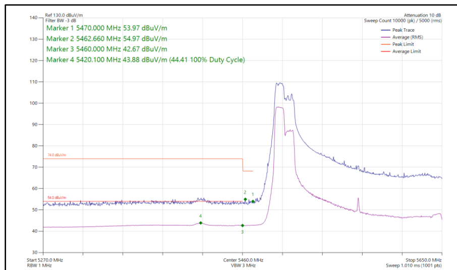
Figure 637 - 802.11ax HE160, RU 106-53P, SISO, Core 0 - 5570 MHz Band Edge Frequency 5470 MHz
