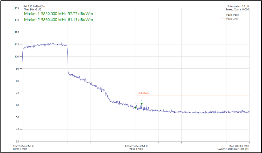
Figure 596 - 802.11ax HE80, SU, SISO, Core 1 - 5690 MHz Band Edge Frequency 5850 MHz
