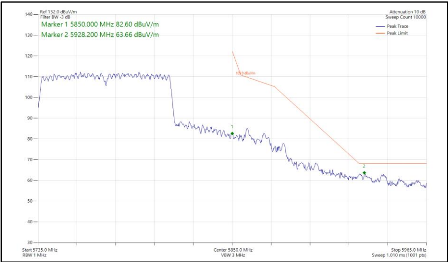
Figure 610 - 802.11ac VHT80, CDD, Core 0 - Core 1 - 5775 MHz Band Edge Frequency 5850 MHz
