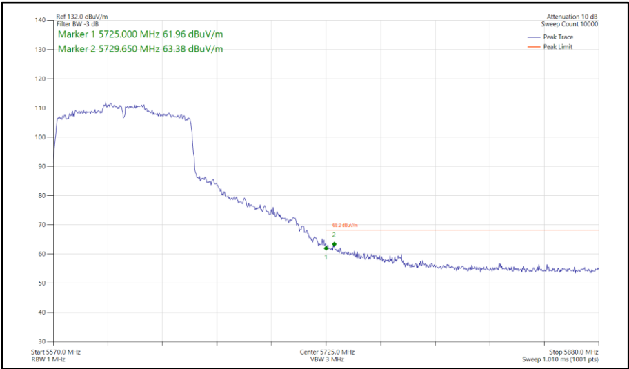
Figure 621 - 802.11ac VHT80, SDM, Core 0 - Core 1 - 5610 MHz Band Edge Frequency 5725 MHz
