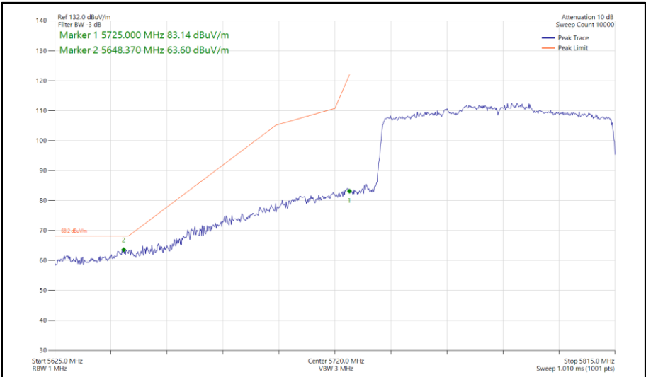
Figure 619 - 802.11ax HE80, SU, SDM, Core 0 - Core 1 - 5775 MHz Band Edge Frequency 5725 MHz
