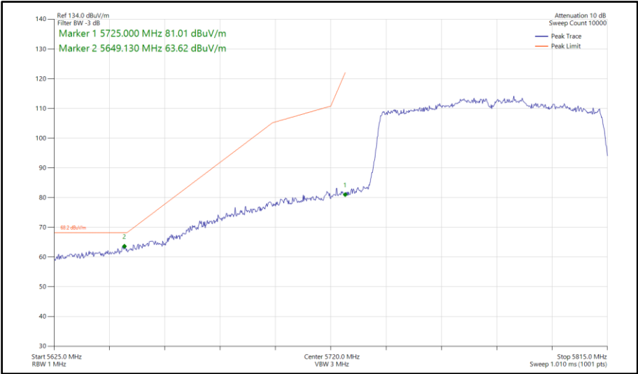
Figure 573 - 802.11ac VHT80, SISO, Core 0 - 5775 MHz Band Edge Frequency 5725 MHz
