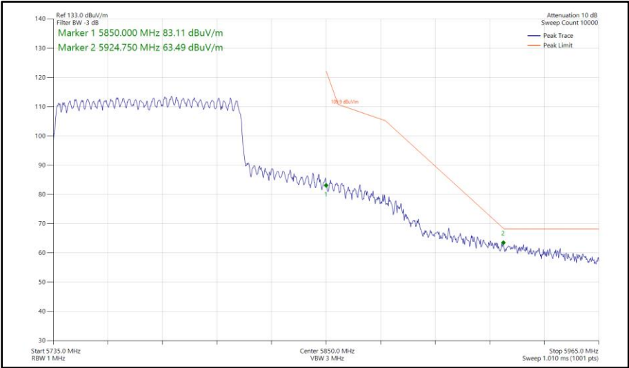
Figure 613 - 802.11ax HE80, SU, CDD, Core 0 - Core 1 - 5775 MHz Band Edge Frequency 5850 MHz
