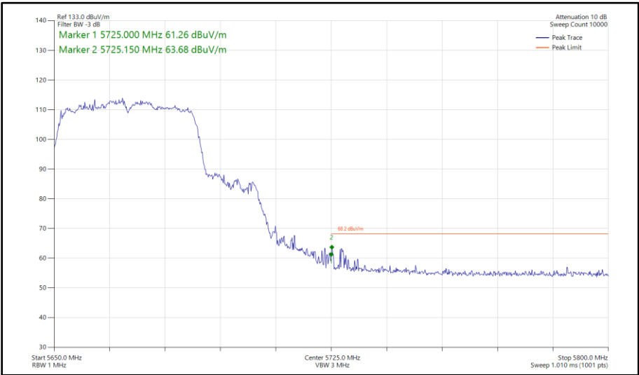
Figure 567 - 802.11ac VHT40, TxBF, Core 0 - Core 1 - 5670 MHz Band Edge Frequency 5725 MHz
