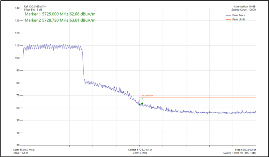
Figure 607 - 802.11ax HE80, SU, CDD, Core 0 - Core 1 - 5610 MHz Band Edge Frequency 5725 MHz
