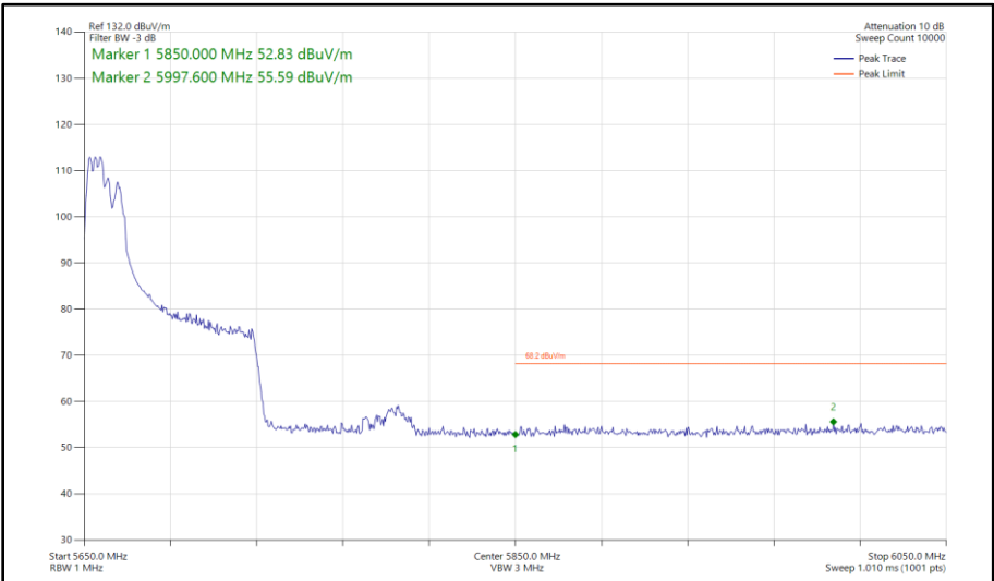
Figure 612 - 802.11ax HE80, RU 106-53, CDD, Core 0 - Core 1 - 5690 MHz Band Edge Frequency 5850 MHz
