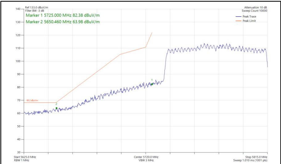
Figure 604 - 802.11ax HE80, SU, CDD, Core 0 - Core 1 - 5775 MHz Band Edge Frequency 5725 MHz
