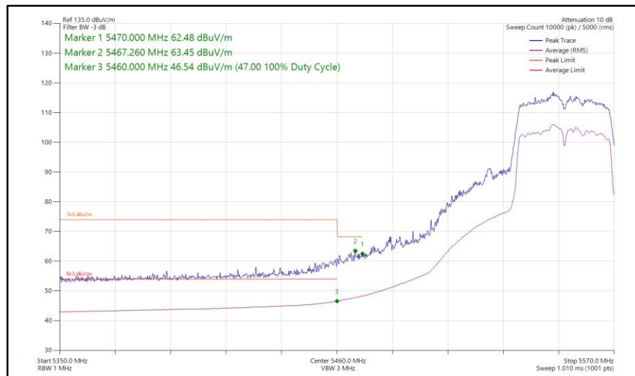
Figure 564 - 802.11ac VHT40, TxBF, Core 0 - Core 1 - 5550 MHz Band Edge Frequency 5470 MHz
