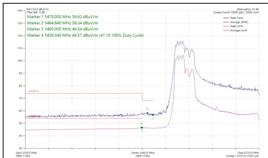
Figure 602 - 802.11ax HE80, RU 106-53, CDD, Core 0 - Core 1 - 5530 MHz Band Edge Frequency 5470 MHz
