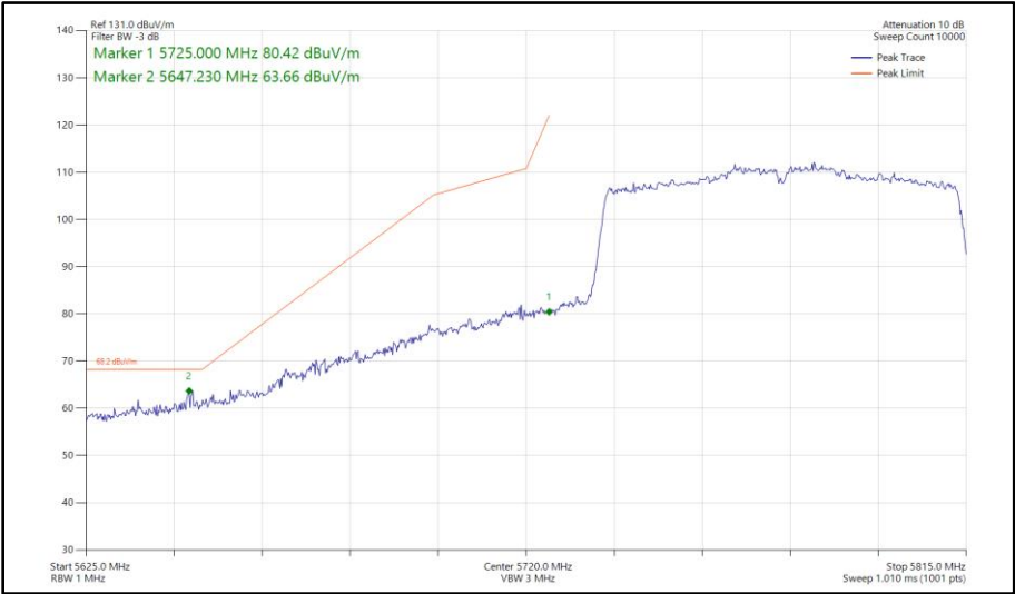
Figure 588 - 802.11ac VHT80, SISO, Core 1 - 5775 MHz Band Edge Frequency 5725 MHz
