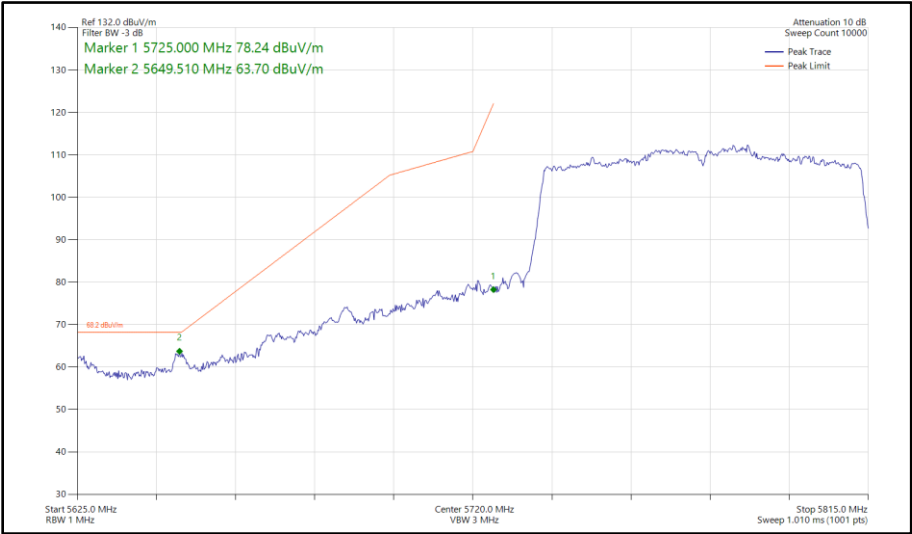
Figure 618 - 802.11ac VHT80, SDM, Core 0 - Core 1 - 5775 MHz Band Edge Frequency 5725 MHz
