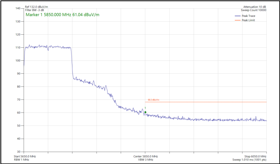
Figure 624 - 802.11ac VHT80, SDM, Core 0 - Core 1 - 5690 MHz Band Edge Frequency 5850 MHz
