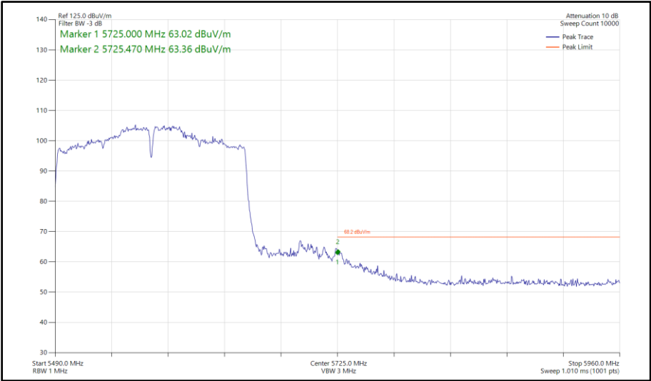
Figure 644 - 802.11ac VHT160, SISO, Core 1 - 5570 MHz Band Edge Frequency 5725 MHz
