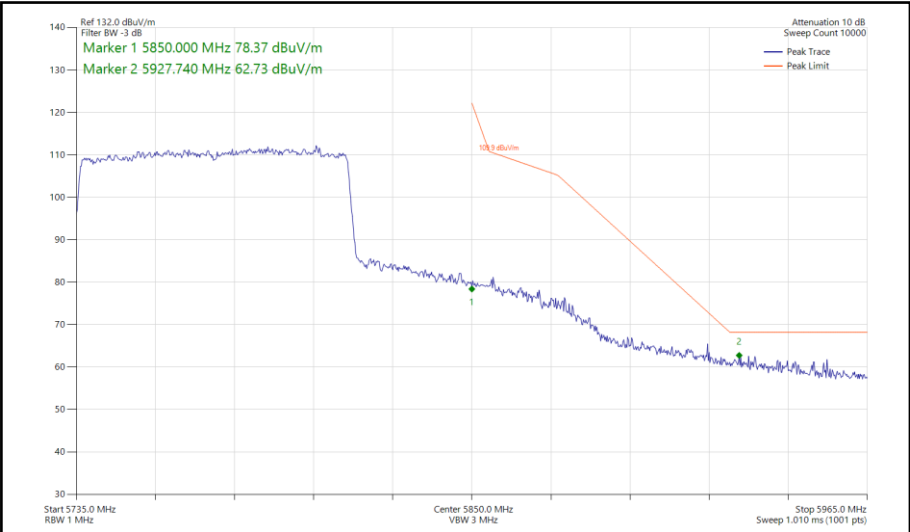
Figure 598 - 802.11ax HE80, SU, SISO, Core 1 - 5775 MHz Band Edge Frequency 5850 MHz
