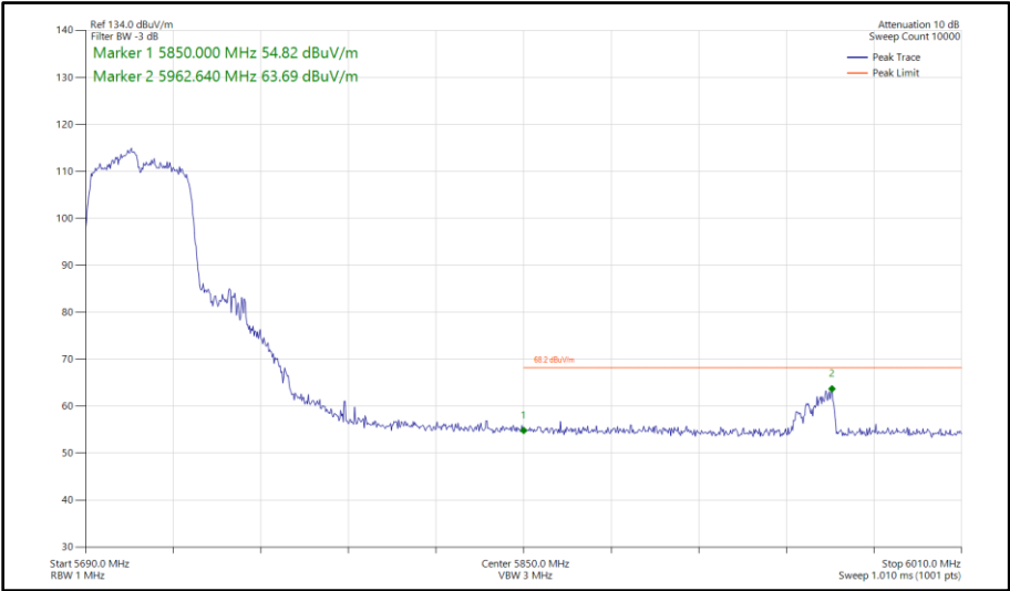
Figure 568 - 802.11ac VHT40, TxBF, Core 0 - Core 1 - 5710 MHz Band Edge Frequency 5850 MHz
