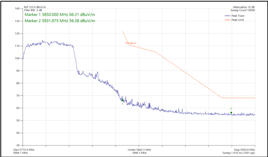
Figure 569 - 802.11ac VHT40, TxBF, Core 0 - Core 1 - 5795 MHz Band Edge Frequency 5850 MHz
