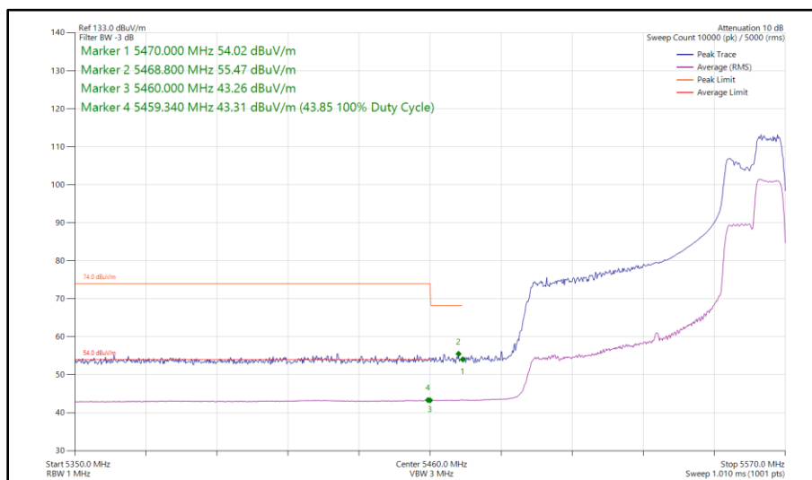
Figure 587 - 802.11ax HE80, RU 106-60, SISO, Core 1 - 5530 MHz Band Edge Frequency 5470 MHz
