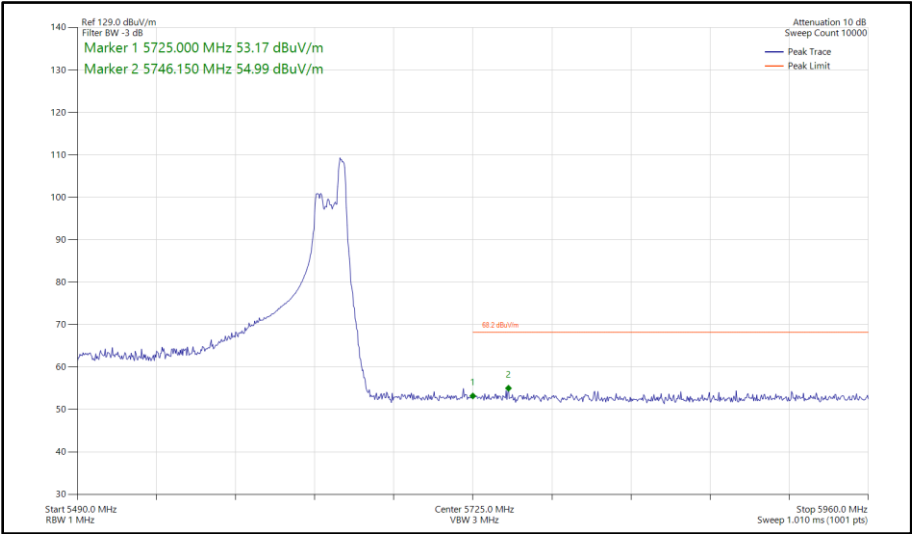
Figure 646 - 802.11ax HE160, RU 52-52S, SISO, Core 1 - 5570 MHz Band Edge Frequency 5725 MHz
