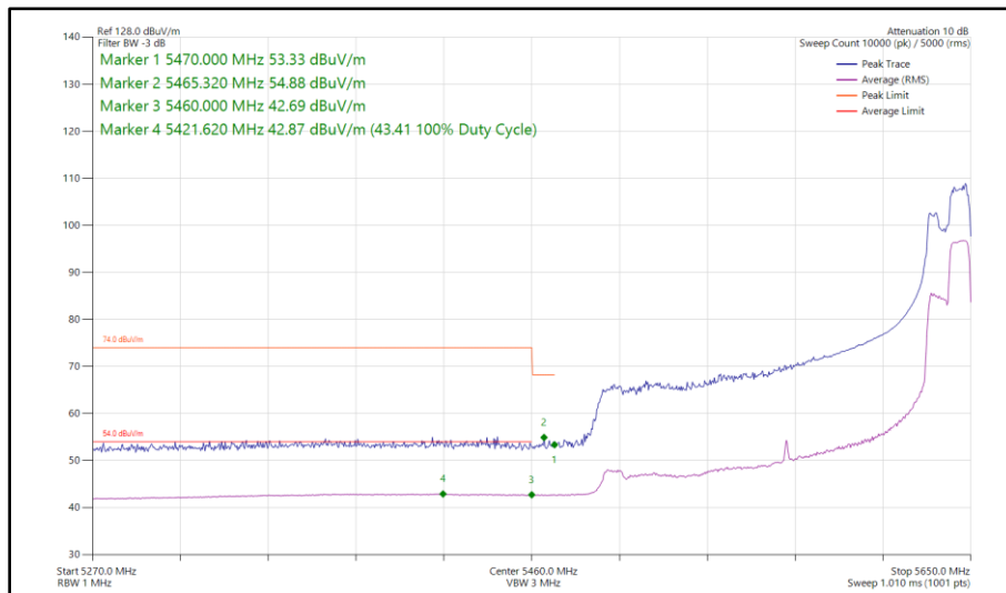
Figure 643 - 802.11ax HE160, RU 106-60S, SISO, Core 1 - 5570 MHz Band Edge Frequency 5470 MHz
