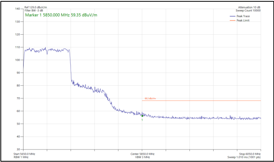
Figure 633 - 802.11ac VHT80, TxBF, Core 0 - Core 1 - 5690 MHz Band Edge Frequency 5850 MHz
