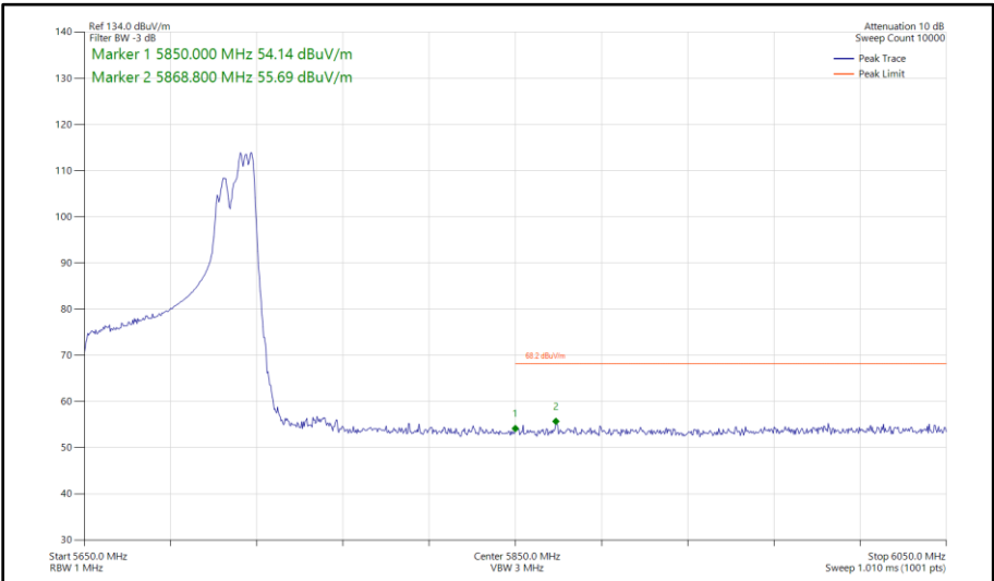
Figure 627 - 802.11ax HE80, RU 106-60, SDM, Core 0 - Core 1 - 5690 MHz Band Edge Frequency 5850 MHz
