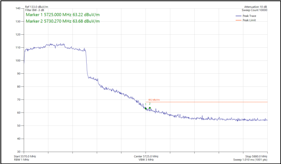
Figure 577 - 802.11ax HE80, SU, SISO, Core 0 - 5610 MHz Band Edge Frequency 5725 MHz
