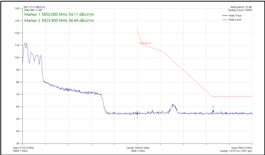
Figure 629 - 802.11ax HE80, RU 52-37, SDM, Core 0 - Core 1 - 5775 MHz Band Edge Frequency 5850 MHz
