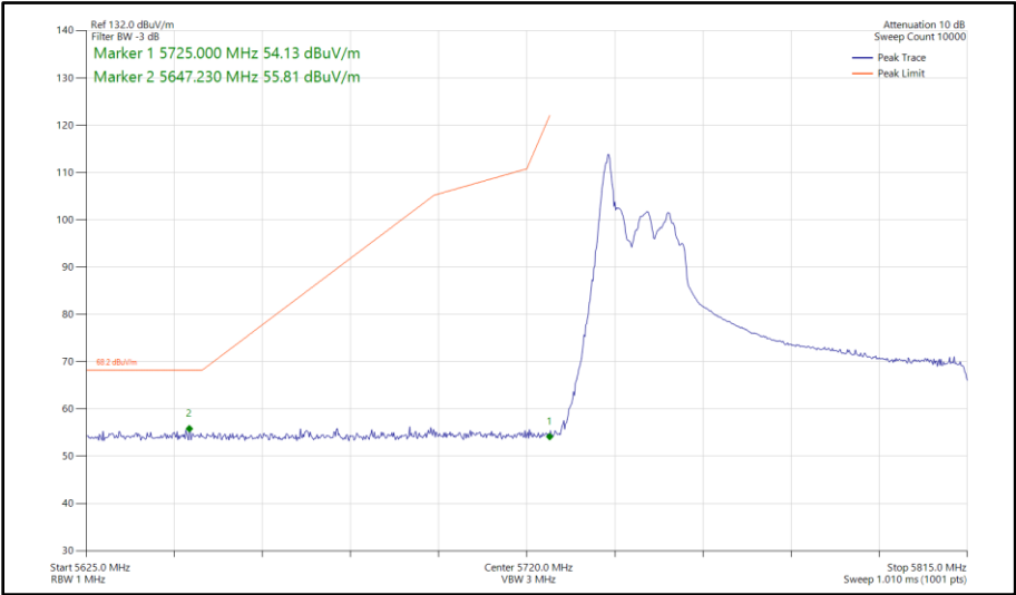
Figure 620 - 802.11ax HE80, RU 26-0, SDM, Core 0 - Core 1 - 5775 MHz Band Edge Frequency 5725 MHz
