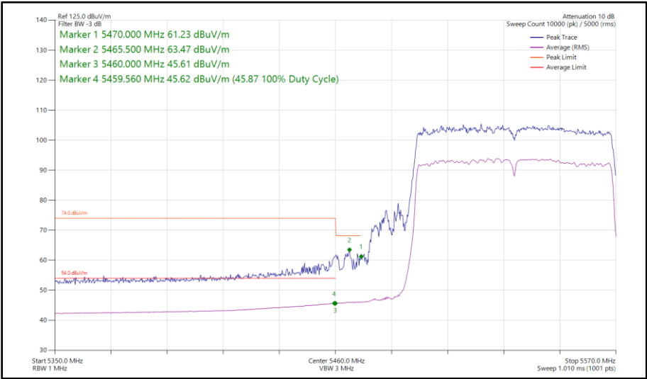
Figure 630 - 802.11ac VHT80, TxBF, Core 0 - Core 1 - 5530 MHz Band Edge Frequency 5470 MHz
