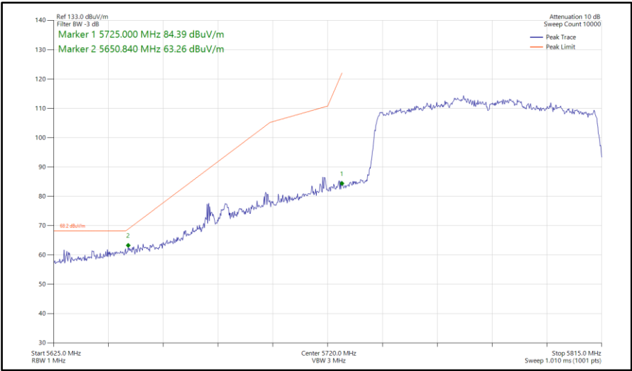
Figure 631 - 802.11ac VHT80, TxBF, Core 0 - Core 1 - 5775 MHz Band Edge Frequency 5725 MHz
