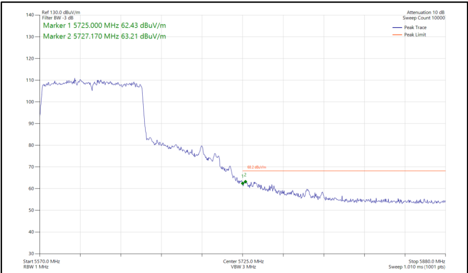
Figure 576 - 802.11ac VHT80, SISO, Core 0 - 5610 MHz Band Edge Frequency 5725 MHz
