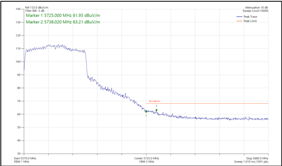
Figure 606 - 802.11ac VHT80, CDD, Core 0 - Core 1 - 5610 MHz Band Edge Frequency 5725 MHz
