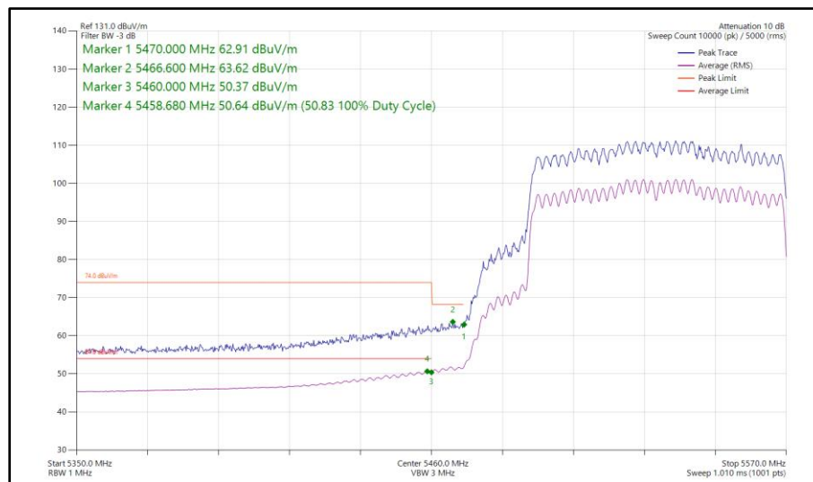
Figure 601 - 802.11ax HE80, SU, CDD, Core 0 - Core 1 - 5530 MHz Band Edge Frequency 5470 MHz
