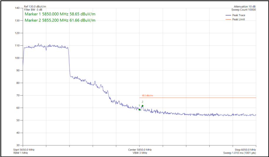
Figure 579 - 802.11ac VHT80, SISO, Core 0 - 5690 MHz Band Edge Frequency 5850 MHz
