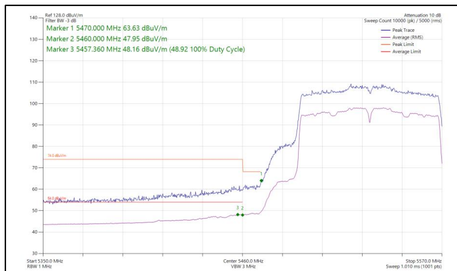
Figure 585 - 802.11ac VHT80, SISO, Core 1 - 5530 MHz Band Edge Frequency 5470 MHz
