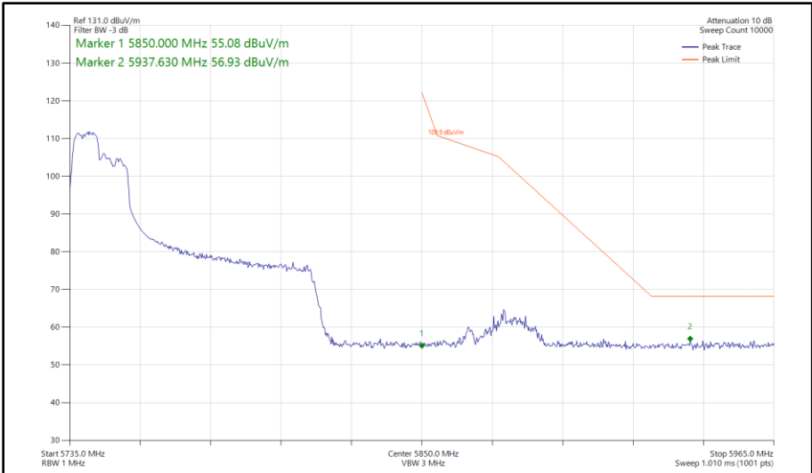
Figure 599 - 802.11ax HE80, RU 106-53, SISO, Core 1 - 5775 MHz Band Edge Frequency 5850 MHz
