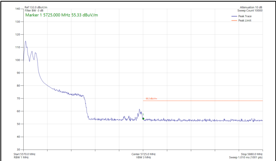
Figure 623 - 802.11ax HE80, RU 52-37, SDM, Core 0 - Core 1 - 5610 MHz Band Edge Frequency 5725 MHz
