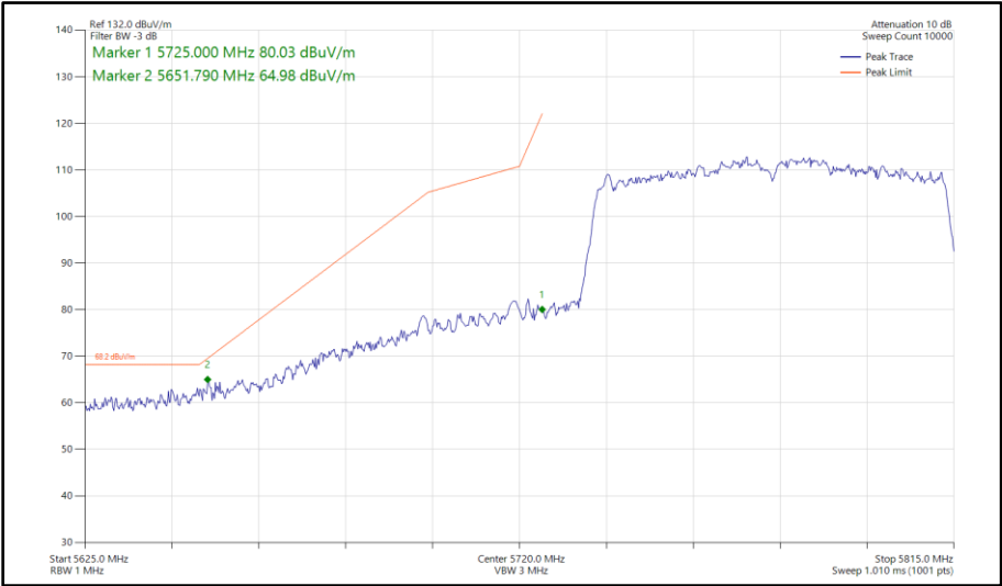
Figure 603 - 802.11ac VHT80, CDD, Core 0 - Core 1 - 5775 MHz Band Edge Frequency 5725 MHz
