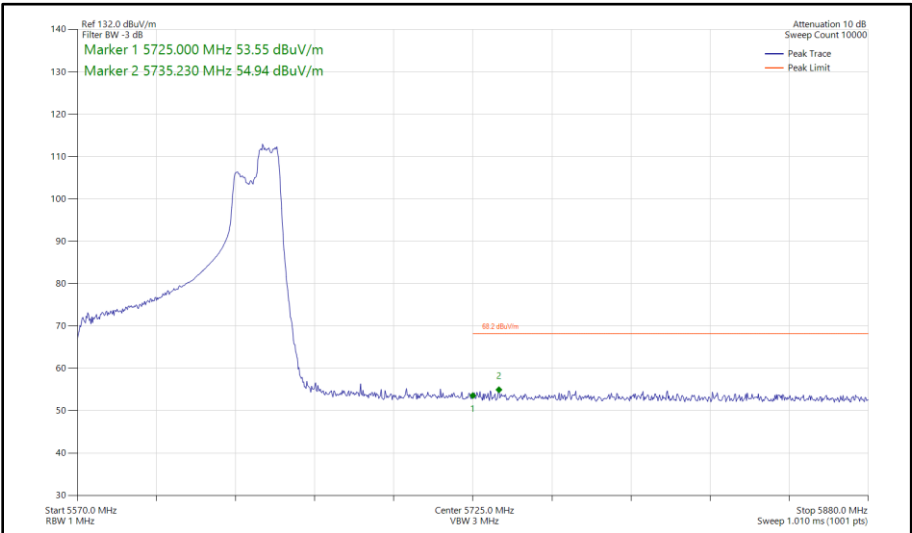
Figure 593 - 802.11ax HE80, RU 106-60, SISO, Core 1 - 5610 MHz Band Edge Frequency 5725 MHz
