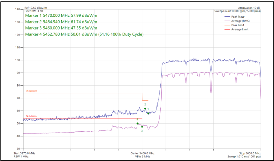
Figure 635 - 802.11ac VHT160, SISO, Core 0 - 5570 MHz Band Edge Frequency 5470 MHz
