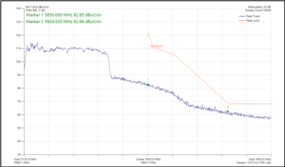
Figure 634 - 802.11ac VHT80, TxBF, Core 0 - Core 1 - 5775 MHz Band Edge Frequency 5850 MHz
