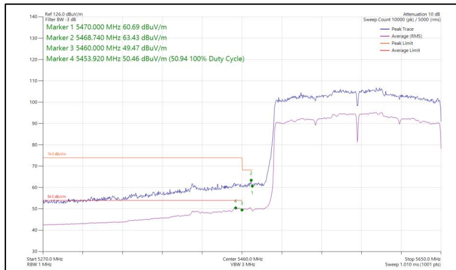
Figure 636 - 802.11ax HE160, SU, SISO, Core 0 - 5570 MHz Band Edge Frequency 5470 MHz
