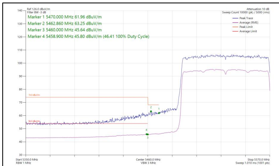
Figure 571 - 802.11ax HE80, SU, SISO, Core 0 - 5530 MHz Band Edge Frequency 5470 MHz
