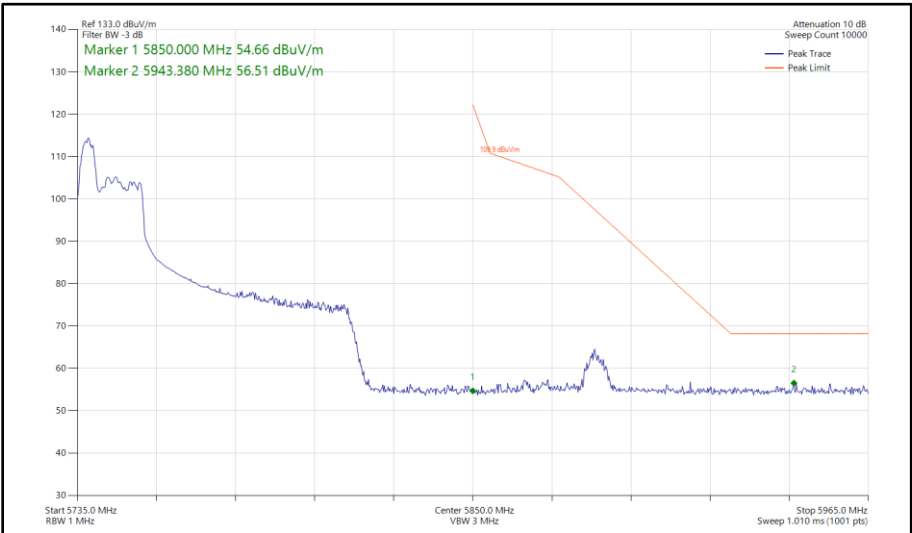
Figure 584 - 802.11ax HE80, RU 52-37, SISO, Core 0 - 5775 MHz Band Edge Frequency 5850 MHz
