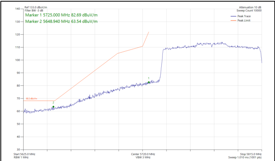
Figure 574 - 802.11ax HE80, SU, SISO, Core 0 - 5775 MHz Band Edge Frequency 5725 MHz
