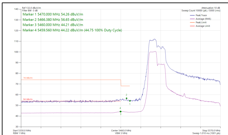
Figure 572 - 802.11ax HE80, RU 106-53, SISO, Core 0 - 5530 MHz Band Edge Frequency 5470 MHz
