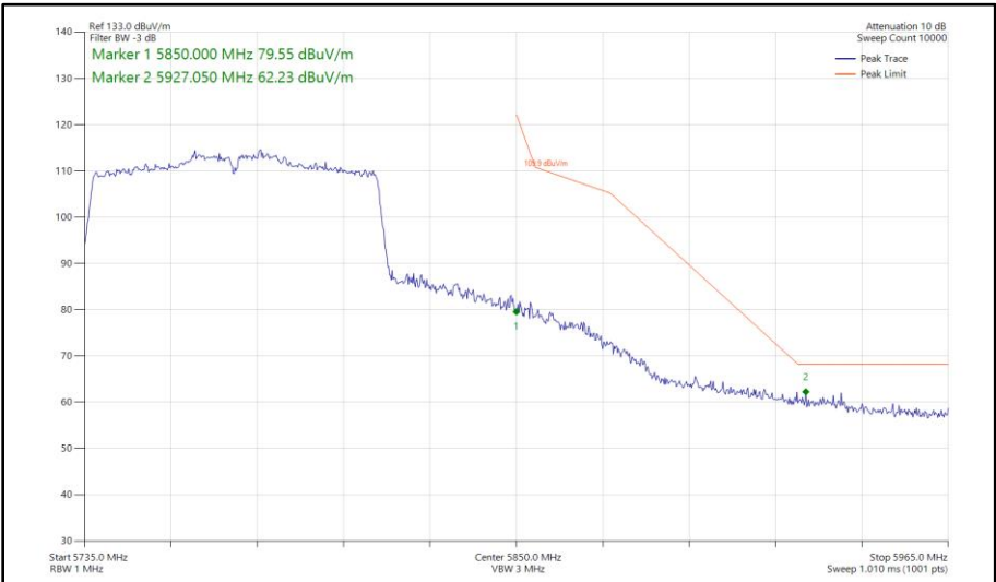
Figure 580 - 802.11ac VHT80, SISO, Core 0 - 5775 MHz Band Edge Frequency 5850 MHz
