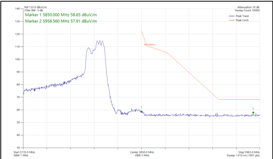
Figure 614 - 802.11ax HE80, RU 106-60, CDD, Core 0 - Core 1 - 5775 MHz Band Edge Frequency 5850 MHz
