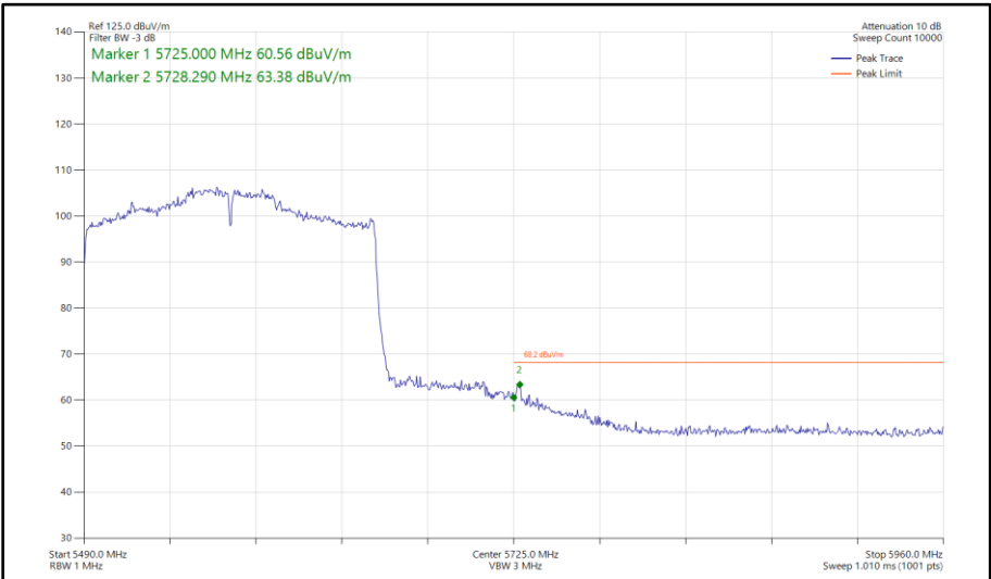
Figure 639 - 802.11ax HE160, SU, SISO, Core 0 - 5570 MHz Band Edge Frequency 5725 MHz
