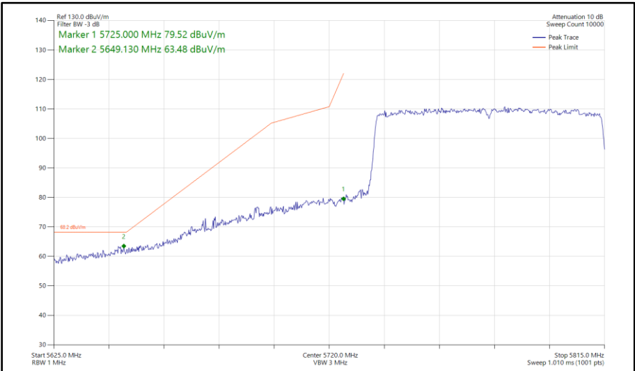
Figure 589 - 802.11ax HE80, SU, SISO, Core 1 - 5775 MHz Band Edge Frequency 5725 MHz
