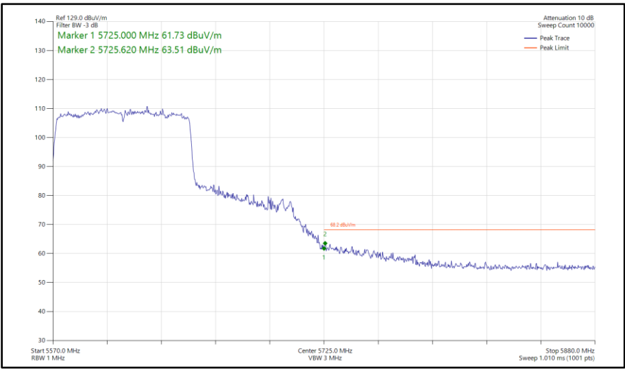
Figure 632 - 802.11ac VHT80, TxBF, Core 0 - Core 1 - 5610 MHz Band Edge Frequency 5725 MHz
