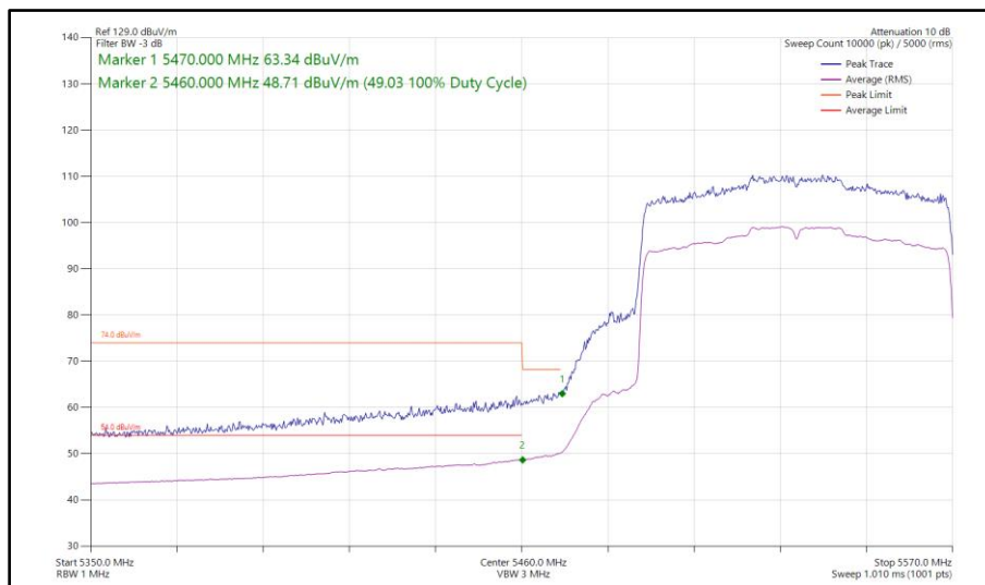
Figure 586 - 802.11ax HE80, SU, SISO, Core 1 - 5530 MHz Band Edge Frequency 5470 MHz
