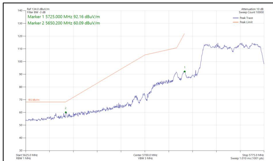
Figure 565 - 802.11ac VHT40, TxBF, Core 0 - Core 1 - 5755 MHz Band Edge Frequency 5725 MHz
