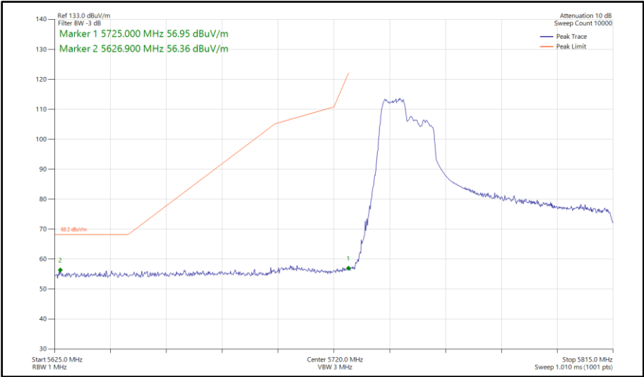
Figure 575 - 802.11ax HE80, RU 106-53, SISO, Core 0 - 5775 MHz Band Edge Frequency 5725 MHz
