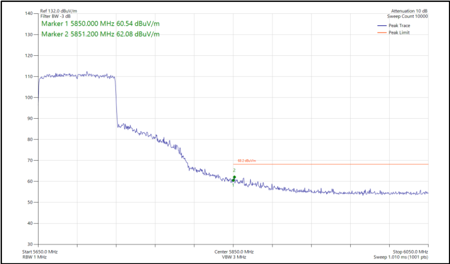
Figure 581 - 802.11ax HE80, SU, SISO, Core 0 - 5690 MHz Band Edge Frequency 5850 MHz
