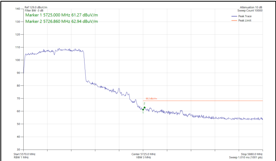
Figure 591 - 802.11ac VHT80, SISO, Core 1 - 5610 MHz Band Edge Frequency 5725 MHz
