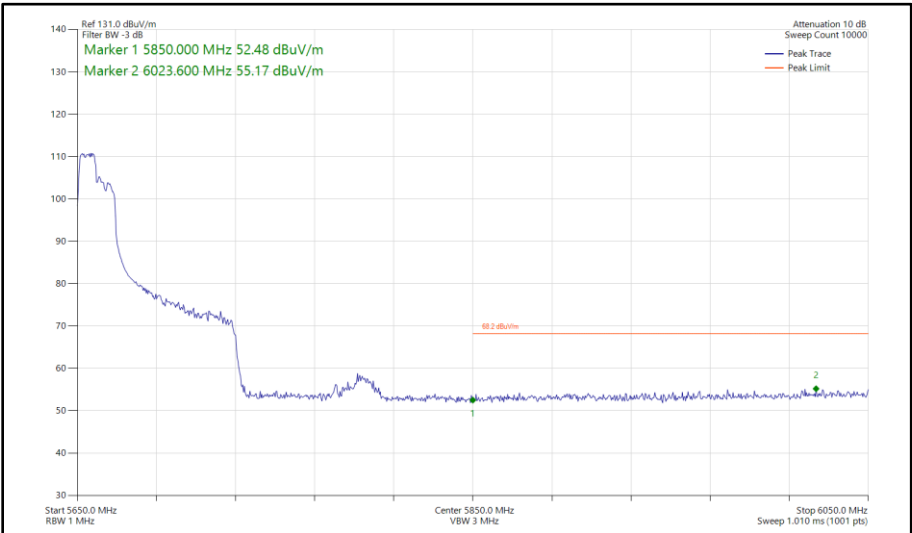
Figure 597 - 802.11ax HE80, RU 106-53, SISO, Core 1 - 5690 MHz Band Edge Frequency 5850 MHz
