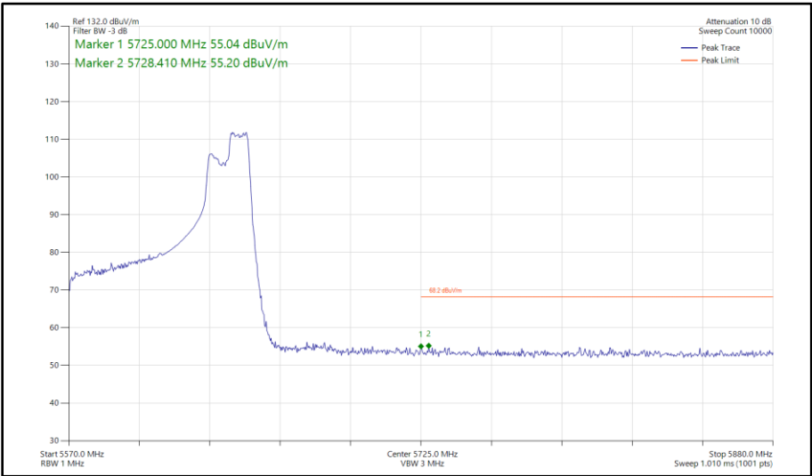
Figure 578 - 802.11ax HE80, RU 106-60, SISO, Core 0 - 5610 MHz Band Edge Frequency 5725 MHz
