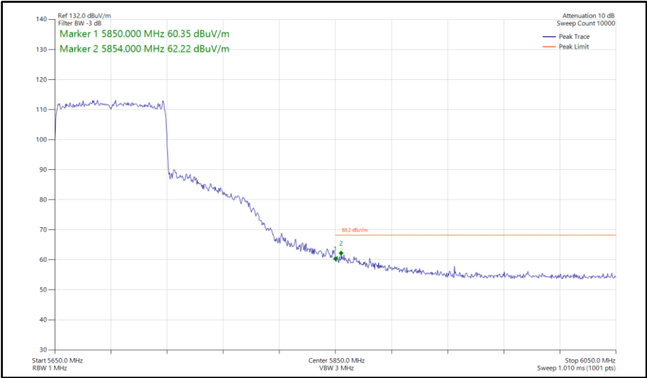
Figure 626 - 802.11ax HE80, SU, SDM, Core 0 - Core 1 - 5690 MHz Band Edge Frequency 5850 MHz
