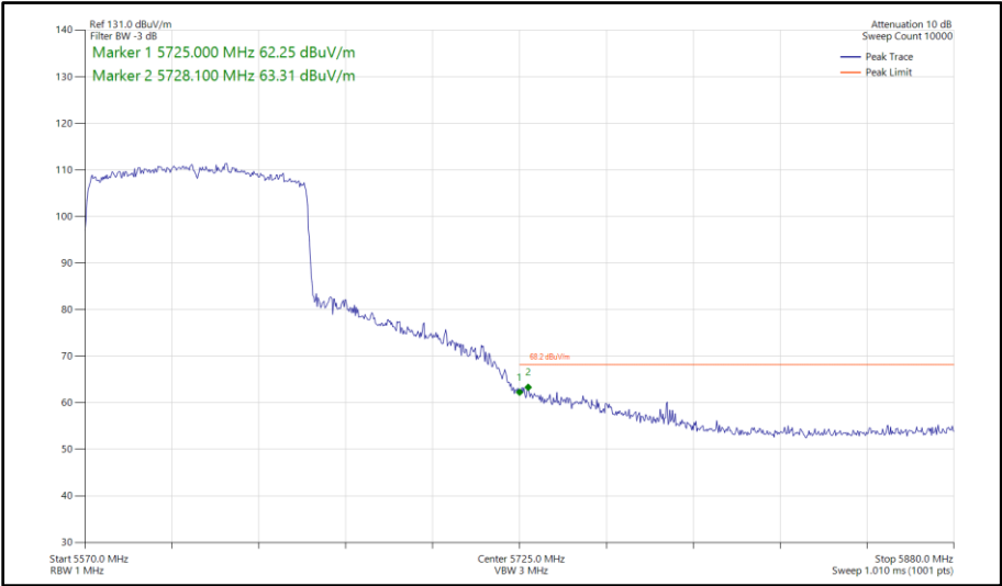
Figure 592 - 802.11ax HE80, SU, SISO, Core 1 - 5610 MHz Band Edge Frequency 5725 MHz
