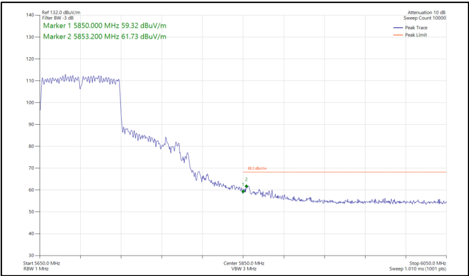
Figure 609 - 802.11ac VHT80, CDD, Core 0 - Core 1 - 5690 MHz Band Edge Frequency 5850 MHz
