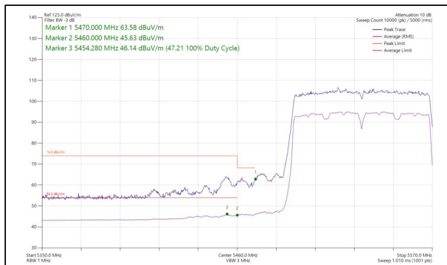
Figure 570 - 802.11ac VHT80, SISO, Core 0 - 5530 MHz Band Edge Frequency 5470 MHz
