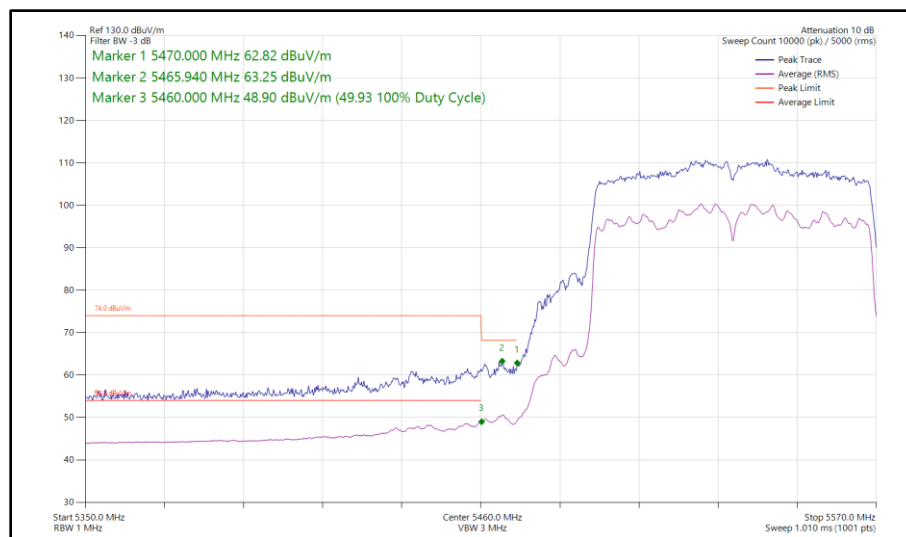
Figure 615 - 802.11ac VHT80, SDM, Core 0 - Core 1 - 5530 MHz Band Edge Frequency 5470 MHz
