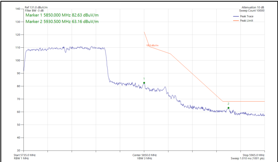
Figure 625 - 802.11ac VHT80, SDM, Core 0 - Core 1 - 5775 MHz Band Edge Frequency 5850 MHz
