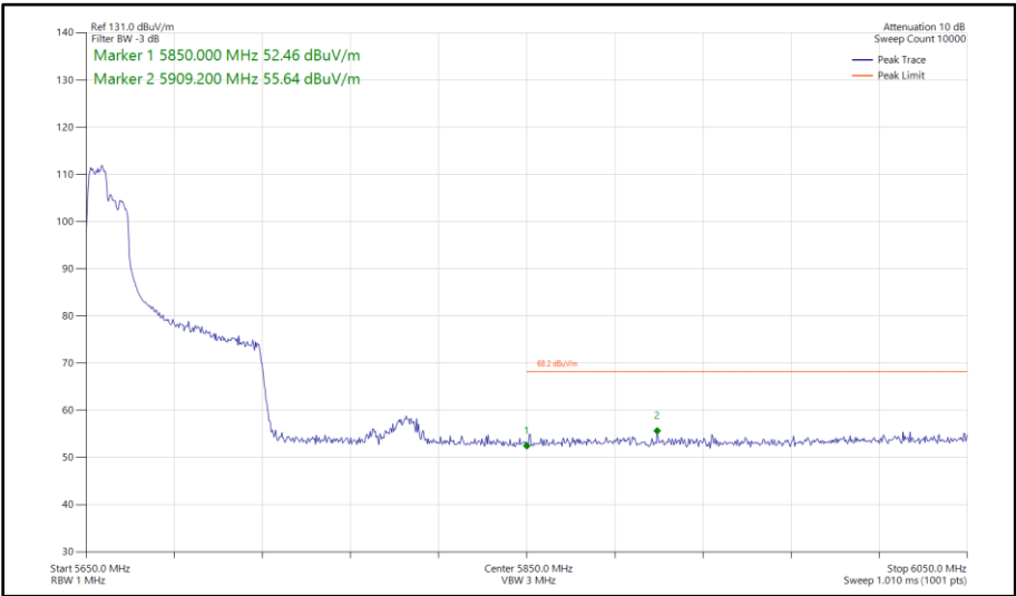
Figure 582 - 802.11ax HE80, RU 106-53, SISO, Core 0 - 5690 MHz Band Edge Frequency 5850 MHz
