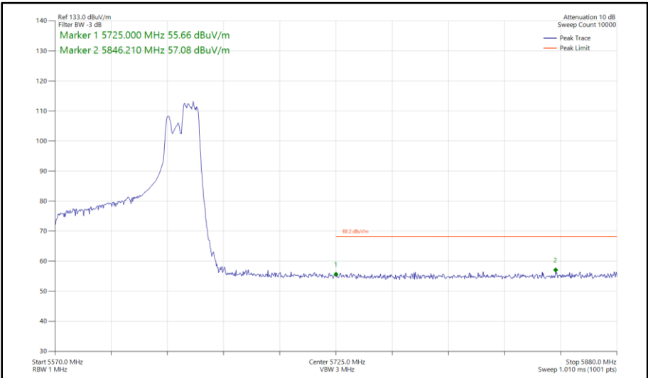
Figure 608 - 802.11ax HE80, RU 106-60, CDD, Core 0 - Core 1 - 5610 MHz Band Edge Frequency 5725 MHz
