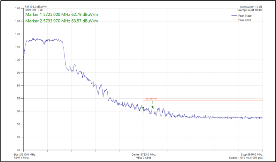
Figure 566 - 802.11ac VHT40, TxBF, Core 0 - Core 1 - 5630 MHz Band Edge Frequency 5725 MHz
