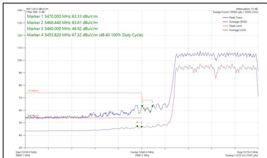
Figure 600 - 802.11ac VHT80, CDD, Core 0 - Core 1 - 5530 MHz Band Edge Frequency 5470 MHz
