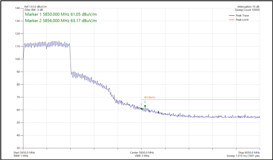
Figure 611 - 802.11ax HE80, SU, CDD, Core 0 - Core 1 - 5690 MHz Band Edge Frequency 5850 MHz
