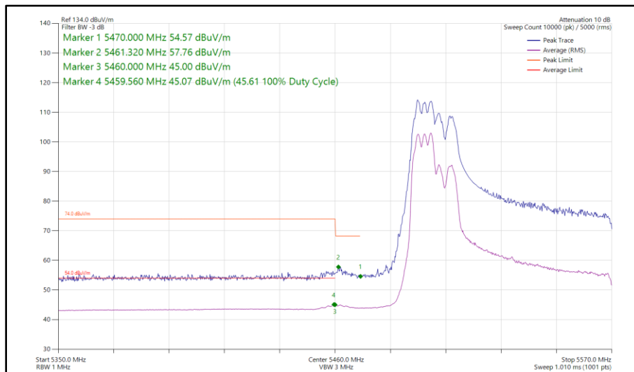
Figure 617 - 802.11ax HE80, RU 106-53, SDM, Core 0 - Core 1 - 5530 MHz Band Edge Frequency 5470 MHz
