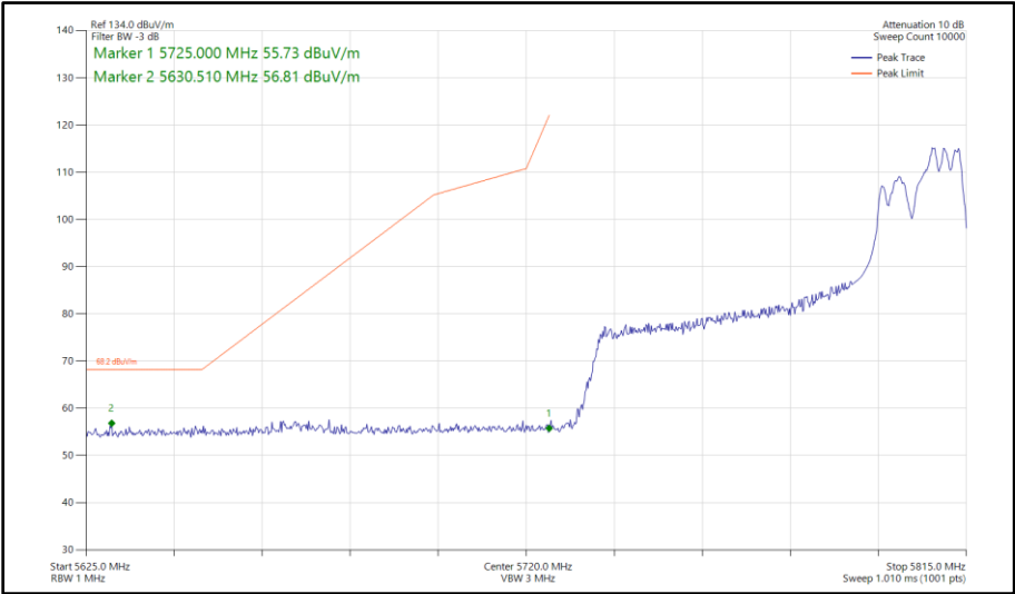
Figure 605 - 802.11ax HE80, RU 106-60, CDD, Core 0 - Core 1 - 5775 MHz Band Edge Frequency 5725 MHz
