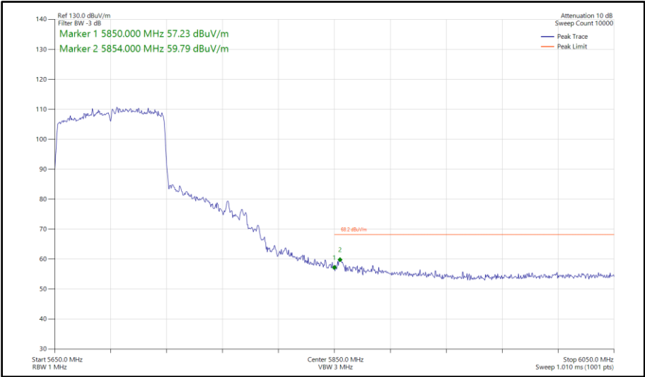
Figure 594 - 802.11ac VHT80, SISO, Core 1 - 5690 MHz Band Edge Frequency 5850 MHz
