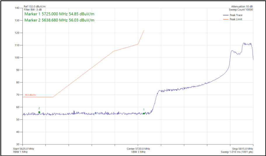
Figure 590 - 802.11ax HE80, RU 106-60, SISO, Core 1 - 5775 MHz Band Edge Frequency 5725 MHz
