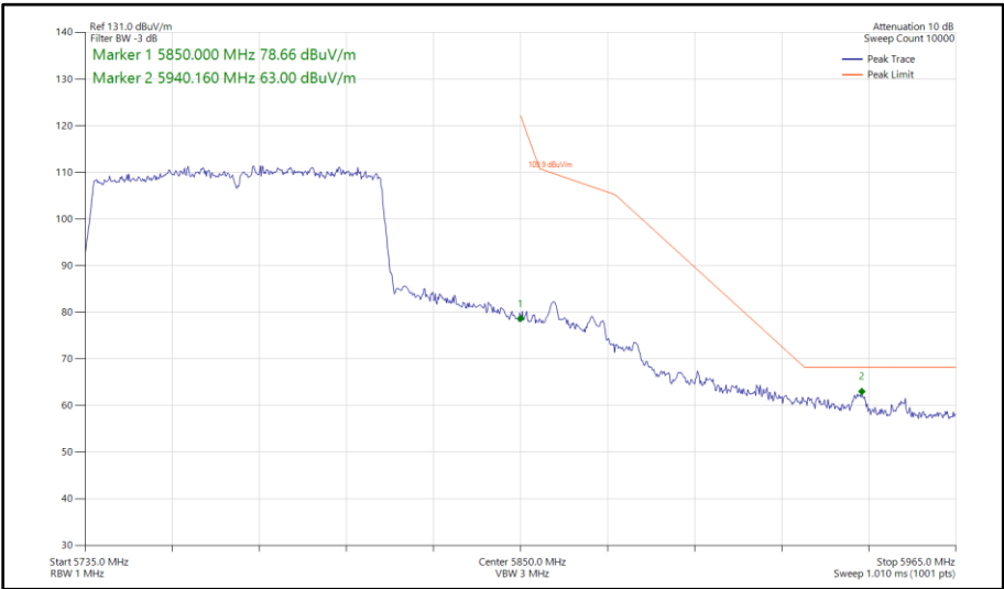
Figure 595 - 802.11ac VHT80, SISO, Core 1 - 5775 MHz Band Edge Frequency 5850 MHz
