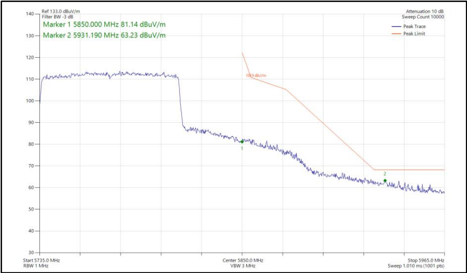
Figure 583 - 802.11ax HE80, SU, SISO, Core 0 - 5775 MHz Band Edge Frequency 5850 MHz
