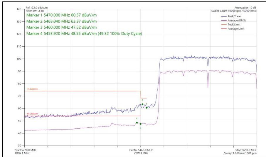
Figure 642 - 802.11ax HE160, SU, SISO, Core 1 - 5570 MHz Band Edge Frequency 5470 MHz
