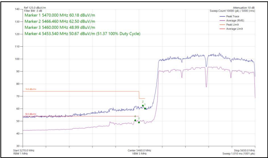
Figure 641 - 802.11ac VHT160, SISO, Core 1 - 5570 MHz Band Edge Frequency 5470 MHz
