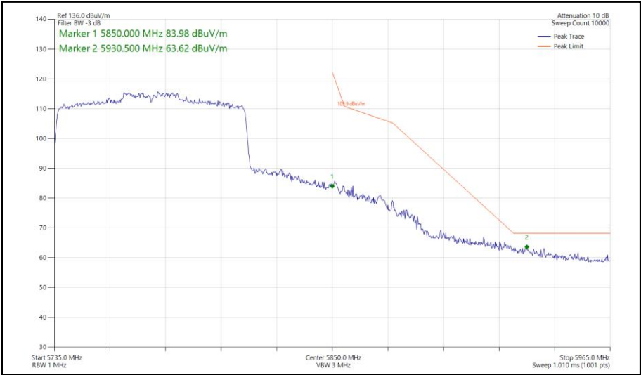
Figure 628 - 802.11ax HE80, SU, SDM, Core 0 - Core 1 - 5775 MHz Band Edge Frequency 5850 MHz
