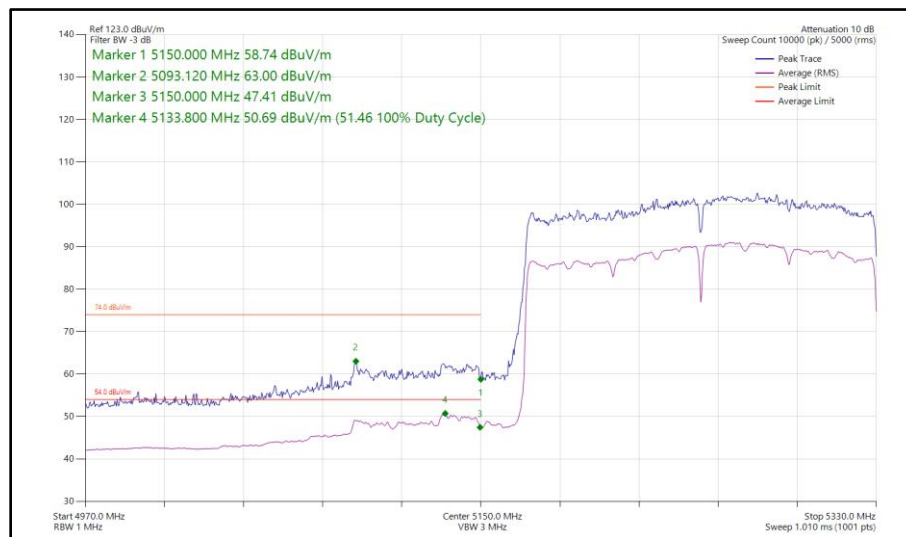
Figure 222 - 802.11ax HE160, SU, SISO, Core 1 - 5250 MHz Band Edge Frequency 5150 MHz
