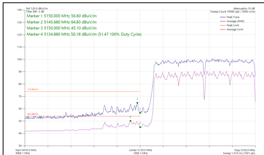
Figure 239 - 802.11ac VHT160, SDM, Core 0 - Core 1 - 5250 MHz Band Edge Frequency 5150 MHz
