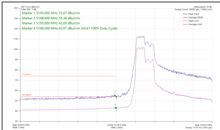
Figure 202 - 802.11ax HE80, RU 106-53, SDM, Core 0 - Core 1 - 5210 MHz Band Edge Frequency 5150 MHz
