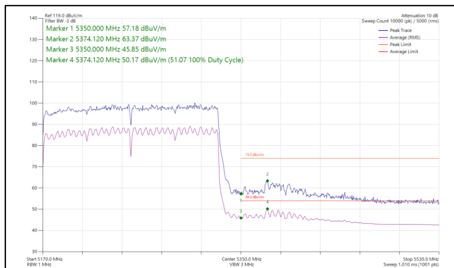
Figure 243 - 802.11ax HE160, SU, SDM, Core 0 - Core 1 - 5250 MHz Band Edge Frequency 5350 MHz
