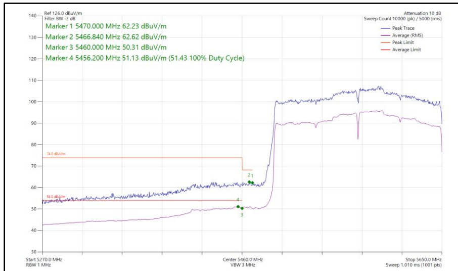
Figure 228 - 802.11ax HE160, SU, SISO, Core 1 - 5570 MHz Band Edge Frequency 5460 MHz
