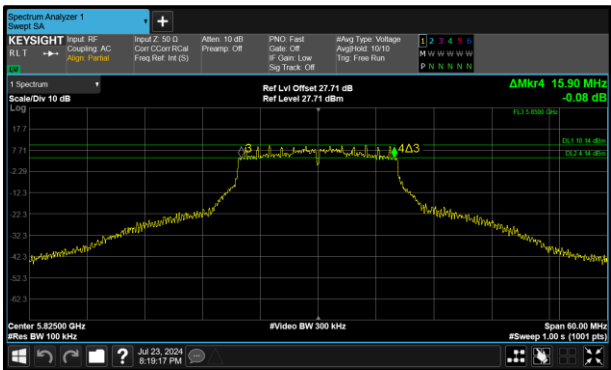
Figure 248 - 802.11a Minimum 6 dB EBW
