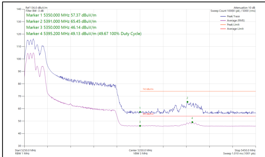
Figure 196 - 802.11ax HE80, RU 106-53, CDD, Core 0 - Core 1 - 5290 MHz Band Edge Frequency 5350 MHz
