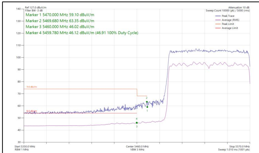
Figure 207 - 802.11ax HE80, SU, SDM, Core 0 - Core 1 - 5530 MHz Band Edge Frequency 5460 MHz
