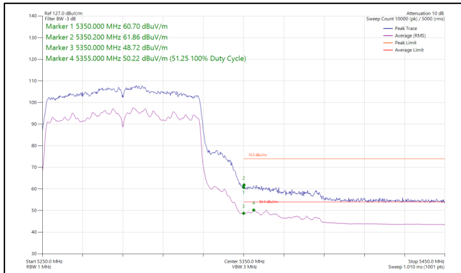
Figure 203 - 802.11ac VHT80, SDM, Core 0 - Core 1 - 5290 MHz Band Edge Frequency 5350 MHz
