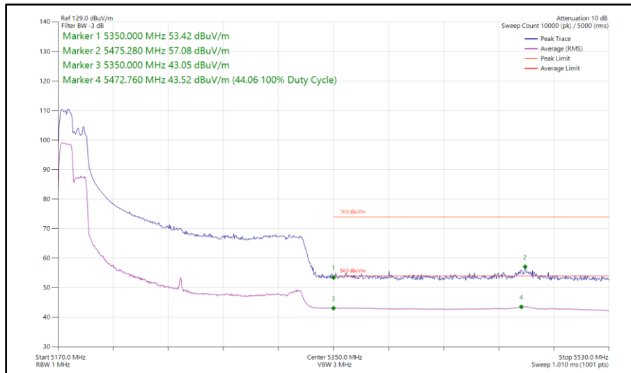
Figure 217 - 802.11ax HE160, RU 106-53P, SISO, Core 0 - 5250 MHz Band Edge Frequency 5350 MHz
