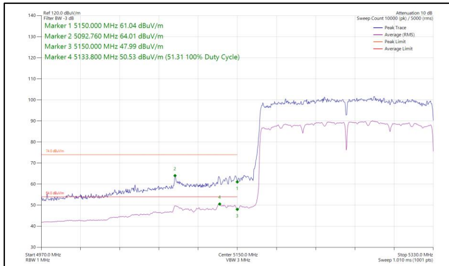
Figure 213 - 802.11ax HE160, SU, SISO, Core 0 - 5250 MHz Band Edge Frequency 5150 MHz
