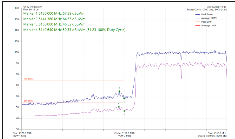
Figure 240 - 802.11ax HE160, SU, SDM, Core 0 - Core 1 - 5250 MHz Band Edge Frequency 5150 MHz
