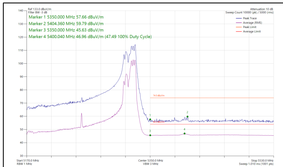
Figure 235 - 802.11ax HE160, RU 106-60S, CDD, Core 0 - Core 1 - 5250 MHz Band Edge Frequency 5350 MHz
