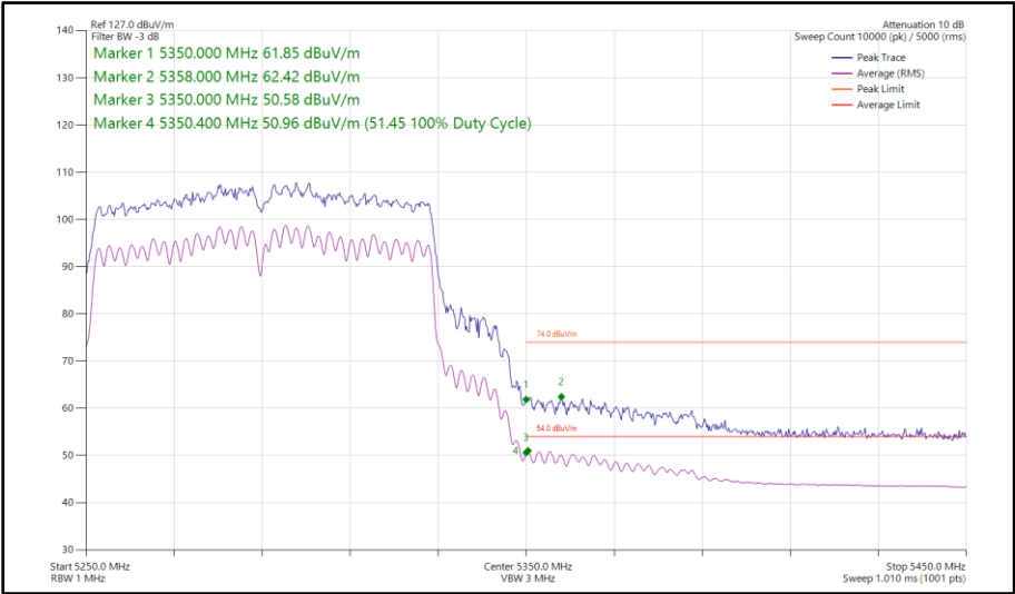
Figure 194 - 802.11ac VHT80, CDD, Core 0 - Core 1 - 5290 MHz Band Edge Frequency 5350 MHz
