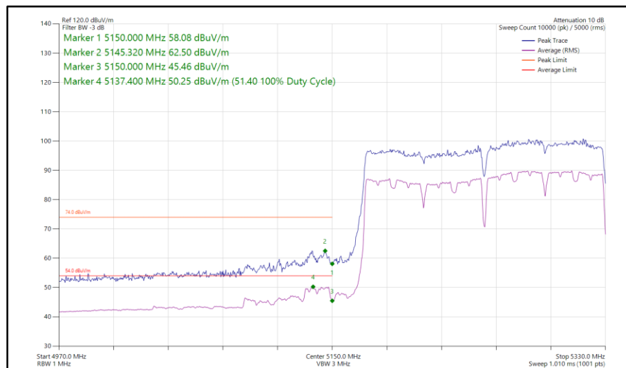
Figure 221 - 802.11ac VHT160, SISO, Core 1 - 5250 MHz Band Edge Frequency 5150 MHz
