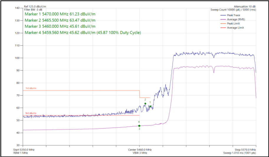
Figure 211 - 802.11ac VHT80, TxBF, Core 0 - Core 1 - 5530 MHz Band Edge Frequency 5460 MHz
