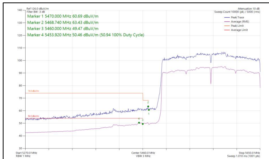
Figure 219 - 802.11ax HE160, SU, SISO, Core 0 - 5570 MHz Band Edge Frequency 5460 MHz
