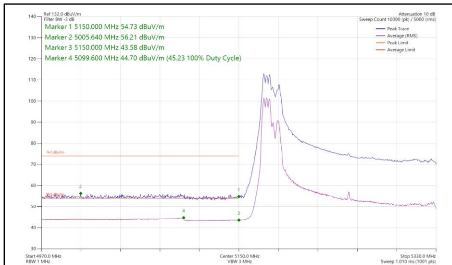
Figure 232 - 802.11ax HE160, RU 106-53P, CDD, Core 0 - Core 1 - 5250 MHz Band Edge Frequency 5150 MHz
