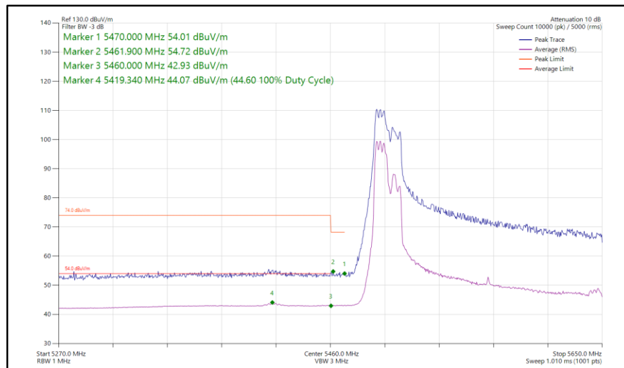
Figure 247 - 802.11ax HE160, RU 106-53P, SDM, Core 0 - Core 1 - 5570 MHz Band Edge Frequency 5460 MHz
