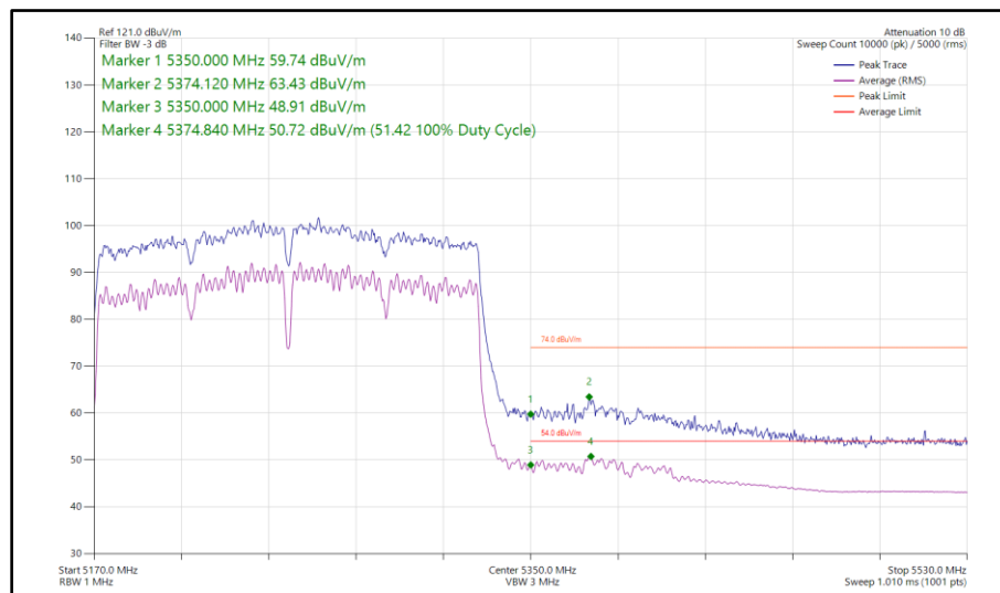
Figure 233 - 802.11ac VHT160, CDD, Core 0 - Core 1 - 5250 MHz Band Edge Frequency 5350 MHz
