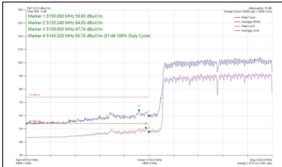
Figure 231 - 802.11ax HE160, SU, CDD, Core 0 - Core 1 - 5250 MHz Band Edge Frequency 5150 MHz
