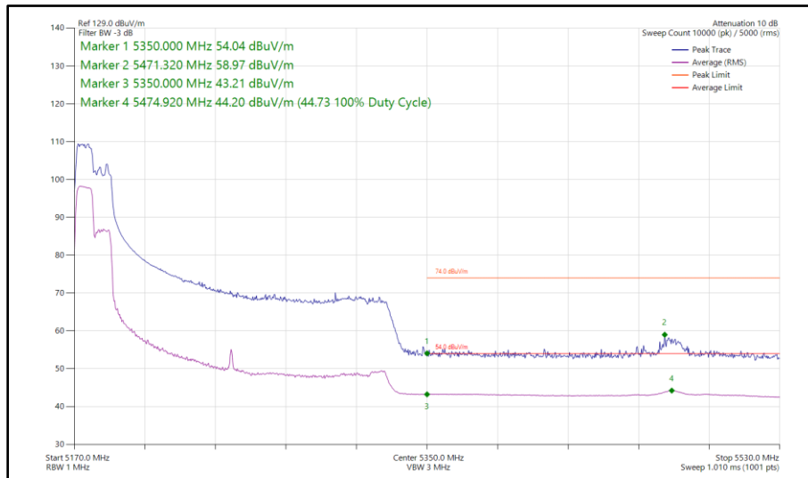
Figure 226 - 802.11ax HE160, RU 106-53P, SISO, Core 1 - 5250 MHz Band Edge Frequency 5350 MHz
