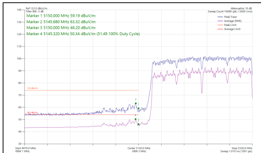
Figure 230 - 802.11ac VHT160, CDD, Core 0 - Core 1 - 5250 MHz Band Edge Frequency 5150 MHz
