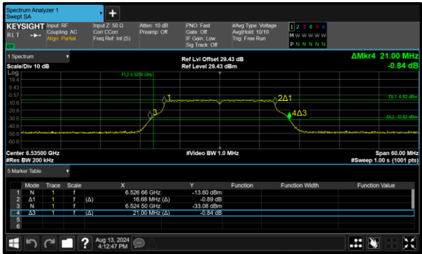
Figure 51 - 802.11a VLP Minimum 99% OBW
