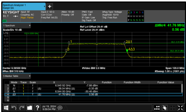
Figure 63 - 802.11ax HE40 SU LPI Minimum 26 dB OBW
