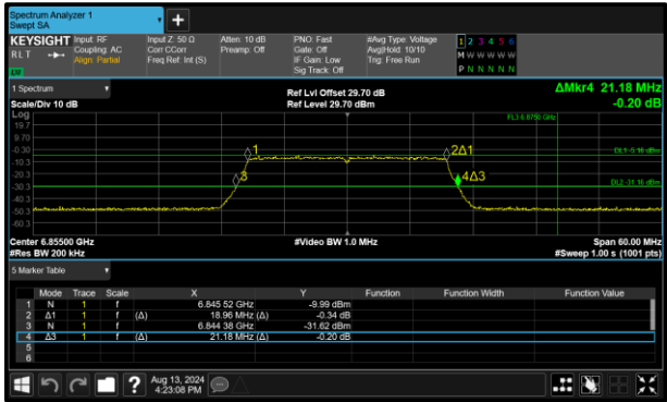
Figure 43 - 802.11ax HE20 SU VLP Minimum 26 dB OBW
