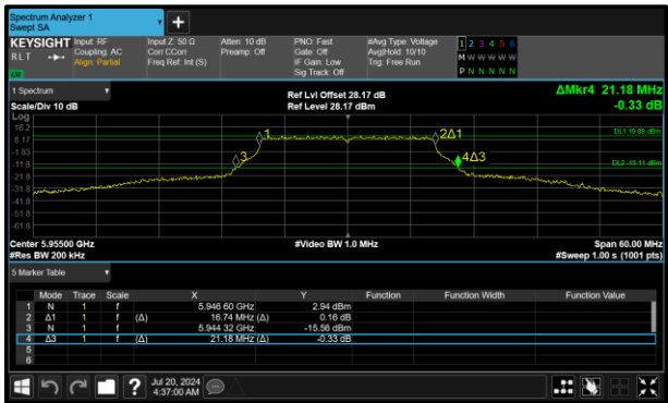
Figure 31 - 802.11a SP Minimum 99% OBW
