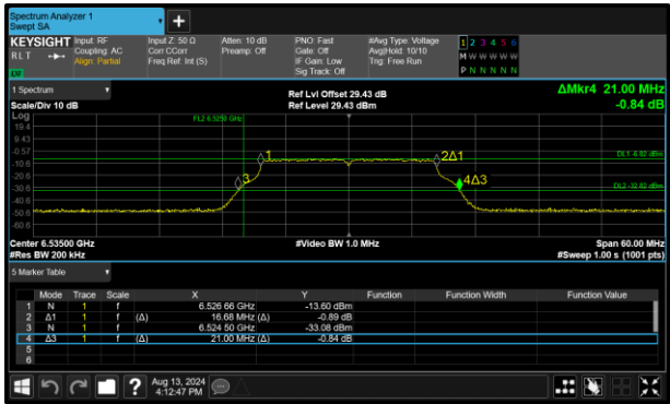
Figure 41 - 802.11a VLP Minimum 26 dB OBW
