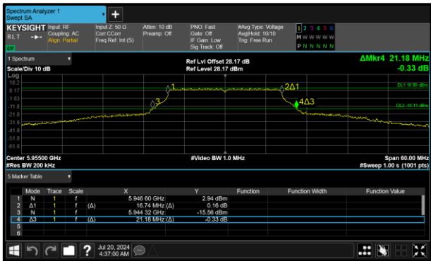
Figure 11 - 802.11a SP Minimum 26 dB OBW
