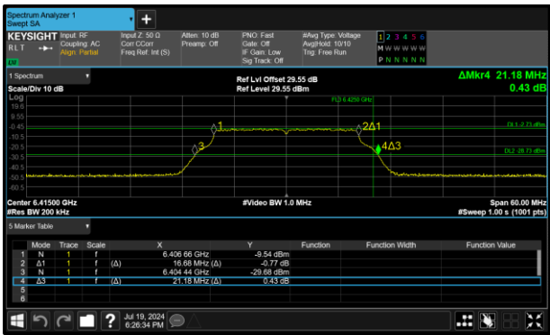
Figure 2 - 802.11a LPI Maximum 26 dB OBW
