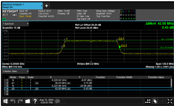
Figure 46 - 802.11ax HE40 SU VLP Maximum 26 dB OBW
