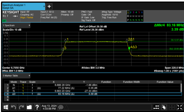
Figure 48 - 802.11ax HE80 SU VLP Maximum 26 dB OBW
