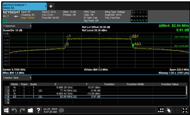
Figure 17 - 802.11ax HE80 SU SP Minimum 26 dB OBW
