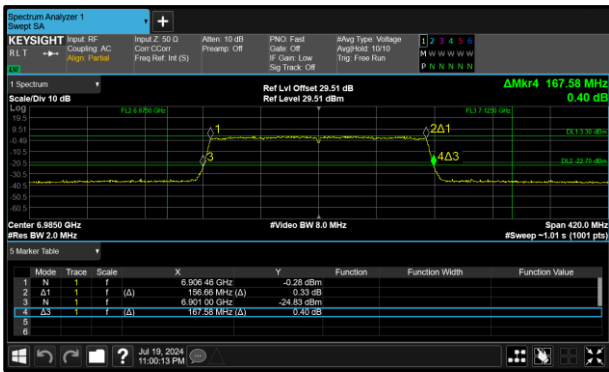
Figure 68 - 802.11ax HE160 SU LPI Maximum 26 dB OBW
