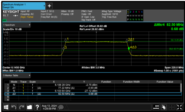
Figure 57 - 802.11ax HE80 SU VLP Minimum 99% OBW
