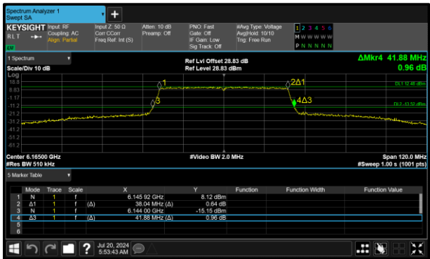
Figure 71 - 802.11ax HE40 SU SP Minimum 26 dB OBW
