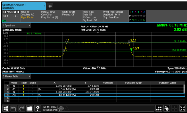
Figure 66 - 802.11ax HE80 SU LPI Maximum 26 dB OBW
