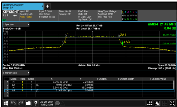
Figure 13 - 802.11ax HE20 SU SP Minimum 26 dB OBW
