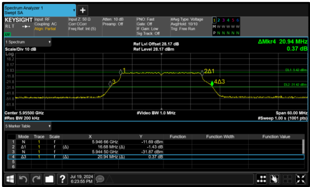
Figure 21 - 802.11a LPI Minimum 99% OBW
