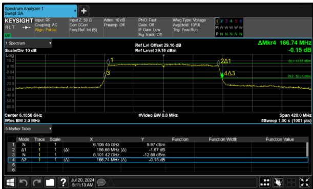
Figure 19 - 802.11ax HE160 SU SP Minimum 26 dB OBW
