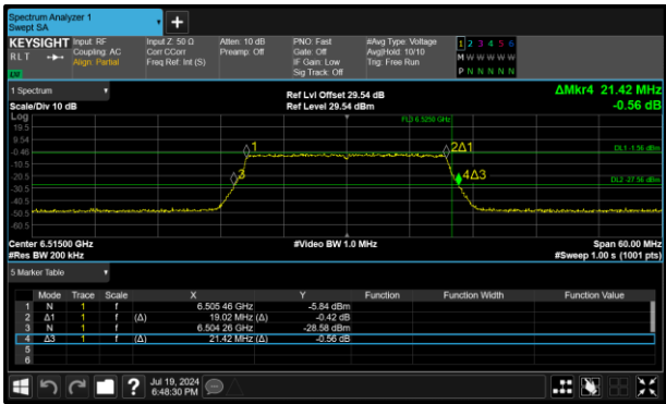
Figure 4 - 802.11ax HE20 SU LPI Maximum 26 dB OBW
