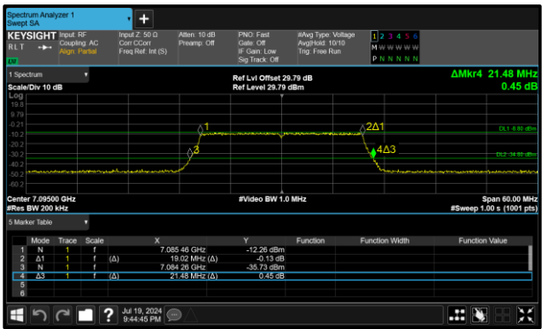
Figure 62 - 802.11ax HE20 SU LPI Maximum 26 dB OBW
