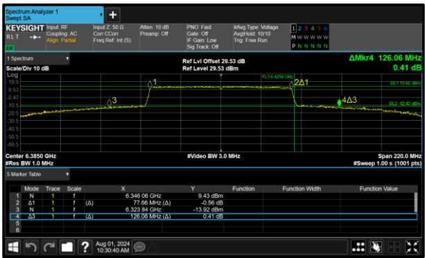
Figure 74 - 802.11ax HE80 SU SP Maximum 26 dB OBW
