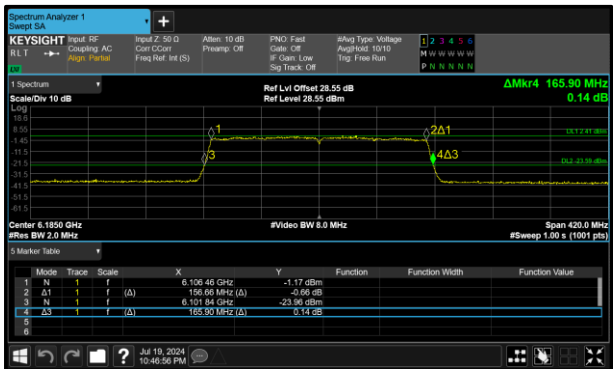
Figure 75 - 802.11ax HE160 SU SP Minimum 26 dB OBW
