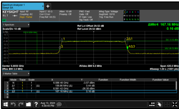
Figure 50 - 802.11ax HE160 SU VLP Maximum 26 dB OBW
