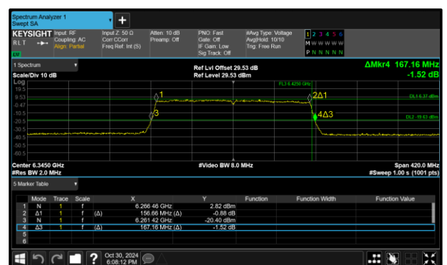
Figure 50 - 802.11ax HE160 SU VLP Maximum 26 dB OBW
