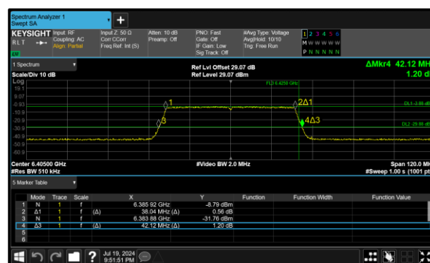
Figure 64 - 802.11ax HE40 SU LPI Maximum 26 dB OBW
