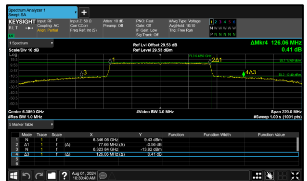
Figure 74 - 802.11ax HE80 SU SP Maximum 26 dB OBW
