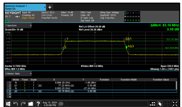
Figure 48 - 802.11ax HE80 SU VLP Maximum 26 dB OBW
