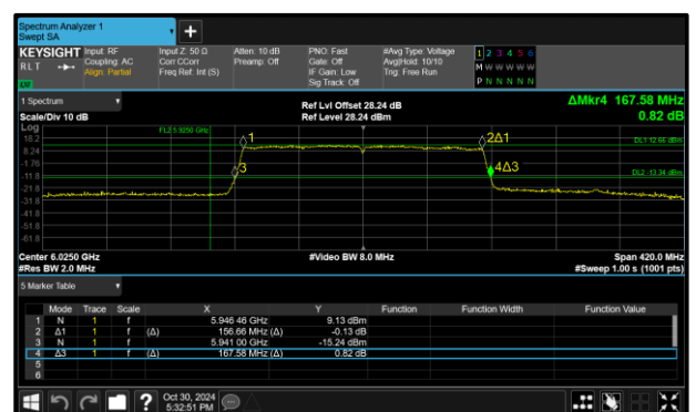
Figure 76 - 802.11ax HE160 SU SP Maximum 26 dB OBW
