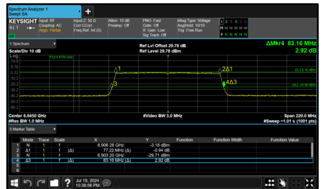
Figure 66 - 802.11ax HE80 SU LPI Maximum 26 dB OBW
