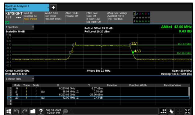
Figure 46 - 802.11ax HE40 SU VLP Maximum 26 dB OBW
