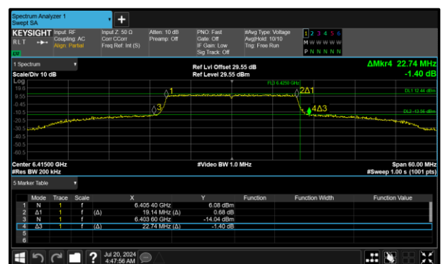
Figure 14 - 802.11ax HE20 SU SP Maximum 26 dB OBW
