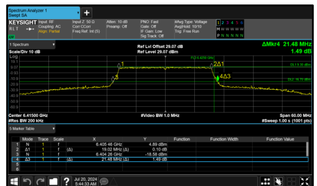
Figure 70 - 802.11ax HE20 SU SP Maximum 26 dB OBW
