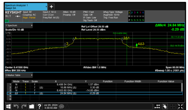
Figure 32 - 802.11a SP Maximum 99% OBW
