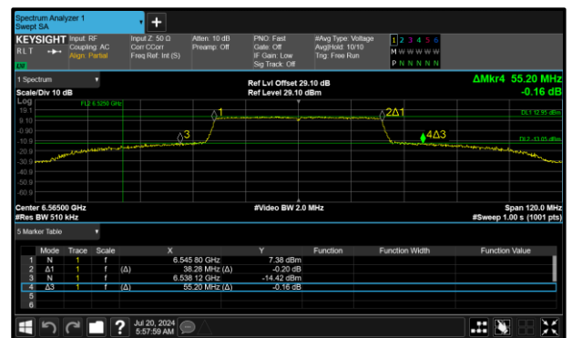
Figure 72 - 802.11ax HE40 SU SP Maximum 26 dB OBW
