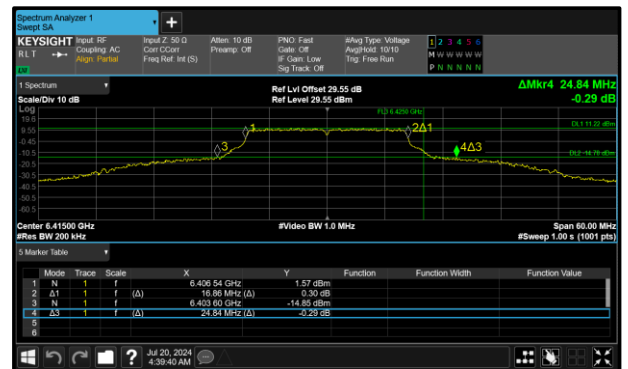
Figure 12 - 802.11a SP Maximum 26 dB OBW
