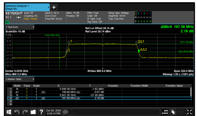
Figure 68 - 802.11ax HE160 SU LPI Maximum 26 dB OBW
