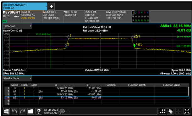
Figure 37 - 802.11ax HE80 SU SP Minimum 99% OBW
