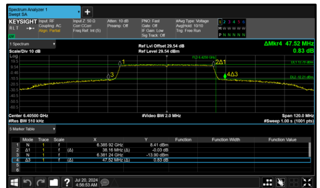
Figure 16 - 802.11ax HE40 SU SP Maximum 26 dB OBW
