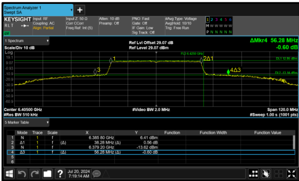
Figure 120 - 802.11ax HE40 SU SP Maximum 26 dB OBW
