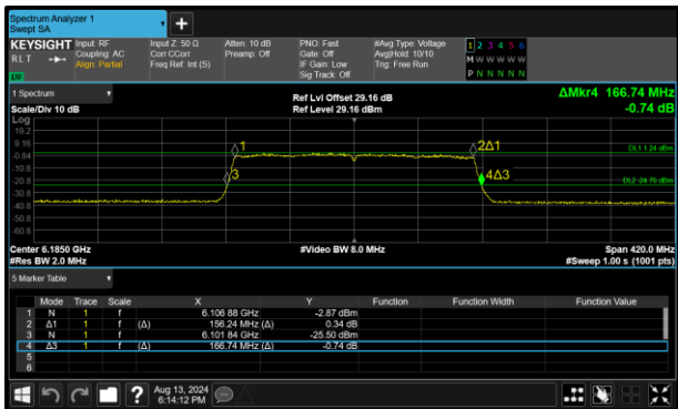
Figure 154 - 802.11ax HE160 SU VLP Minimum 99% OBW
