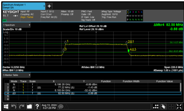
Figure 105 - 802.11ax HE80 SU VLP Minimum 99% OBW
