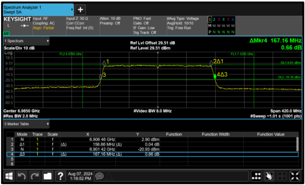
Figure 116 - 802.11ax HE160 SU LPI Maximum 26 dB OBW
