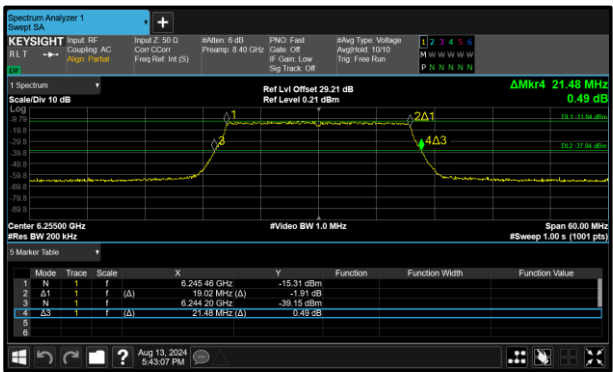
Figure 141 - 802.11ax HE20 SU VLP Maximum 26 dB OBW
