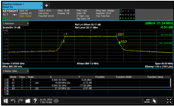
Figure 117 - 802.11ax HE20 SU SP Minimum 26 dB OBW
