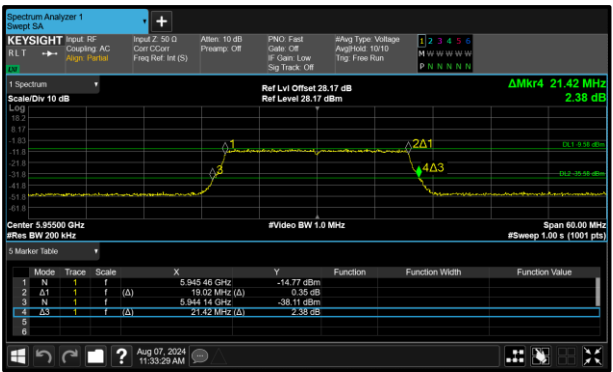
Figure 110 - 802.11ax HE20 SU LPI Maximum 26 dB OBW
