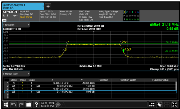
Figure 156 - 802.11ax HE20 SU LPI Minimum 26 dB OBW
