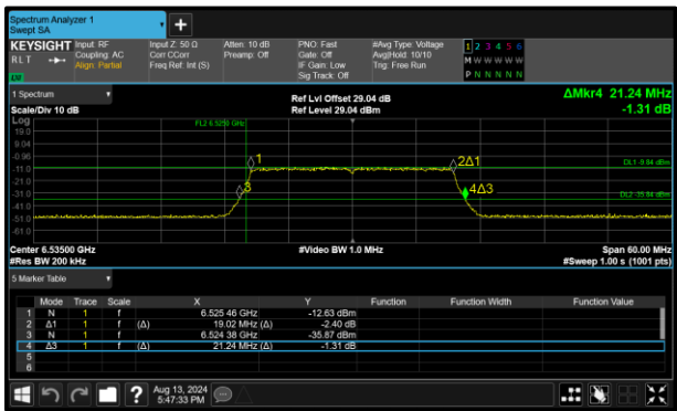
Figure 140 - 802.11ax HE20 SU VLP Minimum 26 dB OBW
