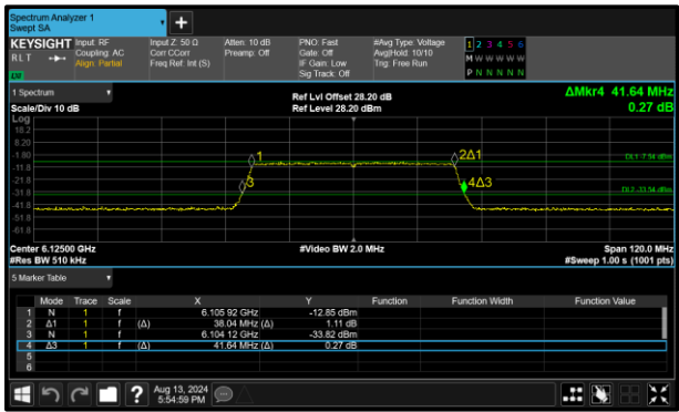
Figure 142 - 802.11ax HE40 SU VLP Minimum 26 dB OBW
