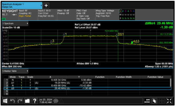
Figure 118 - 802.11ax HE20 SU SP Maximum 26 dB OBW
