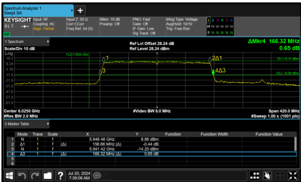
Figure 123 - 802.11ax HE160 SU SP Minimum 26 dB OBW
