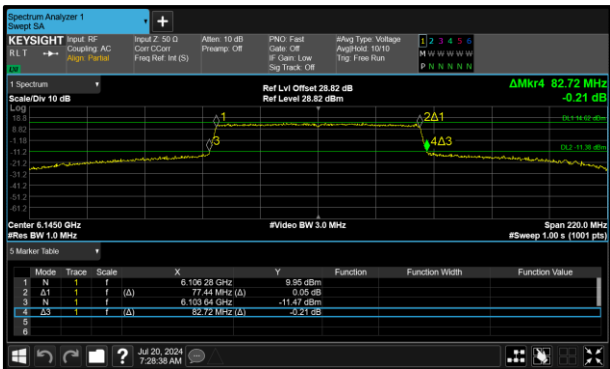
Figure 121 - 802.11ax HE80 SU SP Minimum 26 dB OBW
