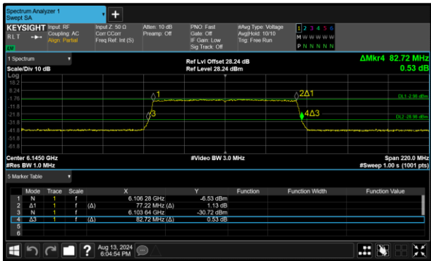
Figure 152 - 802.11ax HE80 SU VLP Minimum 99% OBW
