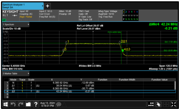
Figure 96 - 802.11ax HE40 SU VLP Maximum 26 dB OBW
