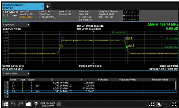
Figure 155 - 802.11ax HE160 SU VLP Maximum 99% OBW
