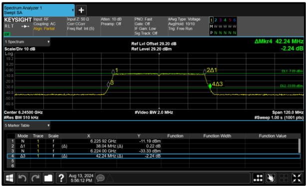
Figure 143 - 802.11ax HE40 SU VLP Maximum 26 dB OBW
