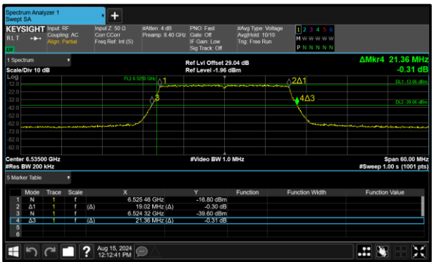
Figure 94 - 802.11ax HE20 SU VLP Maximum 26 dB OBW
