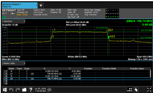
<lageCaption> - 802.11ax HE160 SU SP Maximum 26 dB OBW
