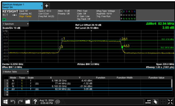
Figure 153 - 802.11ax HE80 SU VLP Maximum 99% OBW
