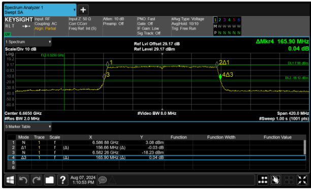
Figure 115 - 802.11ax HE160 SU LPI Minimum 26 dB OBW
