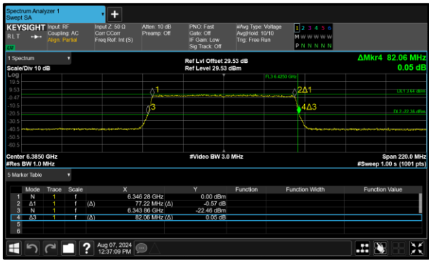
Figure 113 - 802.11ax HE80 SU LPI Minimum 26 dB OBW
