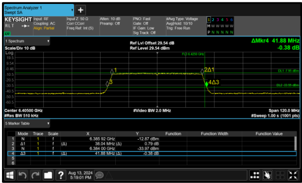
Figure 95 - 802.11ax HE40 SU VLP Minimum 26 dB OBW
