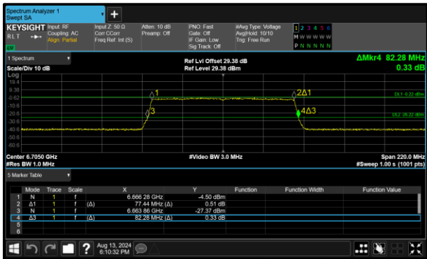
Figure 144 - 802.11ax HE80 SU VLP Minimum 26 dB OBW
