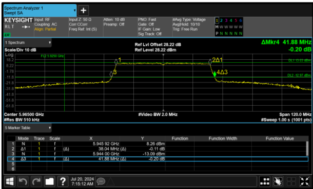
Figure 119 - 802.11ax HE40 SU SP Minimum 26 dB OBW
