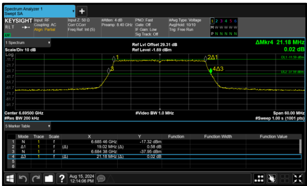
Figure 93 - 802.11ax HE20 SU VLP Minimum 26 dB OBW
