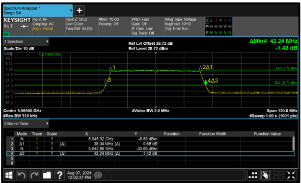
Figure 112 - 802.11ax HE40 SU LPI Maximum 26 dB OBW
