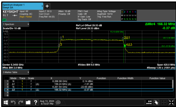
Figure 146 - 802.11ax HE160 SU VLP Minimum 26 dB OBW
