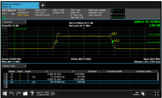
Figure 114 - 802.11ax HE80 SU LPI Maximum 26 dB OBW
