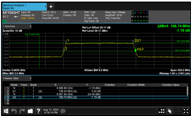
Figure 147 - 802.11ax HE160 SU VLP Maximum 26 dB OBW
