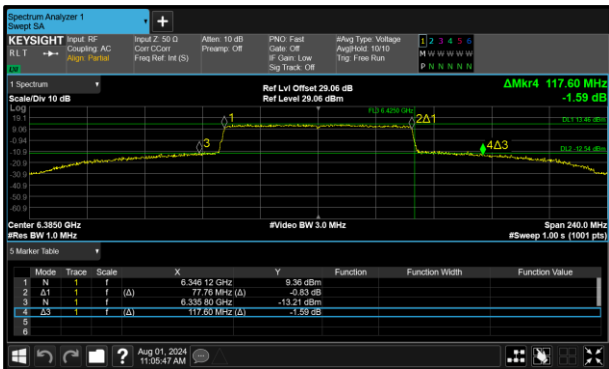
Figure 122 - 802.11ax HE80 SU SP Maximum 26 dB OBW
