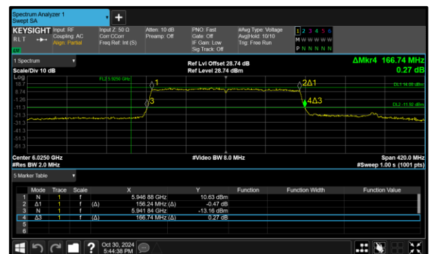
<lageCaption> - 802.11ax HE160 SU SP Maximum 26 dB OBW
