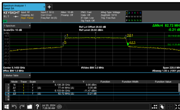
Figure 121 - 802.11ax HE80 SU SP Minimum 26 dB OBW
