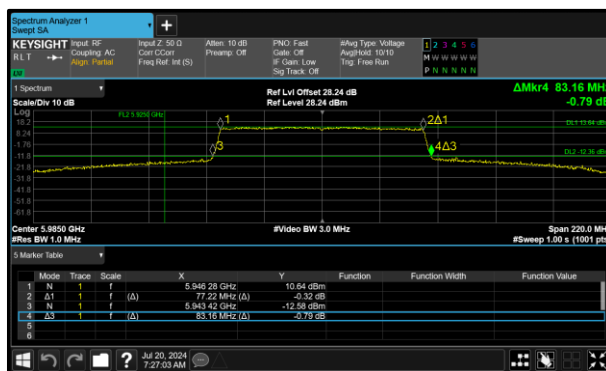
Figure 136 - 802.11ax HE80 SU SP Minimum 99% OBW
