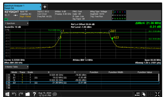
Figure 94 - 802.11ax HE20 SU VLP Maximum 26 dB OBW
