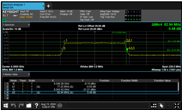
Figure 98 - 802.11ax HE80 SU VLP Maximum 26 dB OBW
