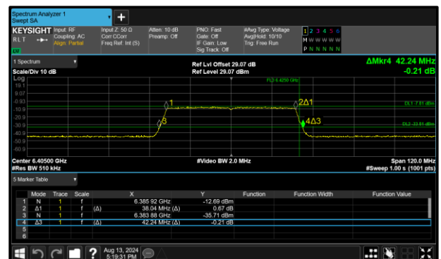
Figure 96 - 802.11ax HE40 SU VLP Maximum 26 dB OBW
