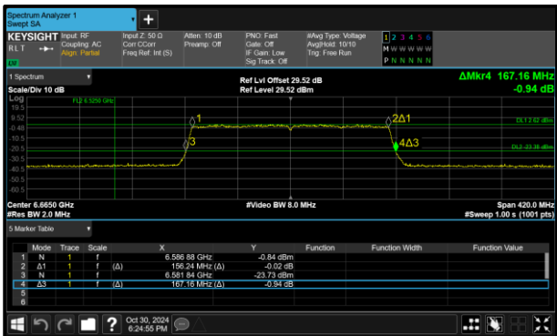
Figure 147 - 802.11ax HE160 SU VLP Maximum 26 dB OBW
