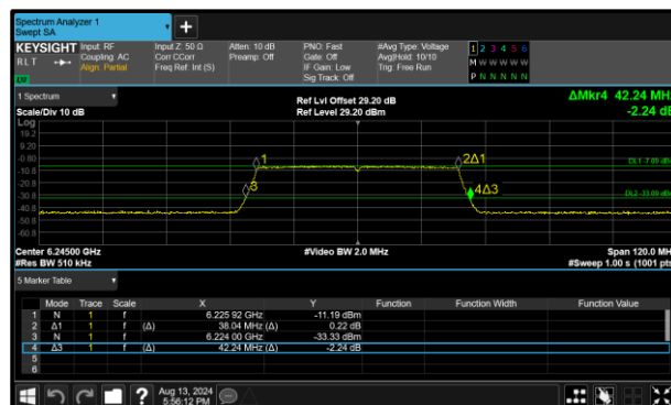
Figure 143 - 802.11ax HE40 SU VLP Maximum 26 dB OBW
