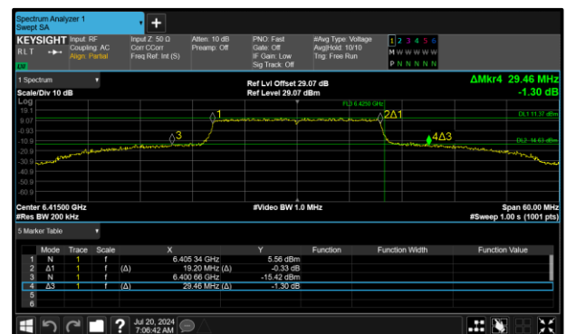
Figure 118 - 802.11ax HE20 SU SP Maximum 26 dB OBW
