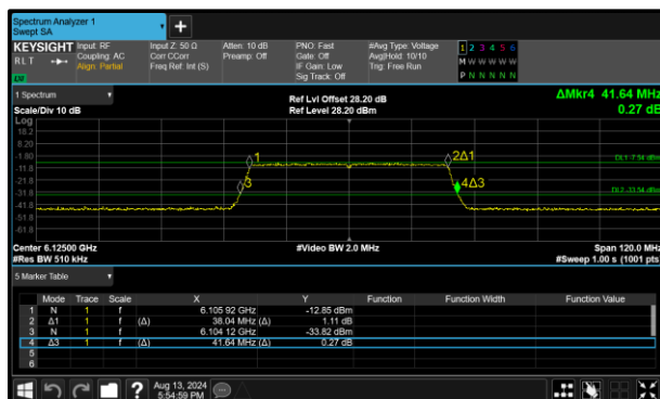
Figure 142 - 802.11ax HE40 SU VLP Minimum 26 dB OBW
