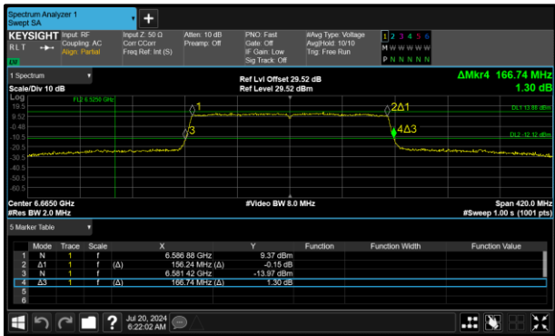
Figure 91 - 802.11ax HE160 SU SP Minimum 99% OBW
