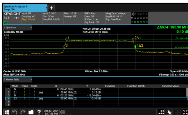
Figure 123 - 802.11ax HE160 SU SP Minimum 26 dB OBW
