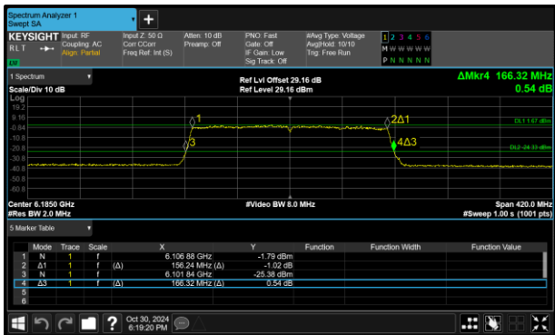
Figure 146 - 802.11ax HE160 SU VLP Minimum 26 dB OBW
