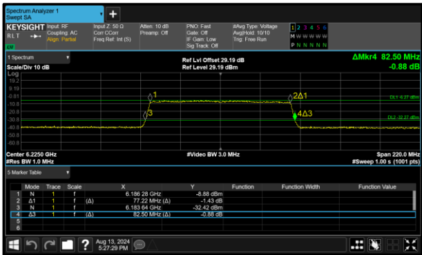
Figure 97 - 802.11ax HE80 SU VLP Minimum 26 dB OBW
