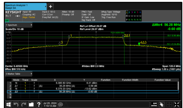
Figure 120 - 802.11ax HE40 SU SP Maximum 26 dB OBW
