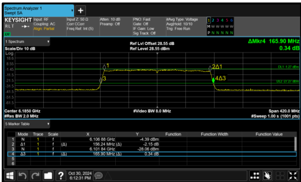
Figure 99 - 802.11ax HE160 SU VLP Minimum 26 dB OBW
