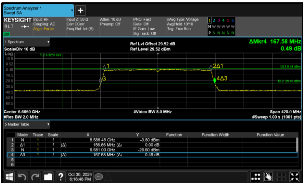
Figure 100 - 802.11ax HE160 SU VLP Maximum 26 dB OBW
