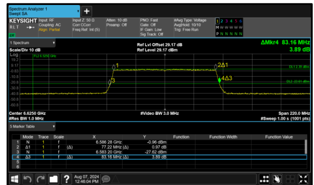
Figure 114 - 802.11ax HE80 SU LPI Maximum 26 dB OBW
