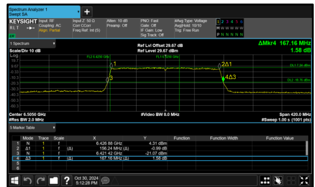
Figure 116 - 802.11ax HE160 SU LPI Maximum 26 dB OBW
