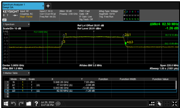
Figure 166 - 802.11ax HE80 SU SP Minimum 26 dB OBW
