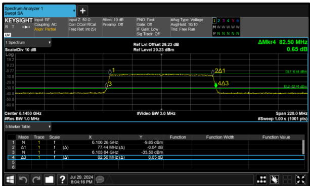
Figure 168 - 802.11ax HE80 SU VLP Minimum 26 dB OBW
