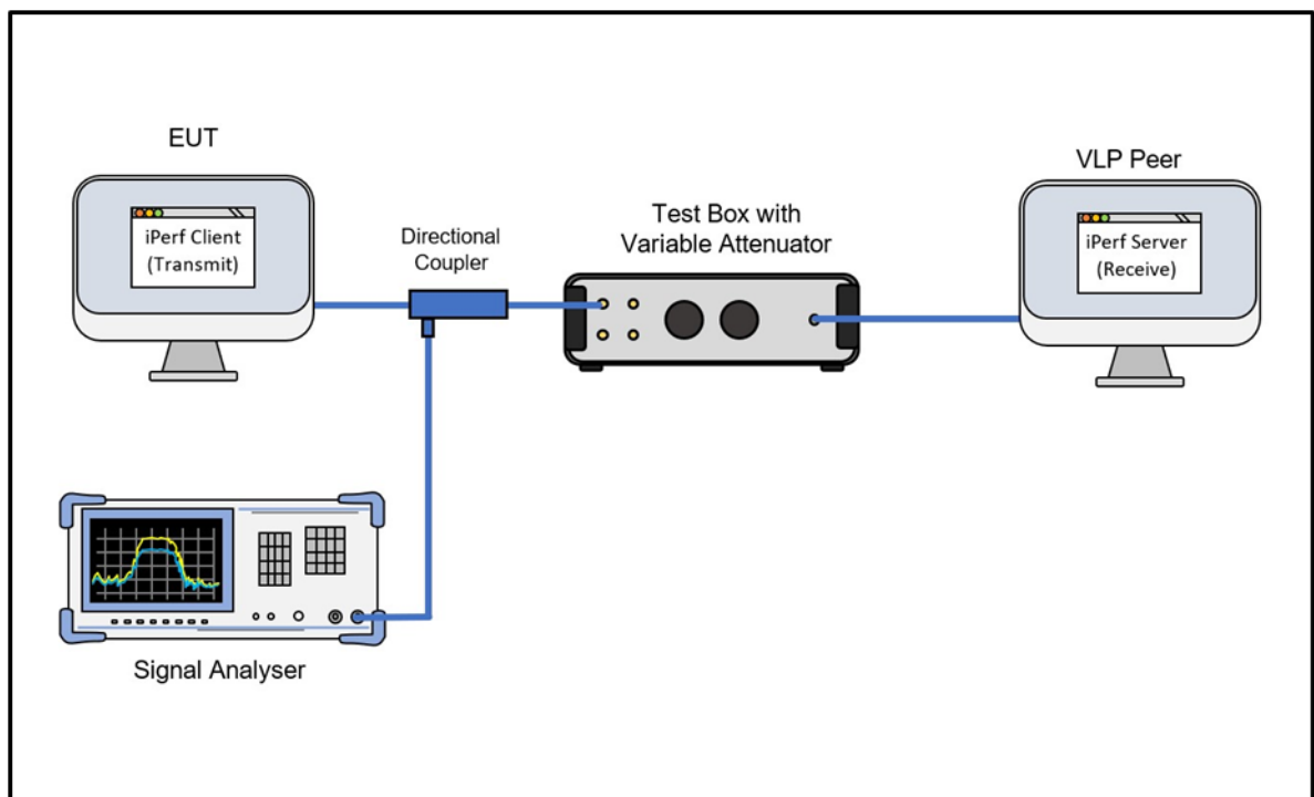
Figure 185 - Test Equipment Setup Diagram
