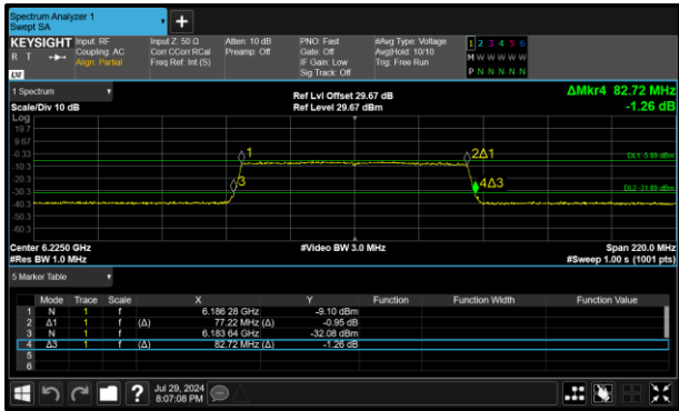
Figure 182 - 802.11ax HE80 SU VLP Minimum 99% OBW
