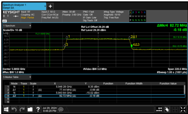
Figure 180 - 802.11ax HE80 SU SP Minimum 99% OBW
