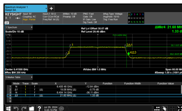
Figure 157 - 802.11ax HE20 SU LPI Maximum 26 dB OBW
