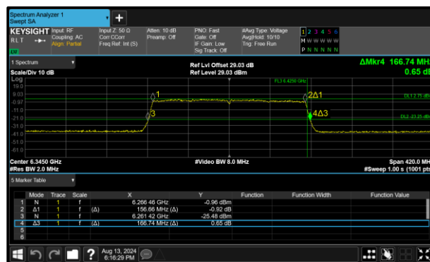
Figure 155 - 802.11ax HE160 SU VLP Maximum 99% OBW
