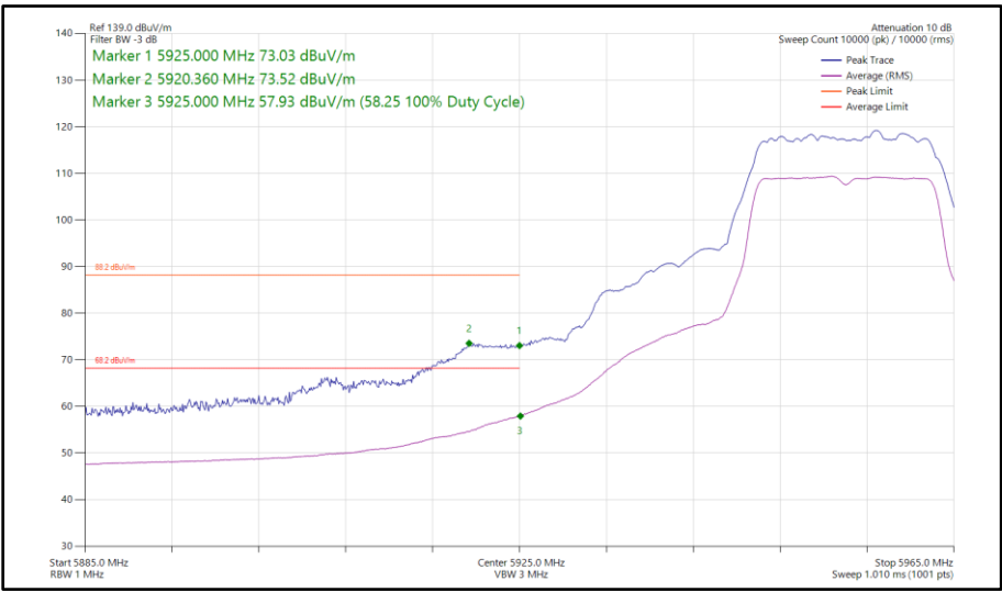
Figure 187 - 802.11a, SISO, Core 0 - 5955 MHz Band Edge Frequency 5925 MHz
