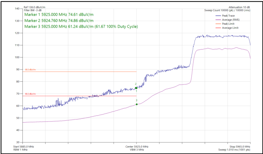
Figure 208 - 802.11ax HE20, SU, SDM, Core 0 - Core 1 - 5955 MHz Band Edge Frequency 5925 MHz
