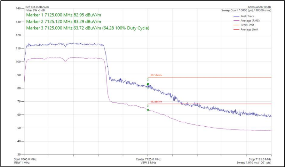
Figure 222 - 802.11ax HE40, SU, SISO, Core 1 - 7085 MHz Band Edge Frequency 7125 MHz
