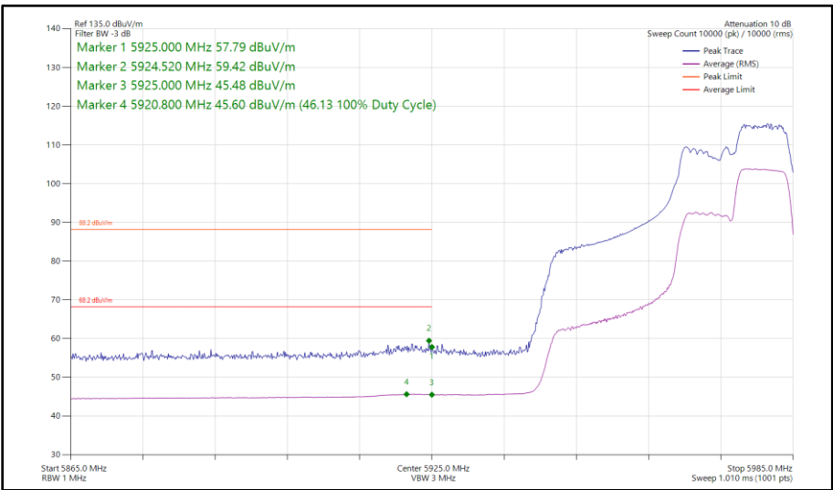
Figure 221 - 802.11ax HE40, RU 106-56, SISO, Core 1 - 5965 MHz Band Edge Frequency 5925 MHz
