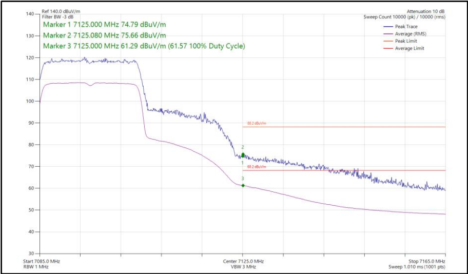
Figure 192 - 802.11ax HE20, SU, SISO, Core 0 - 7095 MHz Band Edge Frequency 7125 MHz
