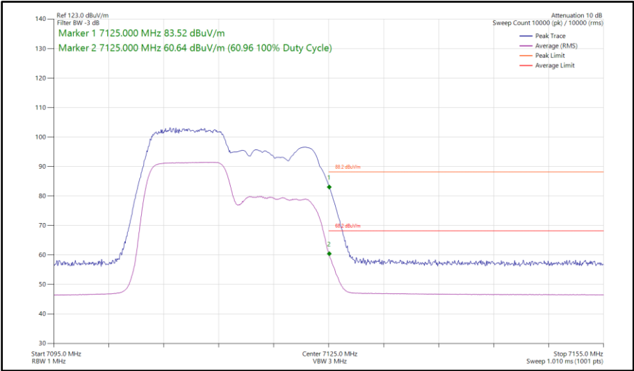
Figure 194 - 802.11ax HE20, RU 106-53, SISO, Core 0 - 7115 MHz Band Edge Frequency 7125 MHz
