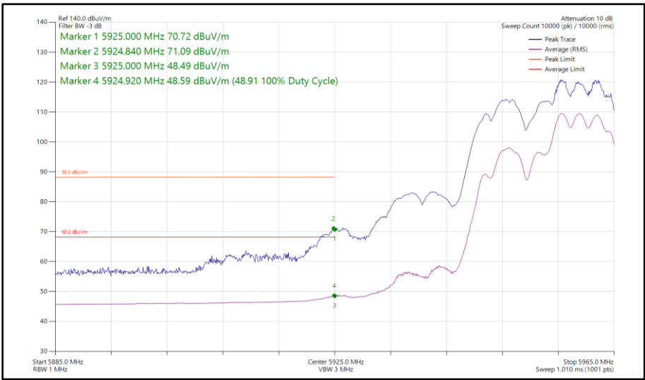
Figure 204 - 802.11ax HE20, RU 106-54, CDD, Core 0 - Core 1 - 5955 MHz Band Edge Frequency 5925 MHz
