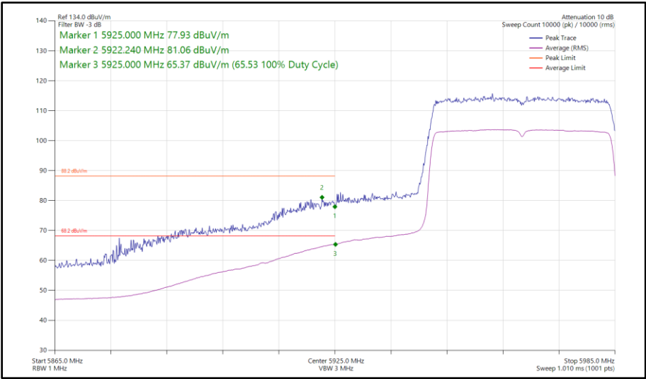
Figure 220 - 802.11ax HE40, SU, SISO, Core 1 - 5965 MHz Band Edge Frequency 5925 MHz
