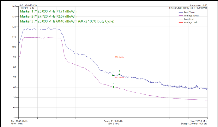
Figure 190 - 802.11a, SISO, Core 0 - 7095 MHz Band Edge Frequency 7125 MHz
