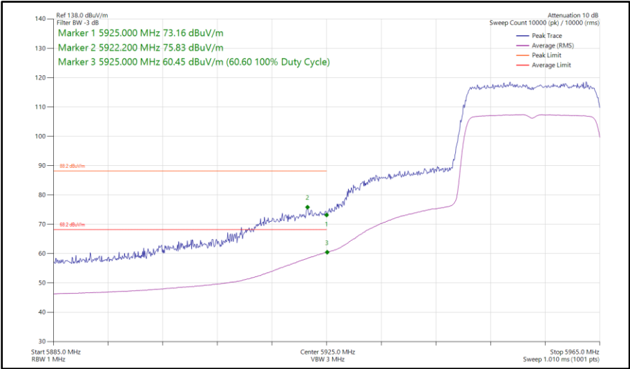
Figure 188 - 802.11ax HE20, SU, SISO, Core 0 - 5955 MHz Band Edge Frequency 5925 MHz
