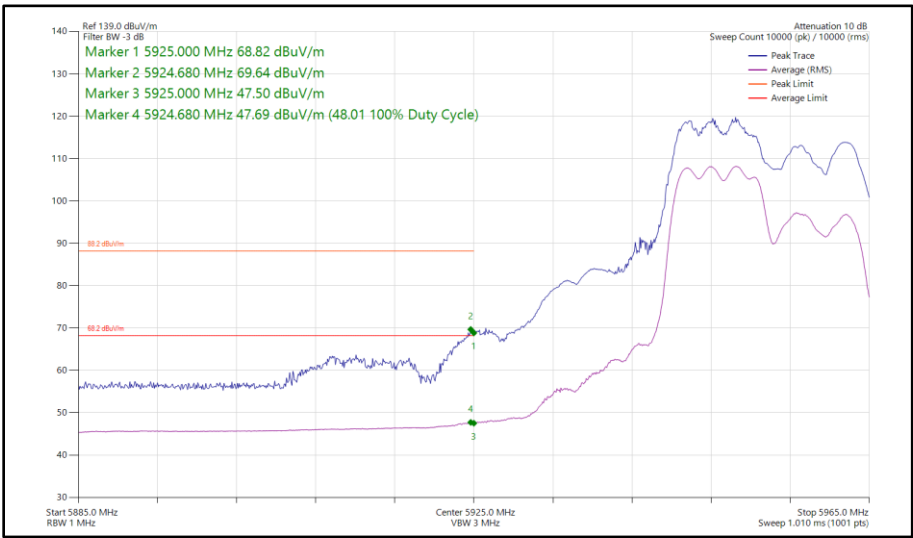
Figure 209 - 802.11ax HE20, RU 106-53, SDM, Core 0 - Core 1 - 5955 MHz Band Edge Frequency 5925 MHz
