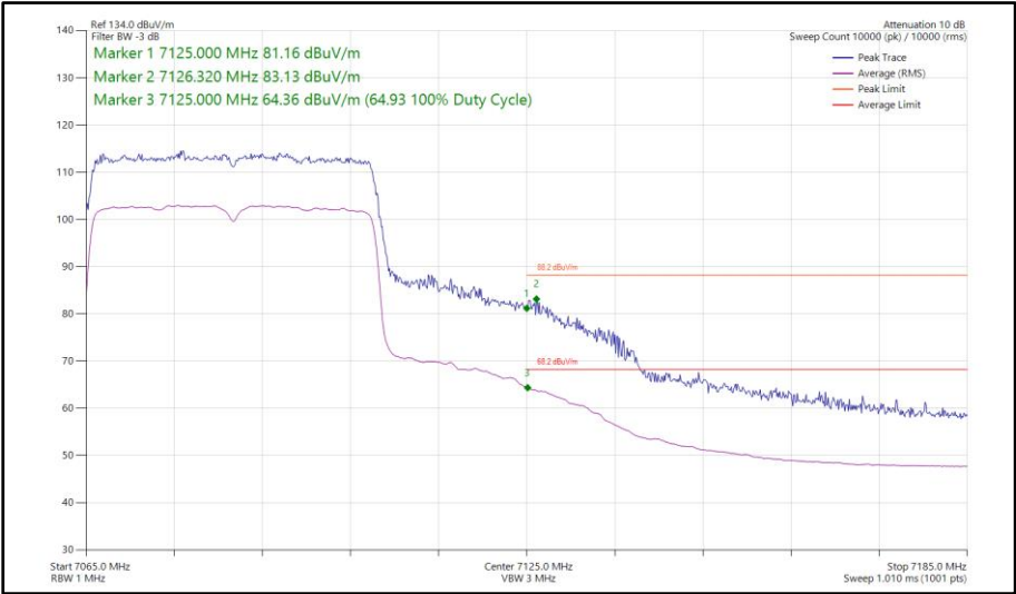
Figure 218 - 802.11ax HE40, SU, SISO, Core 0 - 7085 MHz Band Edge Frequency 7125 MHz
