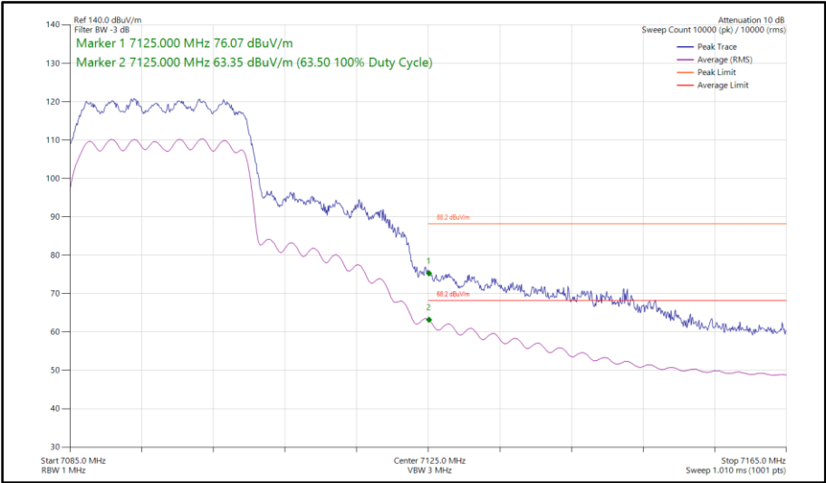
Figure 205 - 802.11ax HE20, SU, CDD, Core 0 - Core 1 - 7095 MHz Band Edge Frequency 7125 MHz
