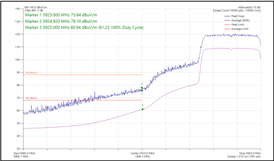
Figure 213 - 802.11ax HE20, SU, TxBF, Core 0 - Core 1 - 5955 MHz Band Edge Frequency 5925 MHz
