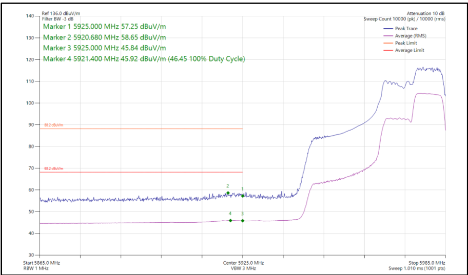
Figure 217 - 802.11ax HE40, RU 106-56, SISO, Core 0 - 5965 MHz Band Edge Frequency 5925 MHz
