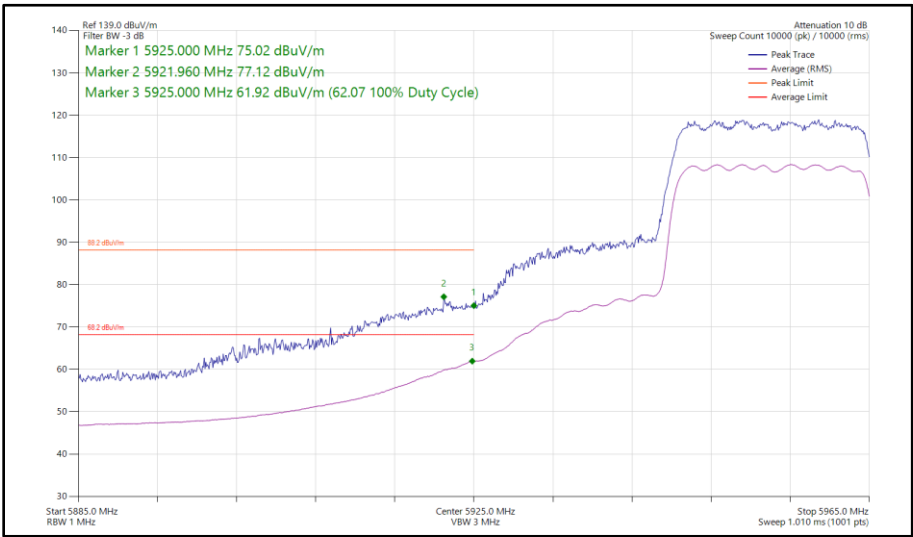
Figure 203 - 802.11ax HE20, SU, CDD, Core 0 - Core 1 - 5955 MHz Band Edge Frequency 5925 MHz
