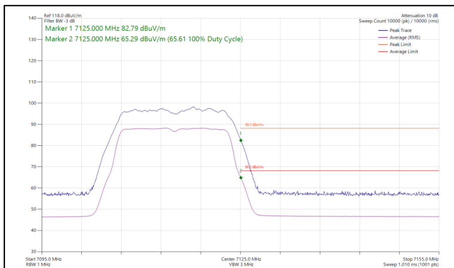
Figure 199 - 802.11a, SISO, Core 1 - 7115 MHz Band Edge Frequency 7125 MHz
