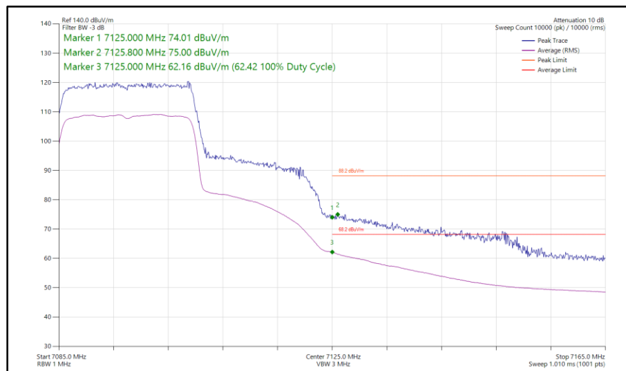
Figure 210 - 802.11ax HE20, SU, SDM, Core 0 - Core 1 - 7095 MHz Band Edge Frequency 7125 MHz
