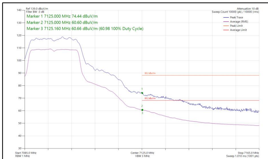
Figure 198 - 802.11a, SISO, Core 1 - 7095 MHz Band Edge Frequency 7125 MHz
