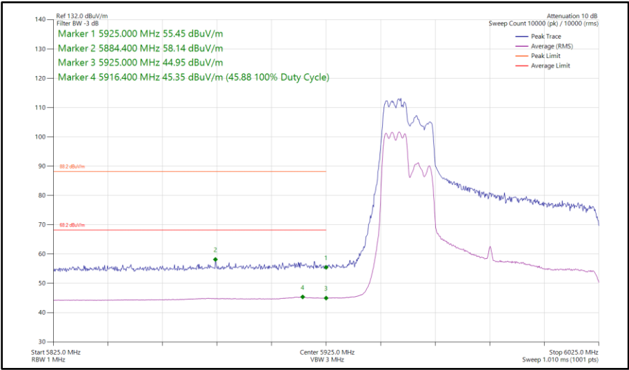
Figure 249 - 802.11ax HE80, RU 106-53, SDM, Core 0 - Core 1 - 5985 MHz Band Edge Frequency 5925 MHz
