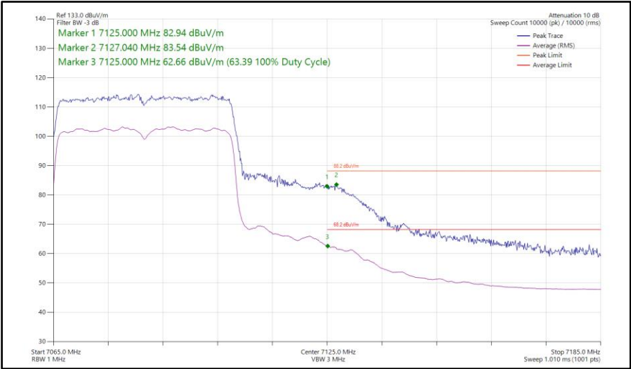
Figure 230 - 802.11ax HE40, SU, SDM, Core 0 - Core 1 - 7085 MHz Band Edge Frequency 7125 MHz
