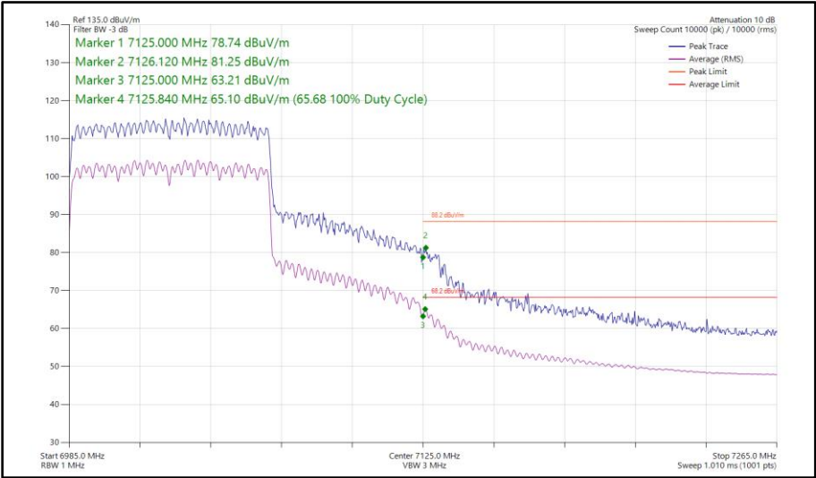
Figure 246 - 802.11ax HE80, SU, CDD, Core 0 - Core 1 - 7025 MHz Band Edge Frequency 7125 MHz
