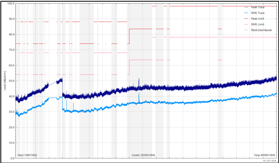
Figure 286 - U-NII-6 - 6475 MHz (CH105), HE20, SU, CDD, Core 0 + Core 1, 1 GHz to 40 GHz, Vertical
