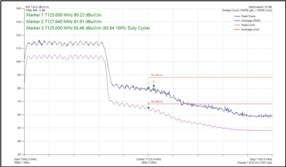
Figure 226 - 802.11ax HE40, SU, CDD, Core 0 - Core 1 - 7085 MHz Band Edge Frequency 7125 MHz
