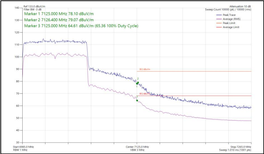
Figure 250 - 802.11ax HE80, SU, SDM, Core 0 - Core 1 - 7025 MHz Band Edge Frequency 7125 MHz
