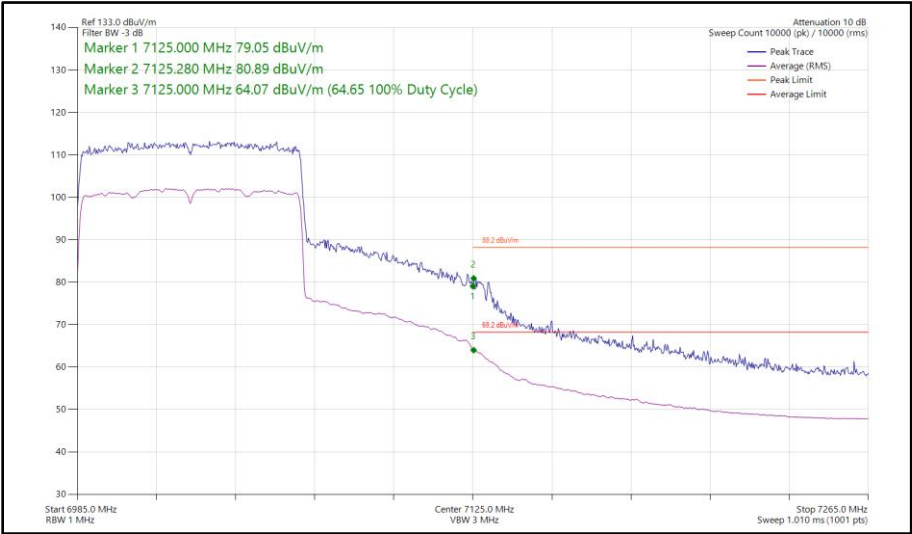
Figure 242 - 802.11ax HE80, SU, SISO, Core 1 - 7025 MHz Band Edge Frequency 7125 MHz
