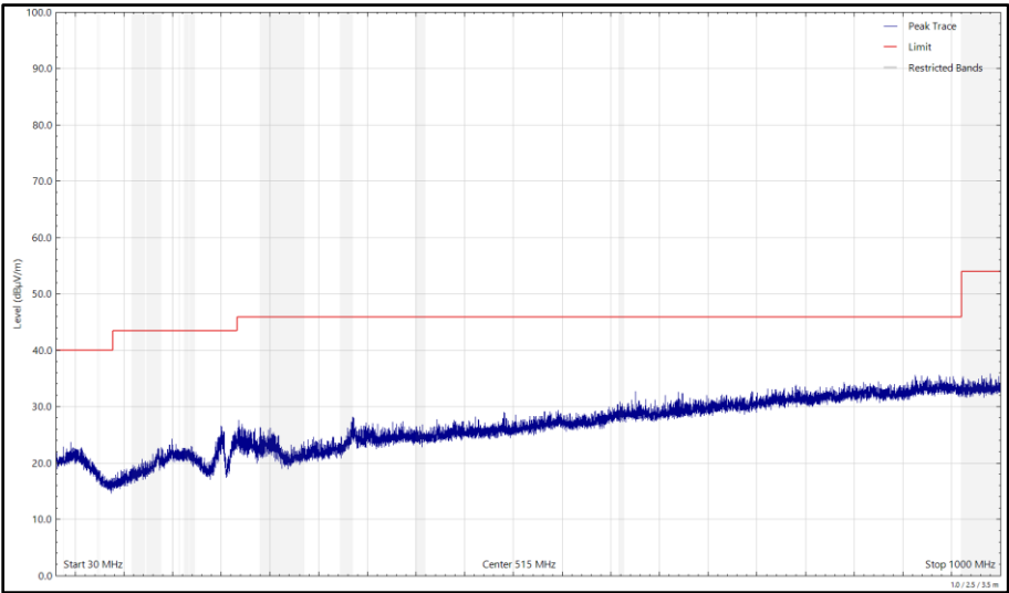
Figure 285 - U-NII-6 - 6475 MHz (CH105), HE20, SU, CDD, Core 0 + Core 1, 30 MHz to 1 GHz, Vertical (Peak)
