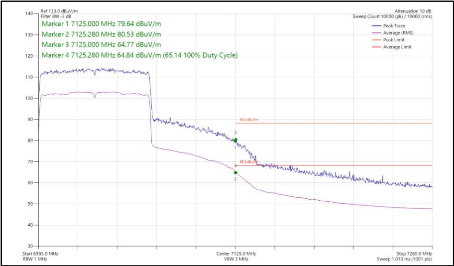
Figure 238 - 802.11ax HE80, SU, SISO, Core 0 - 7025 MHz Band Edge Frequency 7125 MHz
