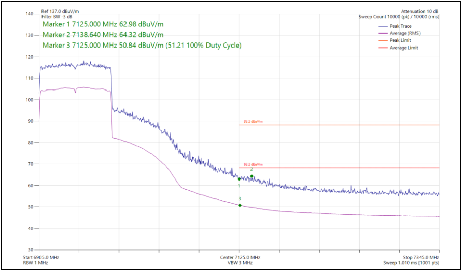
Figure 254 - 802.11ax HE80, SU, TxBF, Core 0 - Core 1 - 6945 MHz Band Edge Frequency 7125 MHz
