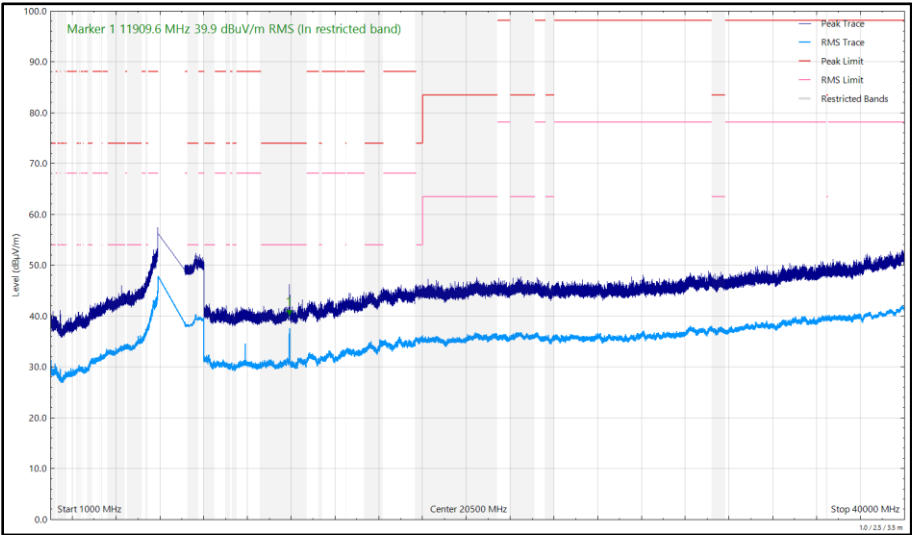
Figure 274 - U-NII-5 - 5955 MHz (CH1), HE20, SU, CDD, Core 0 + Core 1, 1 GHz to 40 GHz, Vertical
