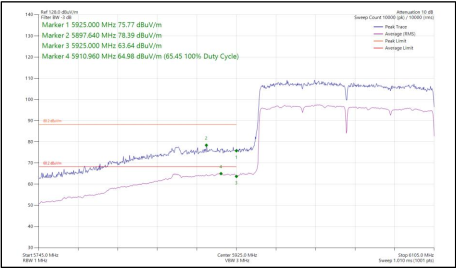
Figure 256 - 802.11ax HE160, SU, SISO, Core 0 - 6025 MHz Band Edge Frequency 5925 MHz
