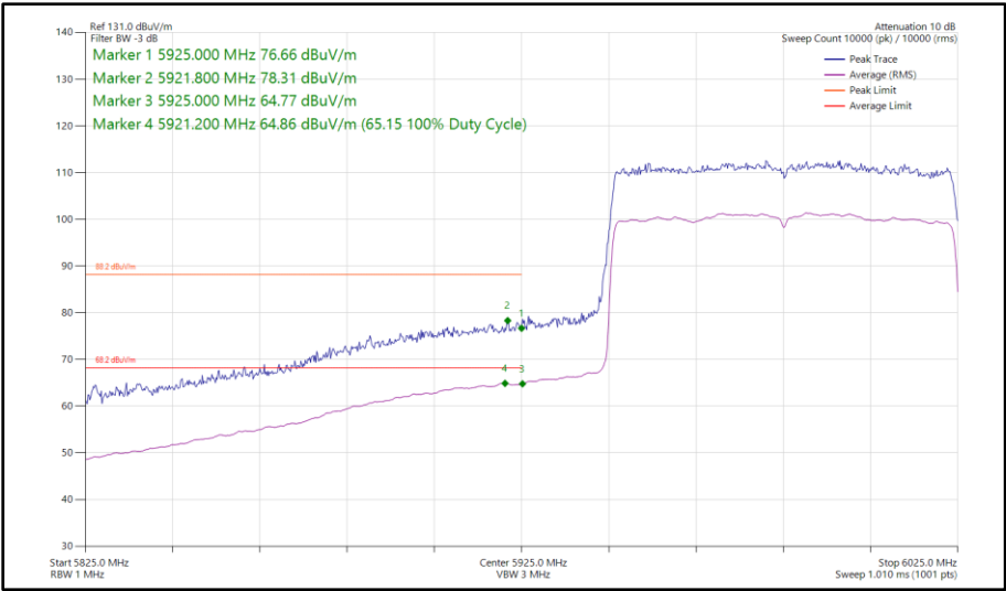
Figure 248 - 802.11ax HE80, SU, SDM, Core 0 - Core 1 - 5985 MHz Band Edge Frequency 5925 MHz
