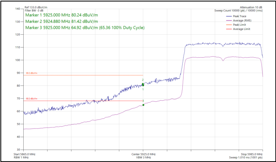
Figure 228 - 802.11ax HE40, SU, SDM, Core 0 - Core 1 - 5965 MHz Band Edge Frequency 5925 MHz
