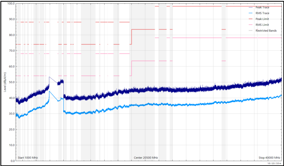
Figure 273 - U-NII-5 - 5955 MHz (CH1), HE20, SU, CDD, Core 0 + Core 1, 1 GHz to 40 GHz, Horizontal
