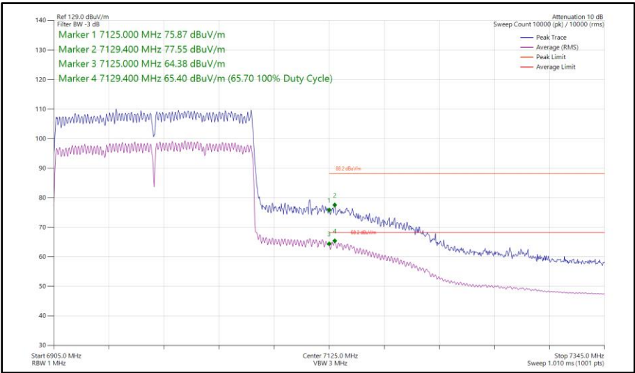
Figure 266 - 802.11ax HE160, SU, CDD, Core 0 - Core 1 - 6985 MHz Band Edge Frequency 7125 MHz
