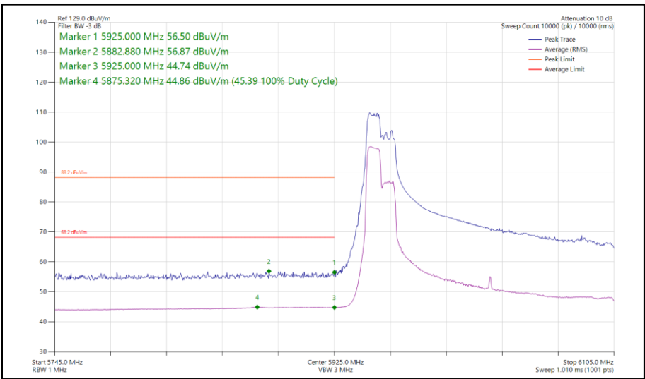
Figure 257 - 802.11ax HE160, RU 106-53P, SISO, Core 0 - 6025 MHz Band Edge Frequency 5925 MHz
