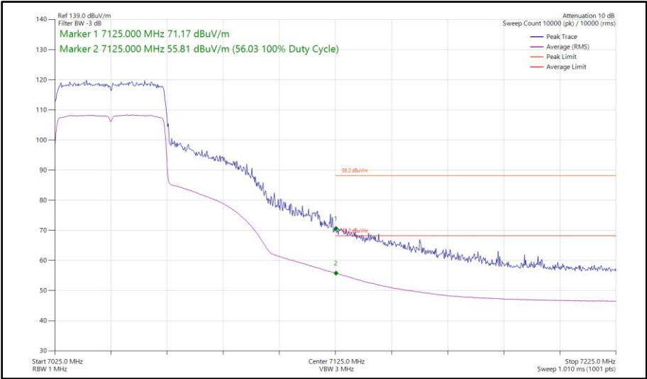
Figure 234 - 802.11ax HE40, SU, TxBF, Core 0 - Core 1 - 7045 MHz Band Edge Frequency 7125 MHz
