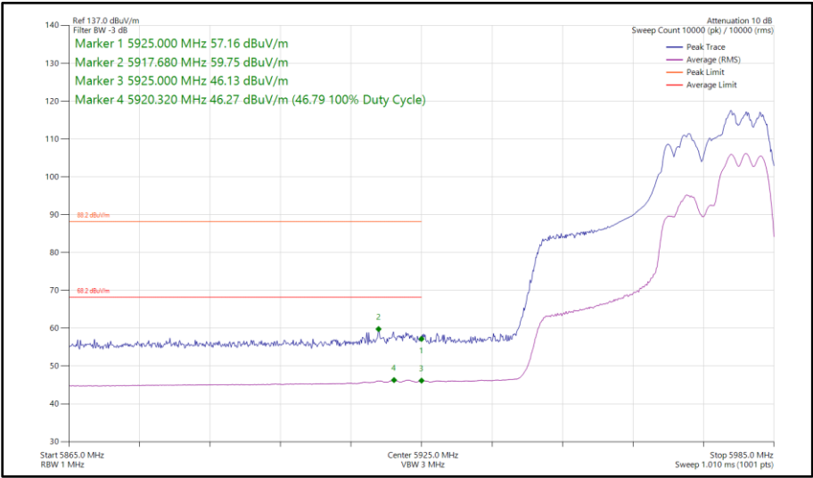
Figure 229 - 802.11ax HE40, RU 106-56, SDM, Core 0 - Core 1 - 5965 MHz Band Edge Frequency 5925 MHz
