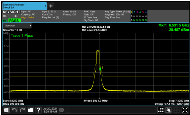
Figure 313 - A (Core 0) 802.11a SP 6515 MHz (CH113)
