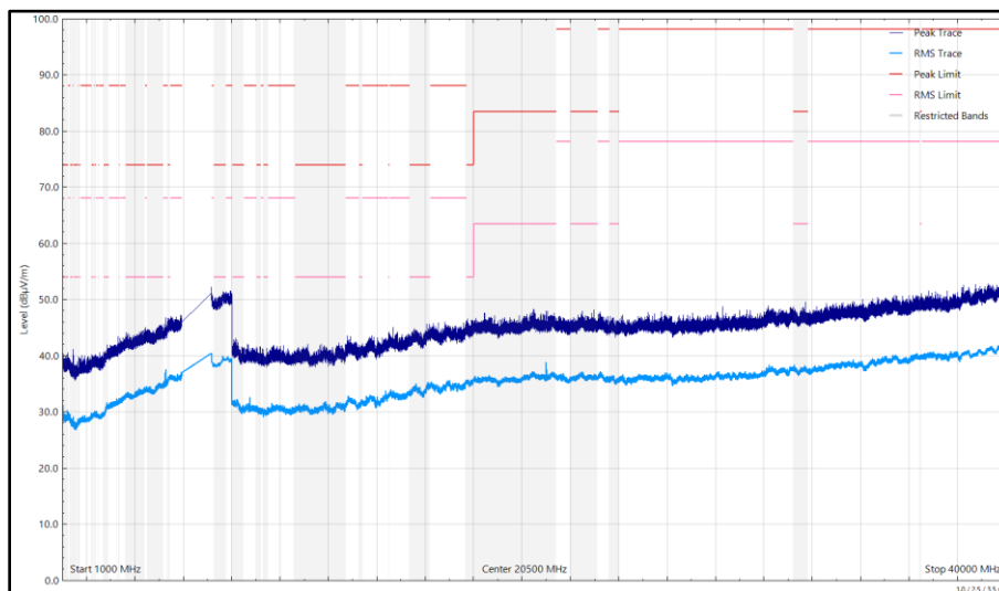
Figure 300 - U-NII-8 - 6995 MHz (CH209), HE20, SU, CDD, Core 0 + Core 1, 1 GHz to 40 GHz, Horizontal
