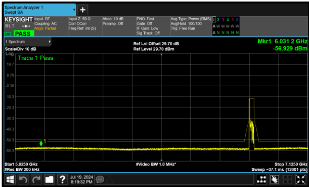
Figure 311 - A (Core 0) 802.11ax HE20 RU26 LPI 6895 MHz (CH189)
