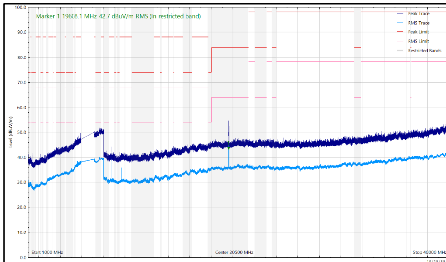
Figure 290 - U-NII-7 - 6535 MHz (CH117), HE20, SU, CDD, Core 0 + Core 1, 1 GHz to 40 GHz, Vertical
