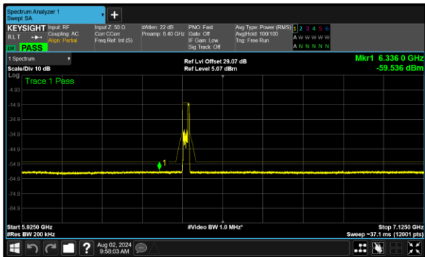
Figure 352 - B (Core 1) 802.11ax HE20 RU52 LPI 6415 MHz (CH93)
