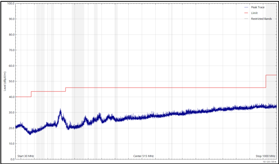
Figure 301 - U-NII-8 - 6995 MHz (CH209), HE20, SU, CDD, Core 0 + Core 1, 30 MHz to 1 GHz, Vertical (Peak)
