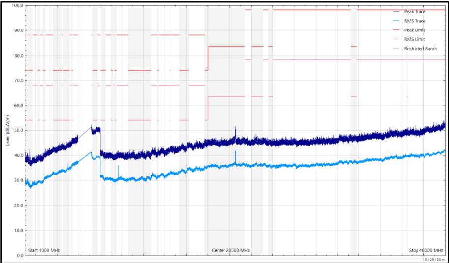
Figure 296 - U-NII-7 - 6855 MHz (CH181), HE20, SU, CDD, Core 0 + Core 1, 1 GHz to 40 GHz, Vertical
