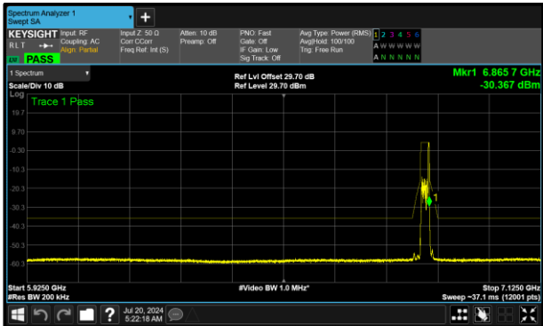
Figure 319 - A (Core 0) 802.11ax HE20 RU26 SP 6855 MHz (CH181)
