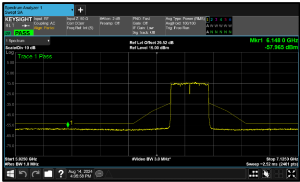
Figure 325 – A (Core 0) 802.11ax HE160 SU VLP 6665 MHz (CH143)
