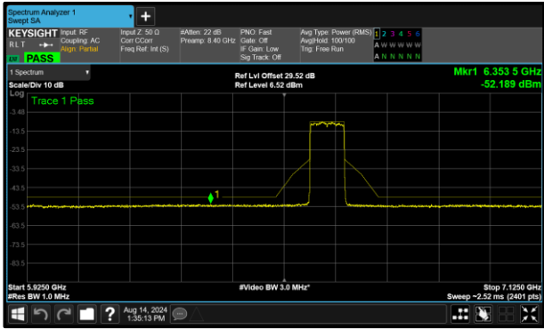
Figure 324 – A (Core 0) 802.11ax HE80 SU VLP 6625 MHz (CH135)
