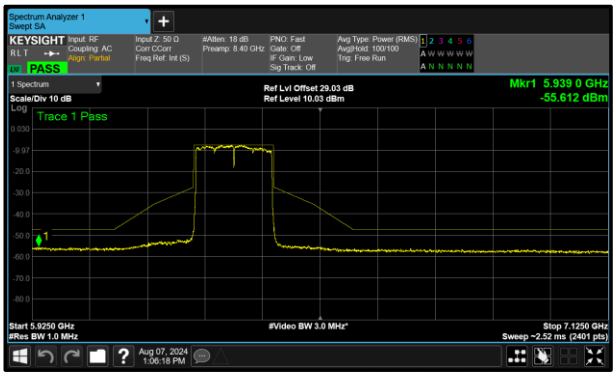
Figure 349 - B (Core 1) 802.11ax HE160 SU LPI 6345 MHz (CH79)
