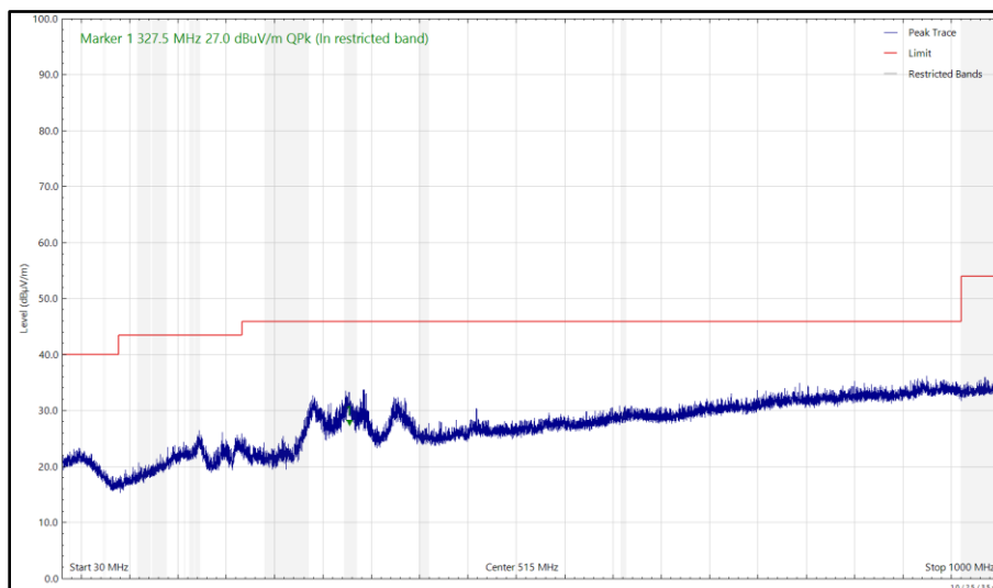
Figure 299 - U-NII-8 - 6995 MHz (CH209), HE20, SU, CDD, Core 0 + Core 1, 30 MHz to 1 GHz, Horizontal (Peak)
