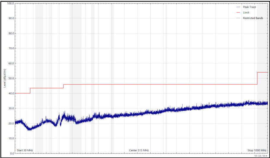
Figure 293 - U-NII-7 - 6695 MHz (CH149), HE20, SU, CDD, Core 0 + Core 1, 30 MHz to 1 GHz, Vertical (Peak)
