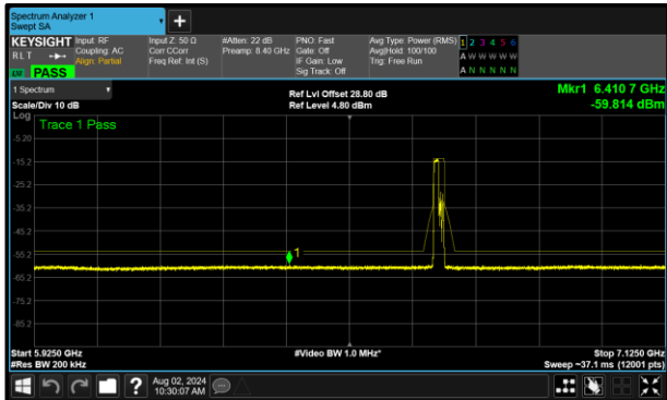
Figure 350 - B (Core 1) 802.11ax HE20 RU106 LPI 6695 MHz (CH149)
