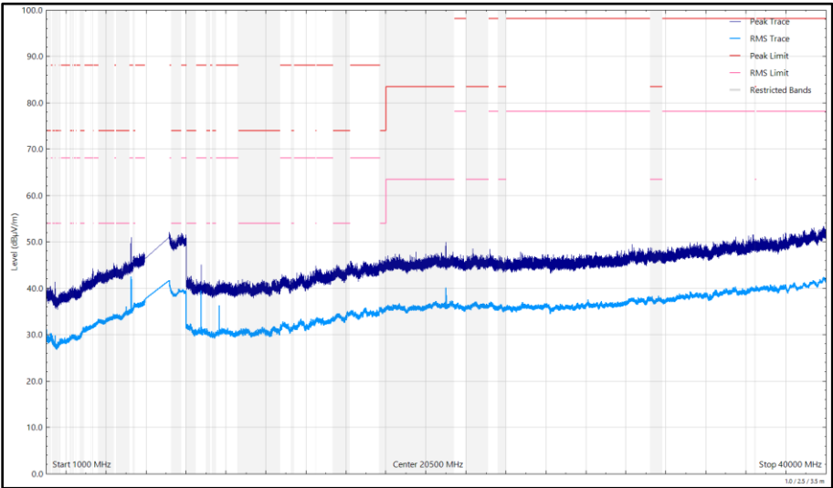
Figure 302 - U-NII-8 - 6995 MHz (CH209), HE20, SU, CDD, Core 0 + Core 1, 1 GHz to 40 GHz, Vertical
