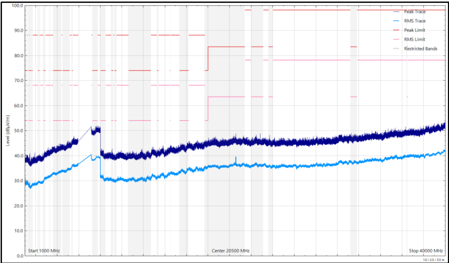
Figure 295 - U-NII-7 - 6855 MHz (CH181), HE20, SU, CDD, Core 0 + Core 1, 1 GHz to 40 GHz, Horizontal
