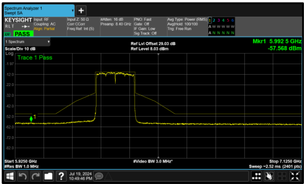
Figure 331 - B (Core 1) 802.11ax HE160 SU LPI 6345 MHz (CH79)
