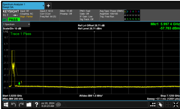
Figure 340 - A (Core 0) 802.11ax HE20 RU26 SP 5955 MHz (CH1)
