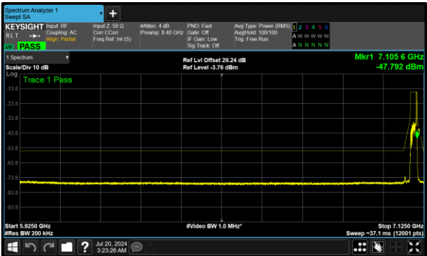
Figure 351 - B (Core 1) 802.11ax HE20 RU26 LPI 7095 MHz (CH229)
