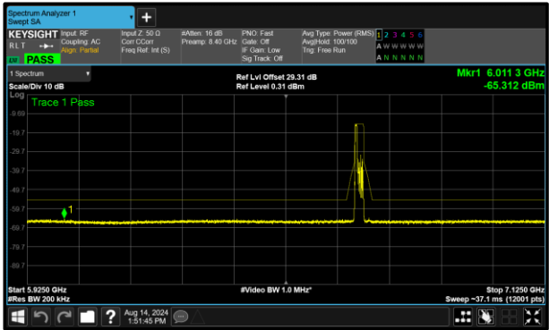
Figure 327 – A (Core 0) 802.11ax HE20 RU52 VLP 6695 MHz (CH149)
