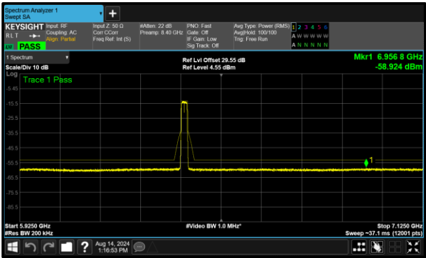
Figure 321 – A (Core 0) 802.11a VLP 6415 MHz (CH93)
