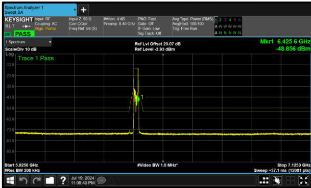
Figure 333 - B (Core 1) 802.11ax HE20 RU26 LPI 6415 MHz (CH93)
