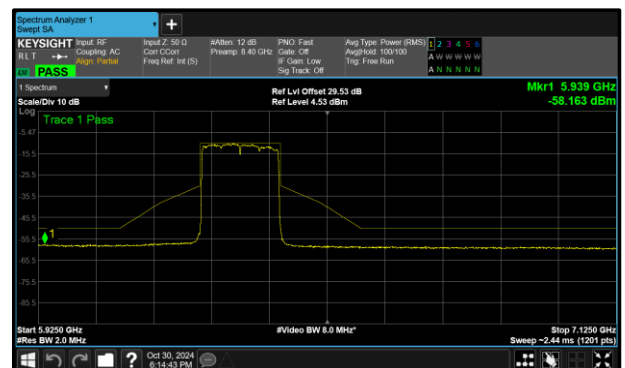
Figure 345 – A (Core 0) 802.11ax HE160 SU VLP 6345 MHz (CH79)
