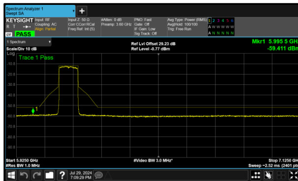
Figure 422 - A (Core 0) 6145 MHz (CH39)
