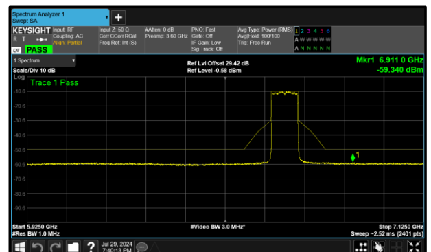
Figure 433 - B (Core 1) 6705 MHz (CH151)
