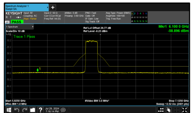
Figure 427 - B (Core 1) 6465 MHz (CH103)
