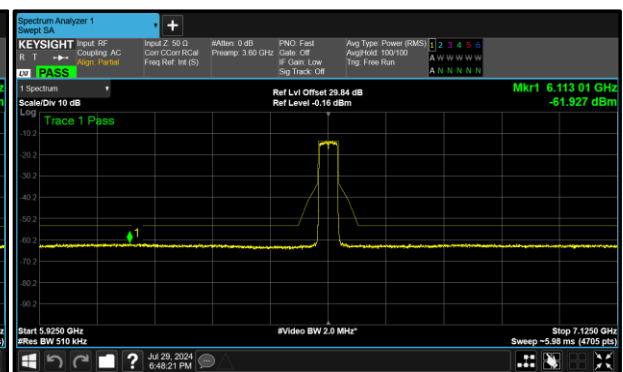
Figure 405 - B (Core 1) 6525 MHz (CH115)
