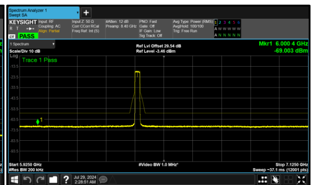
Figure 373 - B (Core 1) 6415 MHz (CH93)
