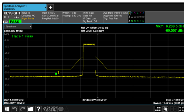
Figure 426 - A (Core 0) 6465 MHz (CH103)
