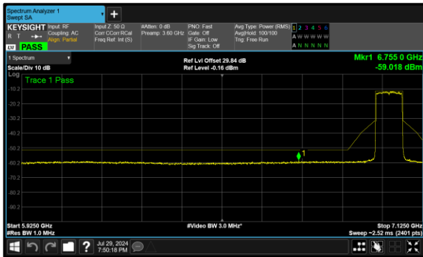
Figure 441 - B (Core 1) 7025 MHz (CH215)
