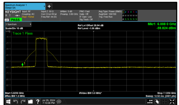
Figure 423 - B (Core 1) 6145 MHz (CH39)
