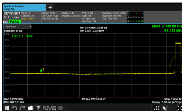
Figure 418 - A (Core 0) 7085 MHz (CH227)
