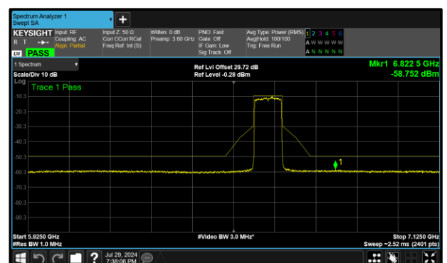
Figure 431 - B (Core 1) 6625 MHz (CH135)
