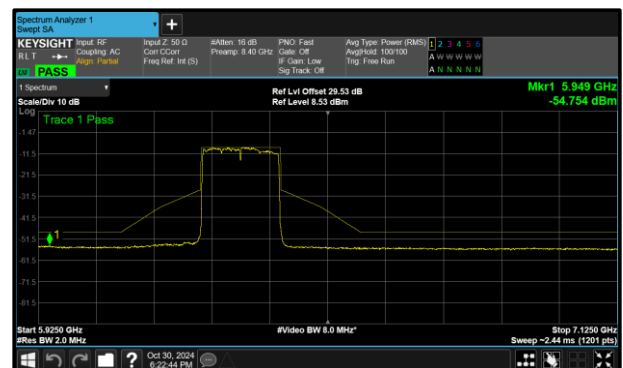
Figure 363 – A(Core 0) 802.11ax HE160 SU VLP 6345 MHz (CH79)
