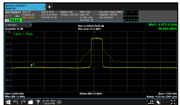
Figure 429 - B (Core 1) 6545 MHz (CH119)
