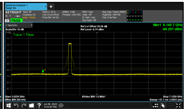
Figure 371 - B (Core 1) 6335 MHz (CH77)
