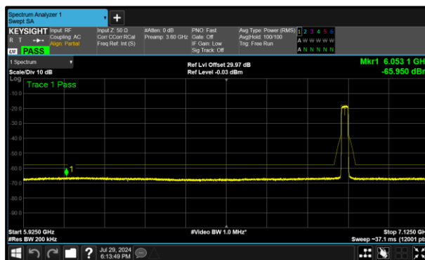
Figure 386 - A (Core 0) 6875 MHz (CH185)
