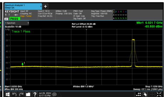
Figure 389 - B (Core 1) 6895 MHz (CH189)
