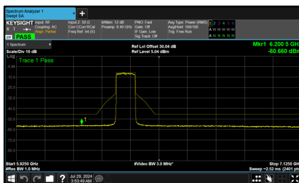
Figure 424 - A (Core 0) 6385 MHz (CH87)
