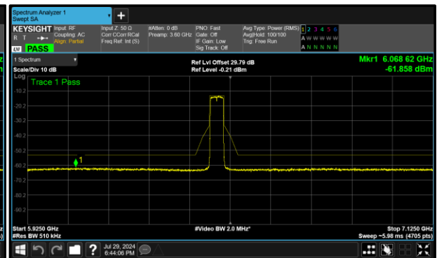
Figure 403 - B (Core 1) 6485 MHz (CH107)
