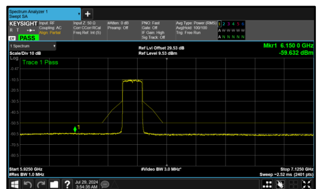
Figure 425 - B (Core 1) 6385 MHz (CH87)
