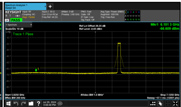
Figure 383 - B (Core 1) 6695 MHz (CH149)
