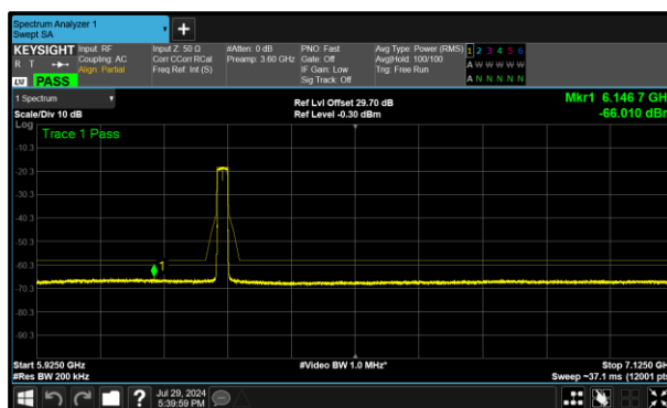
Figure 368 - A (Core 0) 6275 MHz (CH65)
