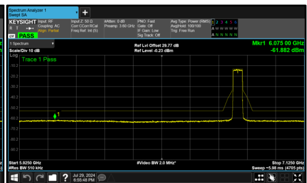
Figure 411 - B (Core 1) 6845 MHz (CH179)
