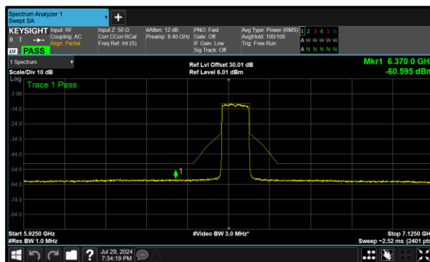
Figure 428 - A (Core 0) 6545 MHz (CH119)
