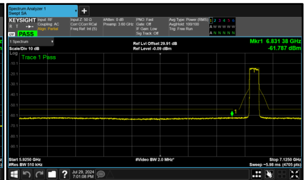
Figure 415 - B (Core 1) 6925 MHz (CH195)
