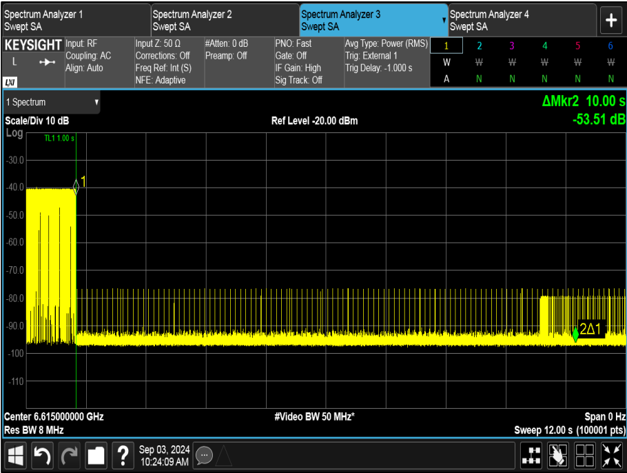
Figure 522 - U-NII-7, Maximum Bandwidth (AWGN Mid)
