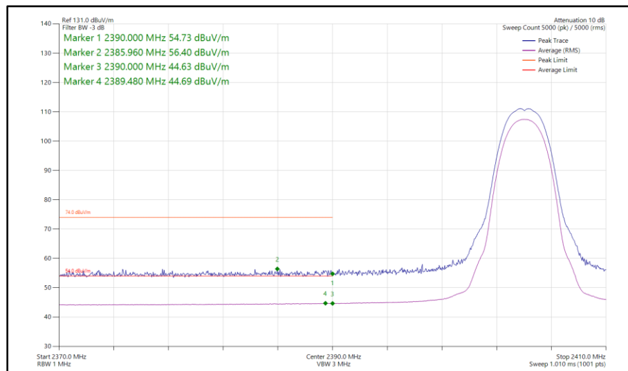
Figure 51 - Bluetooth HDR4, SISO, Core 1 - 2404 MHz Band Edge Frequency 2390 MHz
