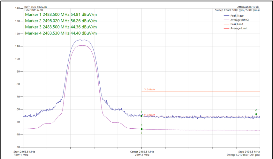
Figure 63 - Bluetooth HDR4, MIMO, Core 0 - Core 1 - 2476 MHz Band Edge Frequency 2483.5 MHz
