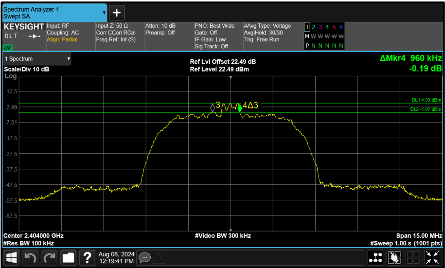
Figure 150 - Core 0 (A) 2404 MHz (CH2) 6 dB Bandwidth
