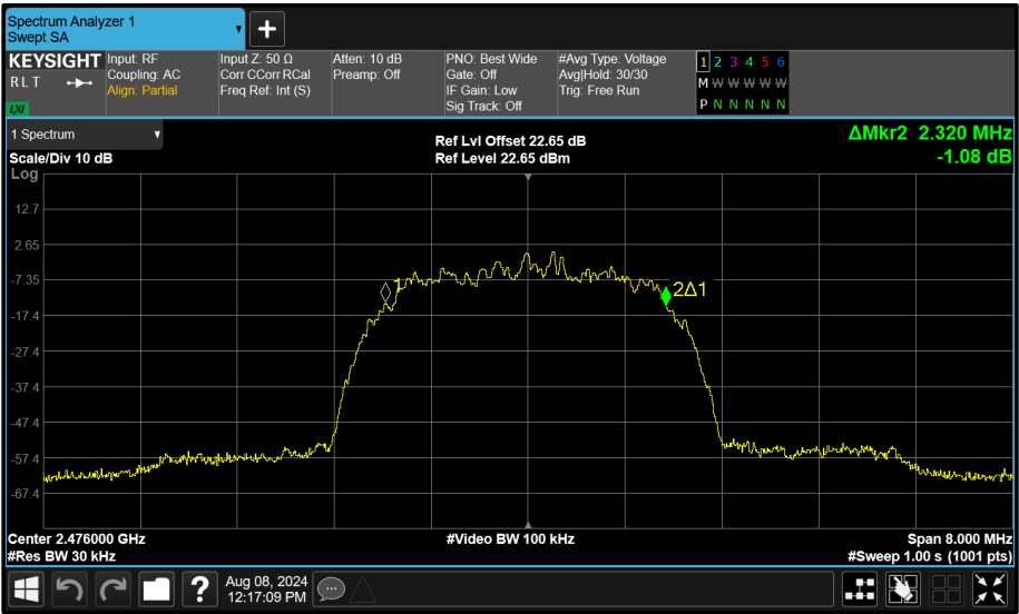
Figure 147 - Core 1 (B) 2476 MHz (CH74) 99% Bandwidth
