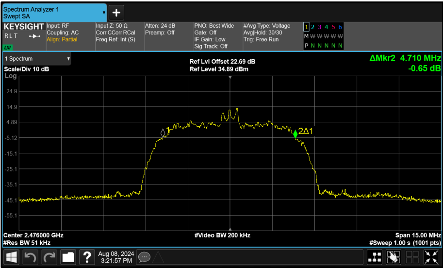
Figure 123 - Core 0 (A) 2476 MHz (CH74) 99% Bandwidth
