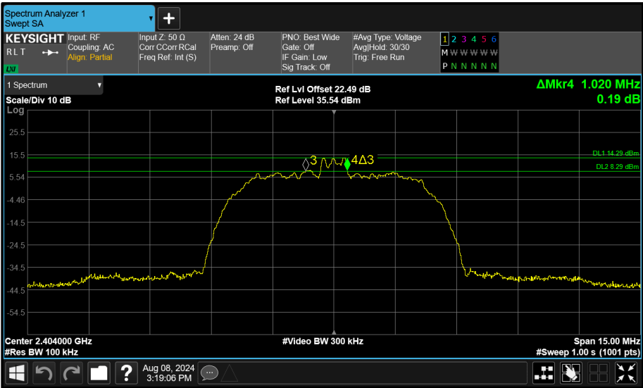
Figure 120 - Core 0 (A) 2404 MHz (CH2) 6 dB Bandwidth
