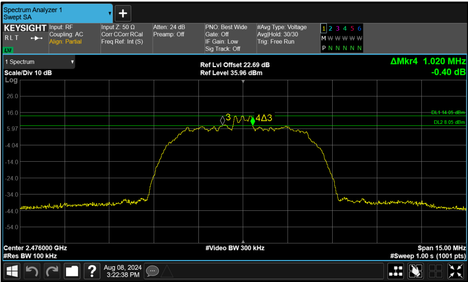
Figure 124 - Core 0 (A) 2476 MHz (CH74) 6 dB Bandwidth
