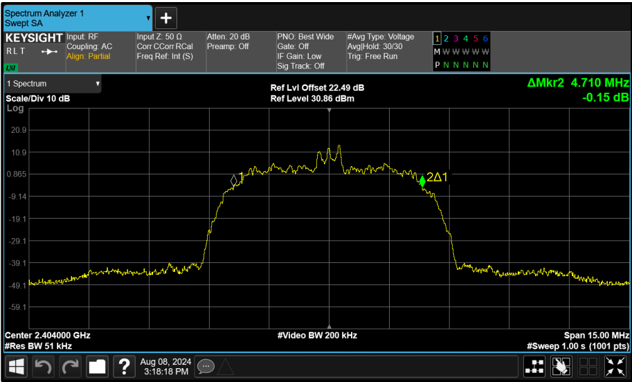
Figure 119 - Core 0 (A) 2404 MHz (CH2) 99% Bandwidth
