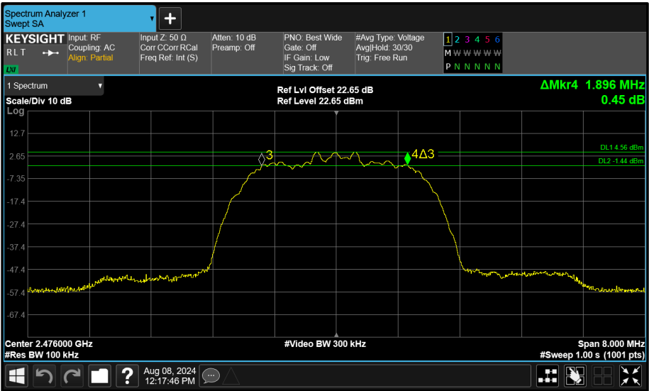
Figure 148 - Core 1 (B) 2476 MHz (CH74) 6 dB Bandwidth
