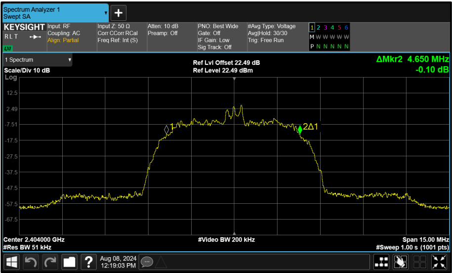
Figure 149 - Core 0 (A) 2404 MHz (CH2) 99% Bandwidth
