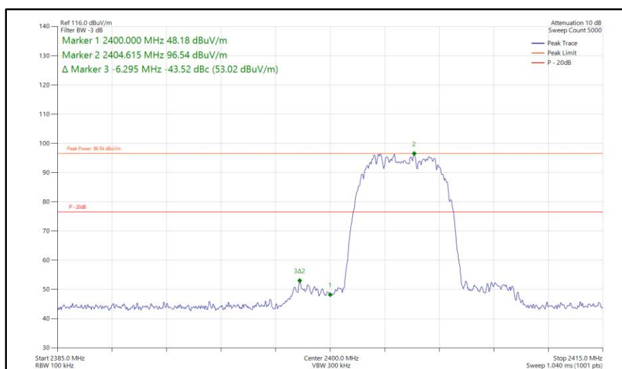
Figure 228 - Bluetooth HDR8, MIMO, Core 0-1 - 2404 MHz Band Edge Frequency 2400 MHz
