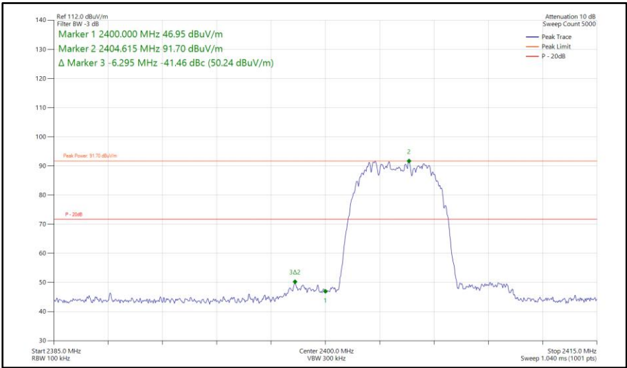
Figure 216 - Bluetooth HDR8, SISO, Core 1 - 2404 MHz Band Edge Frequency 2400 MHz
