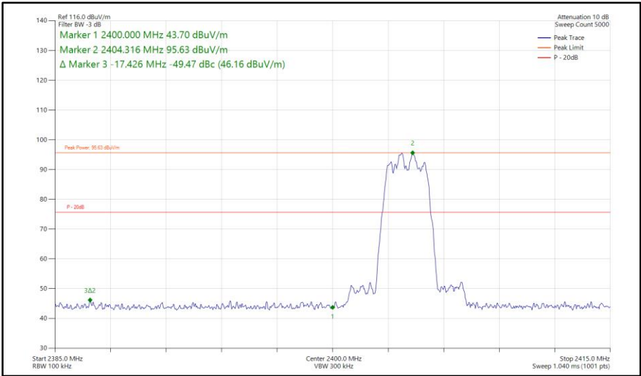
Figure 215 - Bluetooth HDR4, SISO, Core 1 - 2404 MHz Band Edge Frequency 2400 MHz
