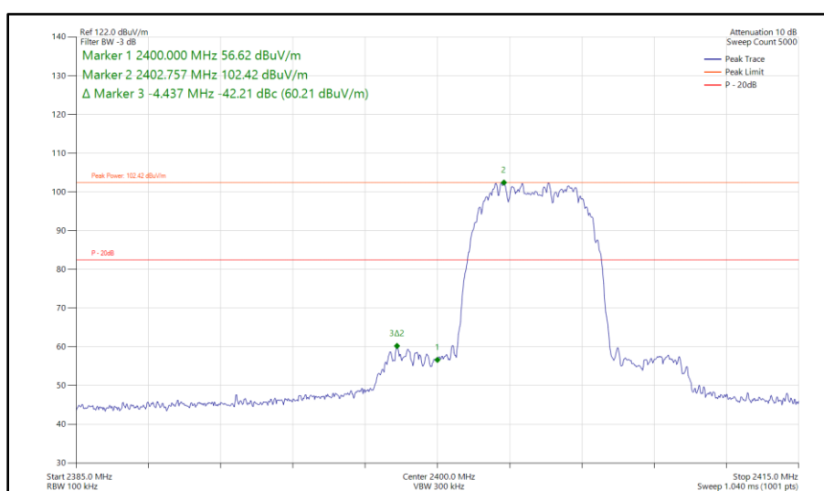
Figure 234 - Bluetooth HDR8, SISO, Core 0 - 2404 MHz Band Edge Frequency 2400 MHz
