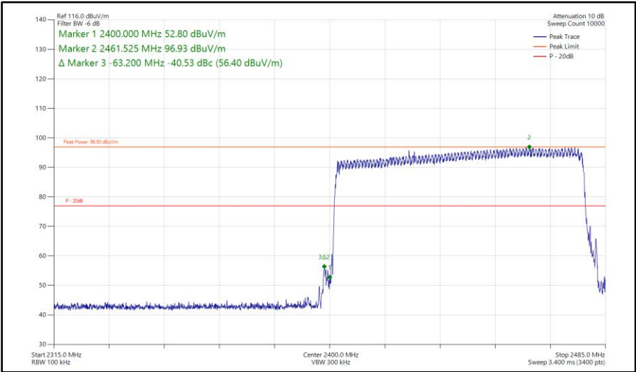
Figure 214 - Bluetooth HDR8, SISO, Core 0 - Hopping Band Edge Frequency 2400 MHz
