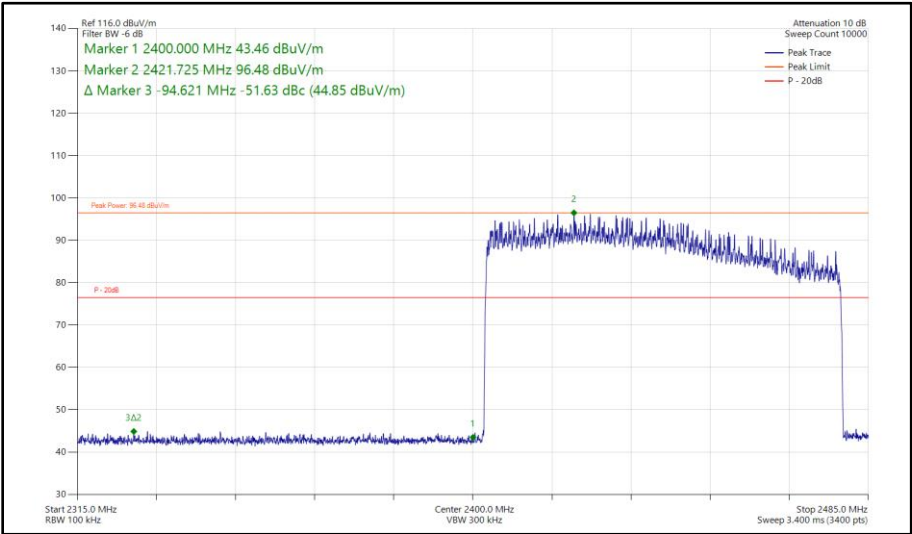
Figure 225 - Bluetooth HDR4, SISO, Core 2 - Hopping Band Edge Frequency 2400 MHz
