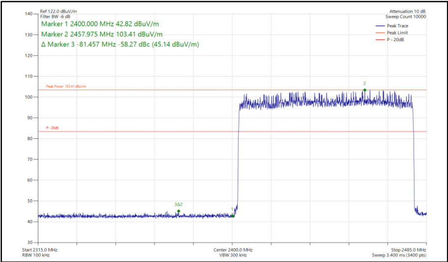
Figure 231 - Bluetooth HDR4, MIMO, Core 0-1 - Hopping Band Edge Frequency 2400 MHz
