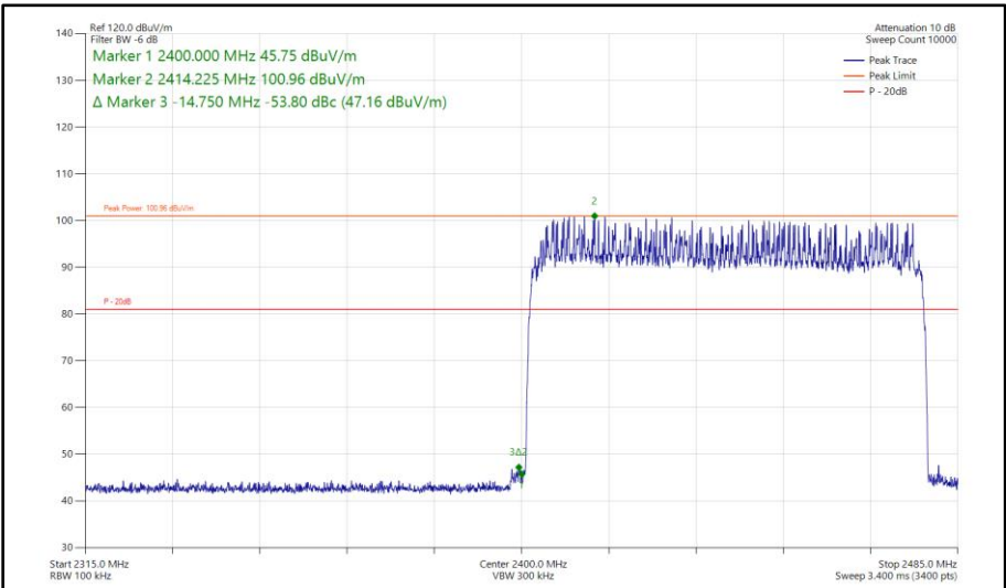
Figure 232 - Bluetooth HDR8, MIMO, Core 0-1 - Hopping Band Edge Frequency 2400 MHz
