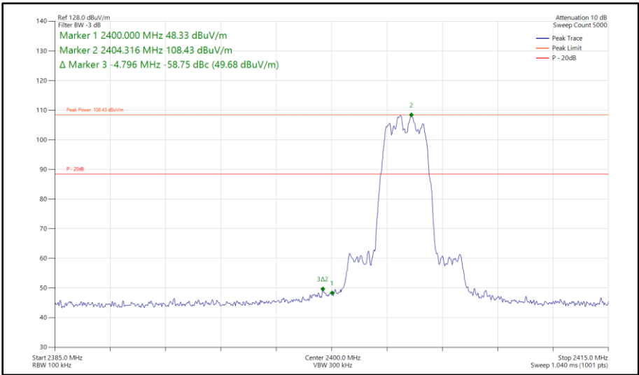
Figure 245 - Bluetooth HDR4, MIMO, Core 0-1 - 2404 MHz Band Edge Frequency 2400 MHz
