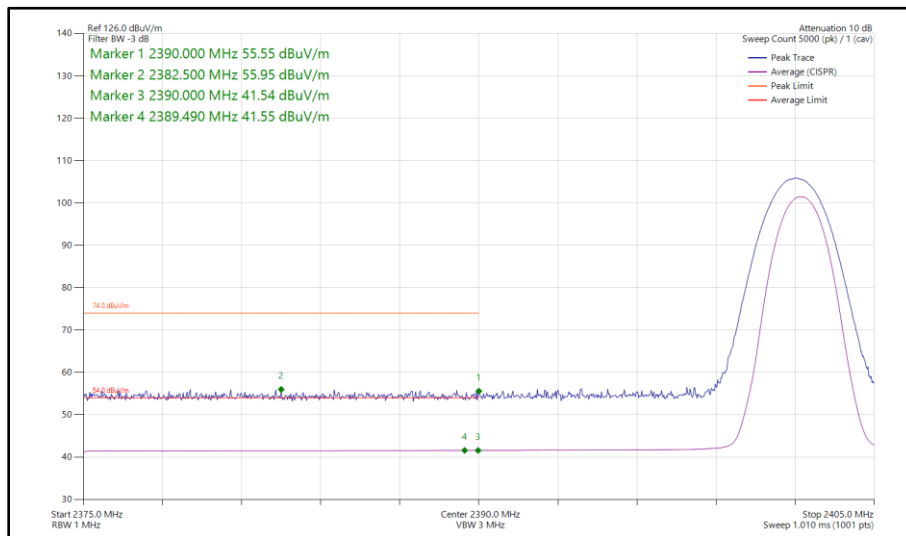
Figure 15 - Bluetooth 3-DH5, SISO, Core 2 - 2402 MHz Band Edge Frequency 2390 MHz
