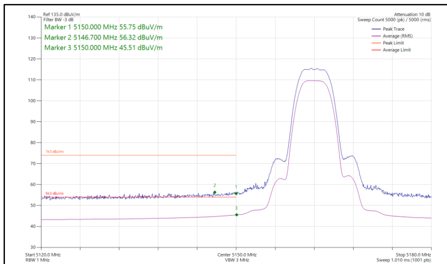
Figure 24 - Narrowband HDR8, SISO, Core 1 - 5162 MHz Band Edge Frequency 5150 MHz
