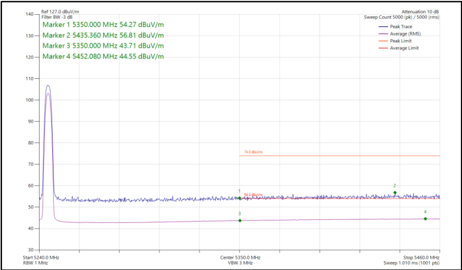
Figure 17 - Narrowband HDR4, MIMO, Core 0 - Core 1 - 5245 MHz Band Edge Frequency 5350 MHz
