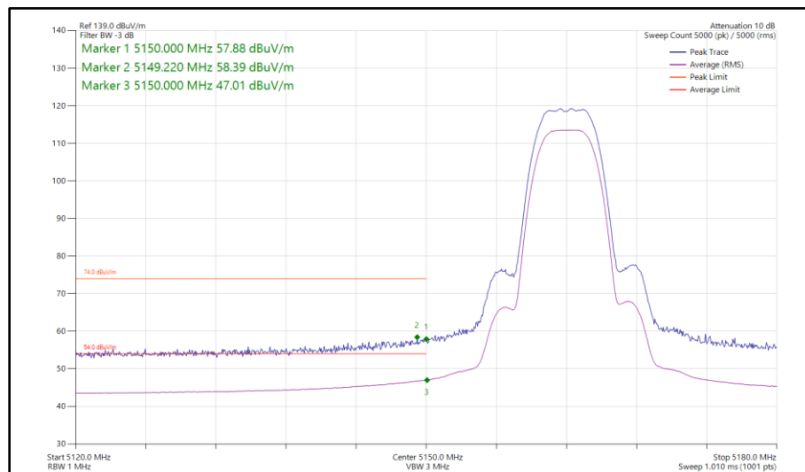
Figure 28 - Narrowband HDR8, MIMO, Core 0 - Core 1 - 5162 MHz Band Edge Frequency 5150 MHz
