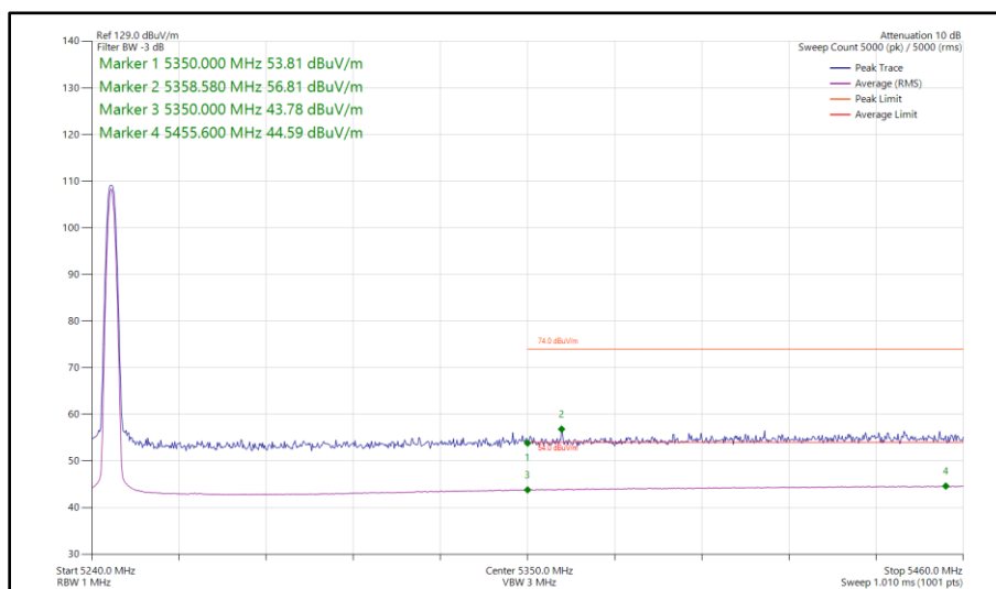
Figure 10 - Narrowband DH5, SISO, Core 1 - 5245 MHz Band Edge Frequency 5350 MHz
