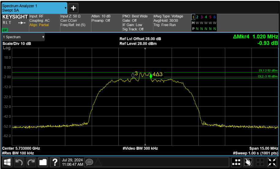
Figure 59 - Core 1 (B) 5733 MHz (CH8) 6 dB Bandwidth
