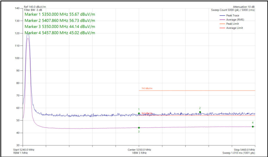
Figure 21 - Narrowband HDR4, SISO, Core 0 - 5245 MHz Band Edge Frequency 5350 MHz
