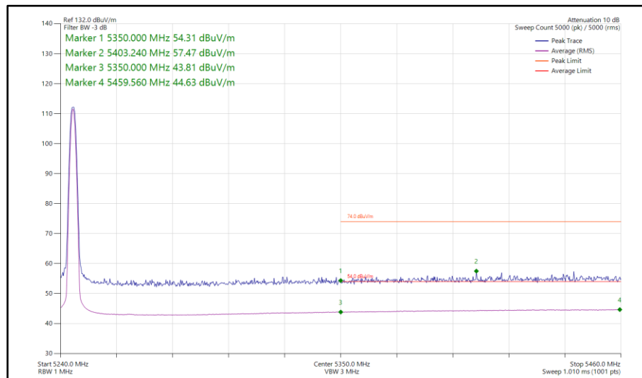
Figure 4 - Narrowband DH5, SISO, Core 0 - 5245 MHz Band Edge Frequency 5350 MHz
