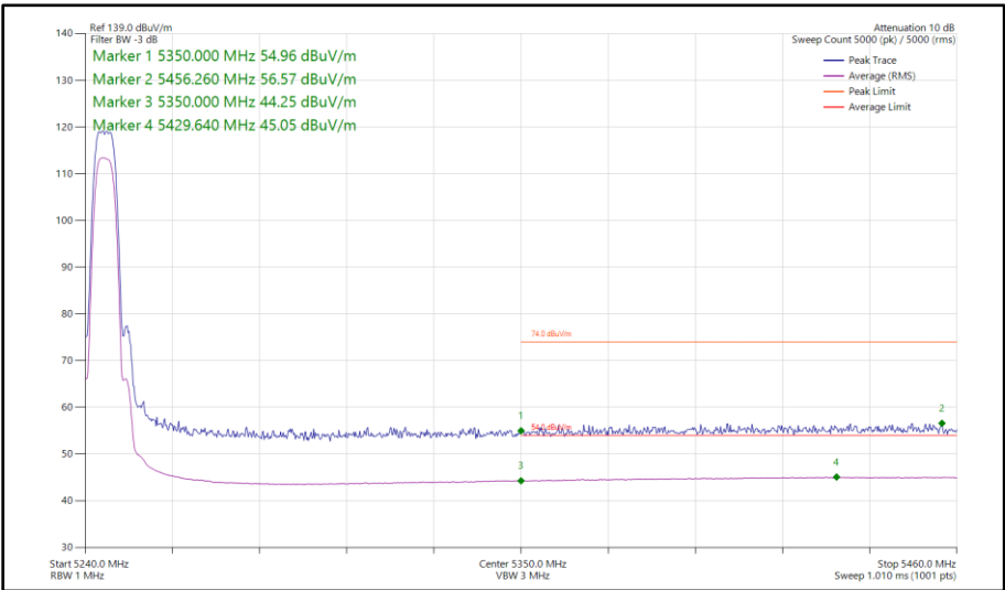
Figure 22 - Narrowband HDR8, SISO, Core 0 - 5245 MHz Band Edge Frequency 5350 MHz
