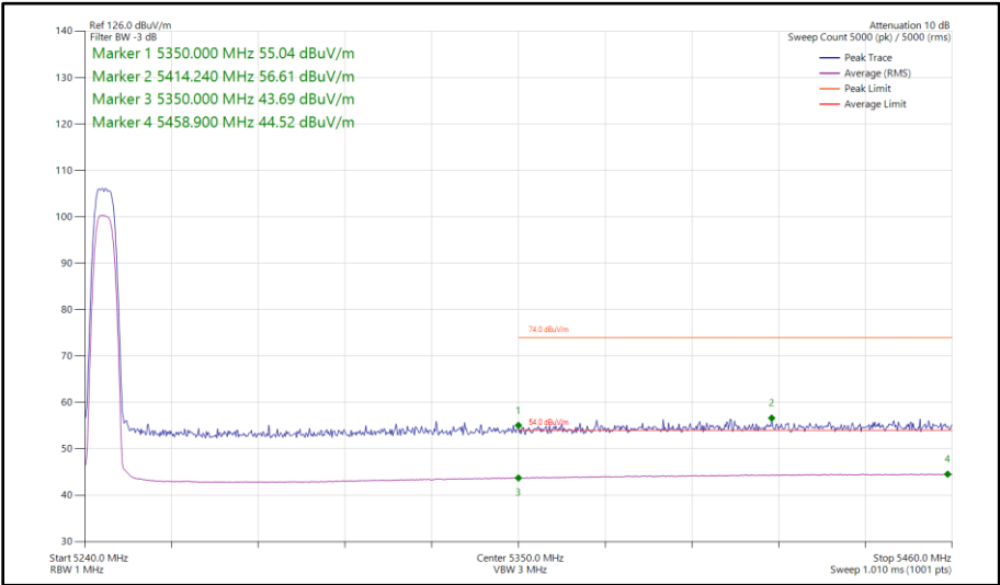
Figure 6 - Narrowband HDR8, SISO, Core 0 - 5245 MHz Band Edge Frequency 5350 MHz
