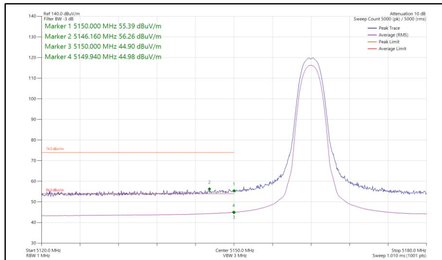
Figure 27 - Narrowband HDR4, MIMO, Core 0 - Core 1 - 5162 MHz Band Edge Frequency 5150 MHz
