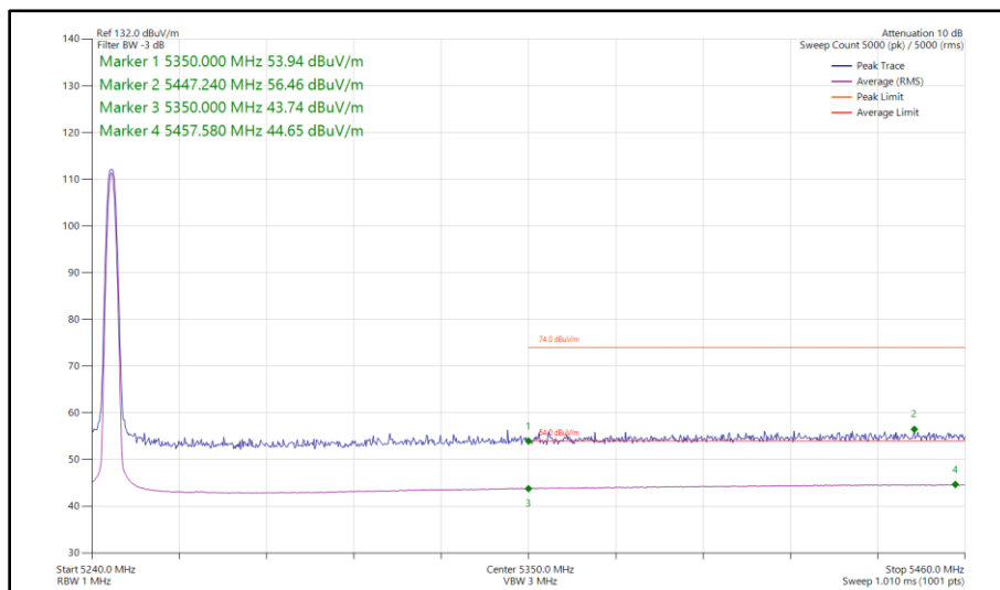
Figure 16 - Narrowband DH5, MIMO, Core 0 - Core 1 - 5245 MHz Band Edge Frequency 5350 MHz
