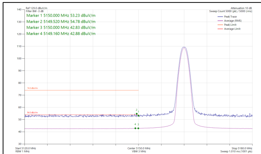
Figure 1 - Narrowband DH5, SISO, Core 0 - 5162 MHz Band Edge Frequency 5150 MHz
