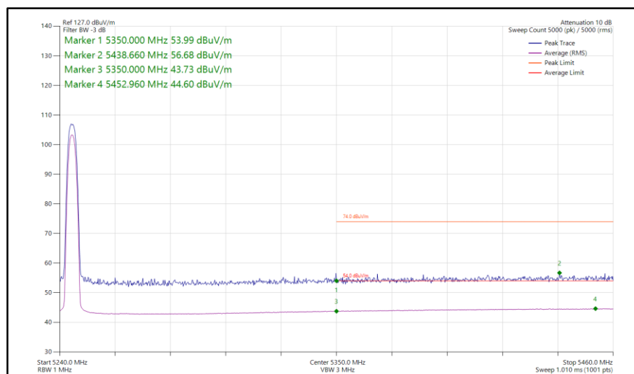
Figure 5 - Narrowband HDR4, SISO, Core 0 - 5245 MHz Band Edge Frequency 5350 MHz
