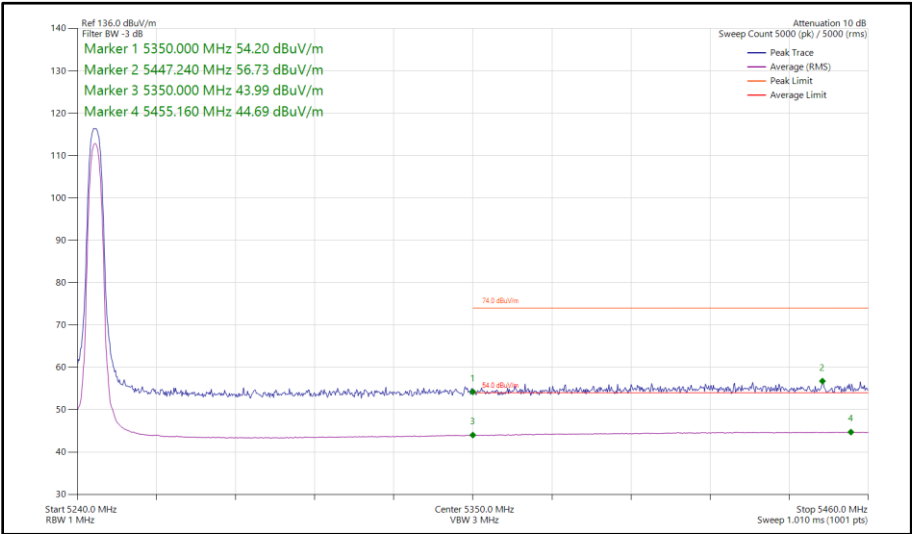
Figure 25 - Narrowband HDR4, SISO, Core 1 - 5245 MHz Band Edge Frequency 5350 MHz
