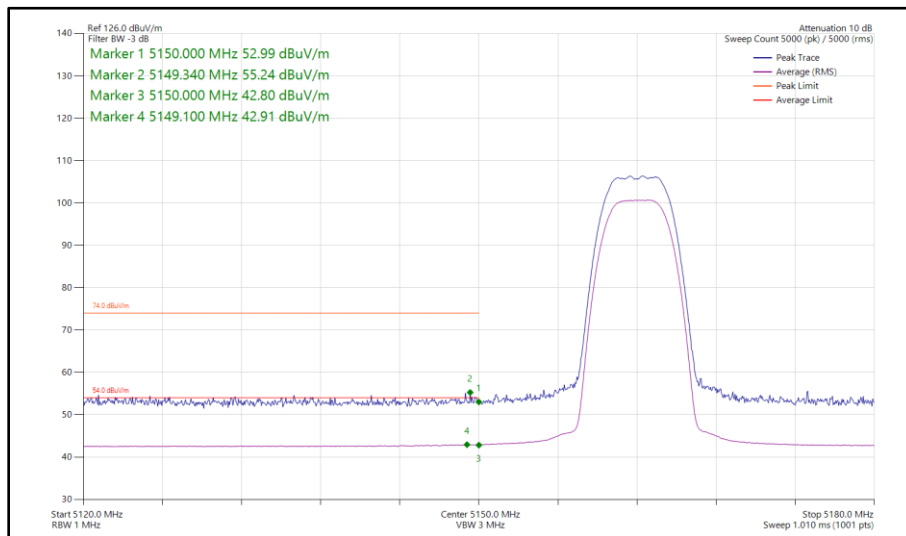
Figure 15 - Narrowband HDR8, MIMO, Core 0 - Core 1 - 5162 MHz Band Edge Frequency 5150 MHz
