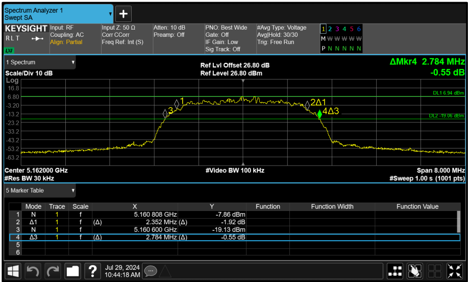
Figure 40 - Core 1 (B) 5162 MHz (CH12) 26 dB and 99% Bandwidth
