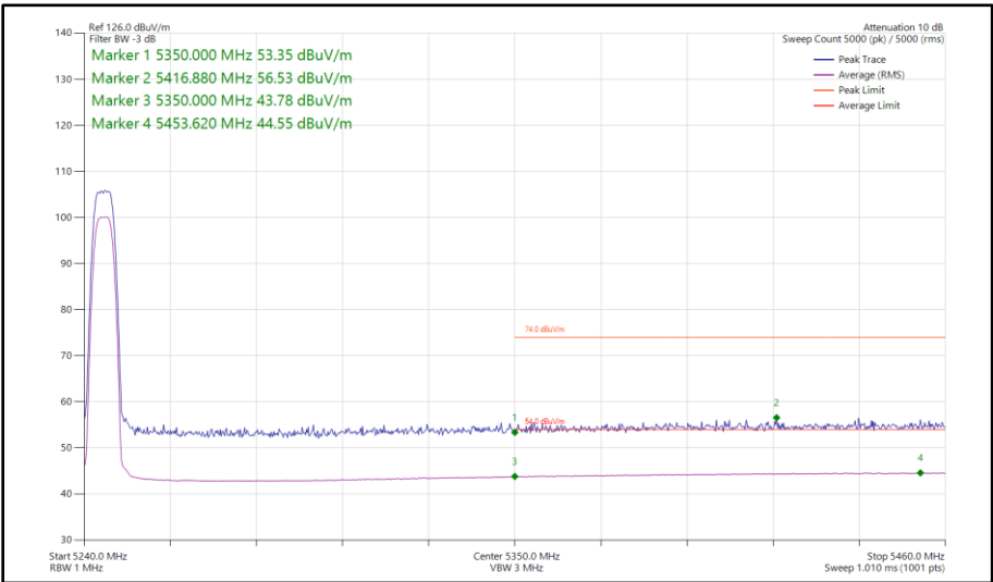
Figure 18 - Narrowband HDR8, MIMO, Core 0 - Core 1 - 5245 MHz Band Edge Frequency 5350 MHz
