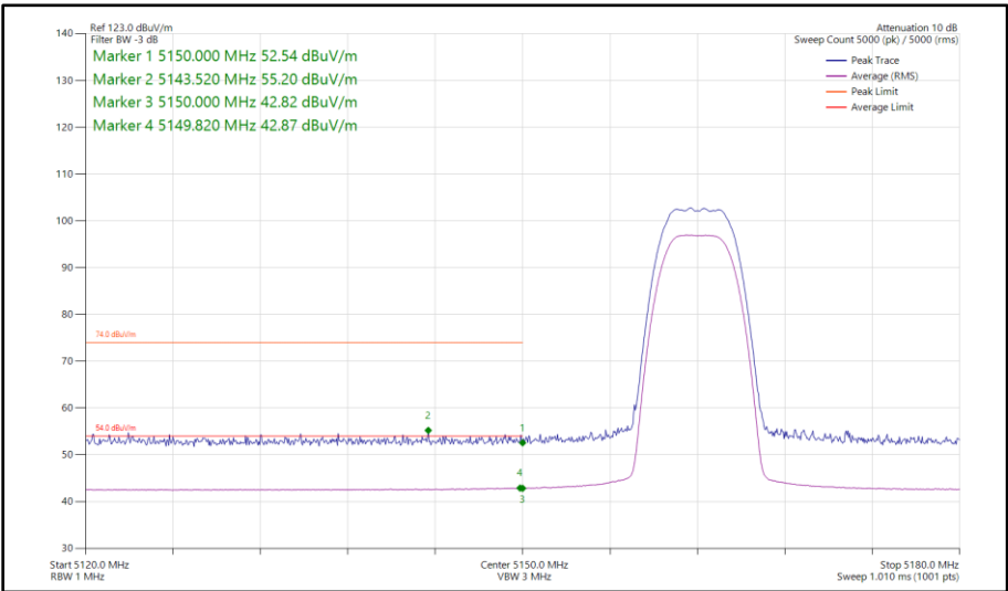
Figure 3 - Narrowband HDR8, SISO, Core 0 - 5162 MHz Band Edge Frequency 5150 MHz
