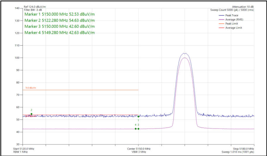
Figure 2 - Narrowband HDR4, SISO, Core 0 - 5162 MHz Band Edge Frequency 5150 MHz
