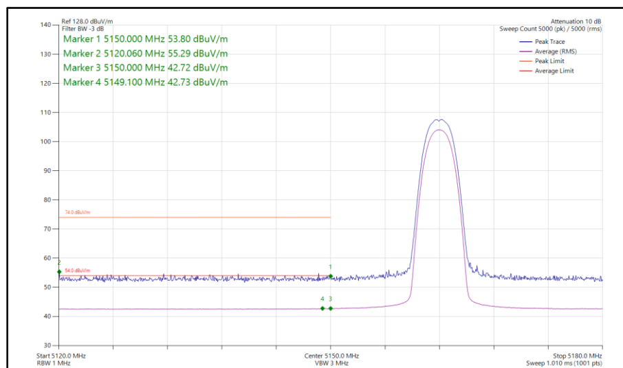
Figure 14 - Narrowband HDR4, MIMO, Core 0 - Core 1 - 5162 MHz Band Edge Frequency 5150 MHz
