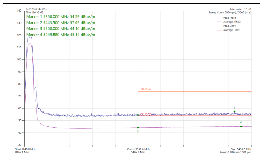
Figure 30 - Narrowband HDR8, MIMO, Core 0 - Core 1 - 5245 MHz Band Edge Frequency 5350 MHz
