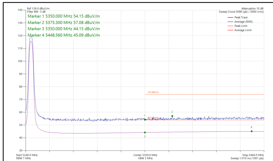
Figure 29 - Narrowband HDR4, MIMO, Core 0 - Core 1 - 5245 MHz Band Edge Frequency 5350 MHz
