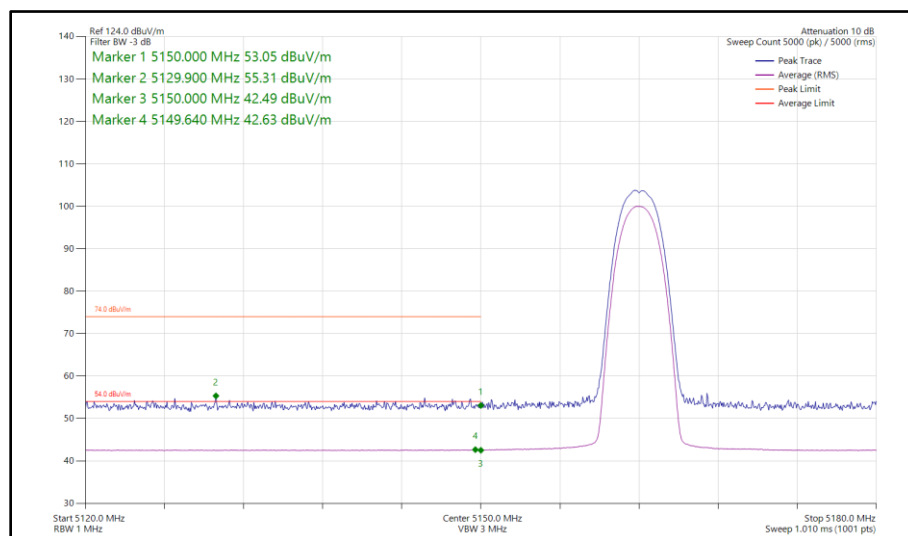
Figure 8 - Narrowband HDR4, SISO, Core 1 - 5162 MHz Band Edge Frequency 5150 MHz
