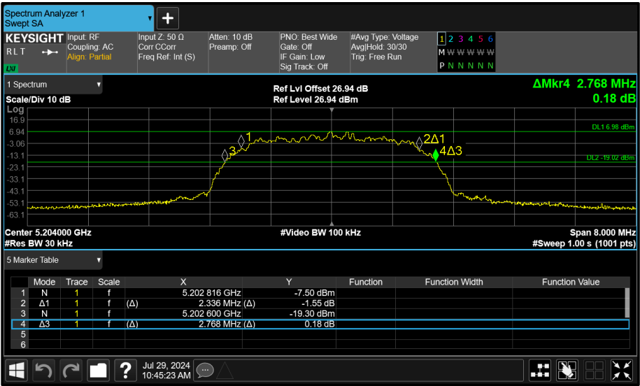
Figure 41 - Core 1 (B) 5204 MHz (CH54) 26 dB and 99% Bandwidth
