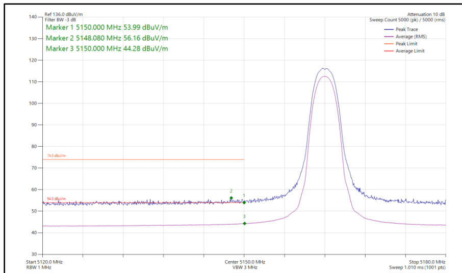
Figure 23 - Narrowband HDR4, SISO, Core 1 - 5162 MHz Band Edge Frequency 5150 MHz
