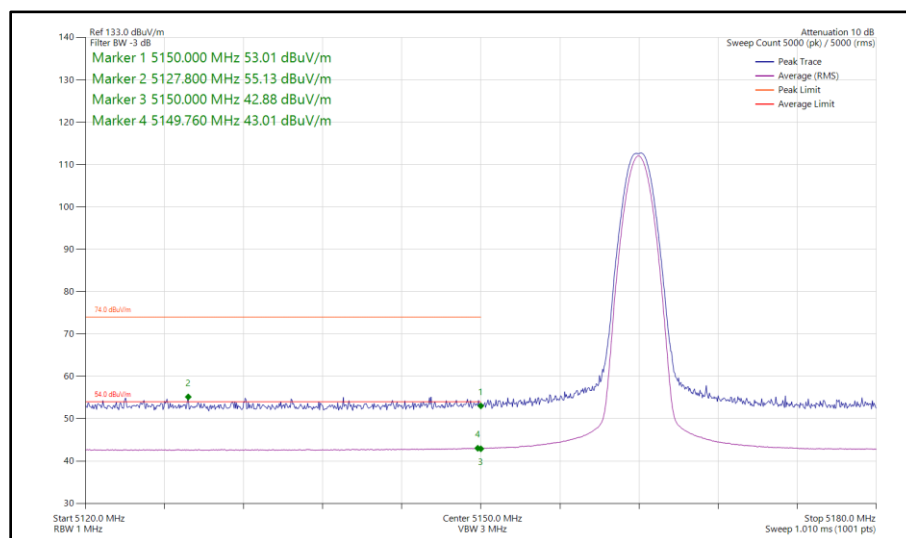
Figure 13 - Narrowband DH5, MIMO, Core 0 - Core 1 - 5162 MHz Band Edge Frequency 5150 MHz
