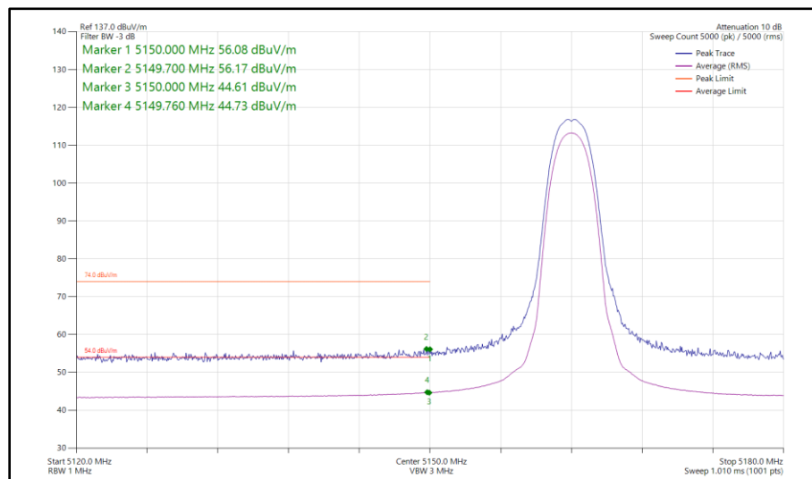
Figure 19 - Narrowband HDR4, SISO, Core 0 - 5162 MHz Band Edge Frequency 5150 MHz
