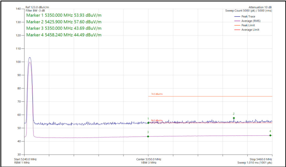
Figure 11 - Narrowband HDR4, SISO, Core 1 - 5245 MHz Band Edge Frequency 5350 MHz
