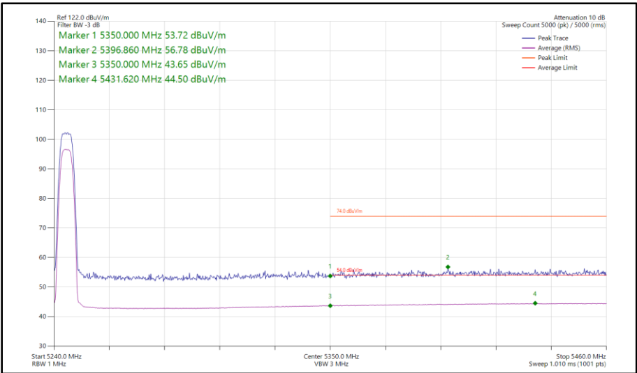
Figure 12 - Narrowband HDR8, SISO, Core 1 - 5245 MHz Band Edge Frequency 5350 MHz
