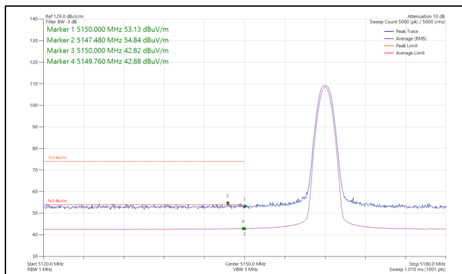
Figure 7 - Narrowband DH5, SISO, Core 1 - 5162 MHz Band Edge Frequency 5150 MHz
