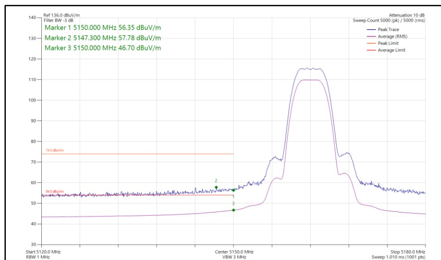
Figure 20 - Narrowband HDR8, SISO, Core 0 - 5162 MHz Band Edge Frequency 5150 MHz
