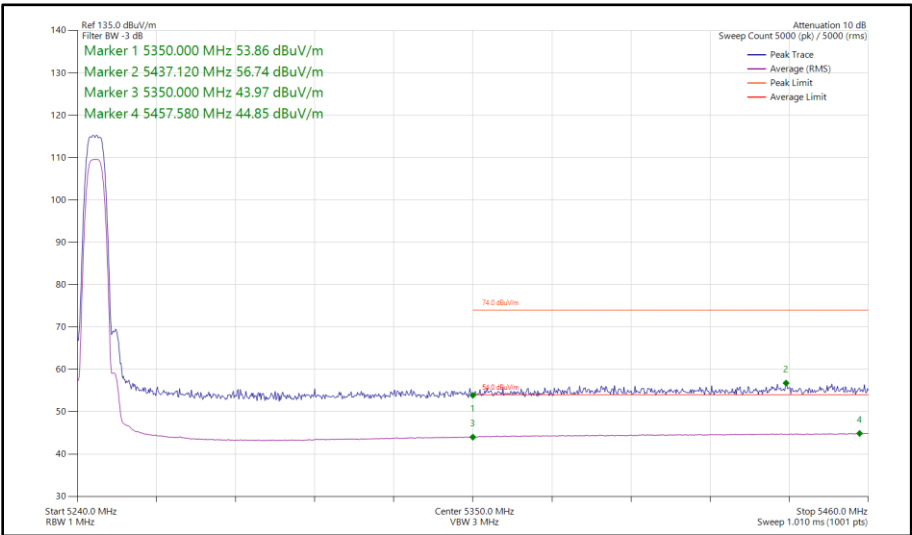
Figure 26 - Narrowband HDR8, SISO, Core 1 - 5245 MHz Band Edge Frequency 5350 MHz
