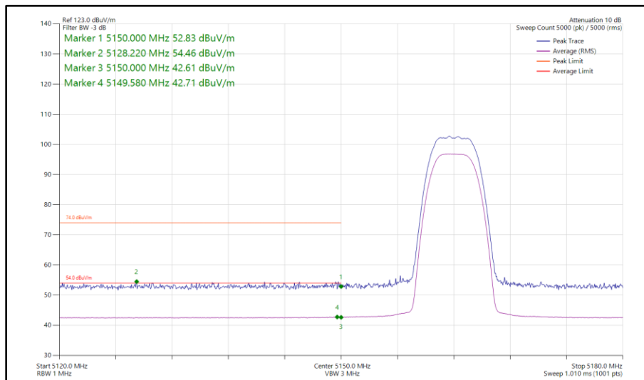
Figure 9 - Narrowband HDR8, SISO, Core 1 - 5162 MHz Band Edge Frequency 5150 MHz
