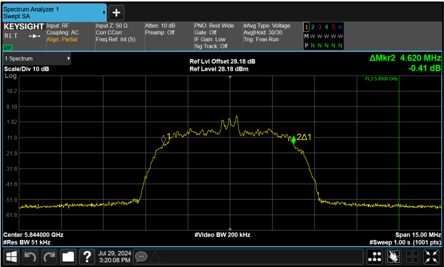
Figure 146 - Core 1 (B) 5844 MHz (CH119) 99% Bandwidth
