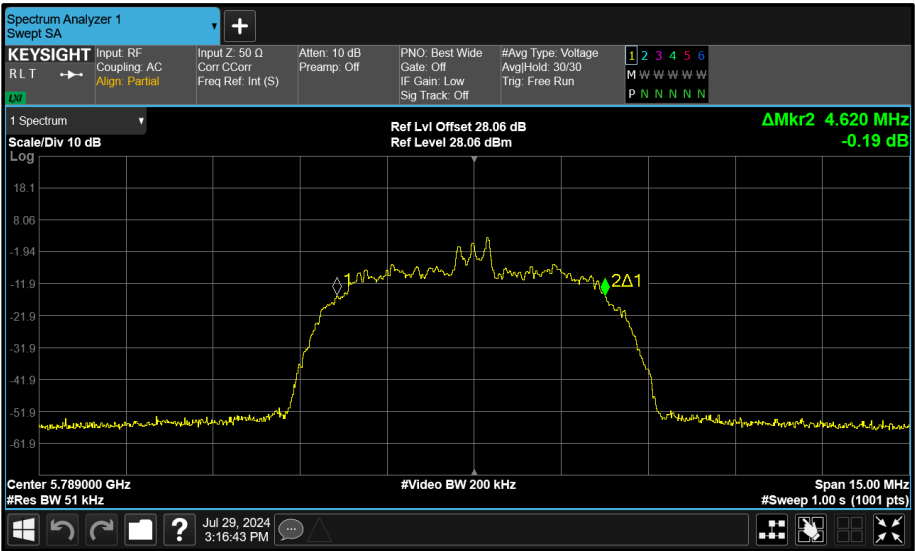
Figure 142 - Core 1 (B) 5789 MHz (CH64) 99% Bandwidth
