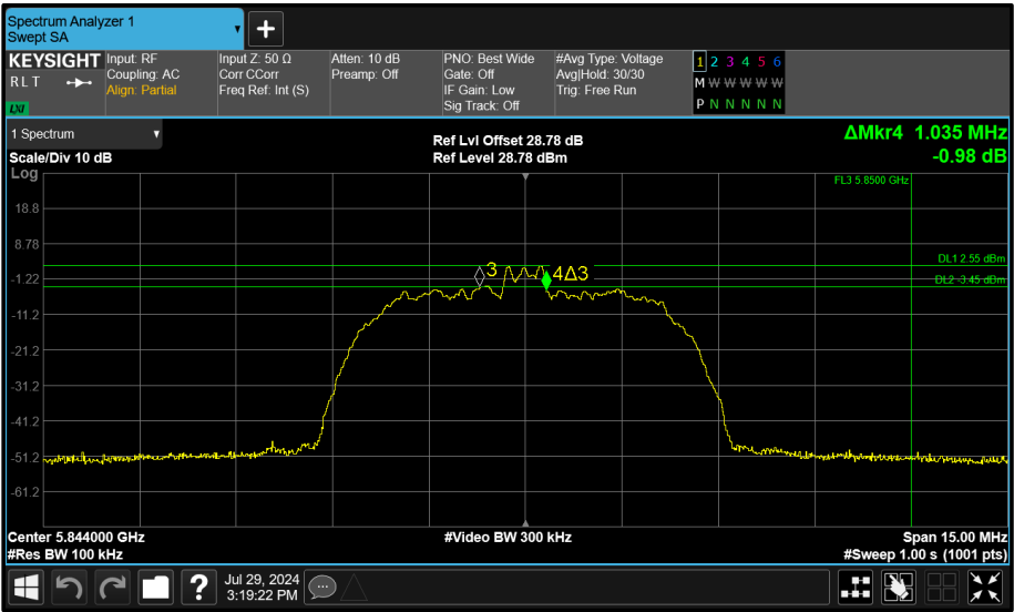
Figure 145 - Core 0 (A) 5844 MHz (CH119) 6 dB Bandwidth
