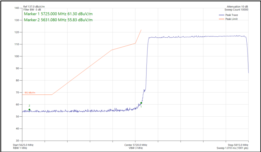
Figure 225 - Narrowband HDR8, SISO, Core 0 - 5733-5811 MHz Band Edge Frequency 5725 MHz
