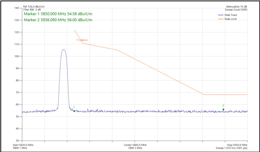
Figure 191 - Narrowband HDR4, SISO, Core 0 - 5844 MHz Band Edge Frequency 5850 MHz
