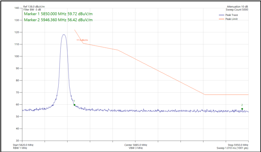
Figure 227 - Narrowband HDR4, SISO, Core 0 - 5844 MHz Band Edge Frequency 5850 MHz
