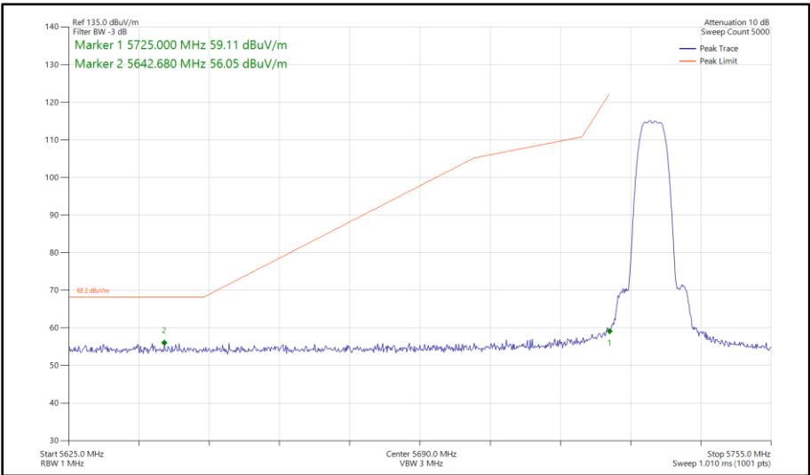
Figure 234 - Narrowband HDR8, SISO, Core 1 - 5733 MHz Band Edge Frequency 5725 MHz
