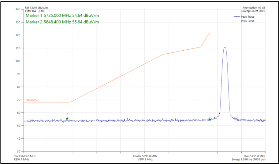
Figure 184 - Narrowband DH5, SISO, Core 0 - 5733 MHz Band Edge Frequency 5725 MHz
