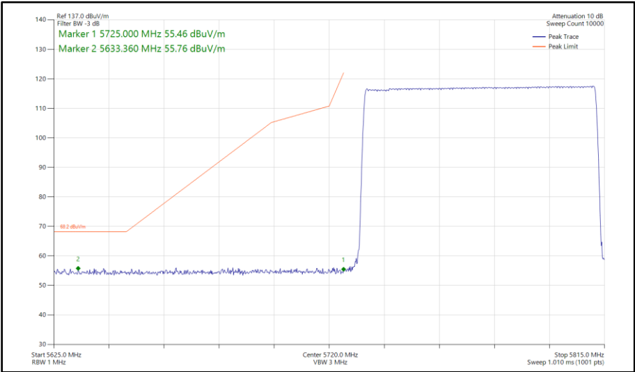
Figure 223 - Narrowband DH5, SISO, Core 0 - 5733-5811 MHz Band Edge Frequency 5725 MHz
