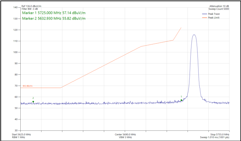
Figure 233 - Narrowband HDR4, SISO, Core 1 - 5733 MHz Band Edge Frequency 5725 MHz
