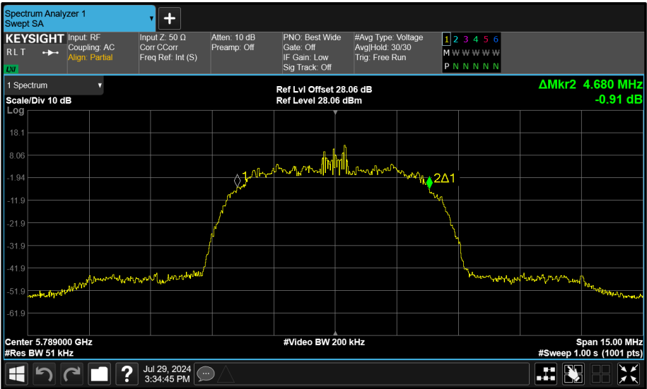
Figure 178 - Core 1 (B) 5789 MHz (CH64) 99% Bandwidth
