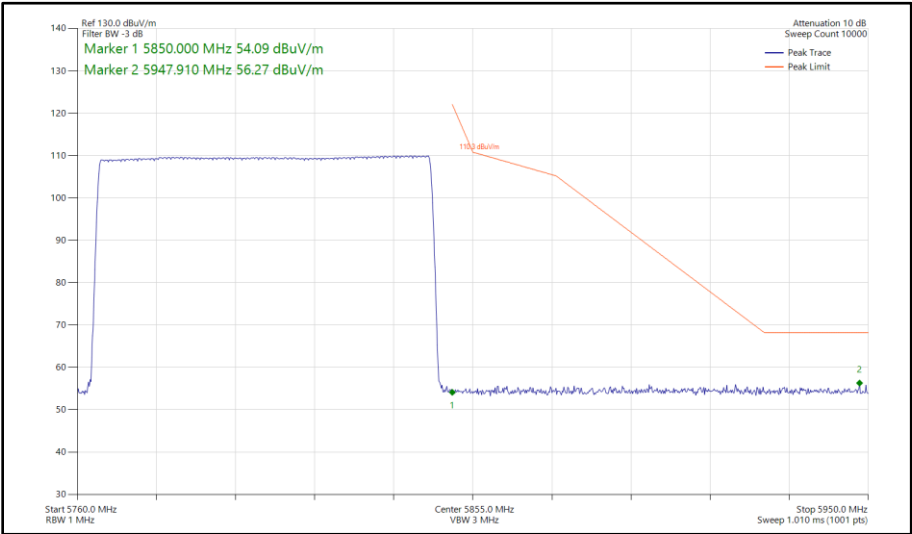
Figure 205 - Narrowband DH5, SISO, Core 1 - 5766-5844 MHz Band Edge Frequency 5850 MHz
