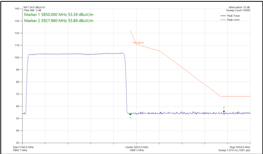
Figure 206 - Narrowband HDR4, SISO, Core 1 - 5766-5844 MHz Band Edge Frequency 5850 MHz
