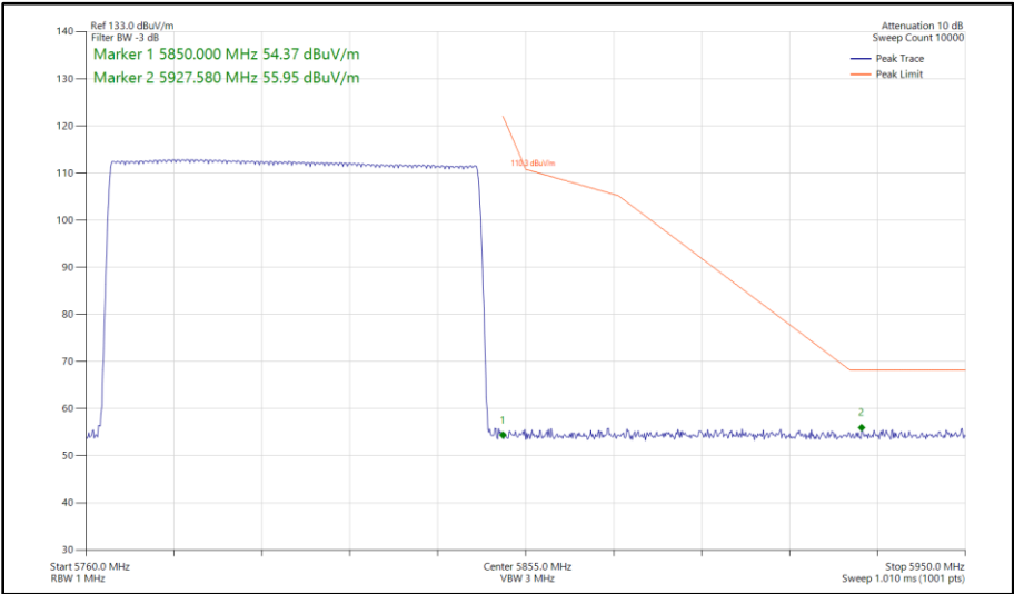
Figure 217 - Narrowband DH5, MIMO, Core 0 - Core 1 - 5766-5844 MHz Band Edge Frequency 5850 MHz
