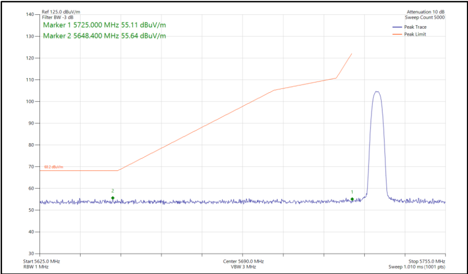
Figure 185 - Narrowband HDR4, SISO, Core 0 - 5733 MHz Band Edge Frequency 5725 MHz
