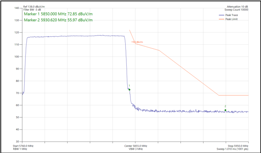
Figure 231 - Narrowband HDR8, SISO, Core 0 - 5766-5844 MHz Band Edge Frequency 5850 MHz
