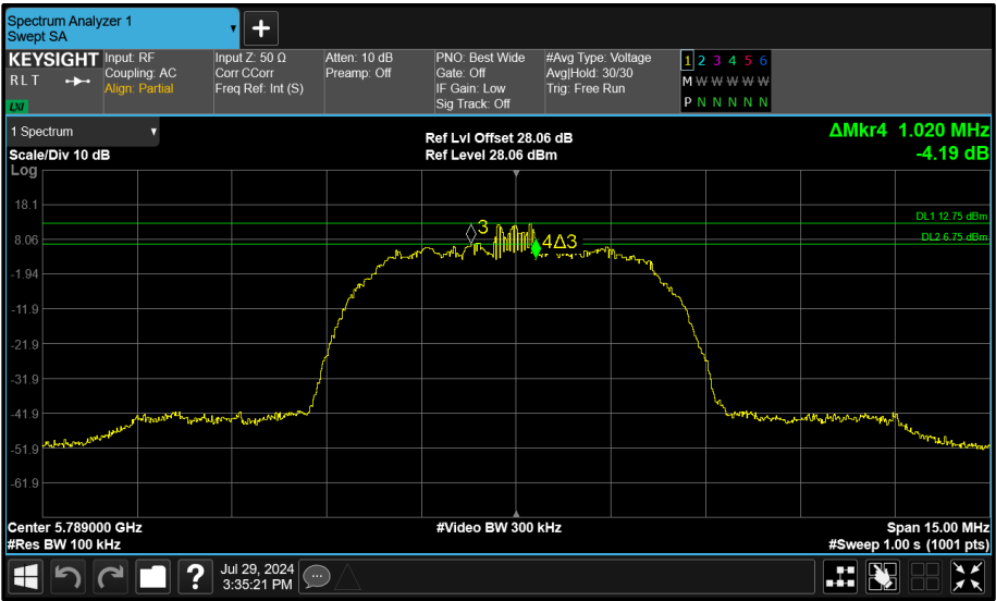
Figure 179 - Core 1 (B) 5789 MHz (CH64) 6 dB Bandwidth
