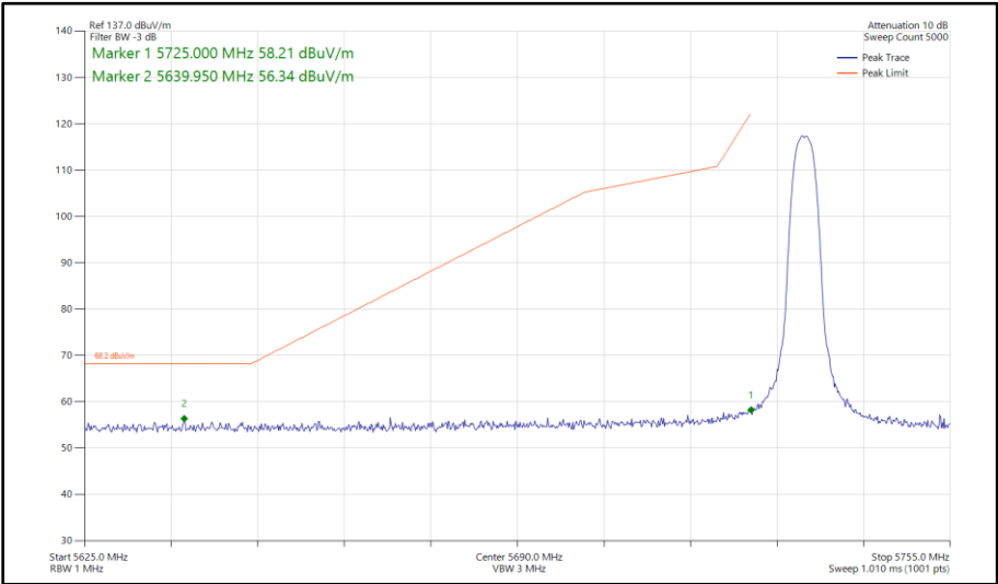
Figure 221 - Narrowband HDR4, SISO, Core 0 - 5733 MHz Band Edge Frequency 5725 MHz
