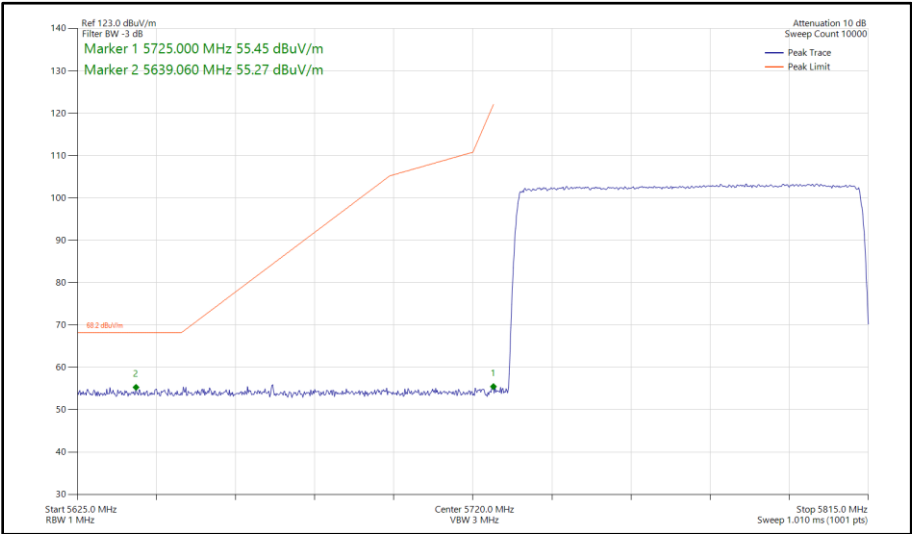
Figure 201 - Narrowband HDR8, SISO, Core 1 - 5733-5811 MHz Band Edge Frequency 5725 MHz
