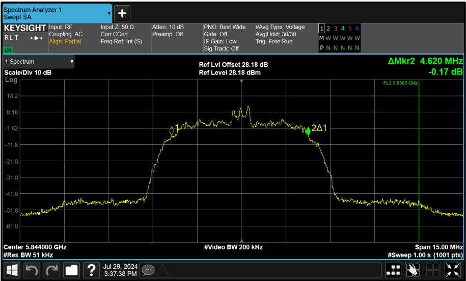
Figure 182 - Core 1 (B) 5844 MHz (CH119) 99% Bandwidth
