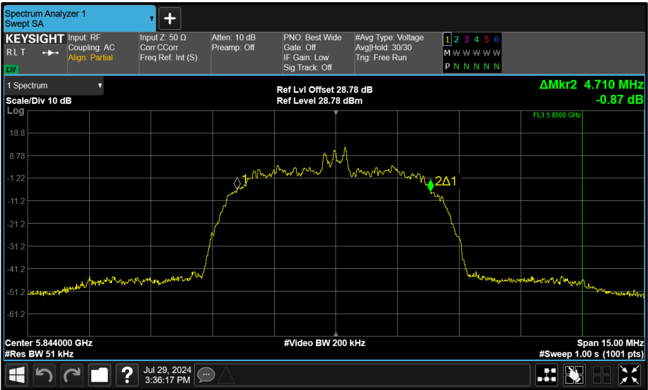
Figure 180 - Core 0 (A) 5844 MHz (CH119) 99% Bandwidth
