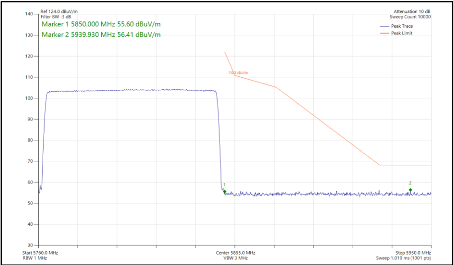
Figure 195 - Narrowband HDR8, SISO, Core 0 - 5766-5844 MHz Band Edge Frequency 5850 MHz
