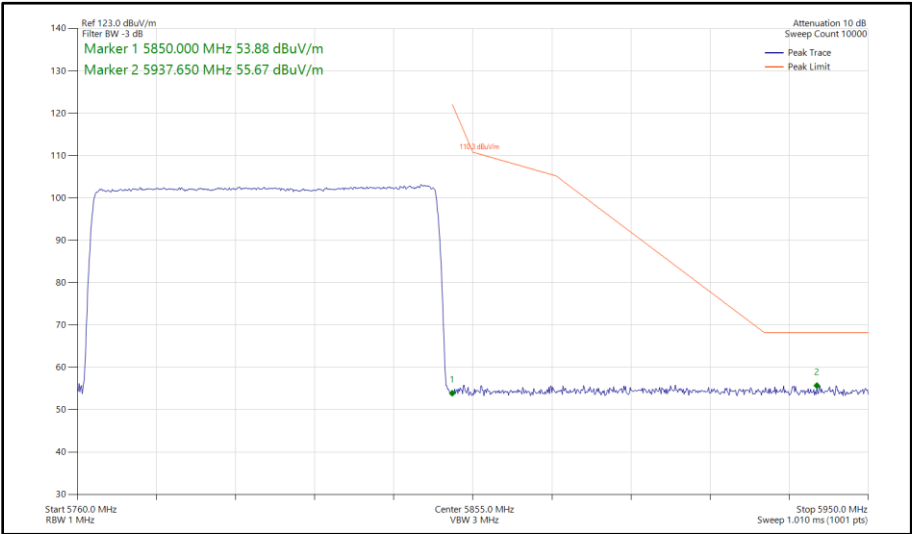
Figure 207 - Narrowband HDR8, SISO, Core 1 - 5766-5844 MHz Band Edge Frequency 5850 MHz
