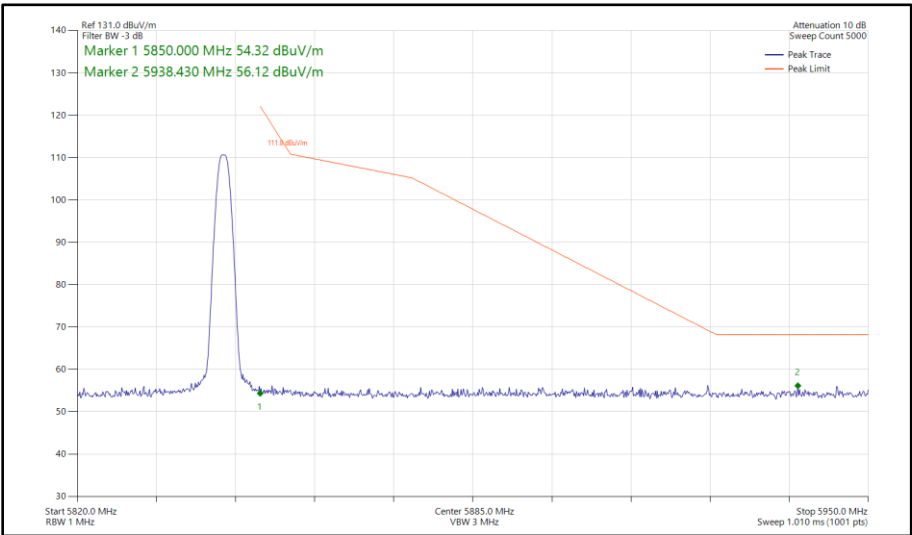
Figure 190 - Narrowband DH5, SISO, Core 0 - 5844 MHz Band Edge Frequency 5850 MHz
