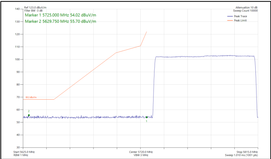
Figure 200 - Narrowband HDR4, SISO, Core 1 - 5733-5811 MHz Band Edge Frequency 5725 MHz
