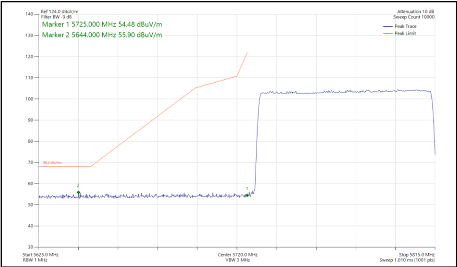
Figure 189 - Narrowband HDR8, SISO, Core 0 - 5733-5811 MHz Band Edge Frequency 5725 MHz
