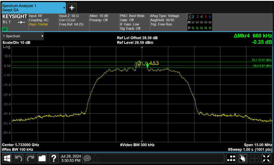
Figure 173 - Core 0 (A) 5733 MHz (CH8) 6 dB Bandwidth
