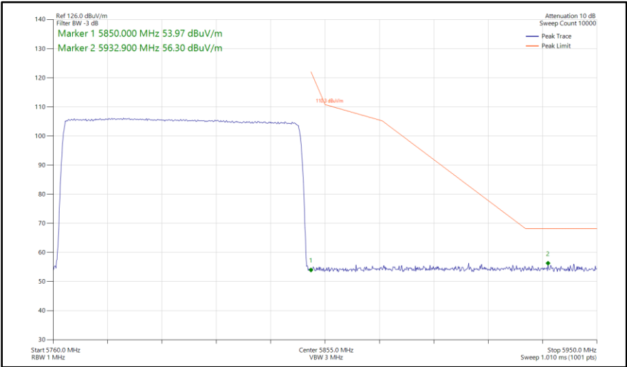
Figure 219 - Narrowband HDR8, MIMO, Core 0 - Core 1 - 5766-5844 MHz Band Edge Frequency 5850 MHz
