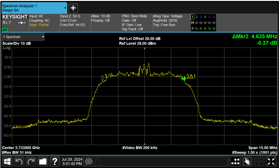
Figure 174 - Core 1 (B) 5733 MHz (CH8) 99% Bandwidth
