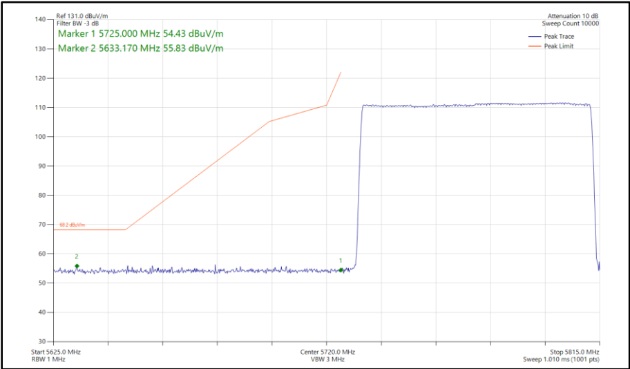
Figure 211 - Narrowband DH5, MIMO, Core 0 - Core 1 - 5733-5811 MHz Band Edge Frequency 5725 MHz
