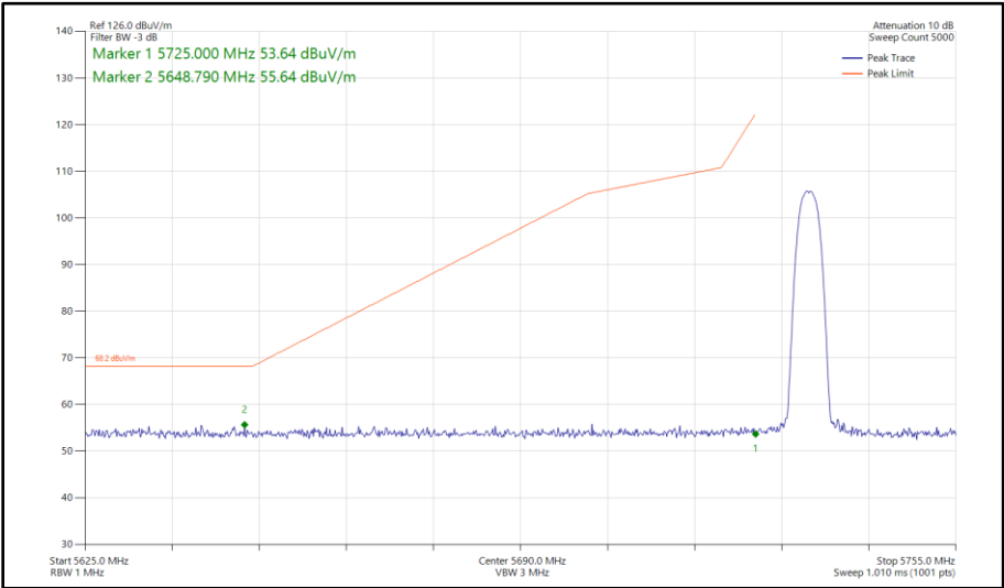
Figure 209 - Narrowband HDR4, MIMO, Core 0 - Core 1 - 5733 MHz Band Edge Frequency 5725 MHz
