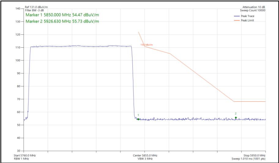
Figure 193 - Narrowband DH5, SISO, Core 0 - 5766-5844 MHz Band Edge Frequency 5850 MHz
