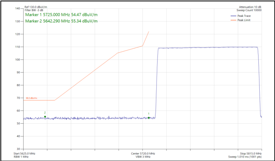
Figure 199 - Narrowband DH5, SISO, Core 1 - 5733-5811 MHz Band Edge Frequency 5725 MHz
