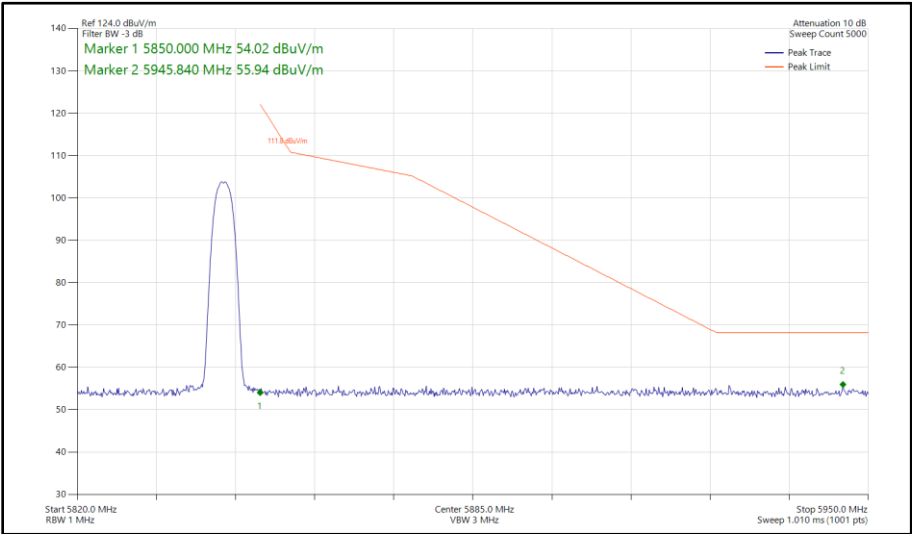
Figure 203 - Narrowband HDR4, SISO, Core 1 - 5844 MHz Band Edge Frequency 5850 MHz
