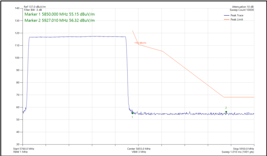
Figure 229 - Narrowband DH5, SISO, Core 0 - 5766-5844 MHz Band Edge Frequency 5850 MHz
