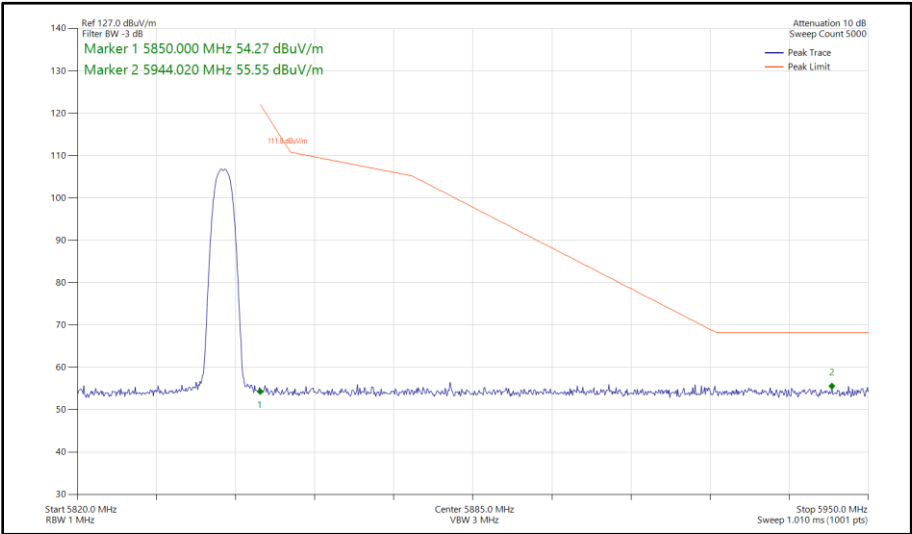
Figure 215 - Narrowband HDR4, MIMO, Core 0 - Core 1 - 5844 MHz Band Edge Frequency 5850 MHz
