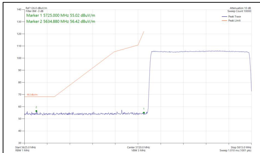
Figure 213 - Narrowband HDR8, MIMO, Core 0 - Core 1 - 5733-5811 MHz Band Edge Frequency 5725 MHz
