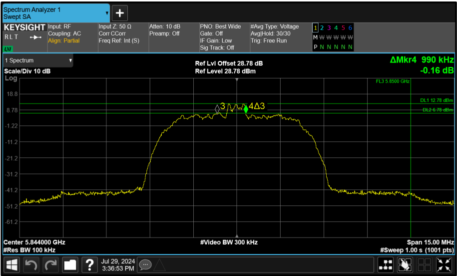
Figure 181 - Core 0 (A) 5844 MHz (CH119) 6 dB Bandwidth
