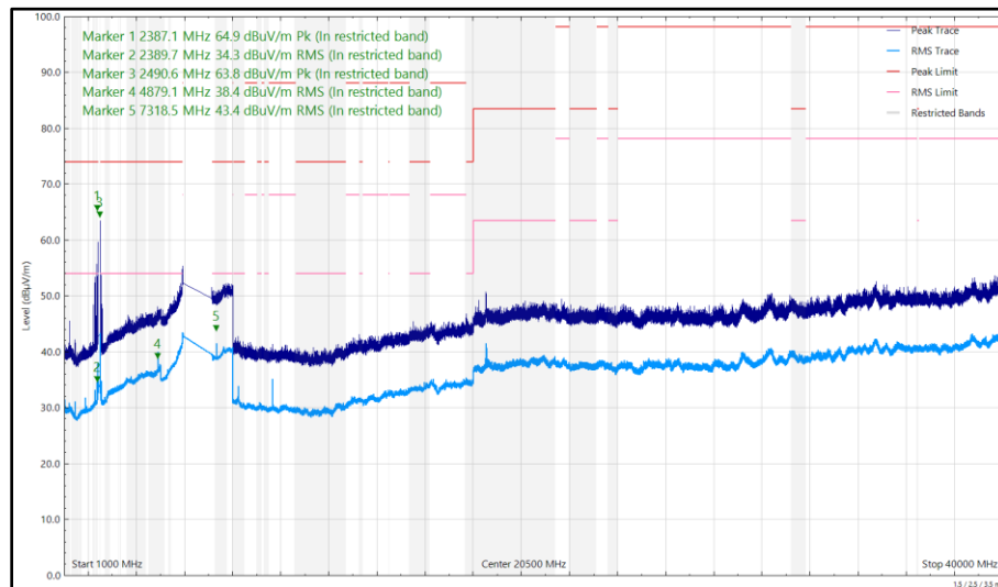
Figure 101 - U-NII-5 - 6175 MHz (CH45), HE20, SU, CDD, Core 0 + Core 1 and 2440 MHz (CH18), Core 1, ePA, 1 GHz to 40 GHz, Vertical
