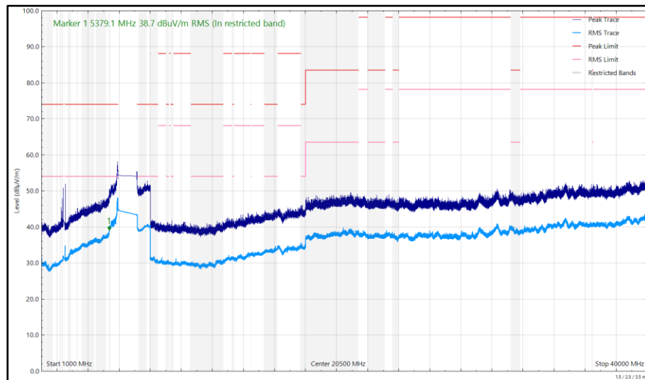
Figure 107 - U-NII-8 - 6995 MHz (CH209), HE20, SU, CDD, Core 0 + Core 1 and 2440 MHz (CH18), Core 1, ePA, 1 GHz to 40 GHz, Horizontal
