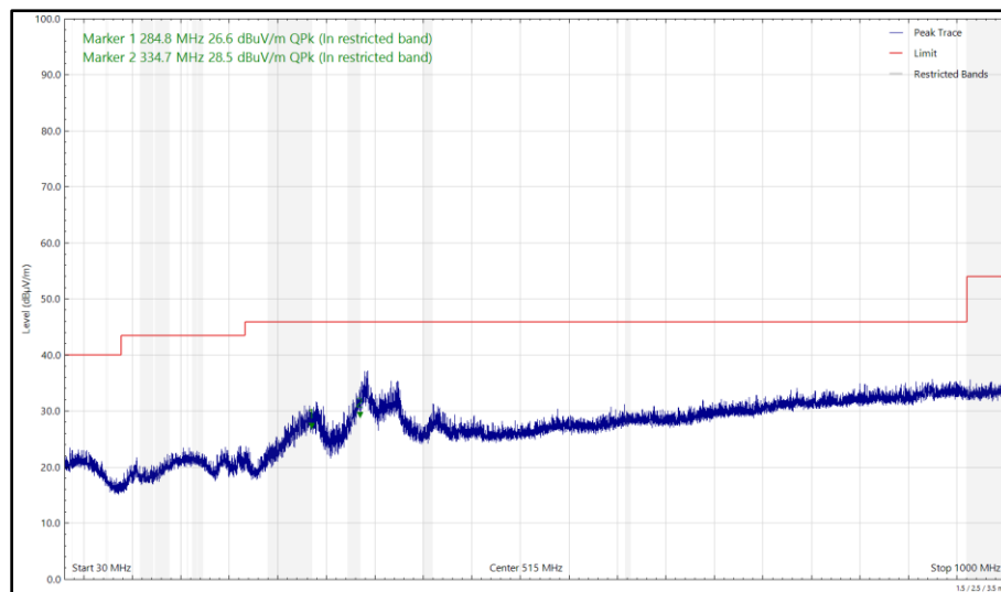
Figure 106 - U-NII-8 - 6995 MHz (CH209), HE20, SU, CDD, Core 0 + Core 1 and 2440 MHz (CH18), Core 1, ePA, 30 MHz to 1 GHz, Horizontal (Peak)
