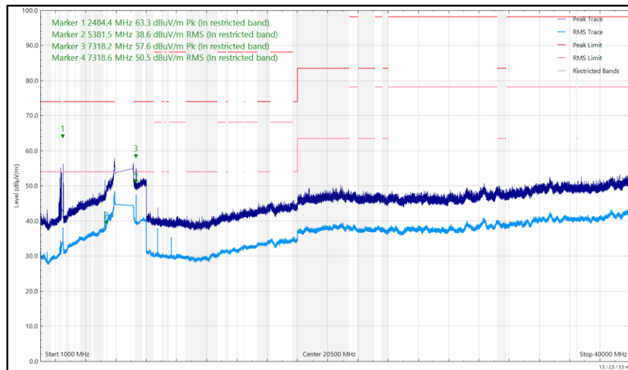
Figure 105 - U-NII-8 - 6995 MHz (CH209), HE20, SU, CDD, Core 0 + Core 1 and 2440 MHz (CH18), Core 0, ePA, 1 GHz to 40 GHz, Vertical
