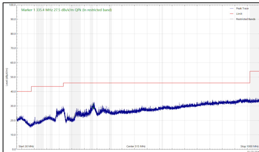
Figure 104 - U-NII-8 - 6995 MHz (CH209), HE20, SU, CDD, Core 0 + Core 1 and 2440 MHz (CH18), Core 0, ePA, 30 MHz to 1 GHz, Vertical (Peak)
