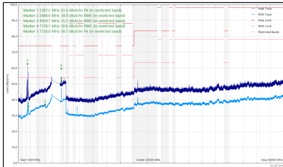
Figure 97 - U-NII-5 - 6175 MHz (CH45), HE20, SU, CDD, Core 0 + Core 1 and 2440 MHz (CH18), Core 0, ePA, 1 GHz to 40 GHz, Vertical
