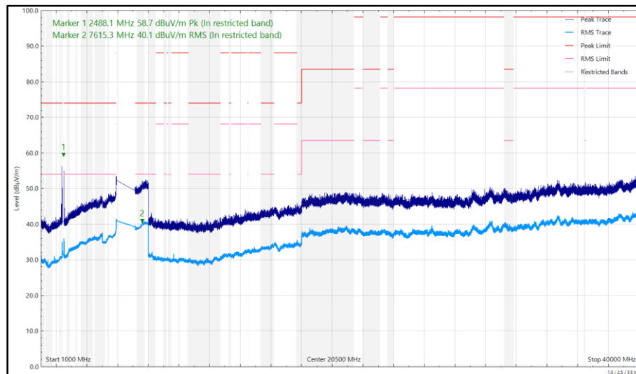
Figure 99 - U-NII-5 - 6175 MHz (CH45), HE20, SU, CDD, Core 0 + Core 1 and 2440 MHz (CH18), Core 1, ePA, 1 GHz to 40 GHz, Horizontal
