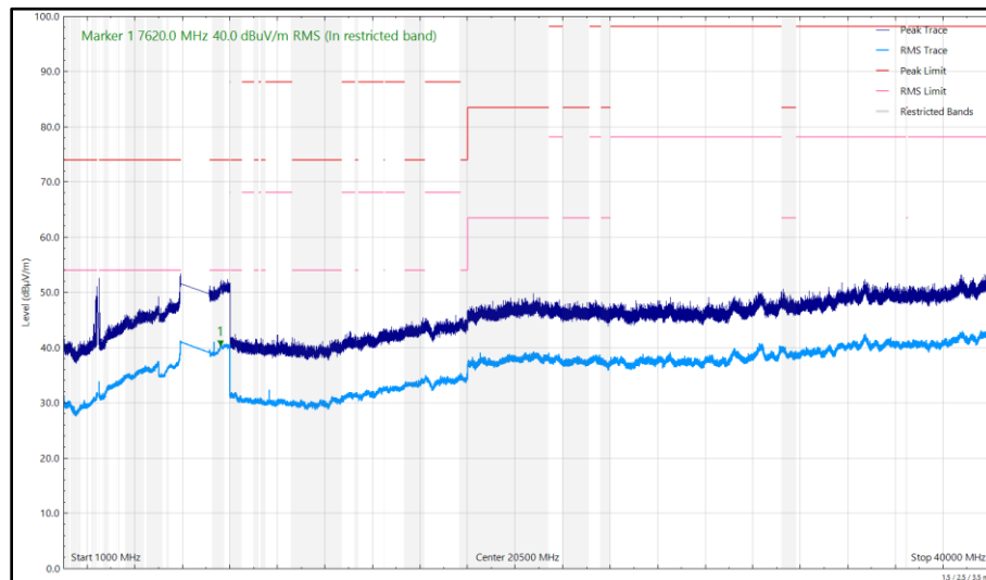
Figure 95 - U-NII-5 - 6175 MHz (CH45), HE20, SU, CDD, Core 0 + Core 1 and 2440 MHz (CH18), Core 0, ePA, 1 GHz to 40 GHz, Horizontal
