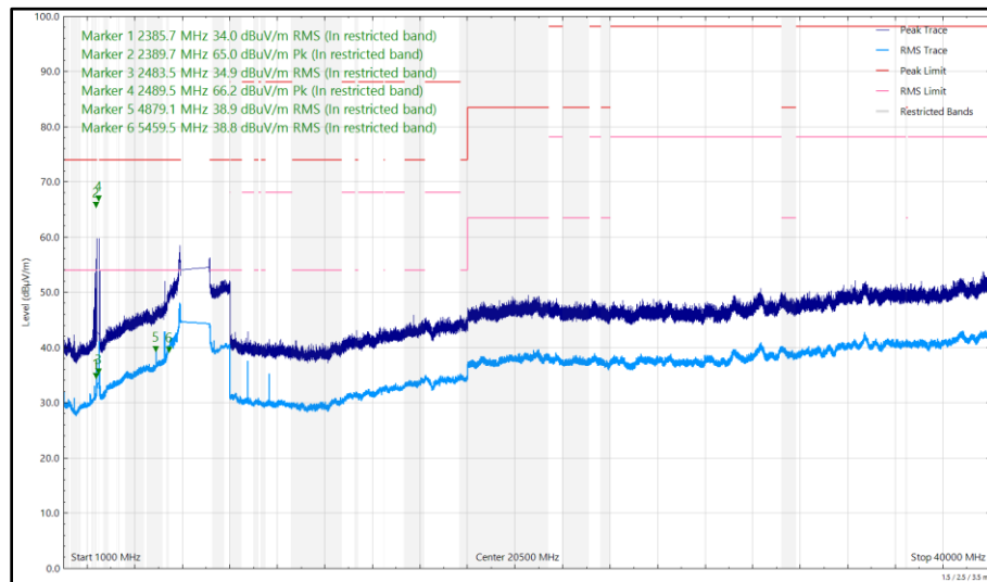
Figure 109 - U-NII-8 - 6995 MHz (CH209), HE20, SU, CDD, Core 0 + Core 1 and 2440 MHz (CH18), Core 1, ePA, 1 GHz to 40 GHz, Vertical
