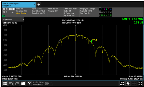
Figure 31 - Core 1 (B) 2440 MHz (CH18) 99% Bandwidth
