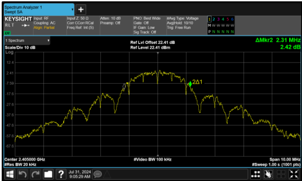
Figure 23 - Core 1 (B) 2405 MHz (CH11) 99% Bandwidth
