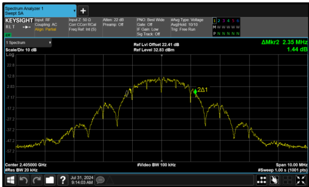
Figure 29 - Core 1 (B) 2405 MHz (CH11) 99% Bandwidth
