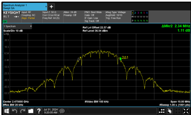
Figure 33 - Core 1 (B) 2475 MHz (CH25) 99% Bandwidth
