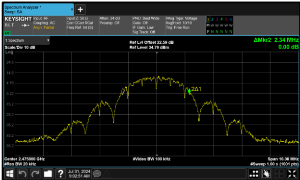
Figure 21 - Core 0 (A) 2475 MHz (CH25) 99% Bandwidth
