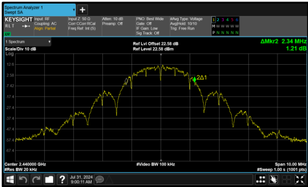
Figure 19 - Core 0 (A) 2440 MHz (CH18) 99% Bandwidth
