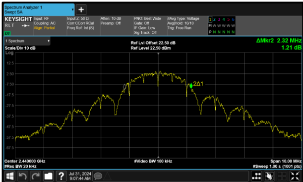
Figure 25 - Core 1 (B) 2440 MHz (CH18) 99% Bandwidth
