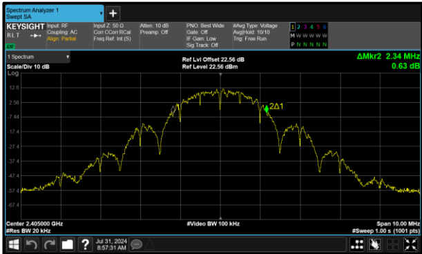
Figure 17 - Core 0 (A) 2405 MHz (CH11) 99% Bandwidth
