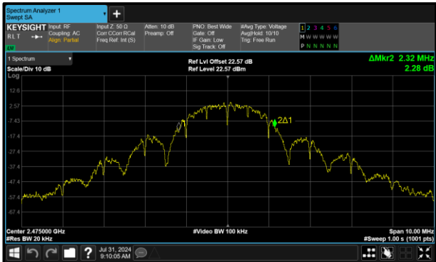
Figure 27 - Core 1 (B) 2475 MHz (CH25) 99% Bandwidth
