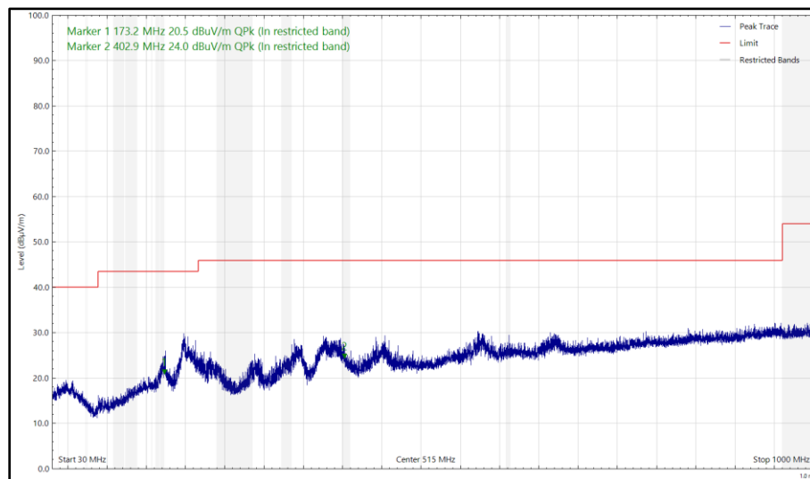
Figure 59 - 2440 MHz (CH18), Thread, Core 1, ePA, 30 MHz to 1 GHz, Vertical (Peak)
