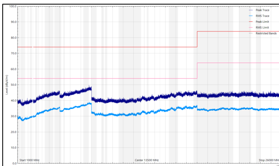
Figure 66 - 2440 MHz (CH18), Thread, iPA, Core 0, 1 GHz to 26 GHz, Horizontal
