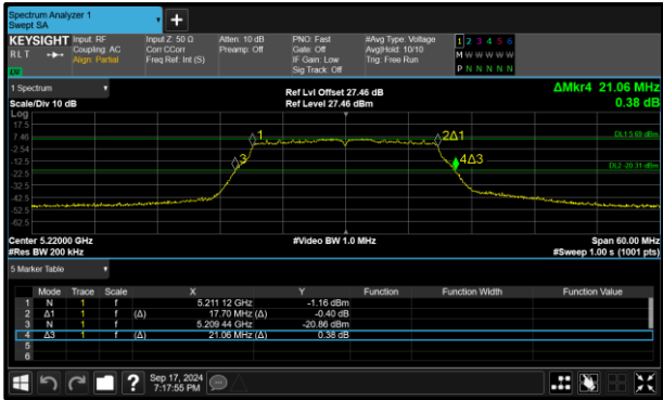
Figure 214 - 802.11n HT20 Minimum 99% OBW
