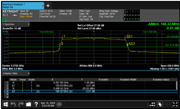
Figure 256 - 802.11ax HE160 SU Minimum 99% OBW
