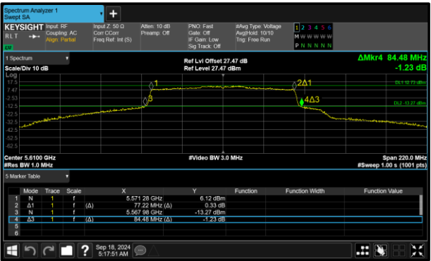
Figure 255 - 802.11ax HE80 SU Maximum 99% OBW
