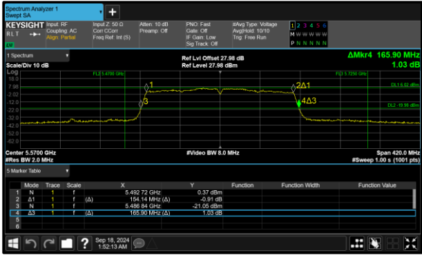
Figure 220 - 802.11ac VHT160 Minimum 99% OBW
