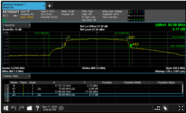
Figure 246 - 802.11ac VHT80 Minimum 99% OBW
