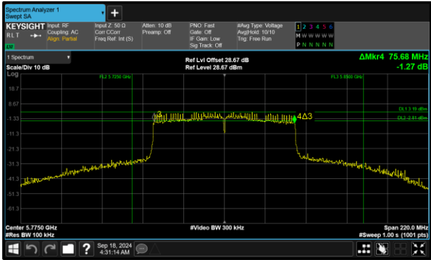
Figure 234 - 802.11ac VHT80 Minimum 6 dB EBW
