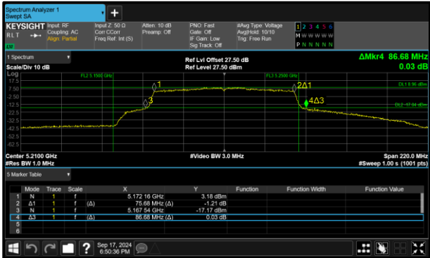
Figure 190 - 802.11ac VHT80 Minimum 99% OBW
