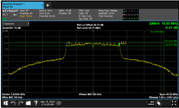
Figure 208 - 802.11ax HE20 SU Minimum 6 dB EBW
