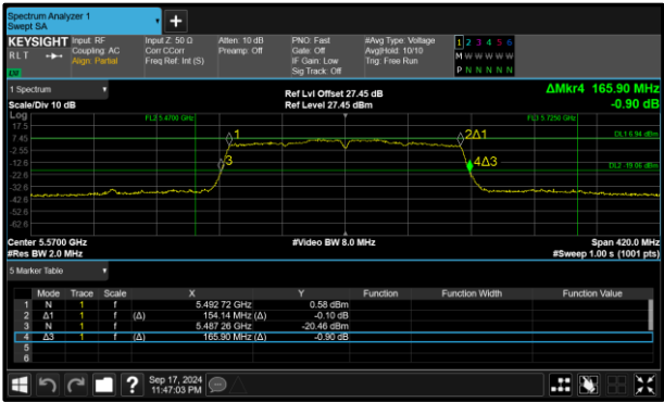
Figure 193 - 802.11ac VHT160 Maximum 99% OBW
