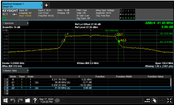
Figure 216 - 802.11n HT40 Minimum 99% OBW
