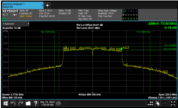
Figure 206 - 802.11ac VHT80 Minimum 6 dB EBW
