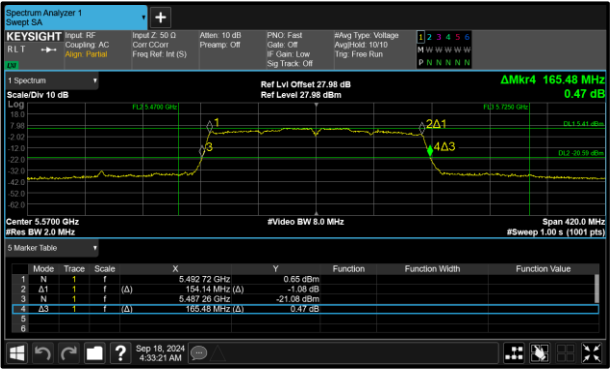
Figure 249 - 802.11ac VHT160 Maximum 99% OBW
