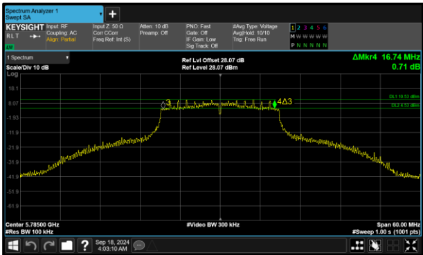
Figure 230 - 802.11n HT20 Minimum 6 dB EBW
