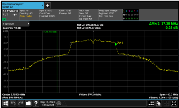
Figure 217 - 802.11n HT40 Maximum 99% OBW
