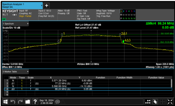
Figure 227 - 802.11ax HE80 SU Maximum 99% OBW
