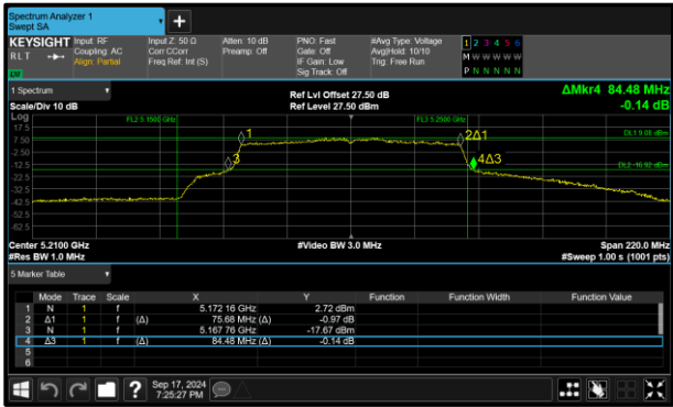
Figure 218 - 802.11ac VHT80 Minimum 99% OBW
