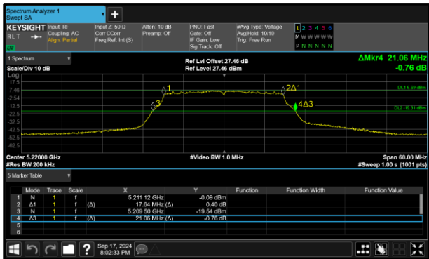
Figure 242 - 802.11n HT20 Minimum 99% OBW
