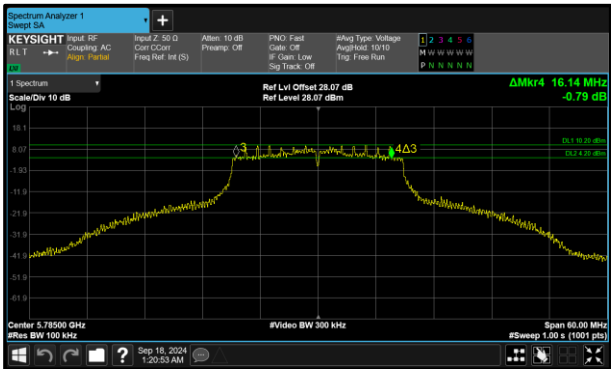
Figure 202 - 802.11n HT20 Minimum 6 dB EBW
