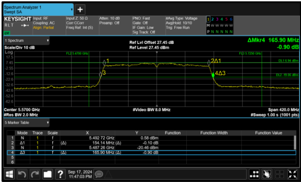
Figure 192 - 802.11ac VHT160 Minimum 99% OBW
