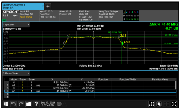
Figure 244 - 802.11n HT40 Minimum 99% OBW
