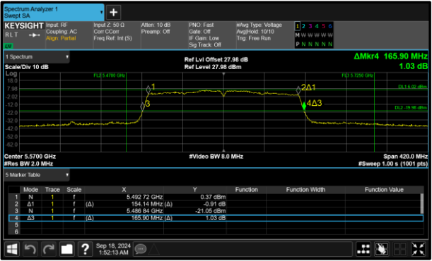
Figure 221 - 802.11ac VHT160 Maximum 99% OBW
