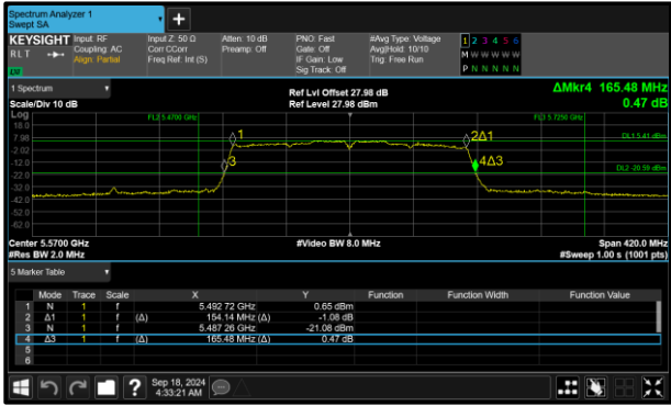
Figure 248 - 802.11ac VHT160 Minimum 99% OBW
