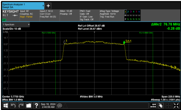
Figure 226 - 802.11ax HE80 SU Minimum 99% OBW
