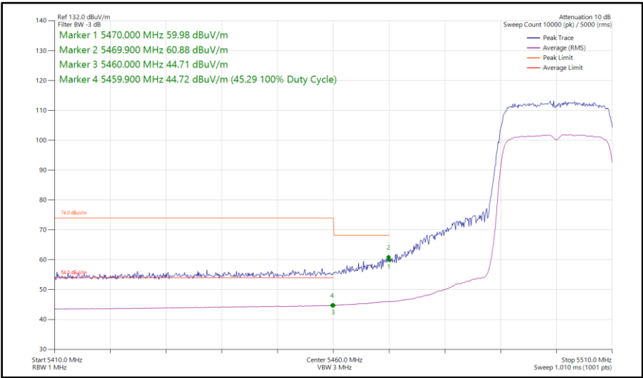
Figure 292 - 802.11ax HE20, SU, SISO, Core 1 - 5500 MHz Band Edge Frequency 5470 MHz
