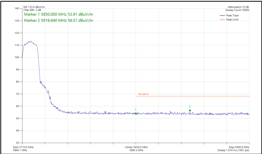
Figure 304 - 802.11n HT20, SISO, Core 1 - 5720 MHz Band Edge Frequency 5850 MHz
