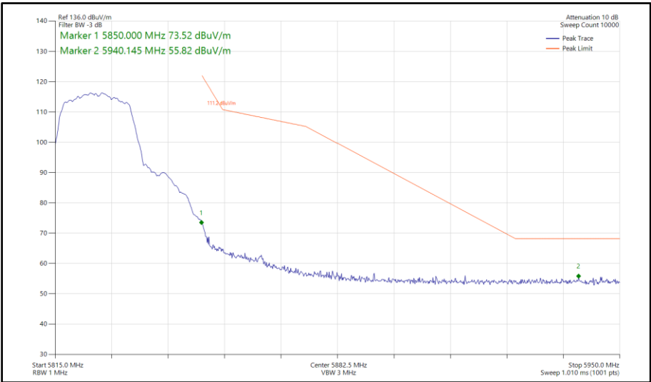
Figure 283 - 802.11a, SISO, Core 0 - 5825 MHz Band Edge Frequency 5850 MHz
