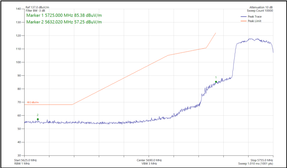
Figure 276 - 802.11ax HE20, SU, SISO, Core 0 - 5745 MHz Band Edge Frequency 5725 MHz
