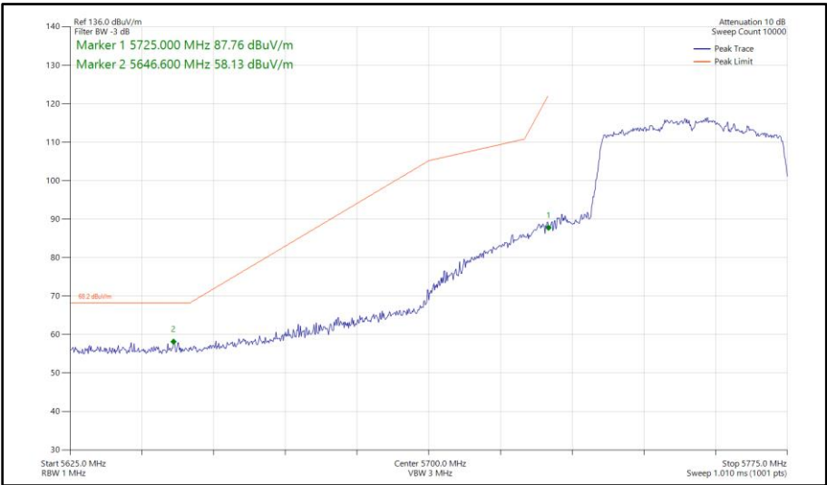
Figure 350 - 802.11ax HE40, SU, SISO, Core 0 - 5755 MHz Band Edge Frequency 5725 MHz
