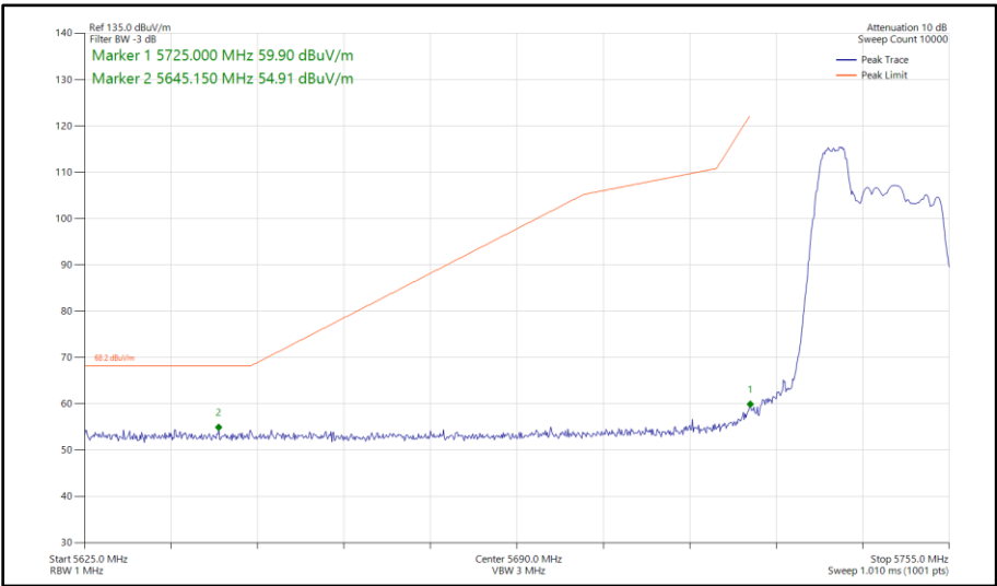
Figure 297 - 802.11ax HE20, RU 52-37, SISO, Core 1 - 5745 MHz Band Edge Frequency 5725 MHz
