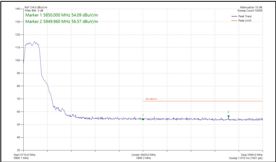
Figure 302 - 802.11a, SISO, Core 1 - 5720 MHz Band Edge Frequency 5850 MHz
