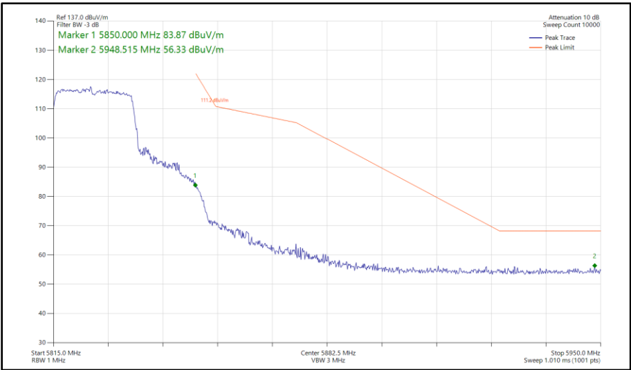
Figure 288 - 802.11ax HE20, SU, SISO, Core 0 - 5825 MHz Band Edge Frequency 5850 MHz
