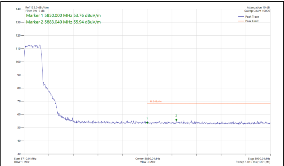
Figure 337 - 802.11ax HE20, SU, SDM, Core 0-1 - 5720 MHz Band Edge Frequency 5850 MHz
