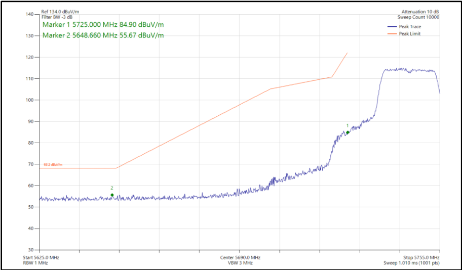
Figure 295 - 802.11n HT20, SISO, Core 1 - 5745 MHz Band Edge Frequency 5725 MHz
