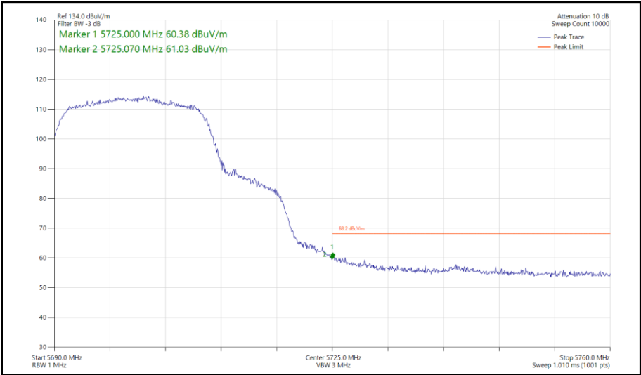
Figure 299 - 802.11n HT20, SISO, Core 1 - 5700 MHz Band Edge Frequency 5725 MHz
