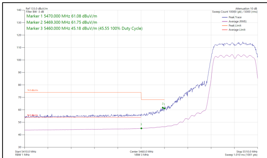
Figure 310 - 802.11n HT20, CDD, Core 0-1 - 5500 MHz Band Edge Frequency 5470 MHz
