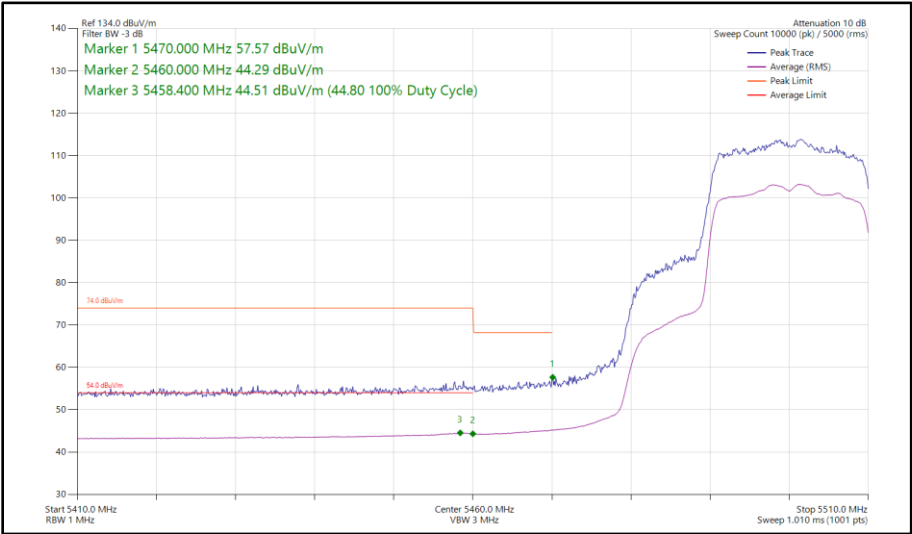
Figure 326 - 802.11ax HE20, SU, SDM, Core 0-1 - 5500 MHz Band Edge Frequency 5470 MHz
