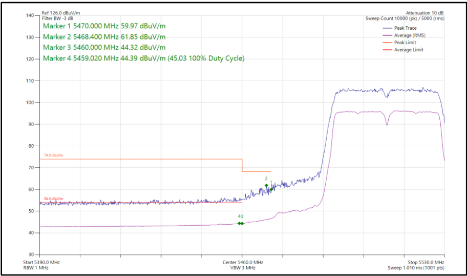
Figure 346 - 802.11n HT40, SISO, Core 0 - 5510 MHz Band Edge Frequency 5470 MHz
