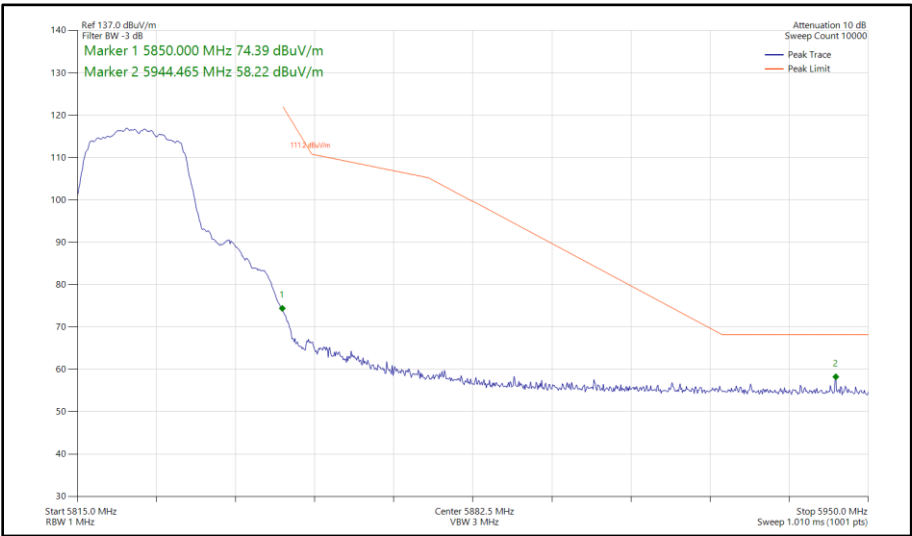
Figure 303 - 802.11a, SISO, Core 1 - 5825 MHz Band Edge Frequency 5850 MHz
