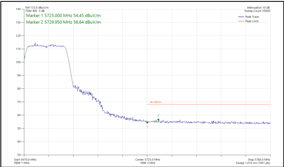
Figure 331 - 802.11n HT20, SDM, Core 0-1 - 5680 MHz Band Edge Frequency 5725 MHz
