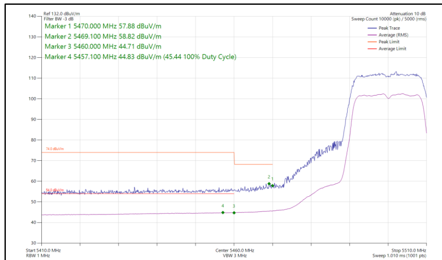
Figure 325 - 802.11n HT20, SDM, Core 0-1 - 5500 MHz Band Edge Frequency 5470 MHz
