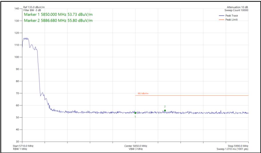
Figure 307 - 802.11ax HE20, RU 106-53, SISO, Core 1 - 5720 MHz Band Edge Frequency 5850 MHz
