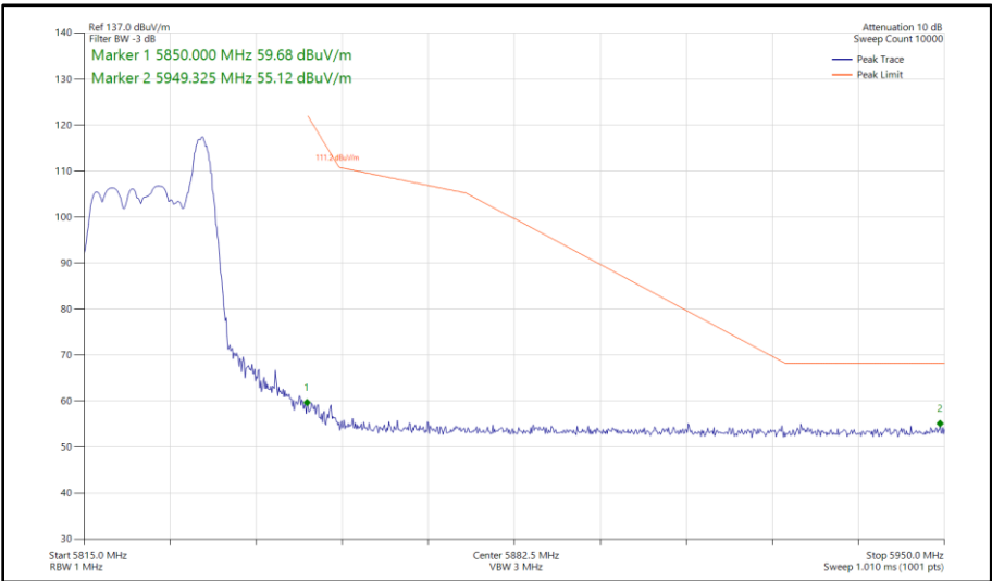
Figure 289 - 802.11ax HE20, RU 26-8, SISO, Core 0 - 5825 MHz Band Edge Frequency 5850 MHz
