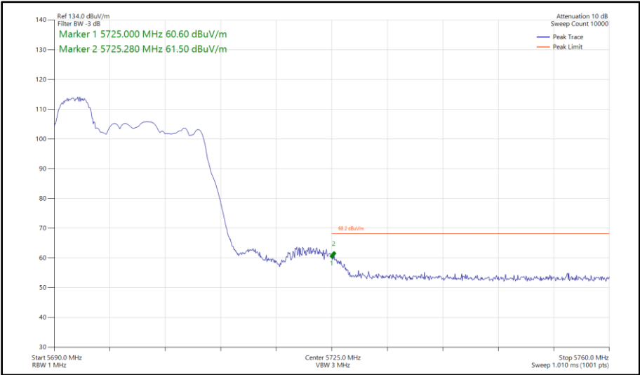
Figure 301 - 802.11ax HE20, RU 52-37, SISO, Core 1 - 5700 MHz Band Edge Frequency 5725 MHz
