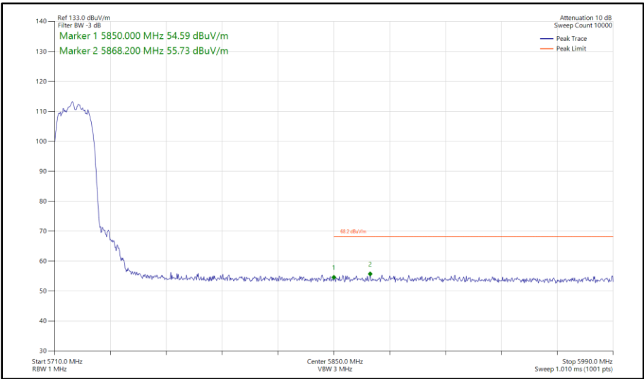
Figure 319 - 802.11n HT20, CDD, Core 0-1 - 5720 MHz Band Edge Frequency 5850 MHz
