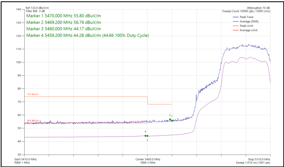
Figure 341 - 802.11ac VHT20, TxBF, Core 0-1 - 5500 MHz Band Edge Frequency 5470 MHz
