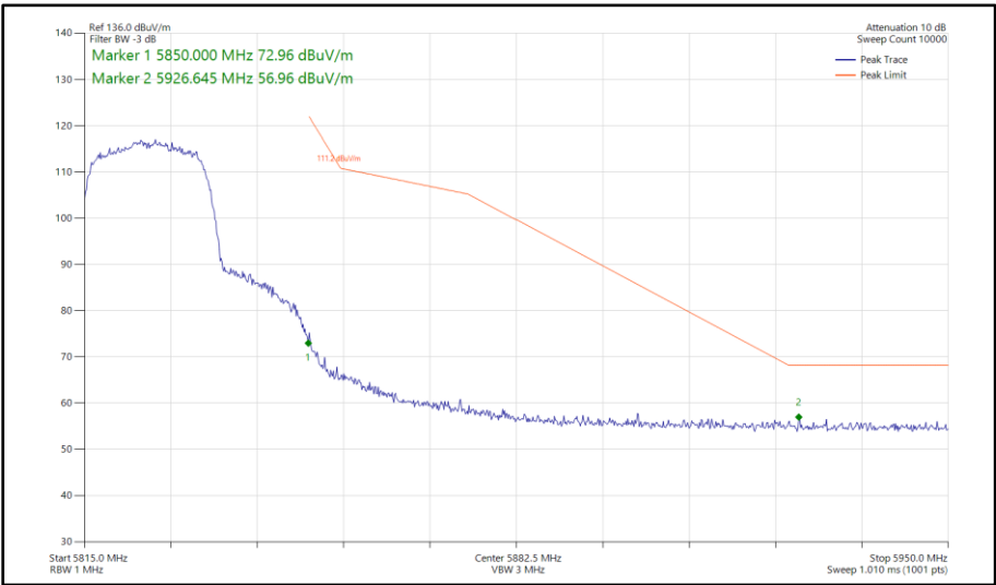
Figure 305 - 802.11n HT20, SISO, Core 1 - 5825 MHz Band Edge Frequency 5850 MHz
