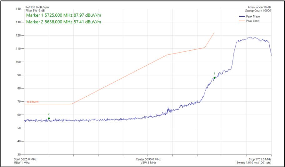
Figure 328 - 802.11n HT20, SDM, Core 0-1 - 5745 MHz Band Edge Frequency 5725 MHz
