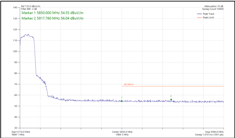
Figure 306 - 802.11ax HE20, SU, SISO, Core 1 - 5720 MHz Band Edge Frequency 5850 MHz
