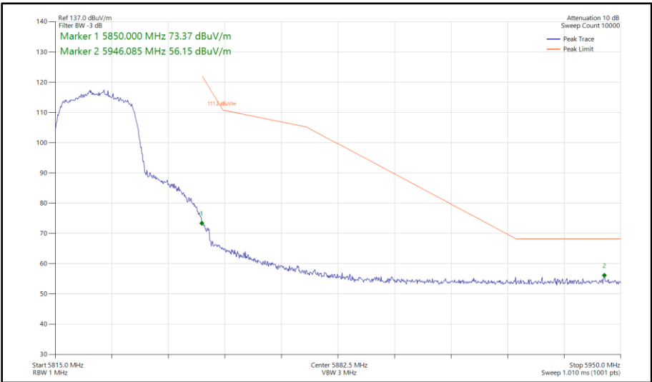
Figure 285 - 802.11n HT20, SISO, Core 0 - 5825 MHz Band Edge Frequency 5850 MHz
