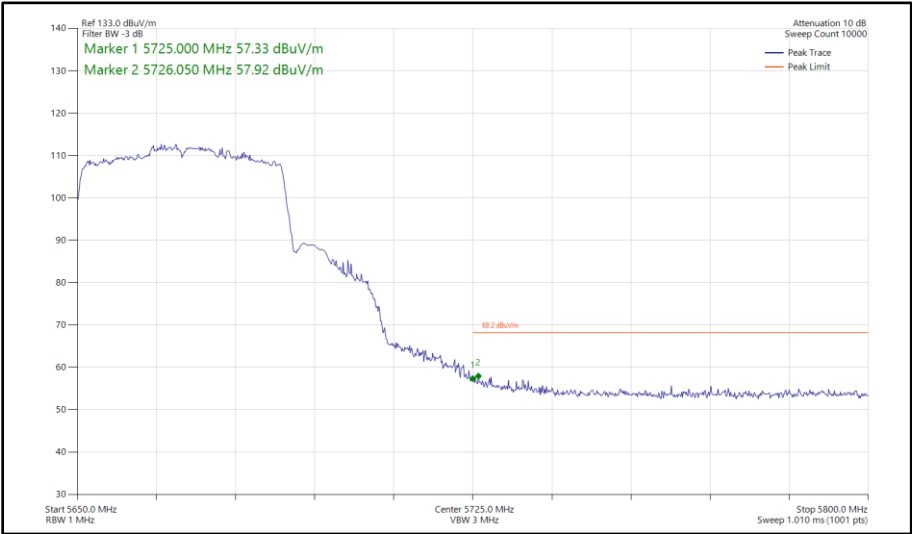
Figure 353 - 802.11ax HE40, SU, SISO, Core 0 - 5670 MHz Band Edge Frequency 5725 MHz
