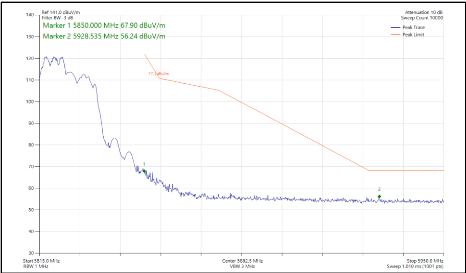
Figure 324 - 802.11ax HE20, RU 106-53, CDD, Core 0-1 - 5825 MHz Band Edge Frequency 5850 MHz
