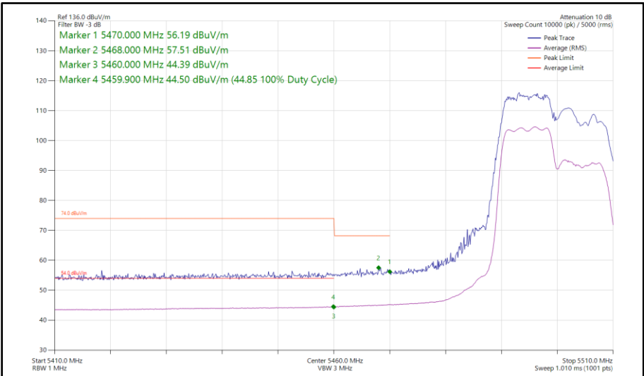
Figure 312 - 802.11ax HE20, RU 106-53, CDD, Core 0-1 - 5500 MHz Band Edge Frequency 5470 MHz
