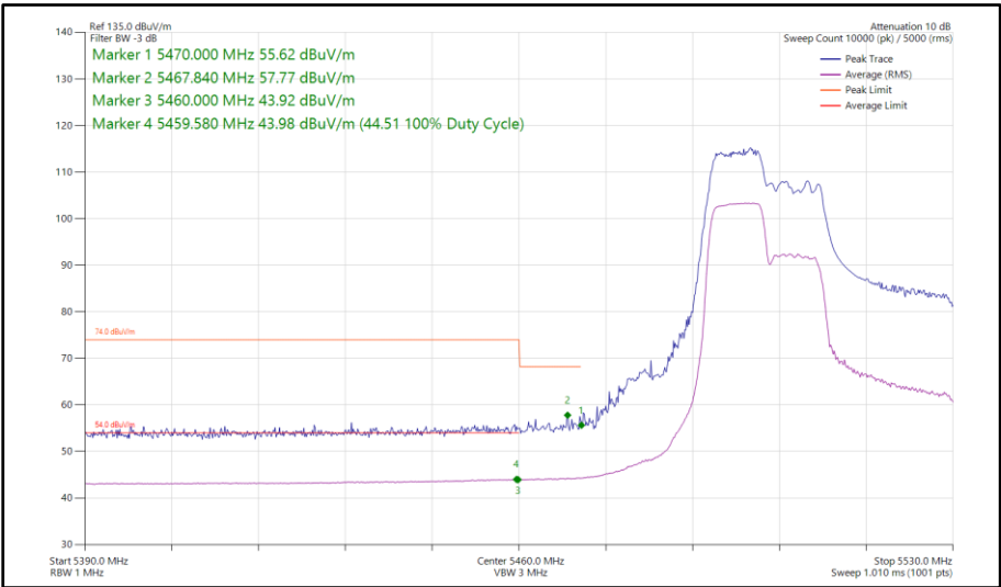
Figure 348 - 802.11ax HE40, RU 106-53, SISO, Core 0 - 5510 MHz Band Edge Frequency 5470 MHz
