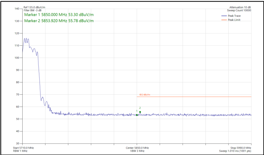
Figure 338 - 802.11ax HE20, RU 106-53, SDM, Core 0-1 - 5720 MHz Band Edge Frequency 5850 MHz
