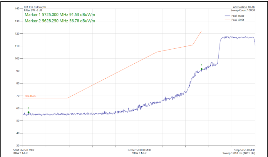
Figure 329 - 802.11ax HE20, SU, SDM, Core 0-1 - 5745 MHz Band Edge Frequency 5725 MHz
