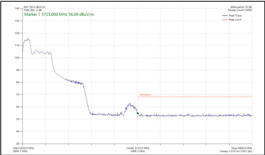
Figure 354 - 802.11ax HE40, RU 52-37, SISO, Core 0 - 5670 MHz Band Edge Frequency 5725 MHz
