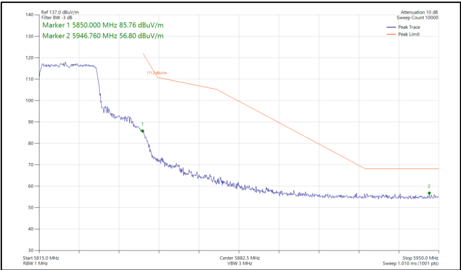
Figure 308 - 802.11ax HE20, SU, SISO, Core 1 - 5825 MHz Band Edge Frequency 5850 MHz
