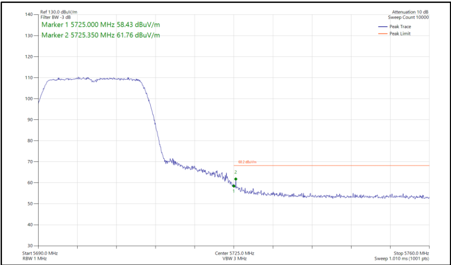
Figure 279 - 802.11n HT20, SISO, Core 0 - 5700 MHz Band Edge Frequency 5725 MHz
