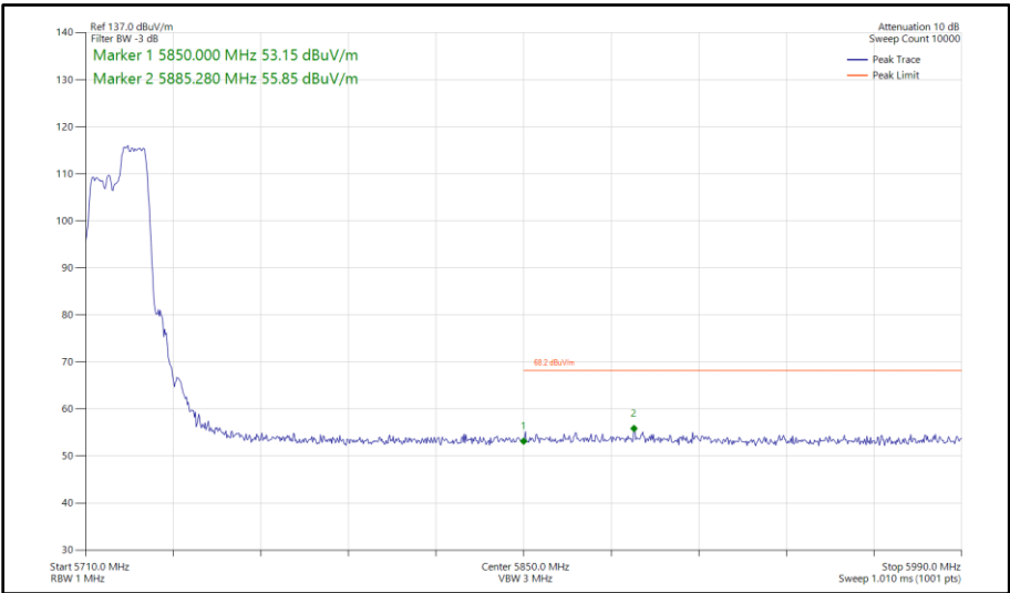
Figure 287 - 802.11ax HE20, RU 106-54, SISO, Core 0 - 5720 MHz Band Edge Frequency 5850 MHz
