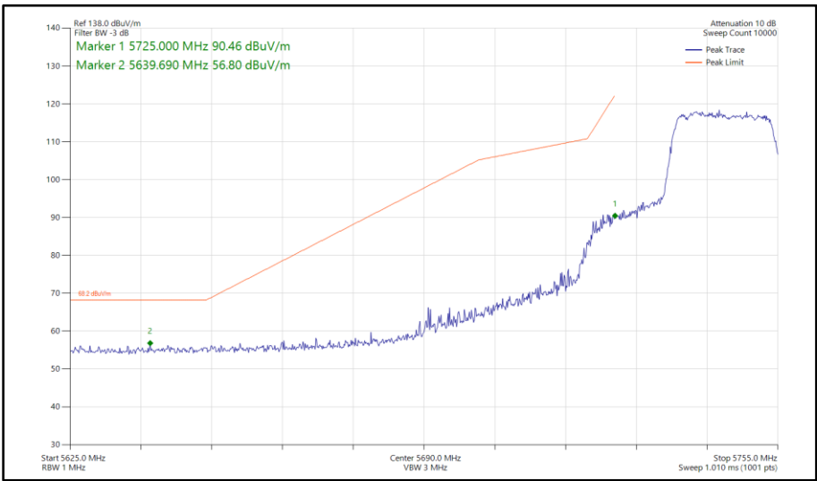
Figure 342 - 802.11ac VHT20, TxBF, Core 0-1 - 5745 MHz Band Edge Frequency 5725 MHz
