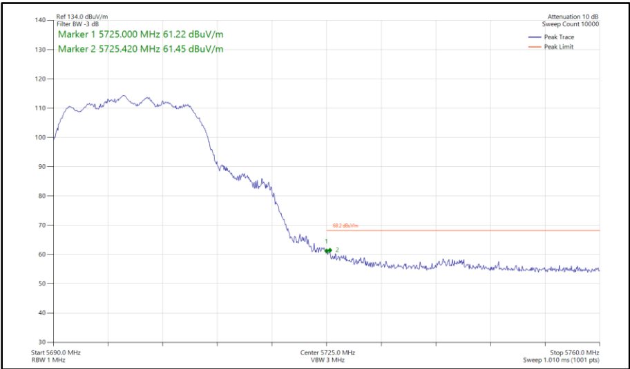
Figure 316 - 802.11n HT20, CDD, Core 0-1 - 5700 MHz Band Edge Frequency 5725 MHz
