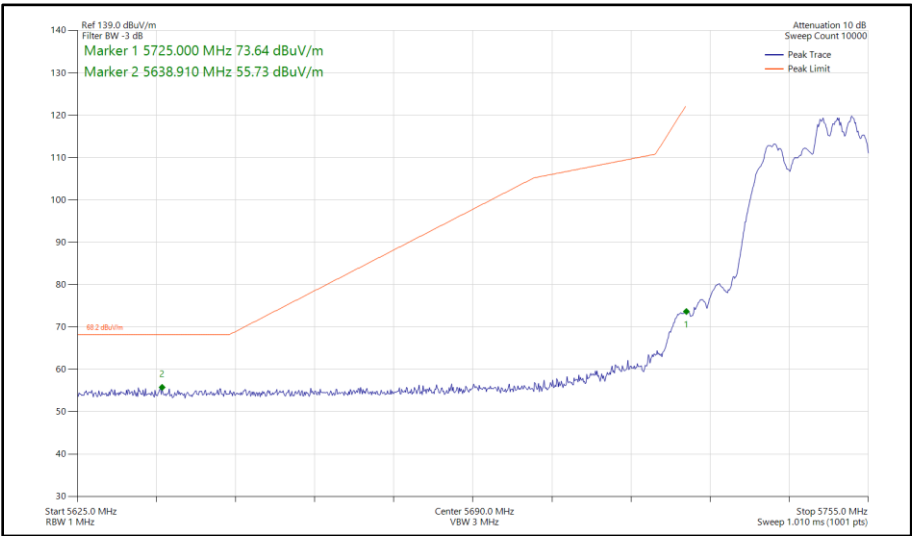
Figure 330 - 802.11ax HE20, RU 106-54, SDM, Core 0-1 - 5745 MHz Band Edge Frequency 5725 MHz
