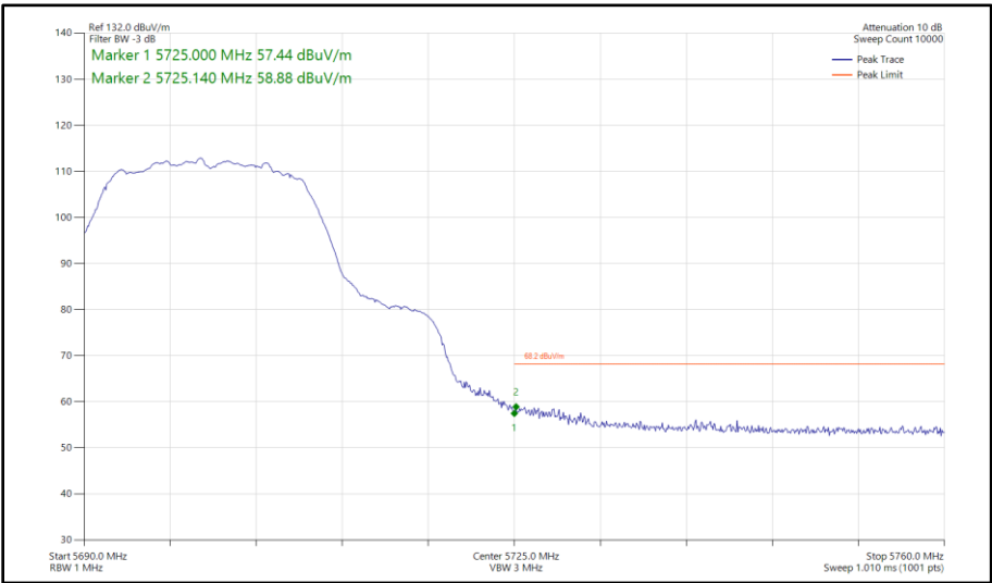
Figure 278 - 802.11a, SISO, Core 0 - 5700 MHz Band Edge Frequency 5725 MHz
