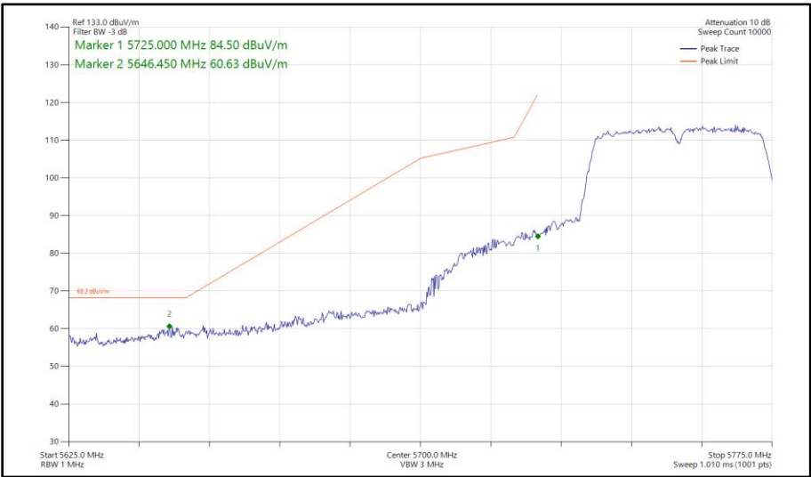
Figure 349 - 802.11n HT40, SISO, Core 0 - 5755 MHz Band Edge Frequency 5725 MHz
