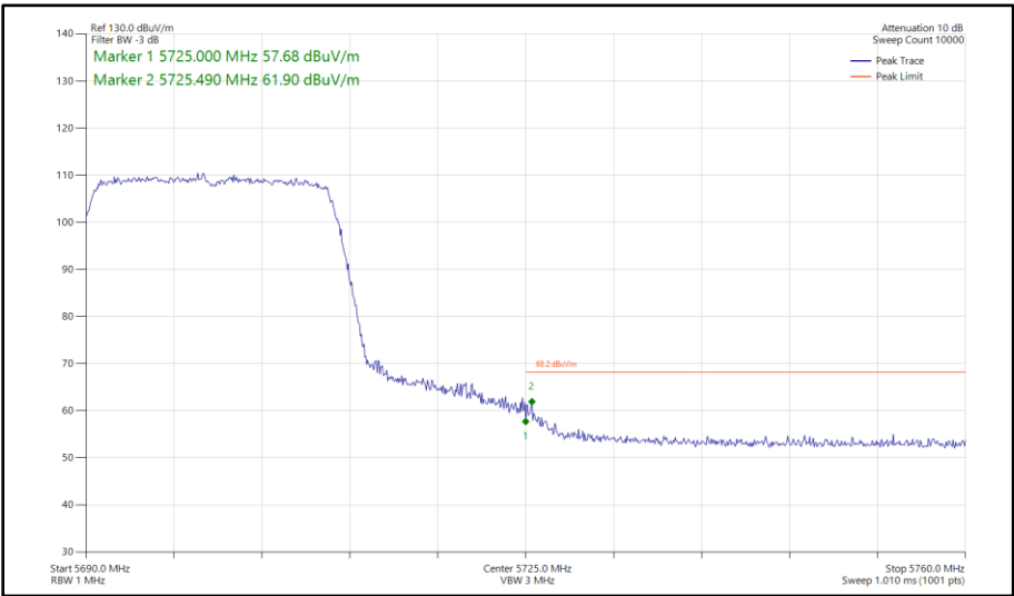
Figure 280 - 802.11ax HE20, SU, SISO, Core 0 - 5700 MHz Band Edge Frequency 5725 MHz
