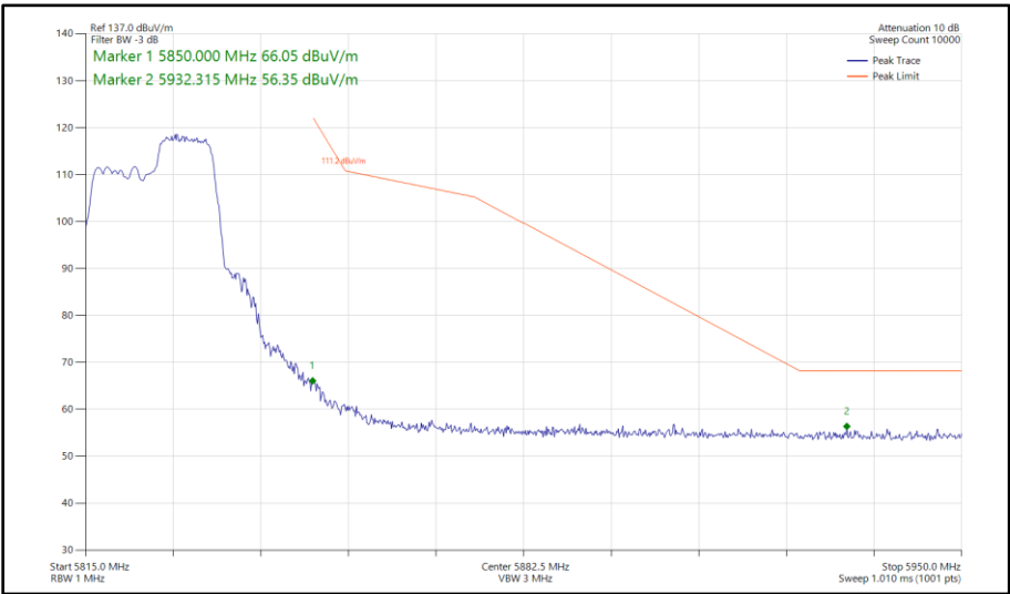
Figure 309 - 802.11ax HE20, RU 106-54, SISO, Core 1 - 5825 MHz Band Edge Frequency 5850 MHz
