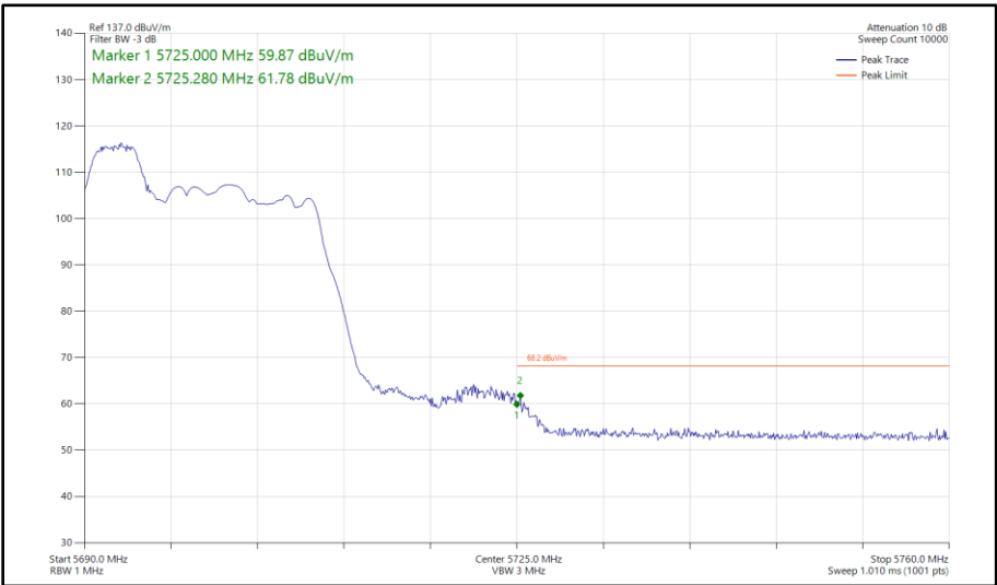
Figure 281 - 802.11ax HE20, RU 52-37, SISO, Core 0 - 5700 MHz Band Edge Frequency 5725 MHz
