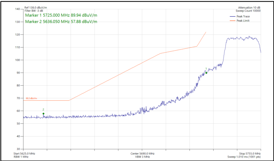
Figure 313 - 802.11n HT20, CDD, Core 0-1 - 5745 MHz Band Edge Frequency 5725 MHz
