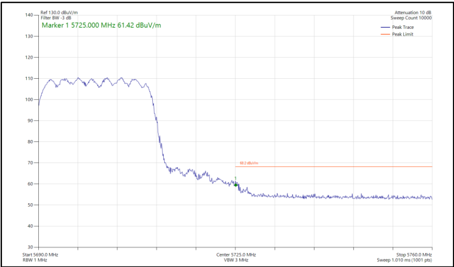
Figure 317 - 802.11ax HE20, SU, CDD, Core 0-1 - 5700 MHz Band Edge Frequency 5725 MHz
