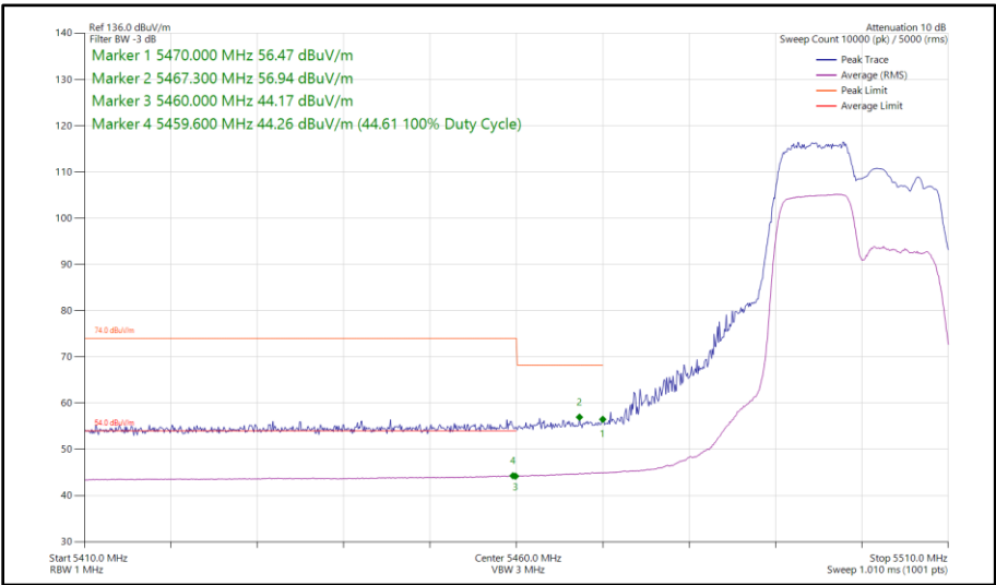
Figure 293 - 802.11ax HE20, RU 106-53, SISO, Core 1 - 5500 MHz Band Edge Frequency 5470 MHz
