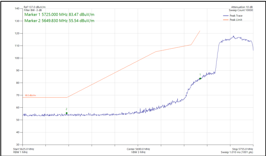
Figure 296 - 802.11ax HE20, SU, SISO, Core 1 - 5745 MHz Band Edge Frequency 5725 MHz
