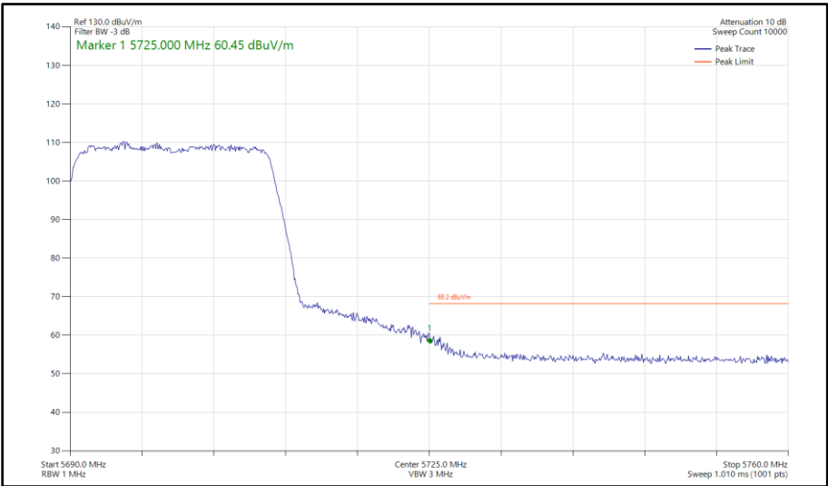
Figure 333 - 802.11ax HE20, SU, SDM, Core 0-1 - 5700 MHz Band Edge Frequency 5725 MHz
