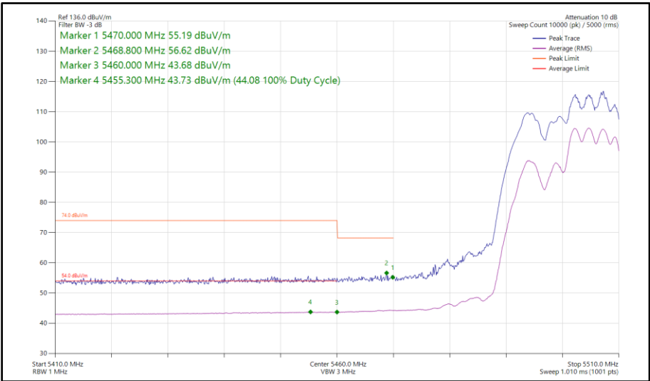
Figure 327 - 802.11ax HE20, RU 106-54, SDM, Core 0-1 - 5500 MHz Band Edge Frequency 5470 MHz
