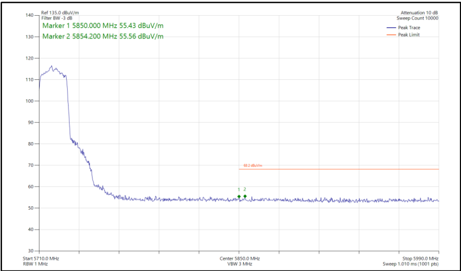
Figure 286 - 802.11ax HE20, SU, SISO, Core 0 - 5720 MHz Band Edge Frequency 5850 MHz
