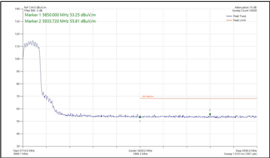
Figure 321 - 802.11ax HE20, SU, CDD, Core 0-1 - 5720 MHz Band Edge Frequency 5850 MHz
