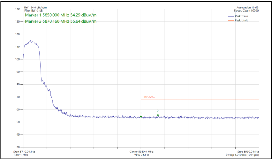
Figure 284 - 802.11n HT20, SISO, Core 0 - 5720 MHz Band Edge Frequency 5850 MHz
