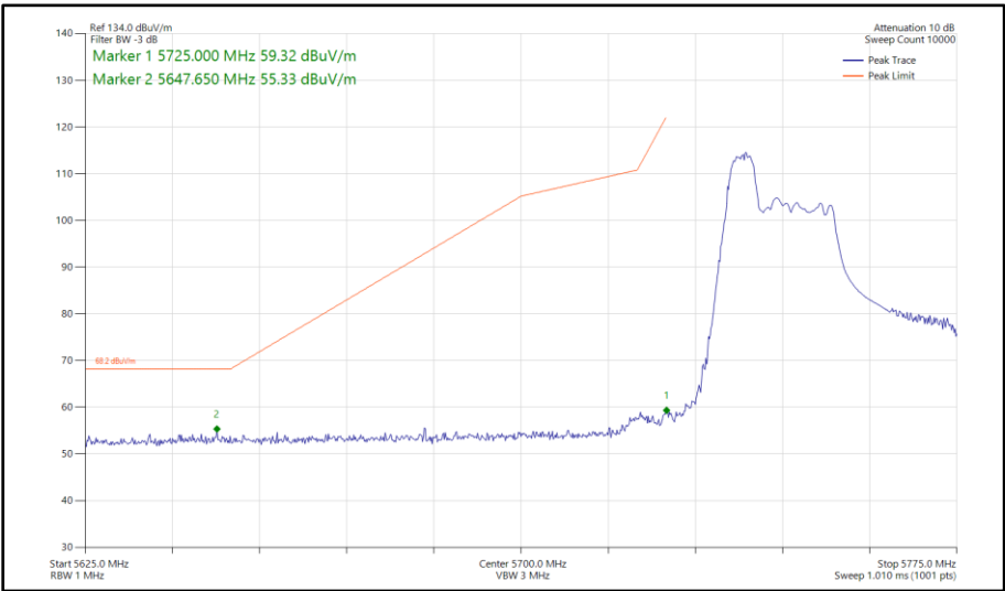
Figure 351 - 802.11ax HE40, RU 52-37, SISO, Core 0 - 5755 MHz Band Edge Frequency 5725 MHz
