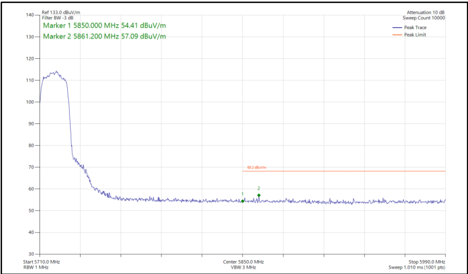
Figure 335 - 802.11n HT20, SDM, Core 0-1 - 5720 MHz Band Edge Frequency 5850 MHz
