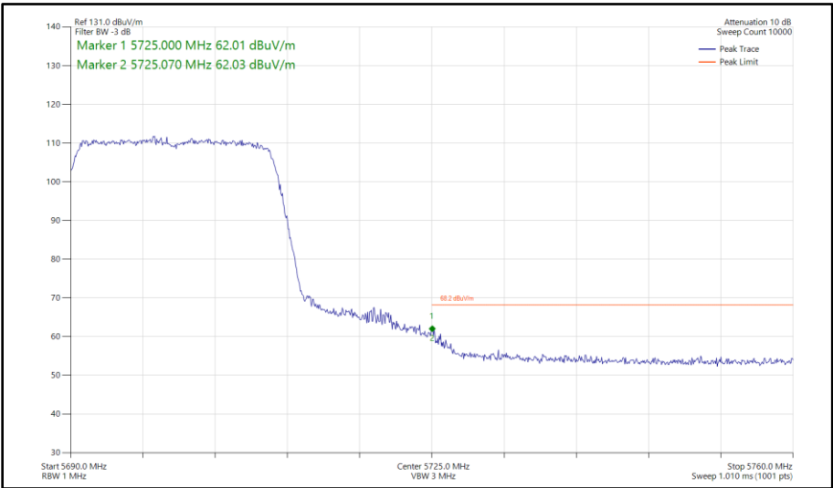
Figure 300 - 802.11ax HE20, SU, SISO, Core 1 - 5700 MHz Band Edge Frequency 5725 MHz
