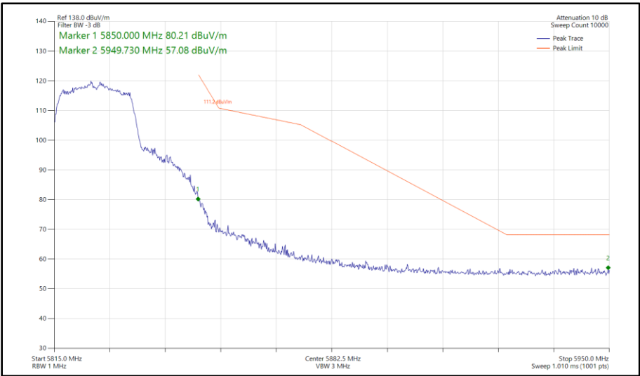
Figure 336 - 802.11n HT20, SDM, Core 0-1 - 5825 MHz Band Edge Frequency 5850 MHz
