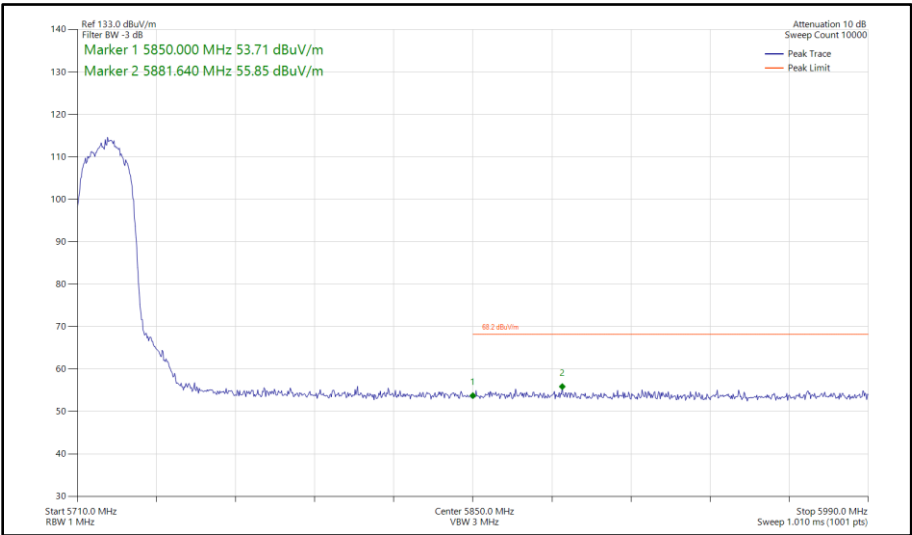
Figure 344 - 802.11ac VHT20, TxBF, Core 0-1 - 5720 MHz Band Edge Frequency 5850 MHz
