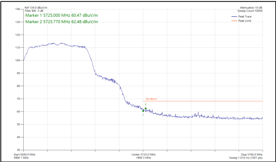
Figure 332 - 802.11n HT20, SDM, Core 0-1 - 5700 MHz Band Edge Frequency 5725 MHz
