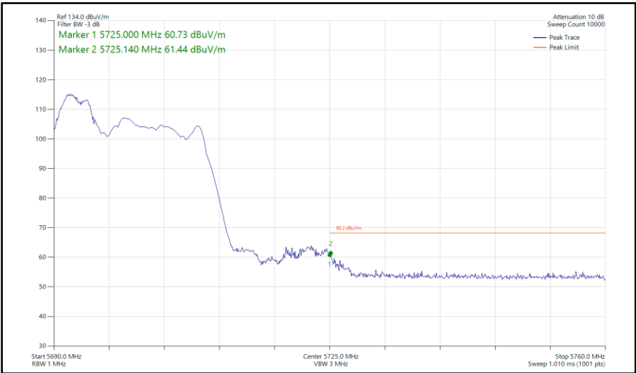
Figure 318 - 802.11ax HE20, RU 52-37, CDD, Core 0-1 - 5700 MHz Band Edge Frequency 5725 MHz
