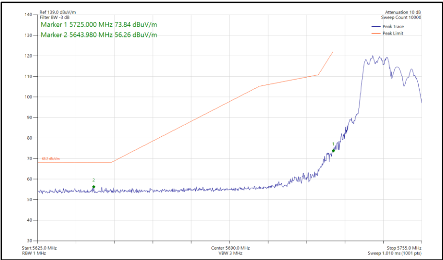
Figure 315 - 802.11ax HE20, RU 106-53, CDD, Core 0-1 - 5745 MHz Band Edge Frequency 5725 MHz
