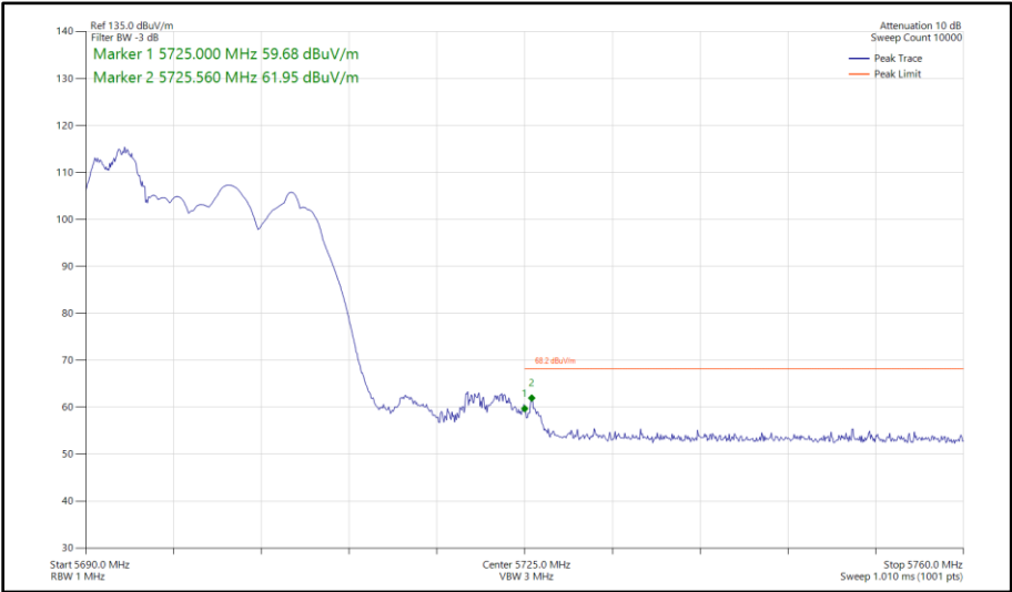
Figure 334 - 802.11ax HE20, RU 52-37, SDM, Core 0-1 - 5700 MHz Band Edge Frequency 5725 MHz
