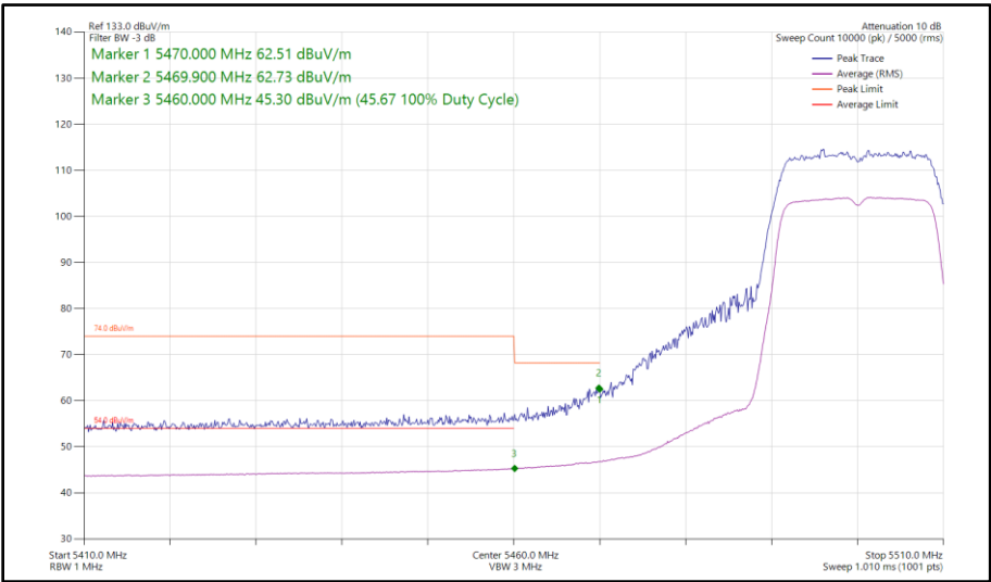
Figure 291 - 802.11n HT20, SISO, Core 1 - 5500 MHz Band Edge Frequency 5470 MHz
