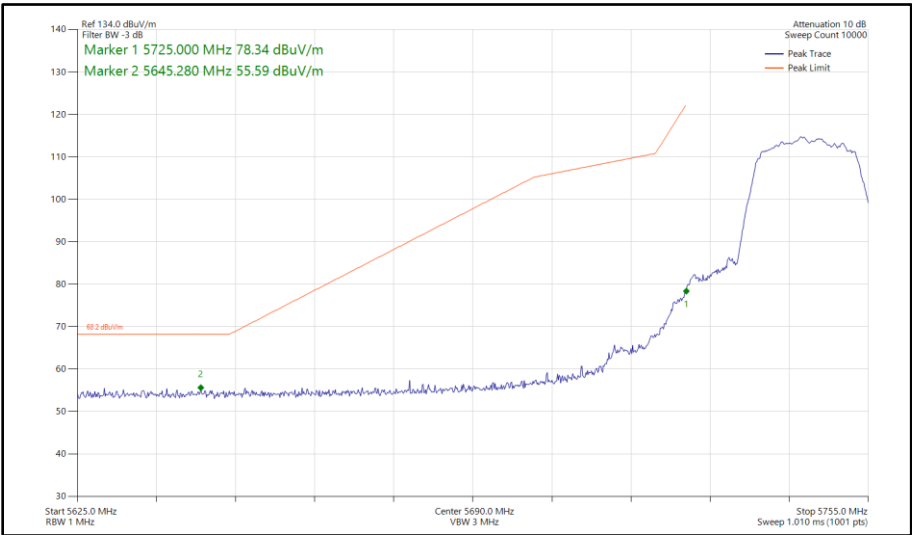
Figure 294 - 802.11a, SISO, Core 1 - 5745 MHz Band Edge Frequency 5725 MHz
