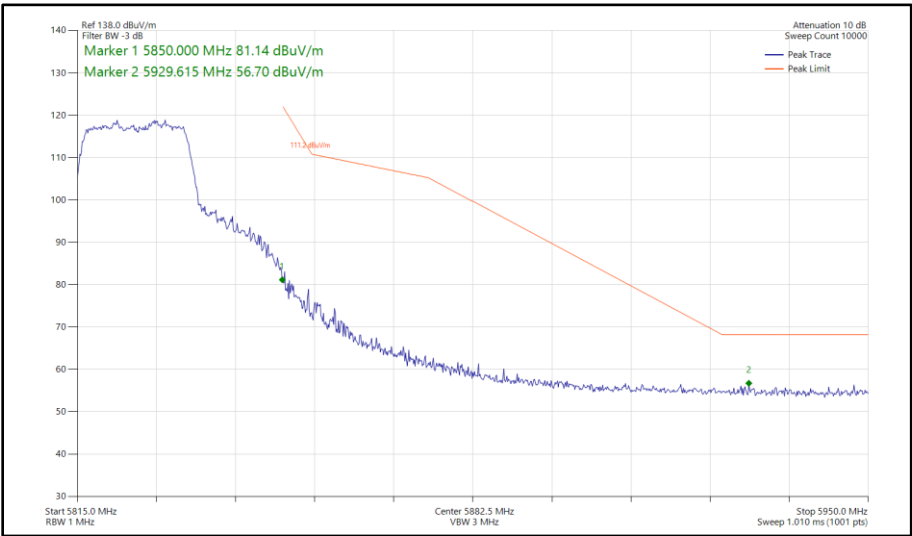
Figure 345 - 802.11ac VHT20, TxBF, Core 0-1 - 5825 MHz Band Edge Frequency 5850 MHz
