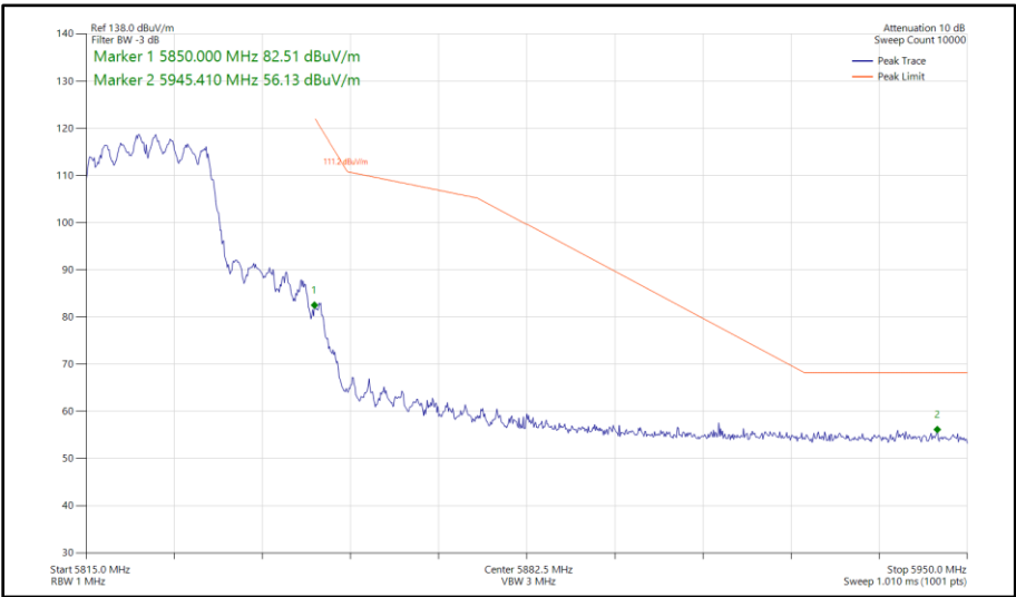
Figure 323 - 802.11ax HE20, SU, CDD, Core 0-1 - 5825 MHz Band Edge Frequency 5850 MHz
