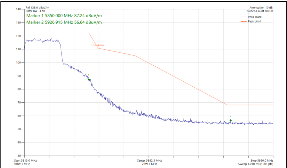
Figure 339 - 802.11ax HE20, SU, SDM, Core 0-1 - 5825 MHz Band Edge Frequency 5850 MHz
