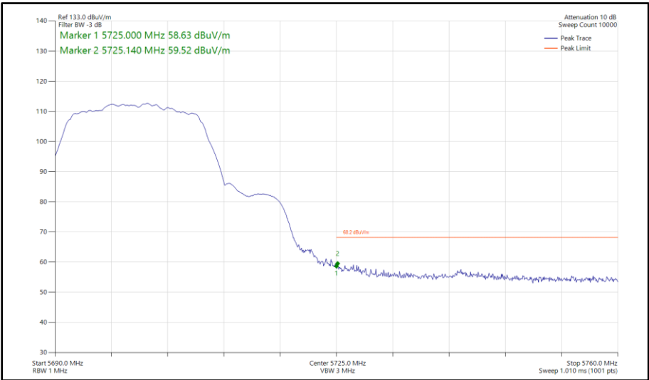
Figure 298 - 802.11a, SISO, Core 1 - 5700 MHz Band Edge Frequency 5725 MHz
