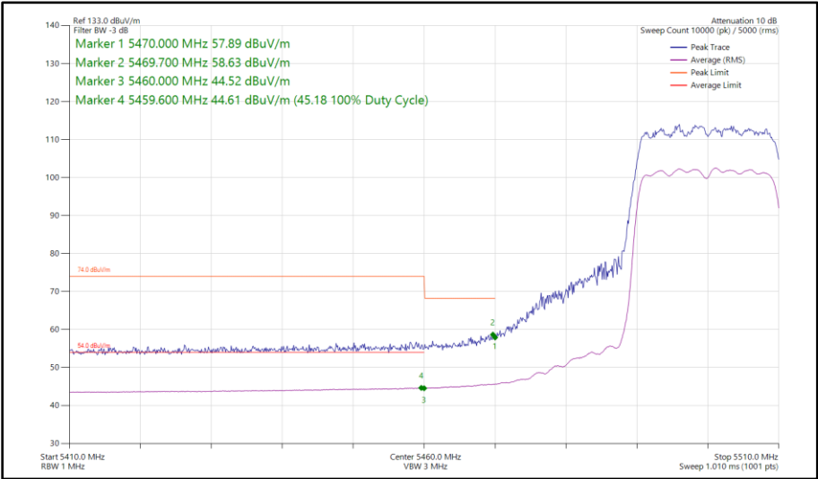
Figure 311 - 802.11ax HE20, SU, CDD, Core 0-1 - 5500 MHz Band Edge Frequency 5470 MHz
