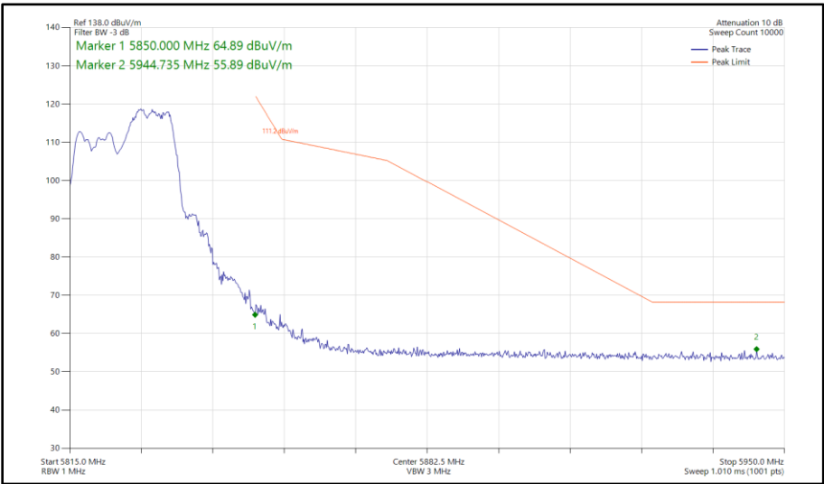
Figure 340 - 802.11ax HE20, RU 106-54, SDM, Core 0-1 - 5825 MHz Band Edge Frequency 5850 MHz
