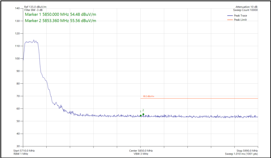
Figure 282 - 802.11a, SISO, Core 0 - 5720 MHz Band Edge Frequency 5850 MHz
