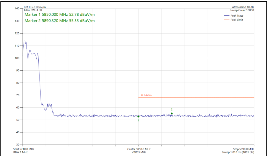
Figure 322 - 802.11ax HE20, RU 52-37, CDD, Core 0-1 - 5720 MHz Band Edge Frequency 5850 MHz
