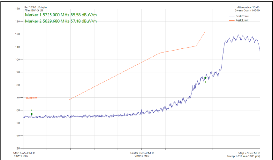
Figure 314 - 802.11ax HE20, SU, CDD, Core 0-1 - 5745 MHz Band Edge Frequency 5725 MHz
