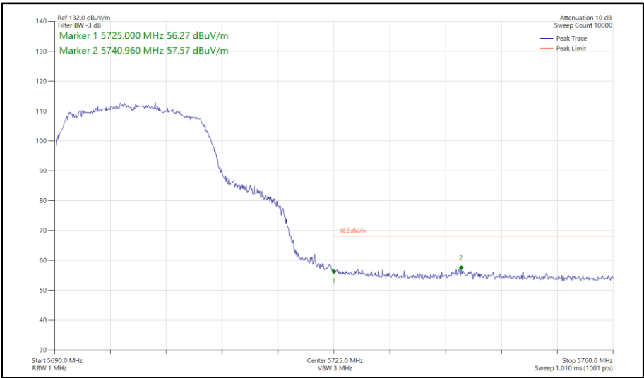
Figure 343 - 802.11ac VHT20, TxBF, Core 0-1 - 5700 MHz Band Edge Frequency 5725 MHz
