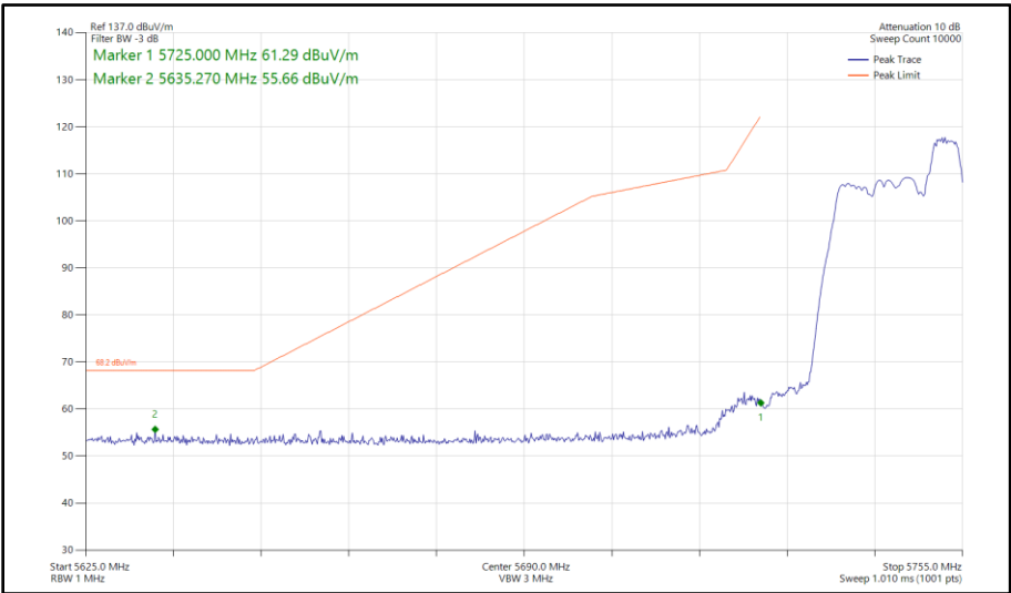
Figure 277 - 802.11ax HE20, RU 52-40, SISO, Core 0 - 5745 MHz Band Edge Frequency 5725 MHz
