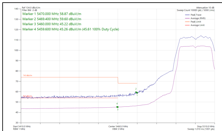
Figure 290 - 802.11a, SISO, Core 1 - 5500 MHz Band Edge Frequency 5470 MHz
