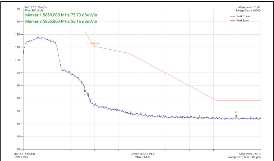
Figure 320 - 802.11n HT20, CDD, Core 0-1 - 5825 MHz Band Edge Frequency 5850 MHz
