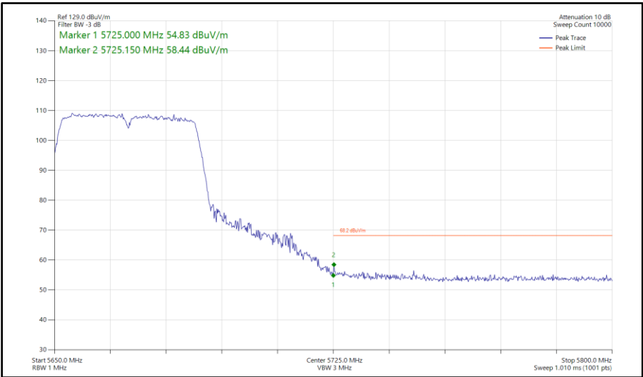
Figure 352 - 802.11n HT40, SISO, Core 0 - 5670 MHz Band Edge Frequency 5725 MHz
