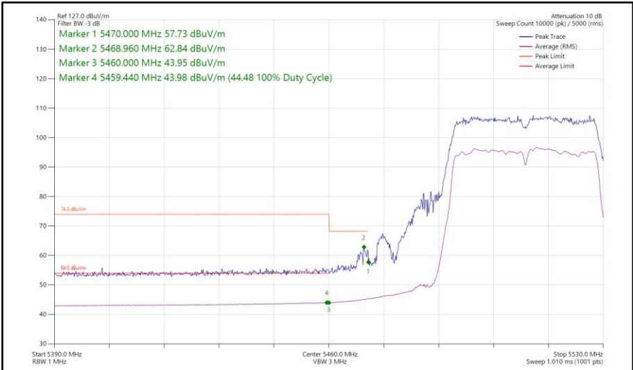
Figure 408 - 802.11ac VHT40, TxBF, Core 0-1 - 5510 MHz Band Edge Frequency 5470 MHz
