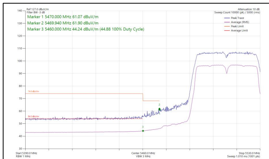
Figure 361 - 802.11n HT40, SISO, Core 1 - 5510 MHz Band Edge Frequency 5470 MHz
