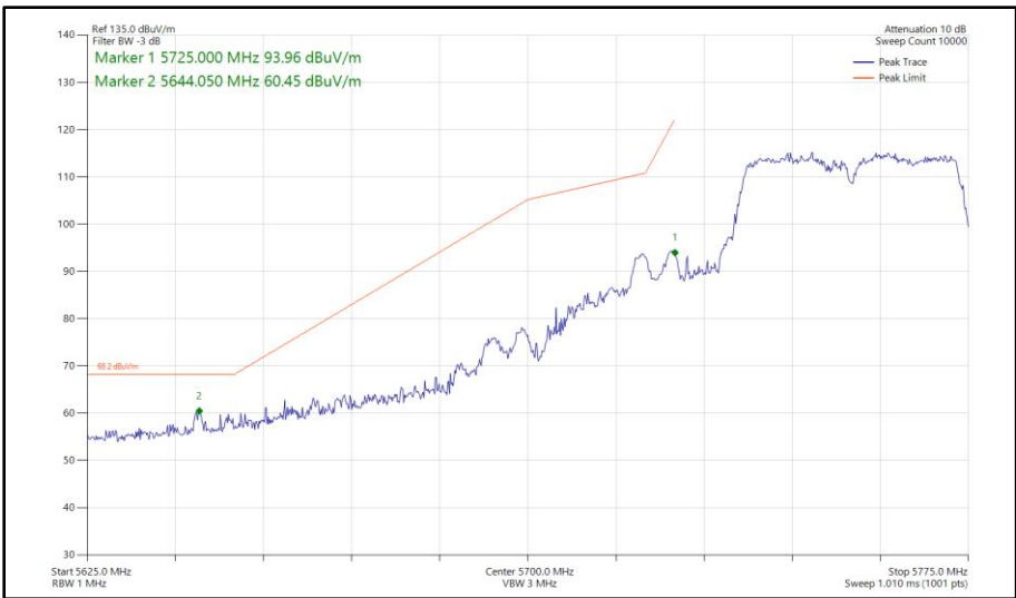
Figure 409 - 802.11ac VHT40, TxBF, Core 0-1 - 5755 MHz Band Edge Frequency 5725 MHz
