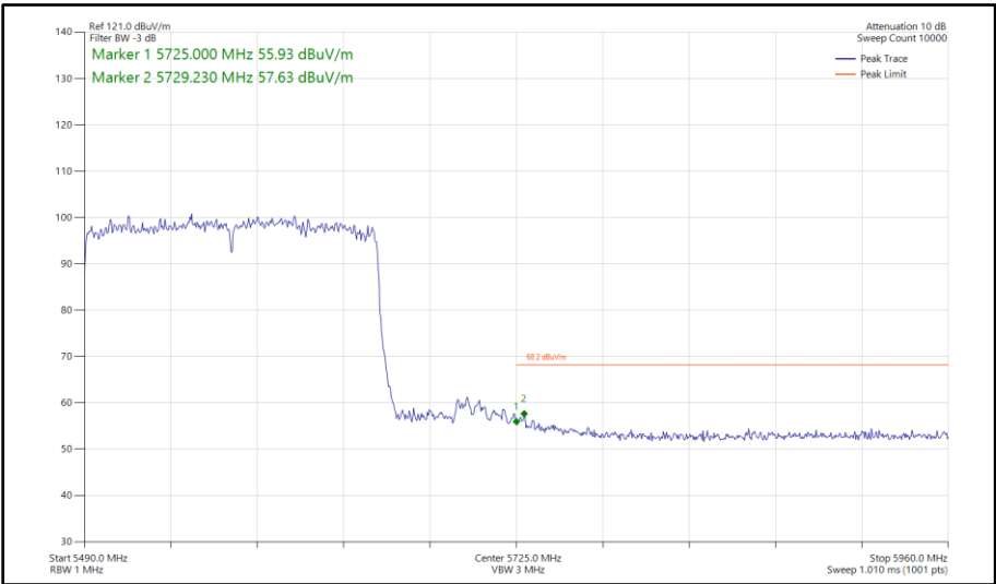
Figure 494 - 802.11ax HE160, SU, CDD, Core 0-1 - 5570 MHz Band Edge Frequency 5725 MHz
