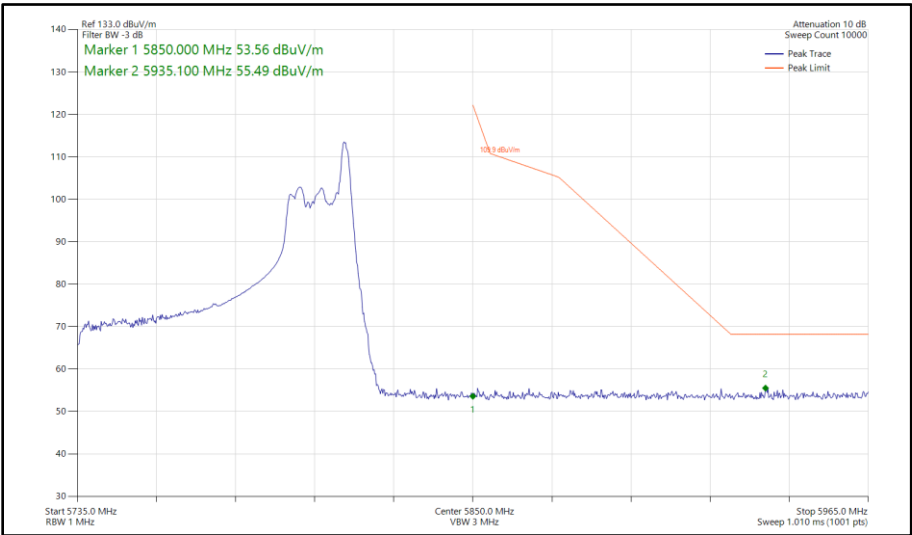
Figure 472 - 802.11ax HE80, RU 26-36, SDM, Core 0-1 - 5775 MHz Band Edge Frequency 5850 MHz
