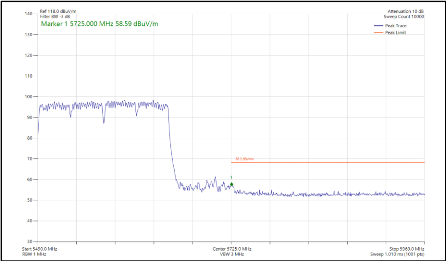
Figure 493 - 802.11ac VHT160, CDD, Core 0-1 - 5570 MHz Band Edge Frequency 5725 MHz
