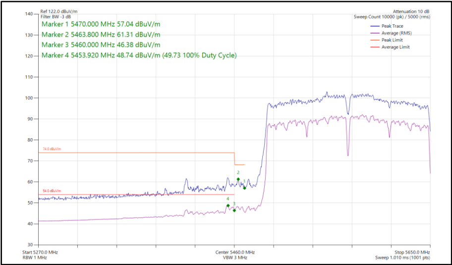
Figure 490 - 802.11ac VHT160, CDD, Core 0-1 - 5570 MHz Band Edge Frequency 5470 MHz
