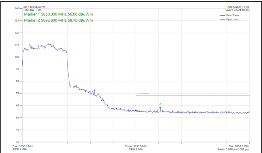
Figure 476 - 802.11ac VHT80, TxBF, Core 0-1 - 5690 MHz Band Edge Frequency 5850 MHz
