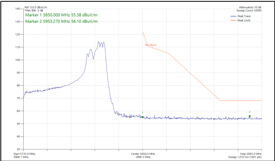
Figure 457 - 802.11ax HE80, RU 106-60, CDD, Core 0-1 - 5775 MHz Band Edge Frequency 5850 MHz
