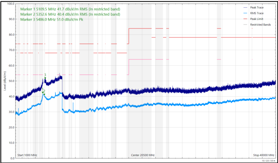
Figure 506 - 5180 MHz (CH36), 802.11a, Core 0, 1 GHz to 40 GHz, Vertical
