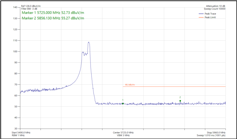
Figure 483 - 802.11ax HE160, RU 52-52S, SISO, Core 0 - 5570 MHz Band Edge Frequency 5725 MHz
