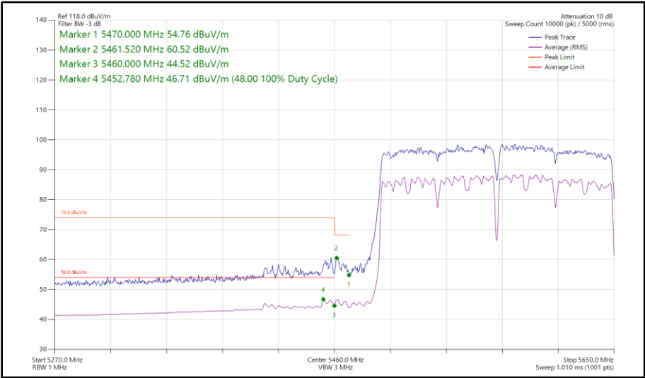
Figure 496 - 802.11ac VHT160, SDM, Core 0-1 - 5570 MHz Band Edge Frequency 5470 MHz
