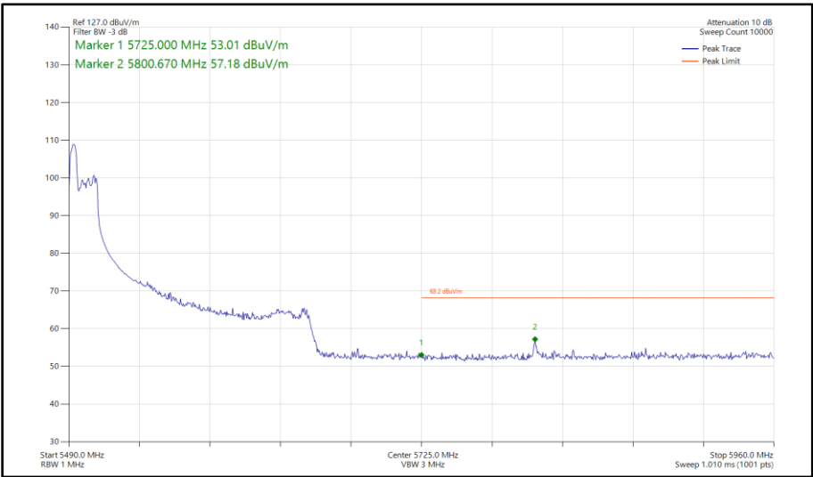
Figure 489 - 802.11ax HE160, RU 52-37P, SISO, Core 1 - 5570 MHz Band Edge Frequency 5725 MHz
