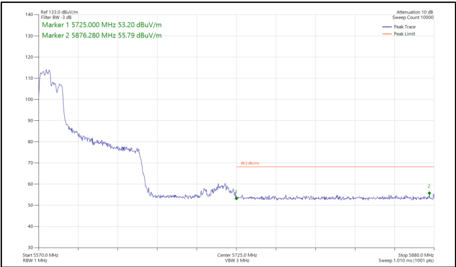
Figure 451 - 802.11ax HE80, RU 106-53, CDD, Core 0-1 - 5610 MHz Band Edge Frequency 5725 MHz
