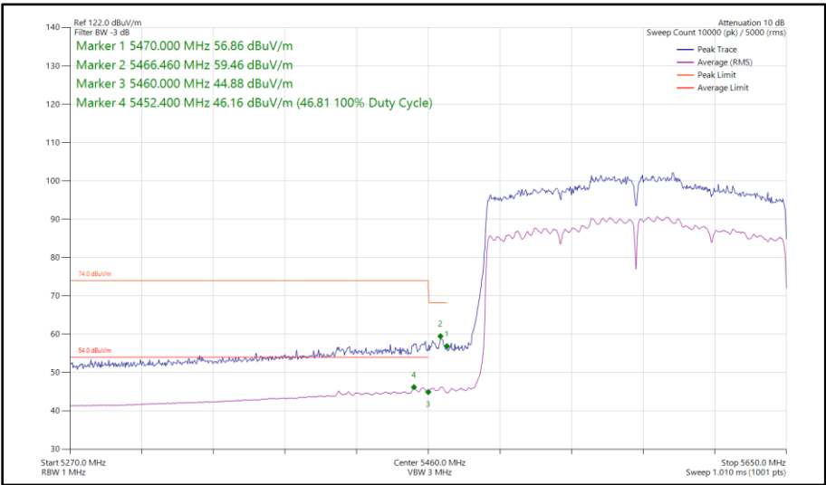
Figure 497 - 802.11ax HE160, SU, SDM, Core 0-1 - 5570 MHz Band Edge Frequency 5470 MHz
