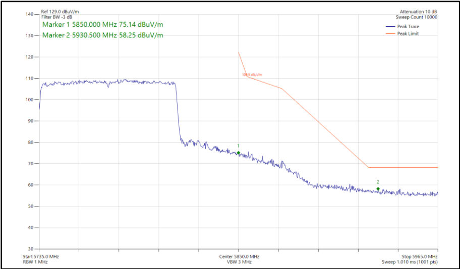
Figure 441 - 802.11ax HE80, SU, SISO, Core 1 - 5775 MHz Band Edge Frequency 5850 MHz
