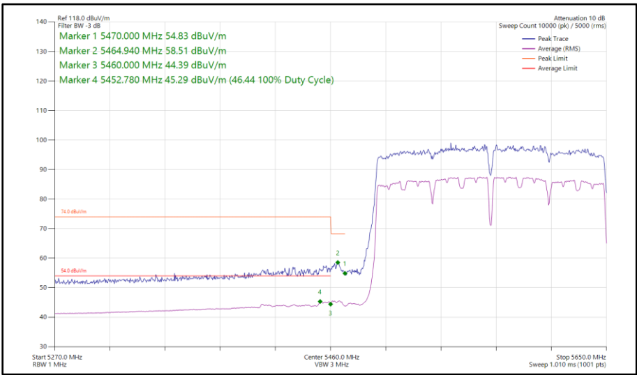
Figure 484 - 802.11ac VHT160, SISO, Core 1 - 5570 MHz Band Edge Frequency 5470 MHz
