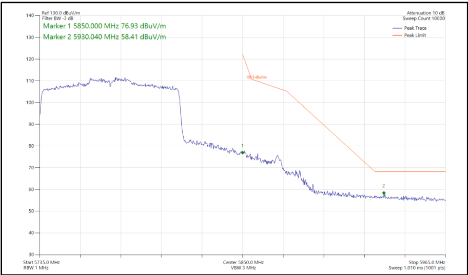
Figure 471 - 802.11ax HE80, SU, SDM, Core 0-1 - 5775 MHz Band Edge Frequency 5850 MHz
