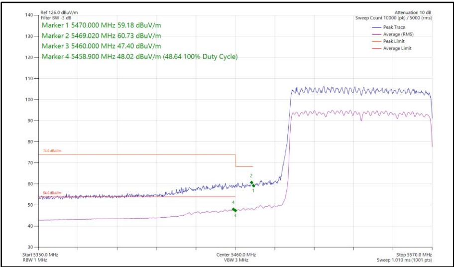
Figure 444 - 802.11ax HE80, SU, CDD, Core 0-1 - 5530 MHz Band Edge Frequency 5470 MHz
