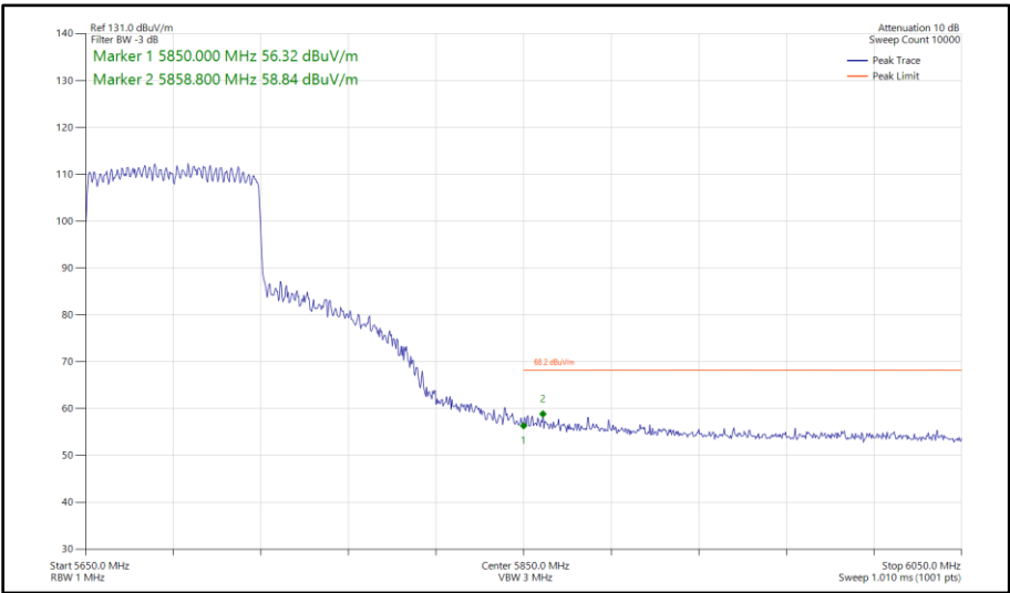
Figure 454 - 802.11ax HE80, SU, CDD, Core 0-1 - 5690 MHz Band Edge Frequency 5850 MHz
