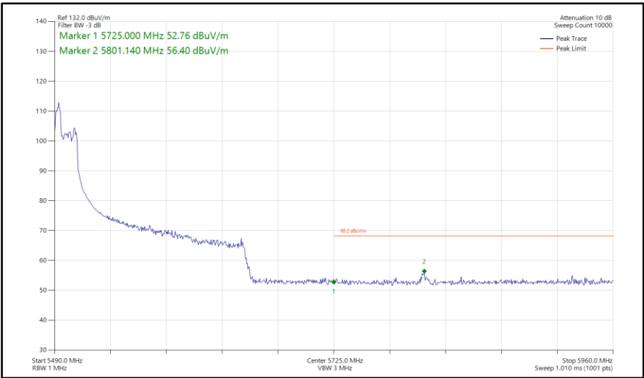
Figure 495 - 802.11ax HE160, RU 52-37P, CDD, Core 0-1 - 5570 MHz Band Edge Frequency 5725 MHz
