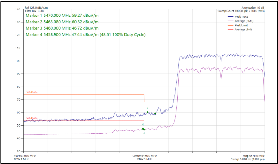
Figure 443 - 802.11ac VHT80, CDD, Core 0-1 - 5530 MHz Band Edge Frequency 5470 MHz
