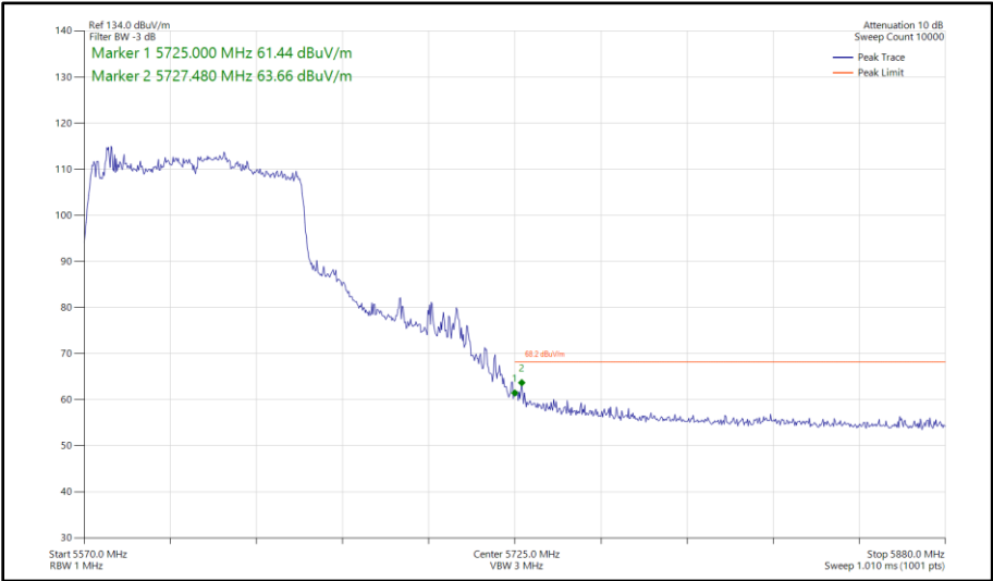
Figure 475 - 802.11ac VHT80, TxBF, Core 0-1 - 5610 MHz Band Edge Frequency 5725 MHz
