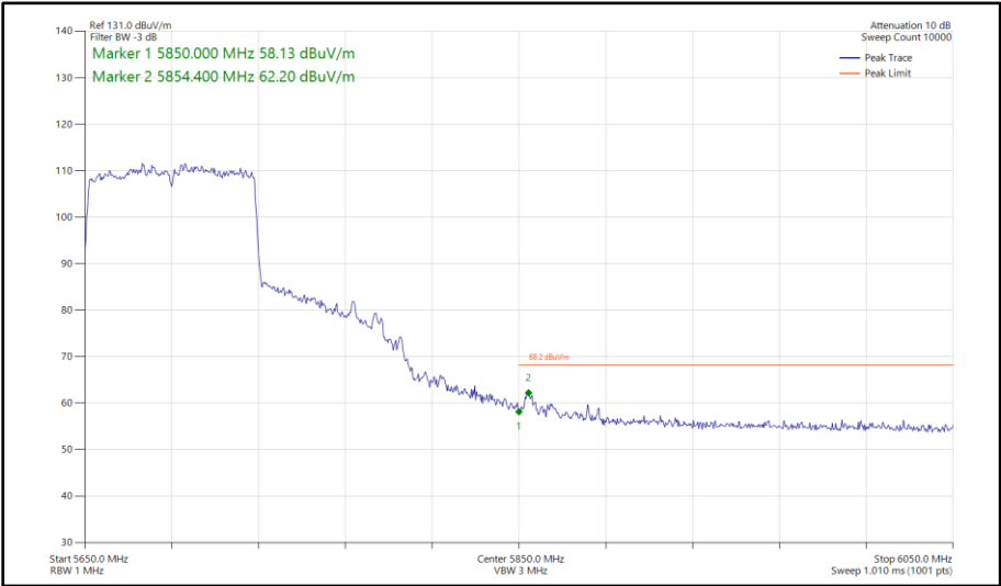
Figure 437 - 802.11ac VHT80, SISO, Core 1 - 5690 MHz Band Edge Frequency 5850 MHz
