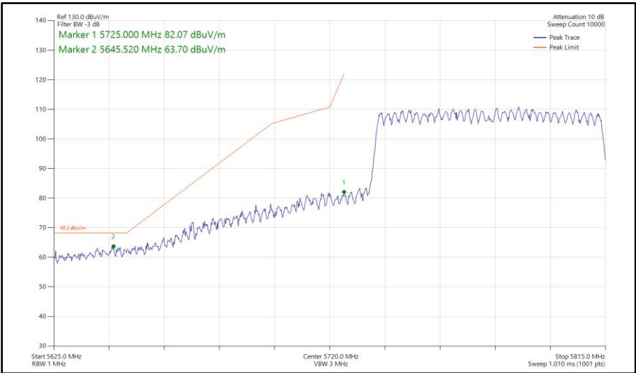
Figure 447 - 802.11ax HE80, SU, CDD, Core 0-1 - 5775 MHz Band Edge Frequency 5725 MHz
