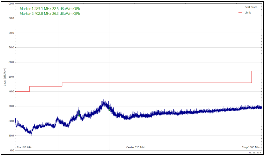
Figure 503 - 5180 MHz (CH36), 802.11a, Core 0, 30 MHz to 1 GHz, Horizontal (Peak)
