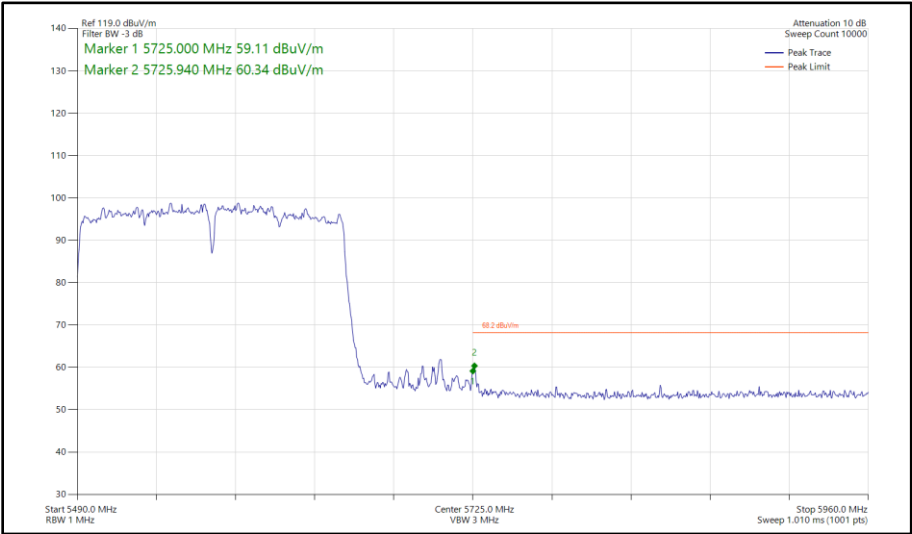
Figure 499 - 802.11ac VHT160, SDM, Core 0-1 - 5570 MHz Band Edge Frequency 5725 MHz
