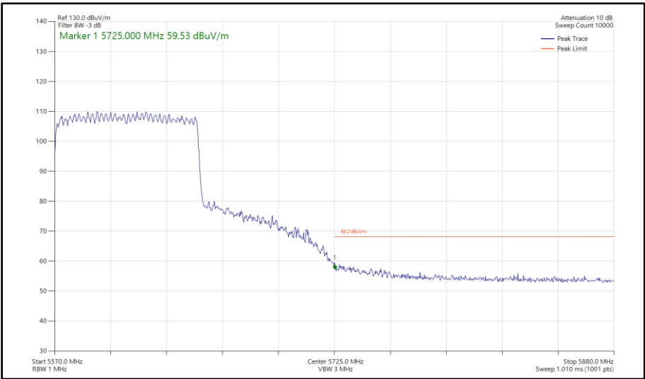
Figure 450 - 802.11ax HE80, SU, CDD, Core 0-1 - 5610 MHz Band Edge Frequency 5725 MHz
