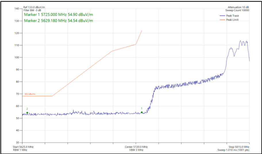
Figure 463 - 802.11ax HE80, RU 106-60, SDM, Core 0-1 - 5775 MHz Band Edge Frequency 5725 MHz
