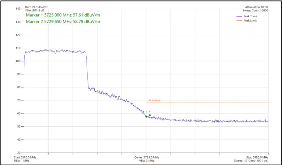
Figure 465 - 802.11ax HE80, SU, SDM, Core 0-1 - 5610 MHz Band Edge Frequency 5725 MHz
