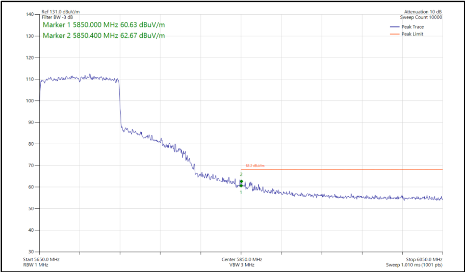
Figure 439 - 802.11ax HE80, SU, SISO, Core 1 - 5690 MHz Band Edge Frequency 5850 MHz
