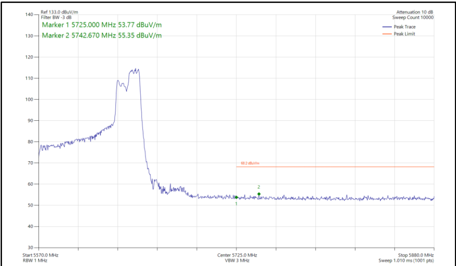
Figure 466 - 802.11ax HE80, RU 106-60, SDM, Core 0-1 - 5610 MHz Band Edge Frequency 5725 MHz
