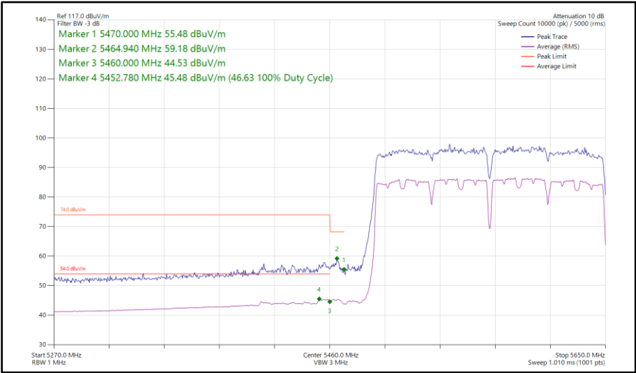
Figure 478 - 802.11ac VHT160, SISO, Core 0 - 5570 MHz Band Edge Frequency 5470 MHz
