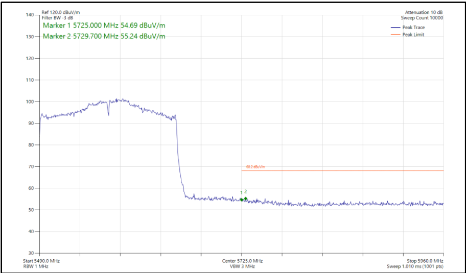
Figure 482 - 802.11ax HE160, SU, SISO, Core 0 - 5570 MHz Band Edge Frequency 5725 MHz
