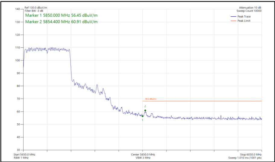
Figure 452 - 802.11ac VHT80, CDD, Core 0-1 - 5690 MHz Band Edge Frequency 5850 MHz
