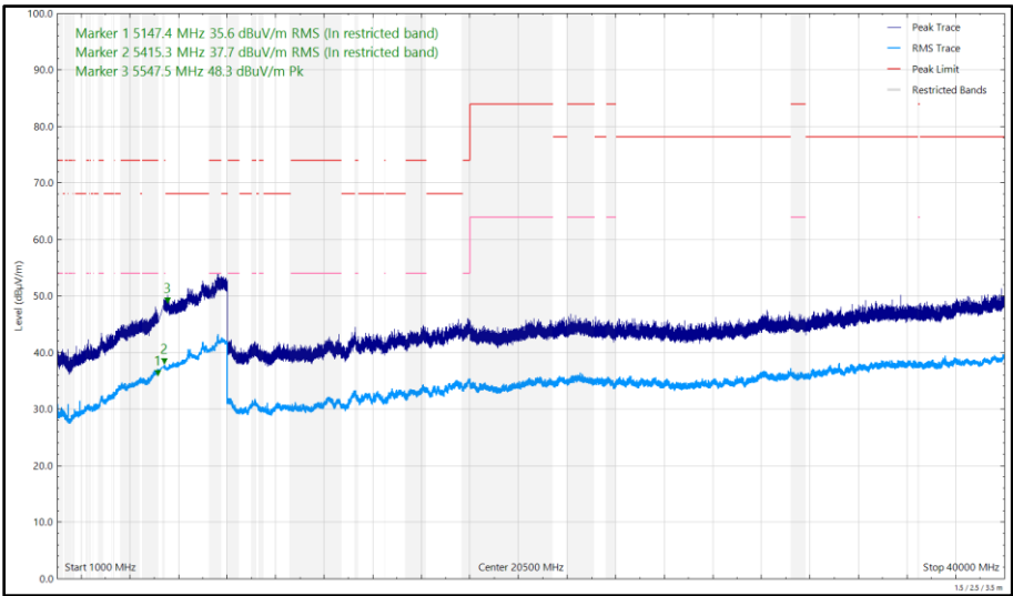
Figure 507 - 5320 MHz (CH64), 802.11a, Core 0, 1 GHz to 40 GHz, Horizontal
