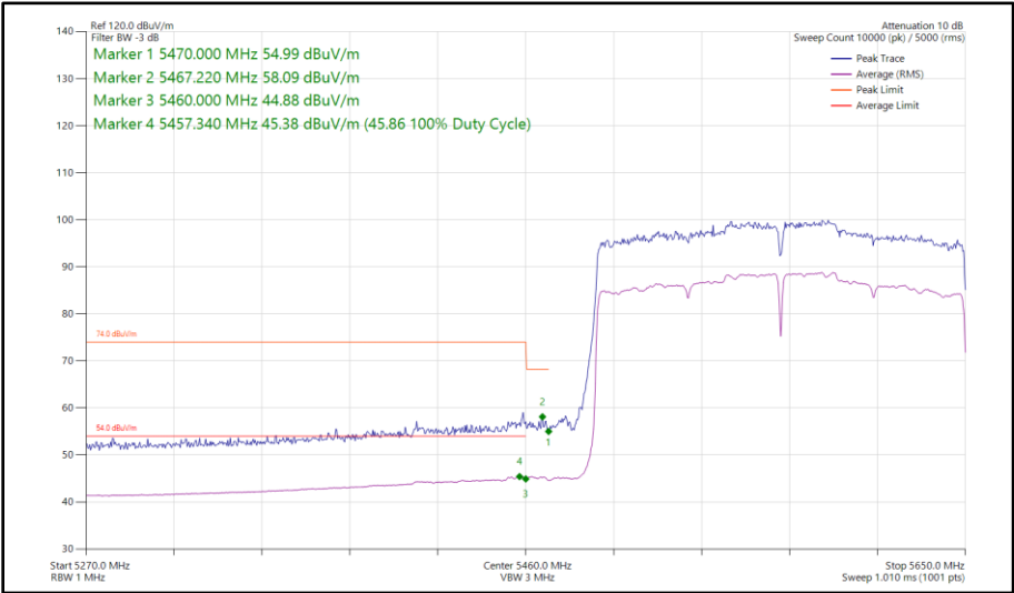
Figure 479 - 802.11ax HE160, SU, SISO, Core 0 - 5570 MHz Band Edge Frequency 5470 MHz
