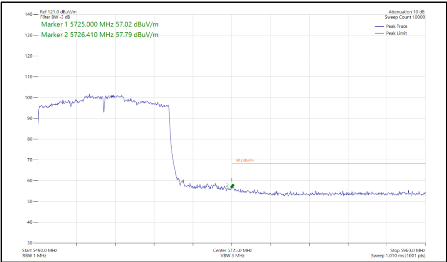
Figure 500 - 802.11ax HE160, SU, SDM, Core 0-1 - 5570 MHz Band Edge Frequency 5725 MHz
