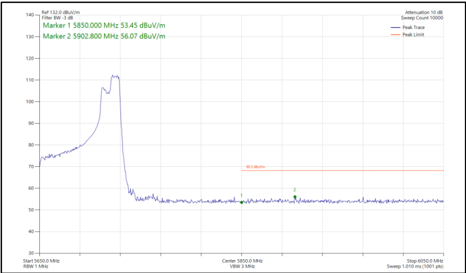
Figure 440 - 802.11ax HE80, RU 106-60, SISO, Core 1 - 5690 MHz Band Edge Frequency 5850 MHz
