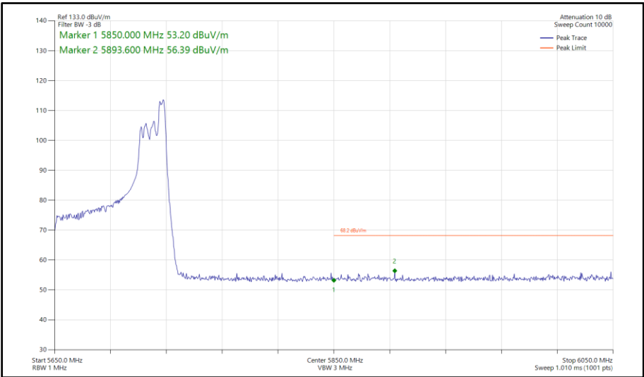
Figure 470 - 802.11ax HE80, RU 52-52, SDM, Core 0-1 - 5690 MHz Band Edge Frequency 5850 MHz
