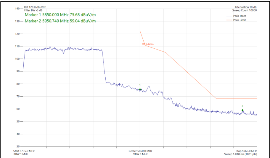
Figure 438 - 802.11ac VHT80, SISO, Core 1 - 5775 MHz Band Edge Frequency 5850 MHz
