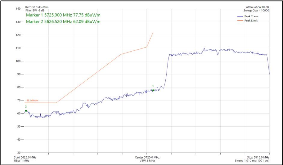
Figure 461 - 802.11ac VHT80, SDM, Core 0-1 - 5775 MHz Band Edge Frequency 5725 MHz
