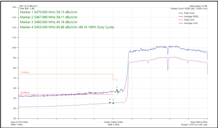
Figure 485 - 802.11ax HE160, SU, SISO, Core 1 - 5570 MHz Band Edge Frequency 5470 MHz
