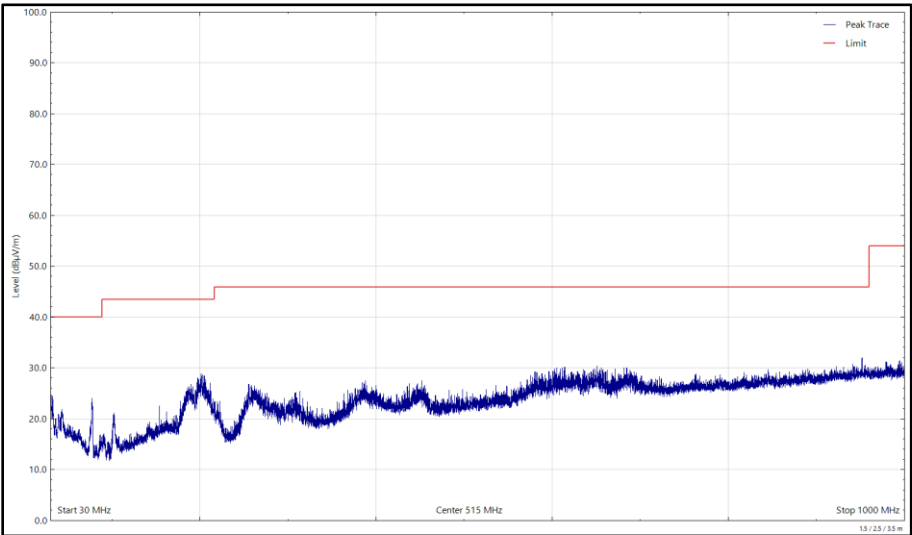
Figure 505 - 5180 MHz (CH36), 802.11a, Core 0, 30 MHz to 1 GHz, Vertical (Peak)
