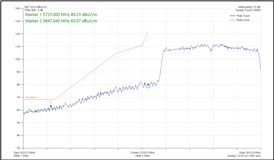
Figure 446 - 802.11ac VHT80, CDD, Core 0-1 - 5775 MHz Band Edge Frequency 5725 MHz
