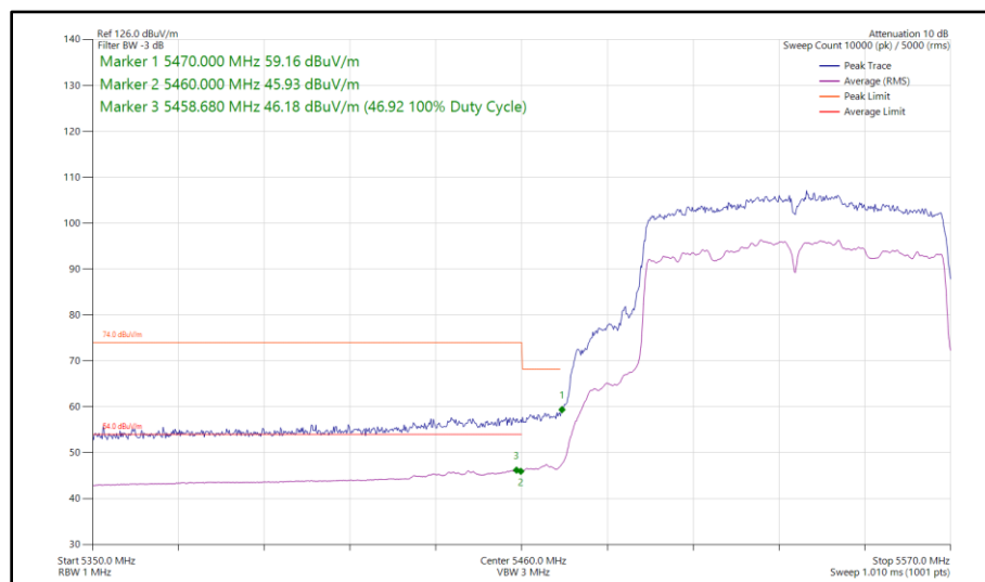
Figure 458 - 802.11ac VHT80, SDM, Core 0-1 - 5530 MHz Band Edge Frequency 5470 MHz
