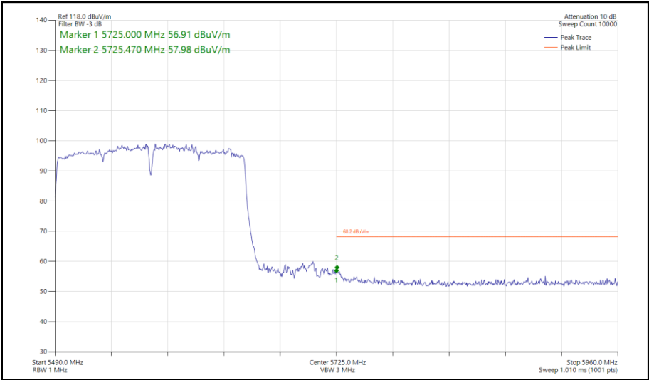
Figure 487 - 802.11ac VHT160, SISO, Core 1 - 5570 MHz Band Edge Frequency 5725 MHz
