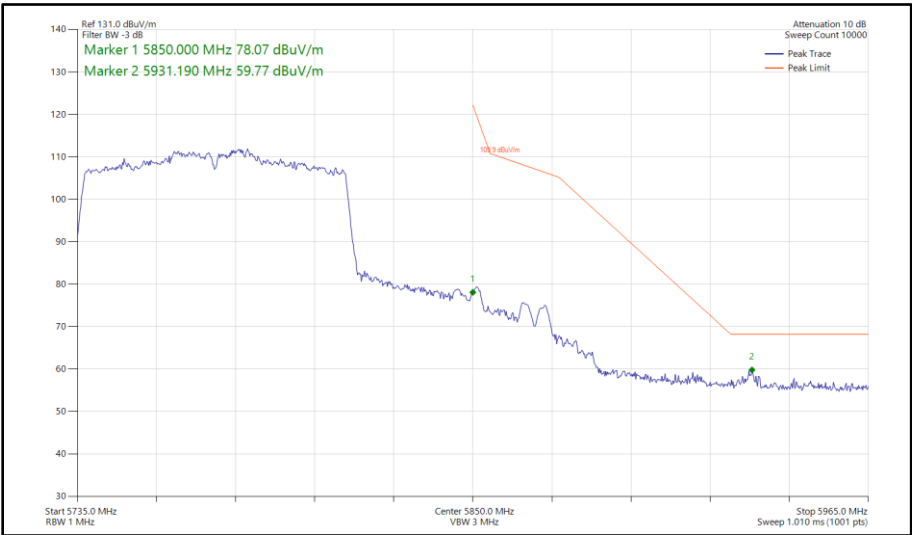
Figure 468 - 802.11ac VHT80, SDM, Core 0-1 - 5775 MHz Band Edge Frequency 5850 MHz
