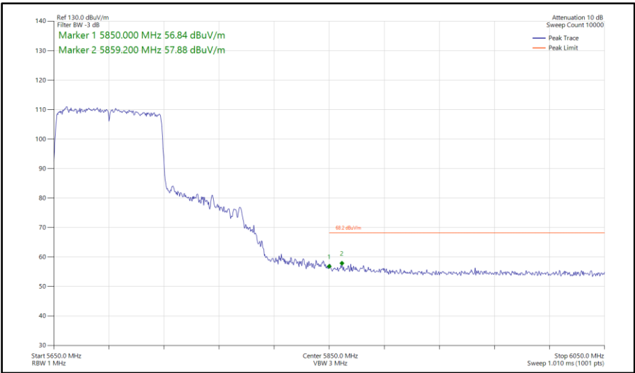
Figure 467 - 802.11ac VHT80, SDM, Core 0-1 - 5690 MHz Band Edge Frequency 5850 MHz
