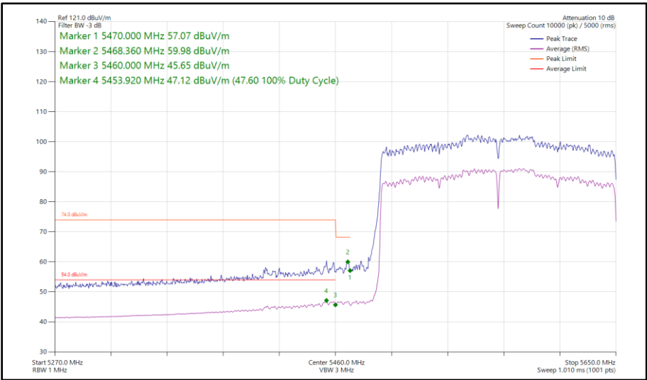
Figure 491 - 802.11ax HE160, SU, CDD, Core 0-1 - 5570 MHz Band Edge Frequency 5470 MHz
