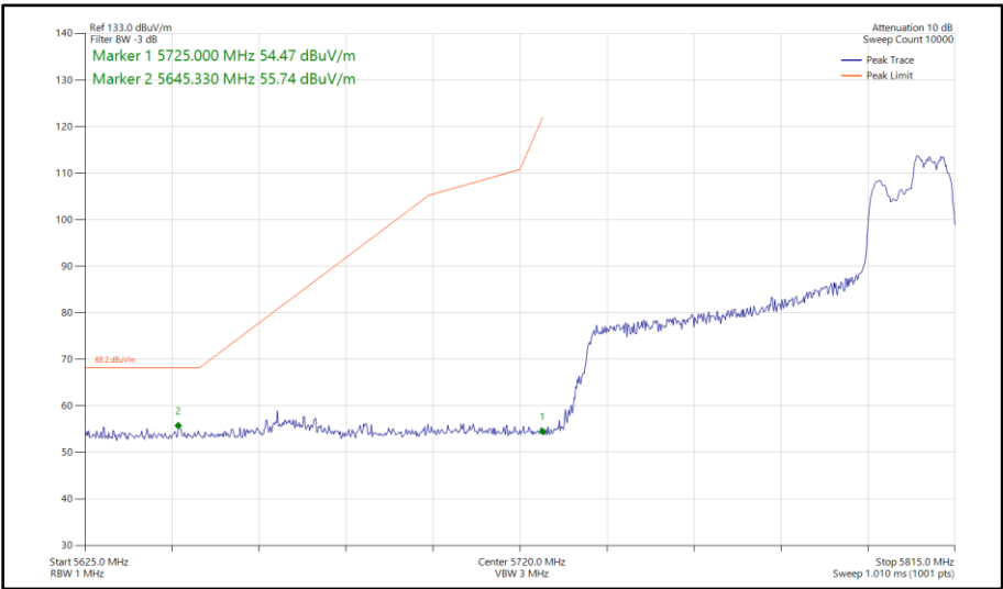
Figure 448 - 802.11ax HE80, RU 106-60, CDD, Core 0-1 - 5775 MHz Band Edge Frequency 5725 MHz
