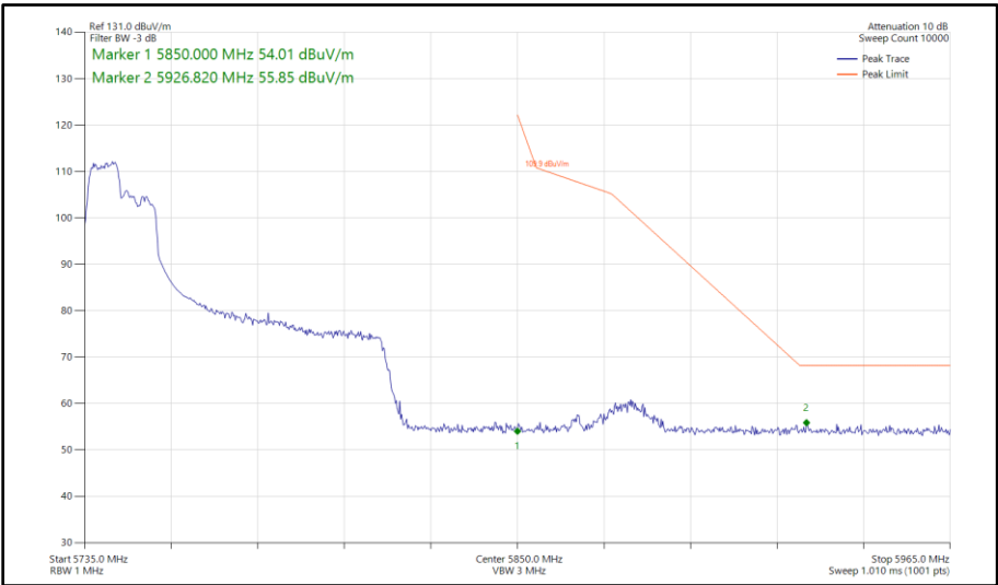
Figure 442 - 802.11ax HE80, RU 106-53, SISO, Core 1 - 5775 MHz Band Edge Frequency 5850 MHz
