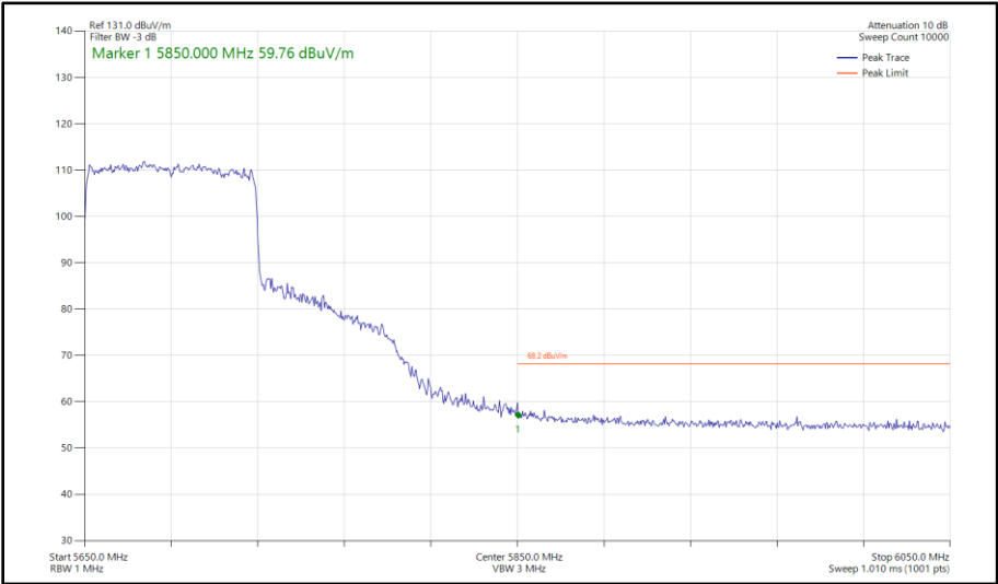
Figure 469 - 802.11ax HE80, SU, SDM, Core 0-1 - 5690 MHz Band Edge Frequency 5850 MHz
