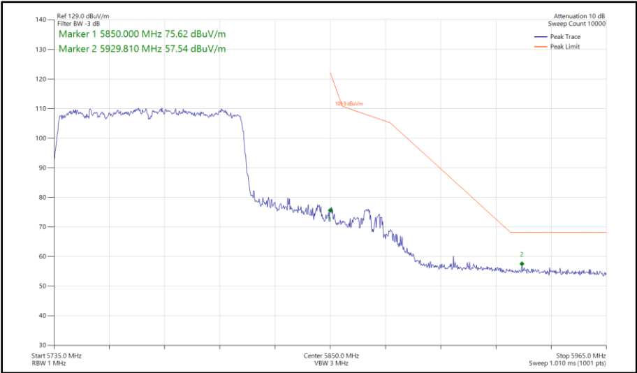
Figure 477 - 802.11ac VHT80, TxBF, Core 0-1 - 5775 MHz Band Edge Frequency 5850 MHz
