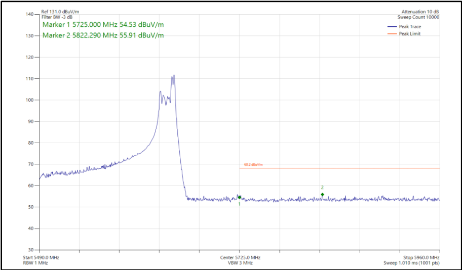
Figure 501 - 802.11ax HE160, RU 52-52S, SDM, Core 0-1 - 5570 MHz Band Edge Frequency 5725 MHz
