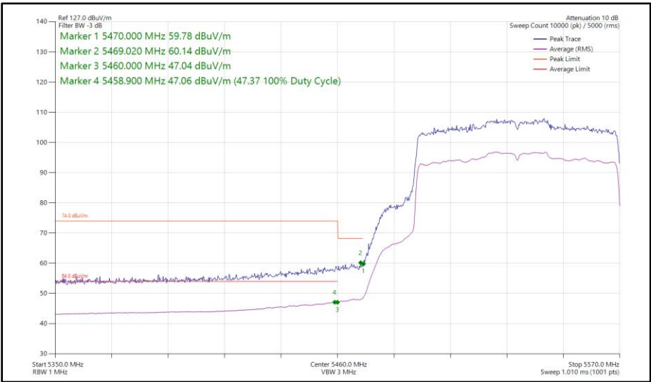
Figure 459 - 802.11ax HE80, SU, SDM, Core 0-1 - 5530 MHz Band Edge Frequency 5470 MHz
