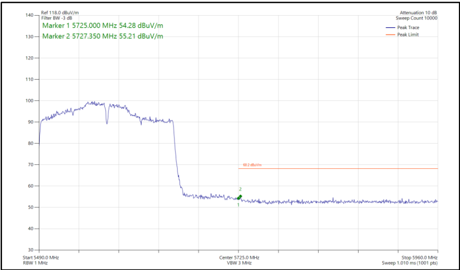
Figure 481 - 802.11ac VHT160, SISO, Core 0 - 5570 MHz Band Edge Frequency 5725 MHz
