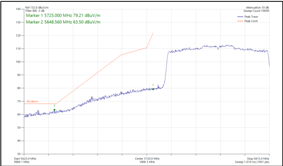
Figure 462 - 802.11ax HE80, SU, SDM, Core 0-1 - 5775 MHz Band Edge Frequency 5725 MHz
