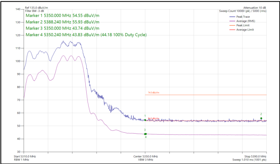
Figure 39 - 802.11ax HE20, RU 106-54, SDM, Core 0-1 - 5320 MHz Band Edge Frequency 5350 MHz
