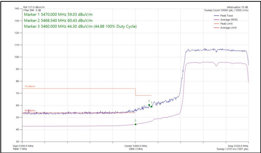
Figure 55 - 802.11ax HE40, SU, SISO, Core 0 - 5510 MHz Band Edge Frequency 5460 MHz
