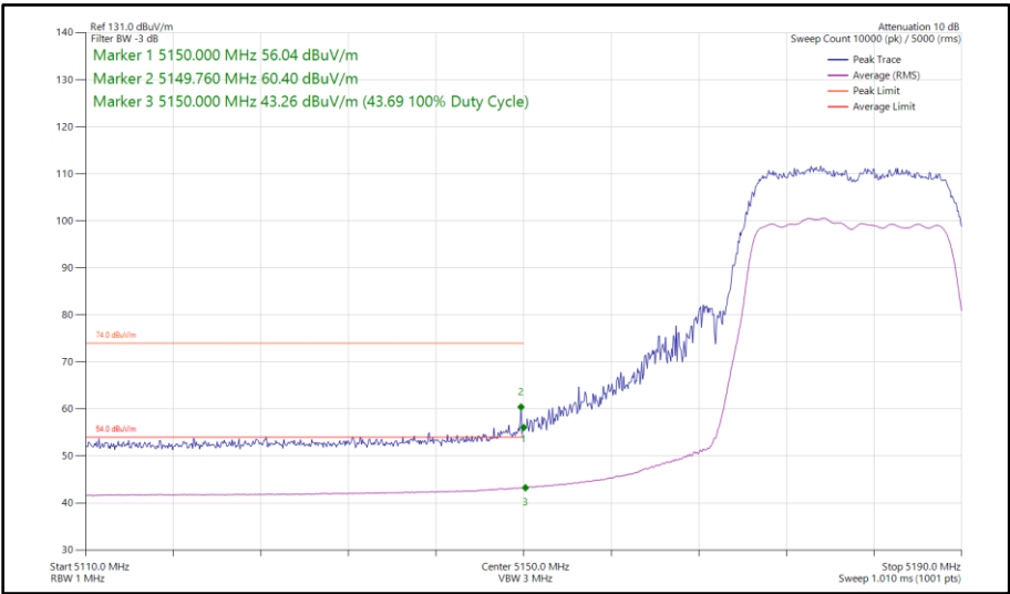
Figure 43 - 802.11ac VHT20, TxBF, Core 0-1 - 5180 MHz Band Edge Frequency 5150 MHz
