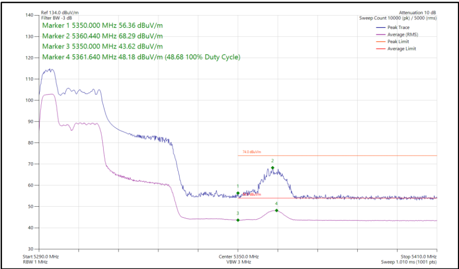
Figure 53 - 802.11ax HE40, RU 52-37, SISO, Core 0 - 5310 MHz Band Edge Frequency 5350 MHz
