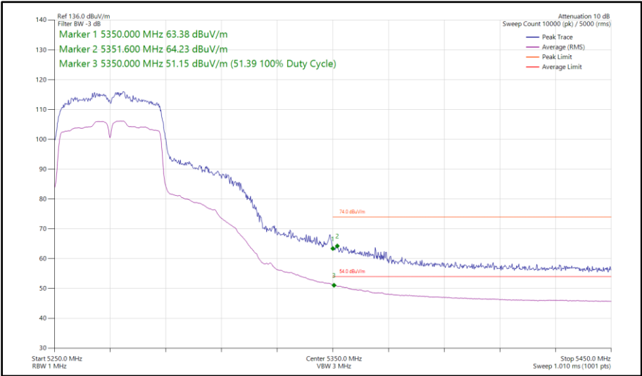
Figure 49 - 802.11n HT40, SISO, Core 0 - 5270 MHz Band Edge Frequency 5350 MHz
