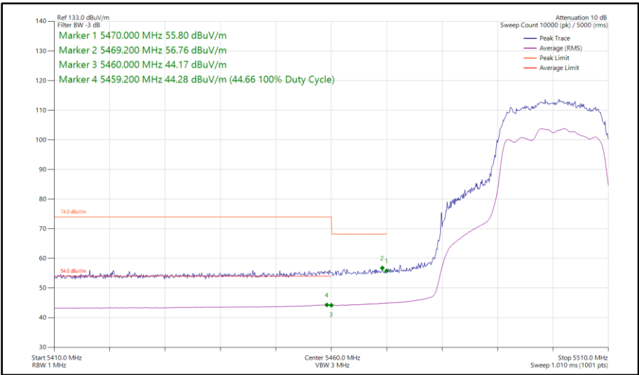
Figure 45 - 802.11ac VHT20, TxBF, Core 0-1 - 5500 MHz Band Edge Frequency 5460 MHz
