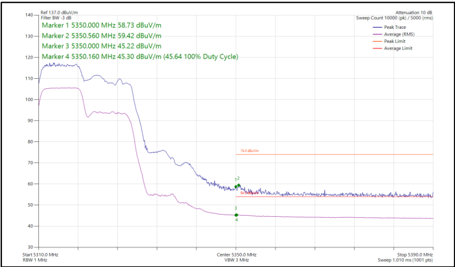
Figure 8 - 802.11ax HE20, RU 106-53, SISO, Core 0 - 5320 MHz Band Edge Frequency 5350 MHz
