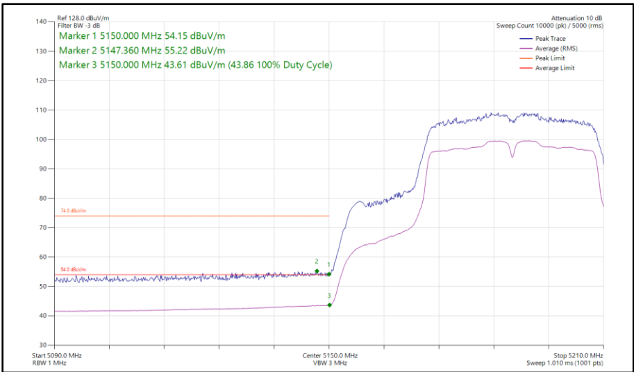
Figure 57 - 802.11n HT40, SISO, Core 1 - 5190 MHz Band Edge Frequency 5150 MHz
