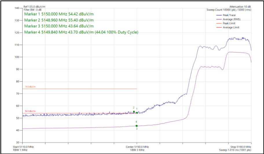
Figure 4 - 802.11ax HE20, RU 106-54, SISO, Core 0 - 5180 MHz Band Edge Frequency 5150 MHz
