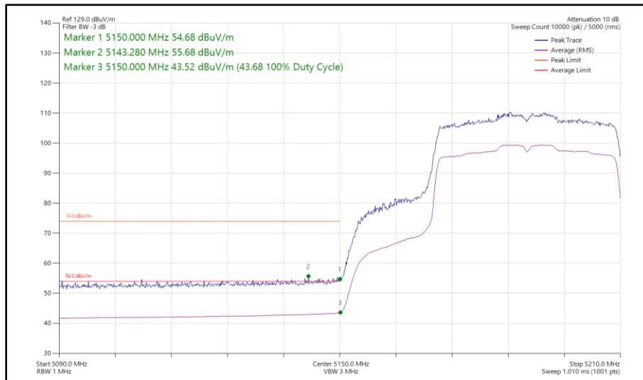
Figure 58 - 802.11ax HE40, SU, SISO, Core 1 - 5190 MHz Band Edge Frequency 5150 MHz
