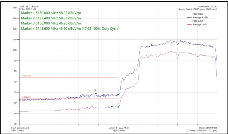
Figure 122 - 802.11ac VHT80, SDM, Core 0-1 - 5210 MHz Band Edge Frequency 5150 MHz
