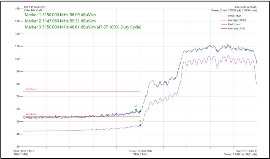
Figure 68 - 802.11n HT40, CDD, Core 0-1 - 5190 MHz Band Edge Frequency 5150 MHz
