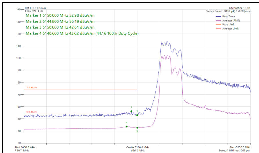
Figure 124 - 802.11ax HE80, RU 106-53, SDM, Core 0-1 - 5210 MHz Band Edge Frequency 5150 MHz
