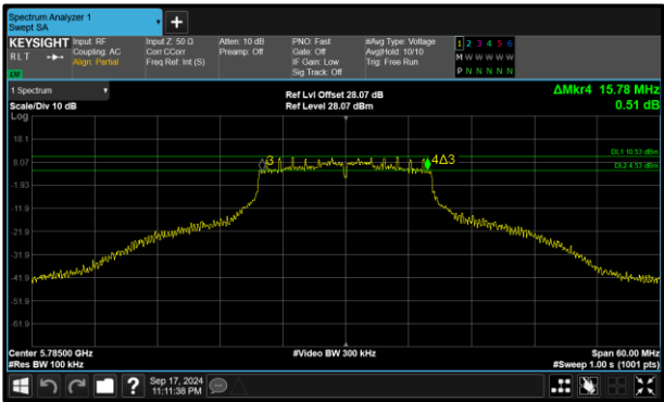
Figure 170 - 802.11a Minimum 6 dB EBW
