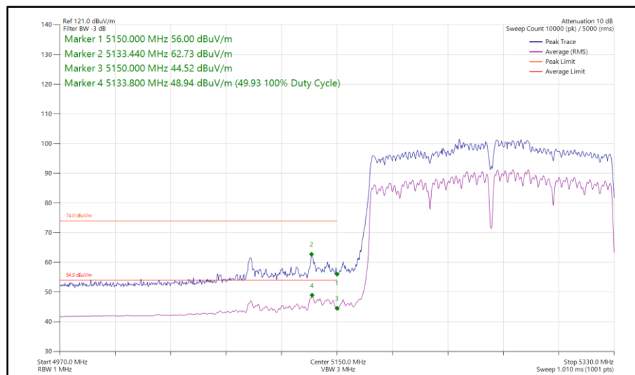
Figure 152 - 802.11ac VHT160, CDD, Core 0-1 - 5250 MHz Band Edge Frequency 5150 MHz
