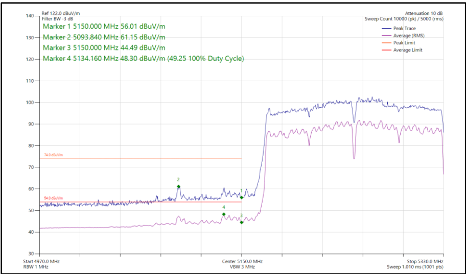
Figure 161 - 802.11ac VHT160, SDM, Core 0-1 - 5250 MHz Band Edge Frequency 5150 MHz
