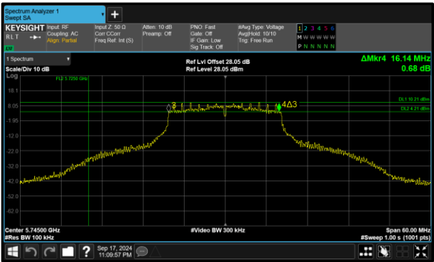
Figure 171 - 802.11a Maximum 6 dB EBW
