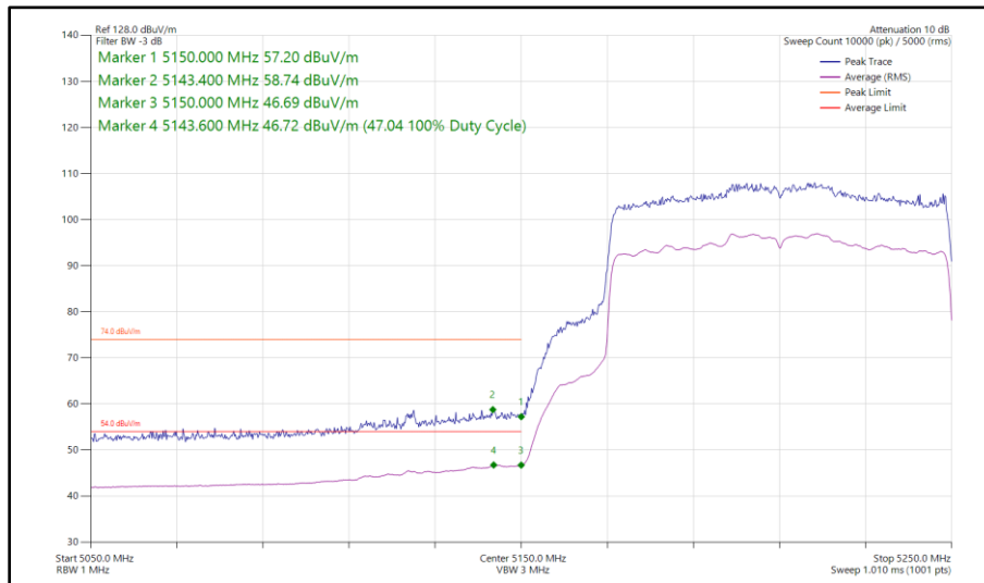
Figure 123 - 802.11ax HE80, SU, SDM, Core 0-1 - 5210 MHz Band Edge Frequency 5150 MHz
