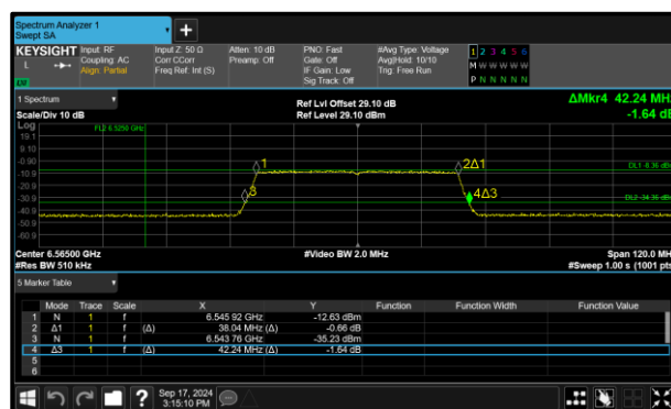
Figure 80 - 802.11ax HE40 SU VLP Maximum 26 dB EBW
