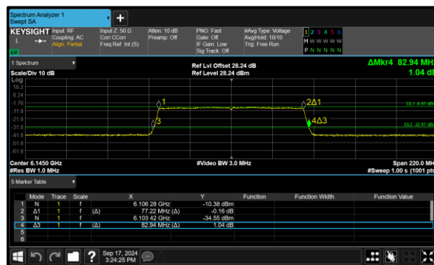
Figure 82 - 802.11ax HE80 SU VLP Maximum 26 dB EBW
