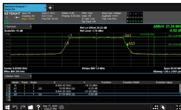
Figure 78 - 802.11ax HE20 SU VLP Maximum 26 dB EBW
