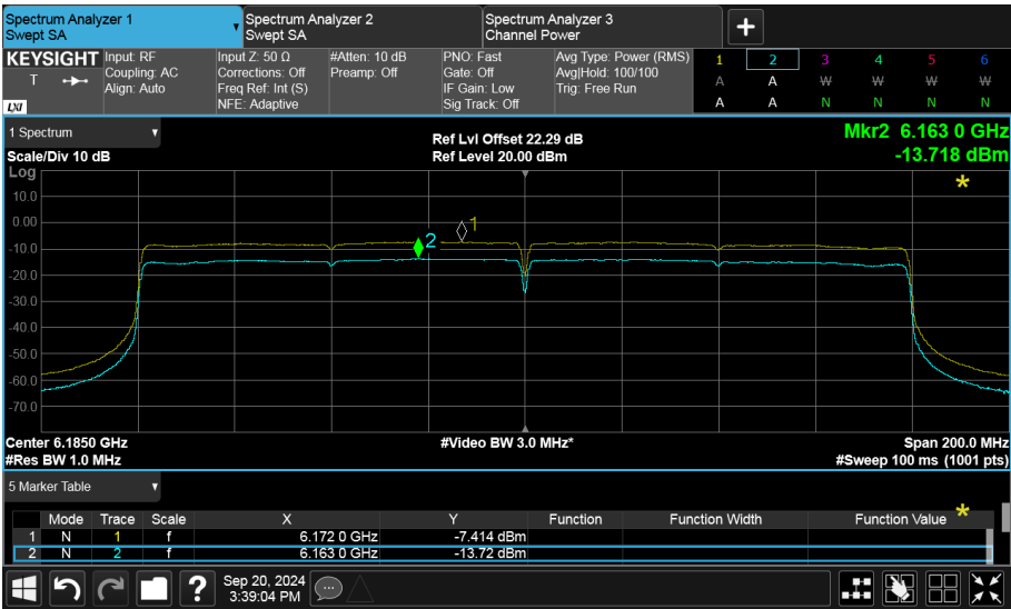
Figure 187 - TPC VLP
