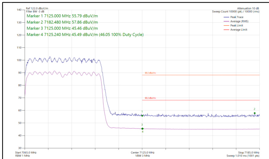
Figure 222 - 802.11ax HE40, SU, CDD, Core 0 - Core 1 - 7085 MHz Band Edge Frequency 7125 MHz
