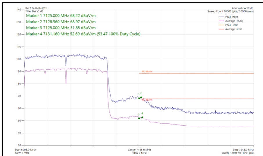
Figure 250 - 802.11ax HE160, SU, SISO, Core 0 - 6985 MHz Band Edge Frequency 7125 MHz
