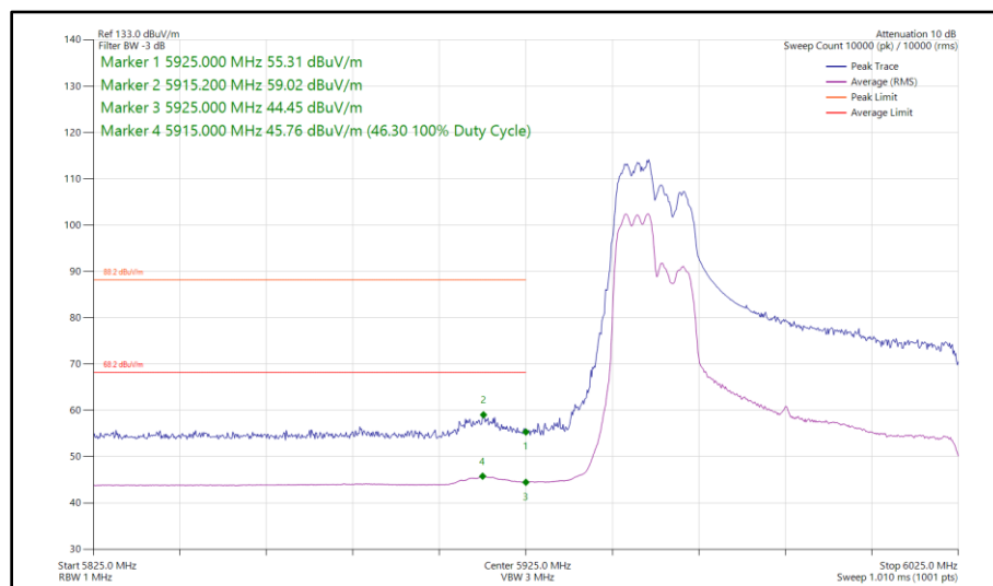
Figure 239 - 802.11ax HE80, RU 106-53, CDD, Core 0 - Core 1 - 5985 MHz Band Edge Frequency 5925 MHz
