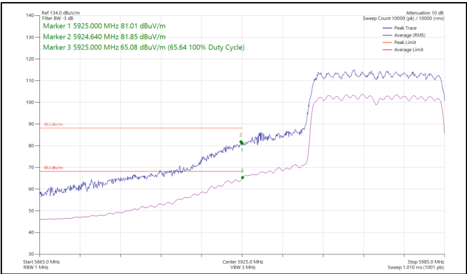
Figure 220 - 802.11ax HE40, SU, CDD, Core 0 - Core 1 - 5965 MHz Band Edge Frequency 5925 MHz
