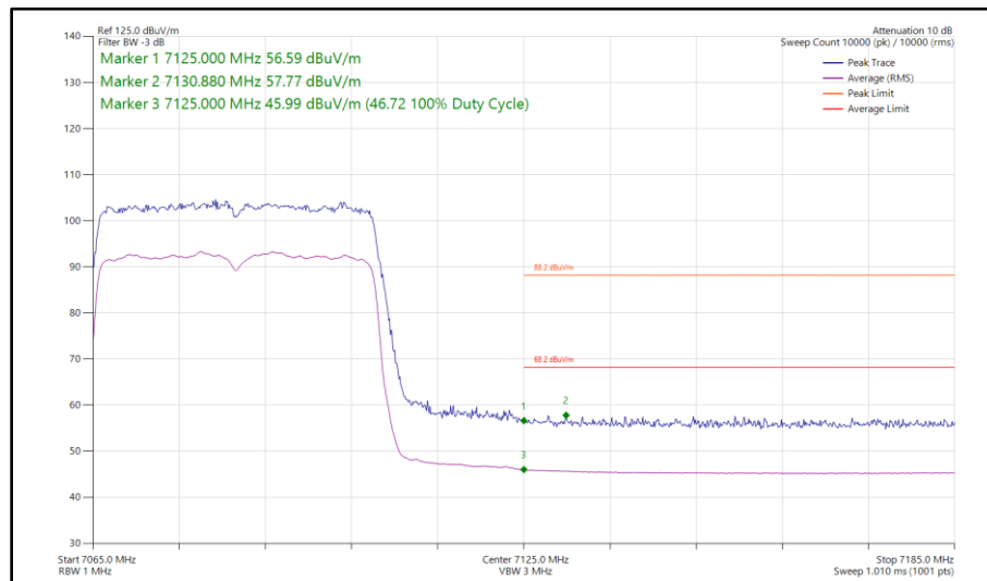
Figure 226 - 802.11ax HE40, SU, SDM, Core 0 - Core 1 - 7085 MHz Band Edge Frequency 7125 MHz
