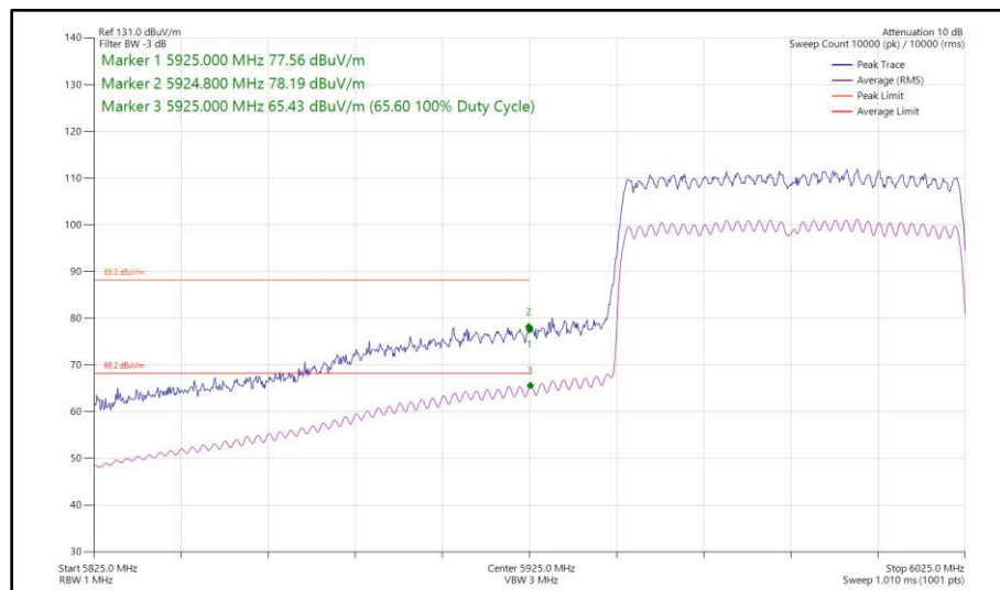
Figure 238 - 802.11ax HE80, SU, CDD, Core 0 - Core 1 - 5985 MHz Band Edge Frequency 5925 MHz
