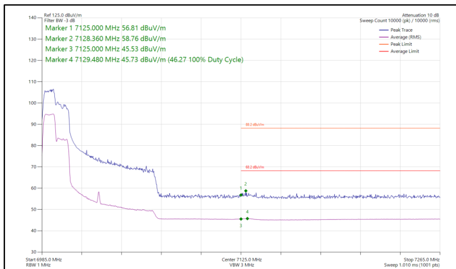
Figure 233 - 802.11ax HE80, RU 106-53, SISO, Core 0 - 7025 MHz Band Edge Frequency 7125 MHz
