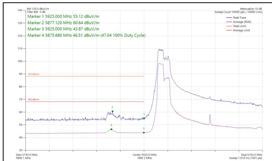
Figure 249 - 802.11ax HE160, RU 106-53P, SISO, Core 0 - 6025 MHz Band Edge Frequency 5925 MHz
