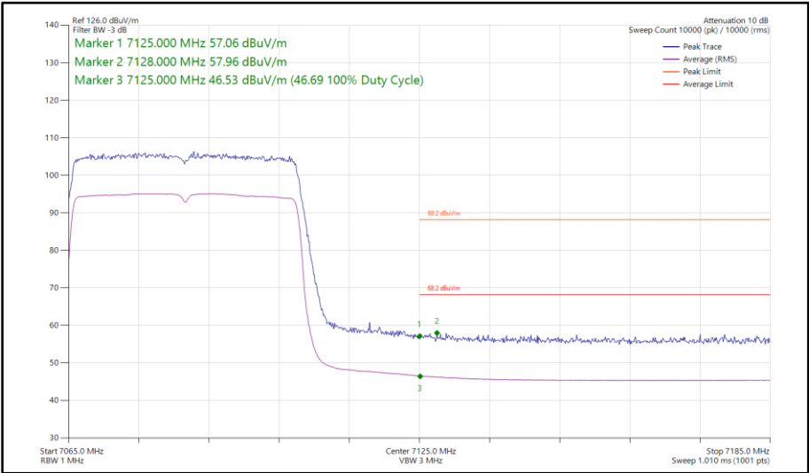
Figure 214 - 802.11ax HE40, SU, SISO, Core 0 - 7085 MHz Band Edge Frequency 7125 MHz
