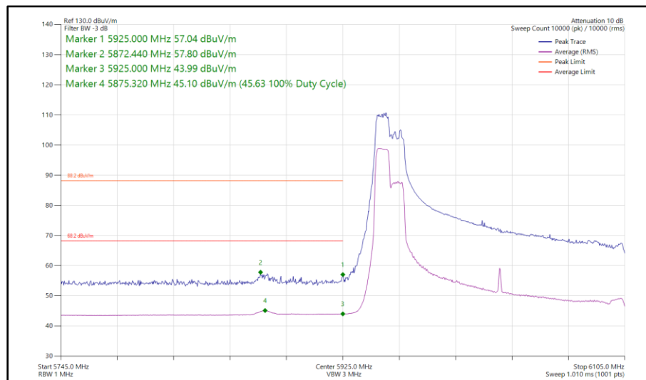
Figure 253 - 802.11ax HE160, RU 106-53P, SISO, Core 1 - 6025 MHz Band Edge Frequency 5925 MHz
