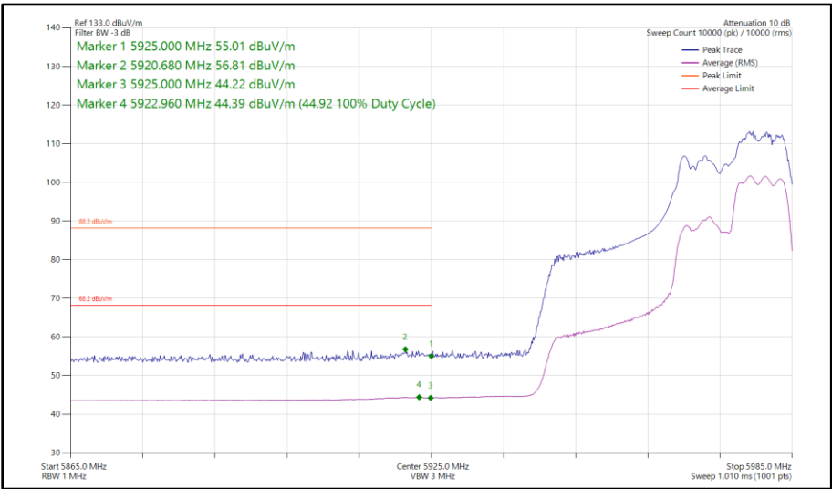
Figure 221 - 802.11ax HE40, RU 106-56, CDD, Core 0 - Core 1 - 5965 MHz Band Edge Frequency 5925 MHz
