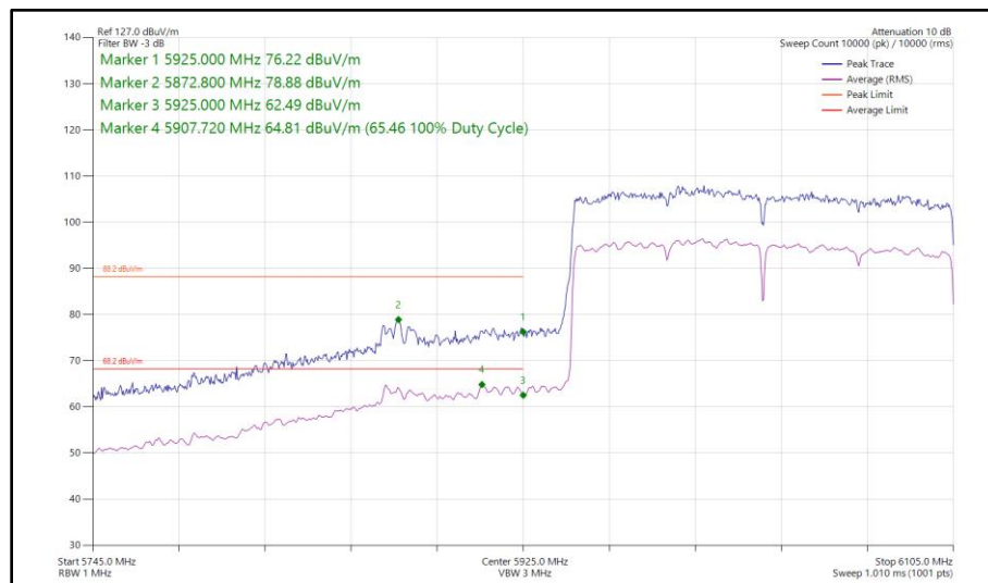
Figure 260 - 802.11ax HE160, SU, SDM, Core 0 - Core 1 - 6025 MHz Band Edge Frequency 5925 MHz
