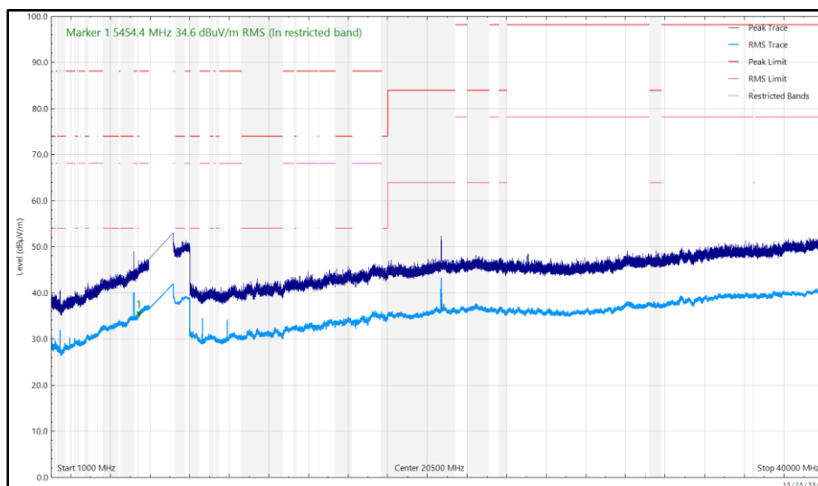
Figure 290 - U-NII-8 - 6895 MHz (CH189), HE20, SU, CDD, Core 0 + Core 1, 1 GHz to 40 GHz, Vertical
