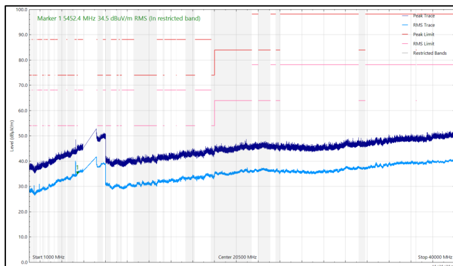
Figure 292 - U-NII-8 - 6995 MHz (CH209), HE20, SU, CDD, Core 0 + Core 1, 1 GHz to 40 GHz, Horizontal
