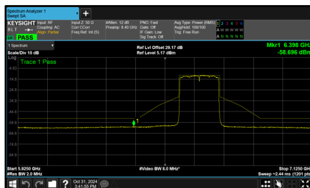
Figure 337 - B (Core 1) 802.11ax HE160 SU VLP 6665 MHz (CH143)
