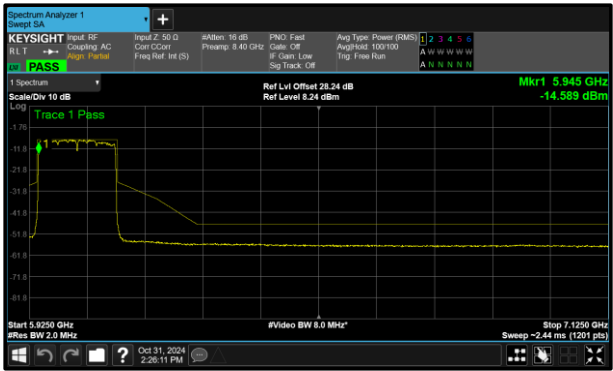
Figure 341 - B (Core 1) 802.11ax HE160 SU LPI 6025 MHz (CH15)
