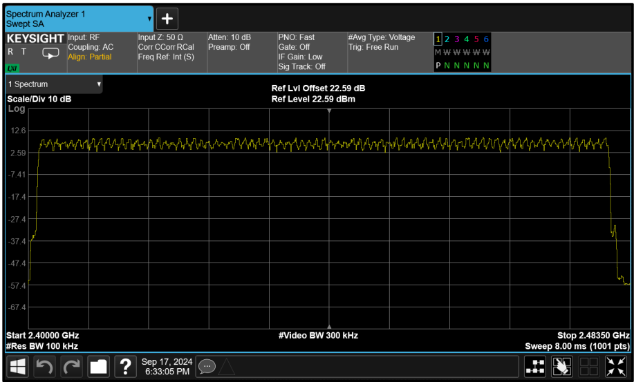
Figure 108 - \pi/4 DQPSK (2-DH5) - Number of Hopping Channels
