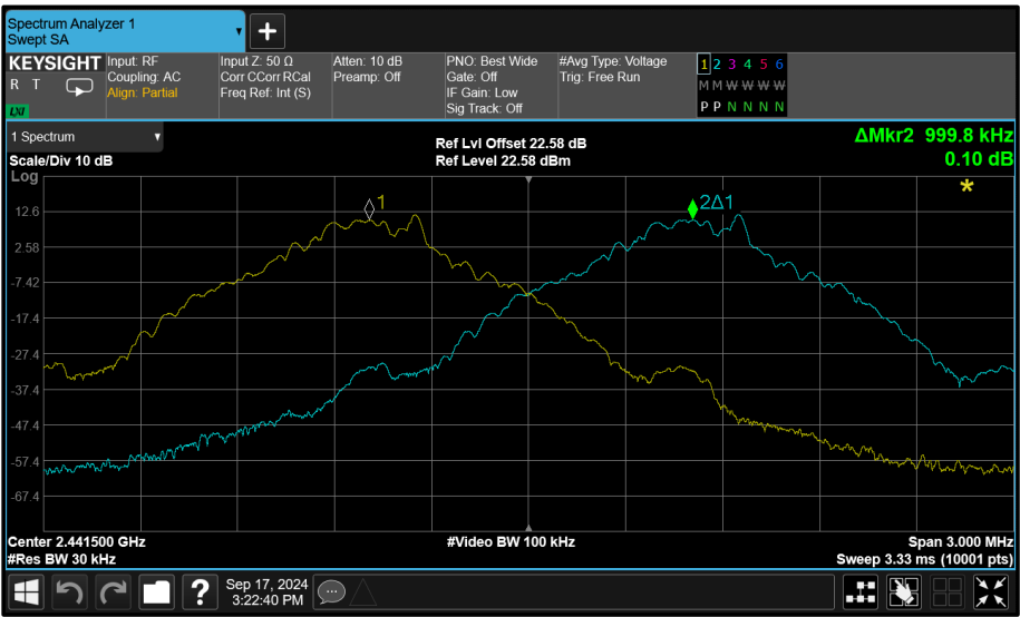
Figure 86 - GFSK - 2441 MHz (CH39)
