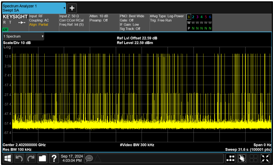
Figure 80 - 8-DPSK - 2402 MHz Accumulated Transmit Time
