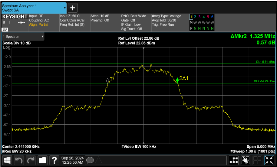
Figure 138 - Core 2 (C) 2441 MHz (CH39) 20 dB Bandwidth
