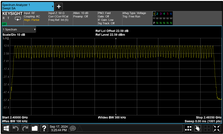
Figure 99 - GFSK (DH5) - Number of Hopping Channels
