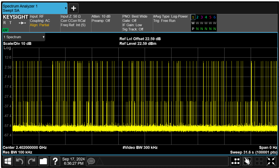
Figure 83 - 8-DPSK - 2402 MHz Accumulated Transmit Time
