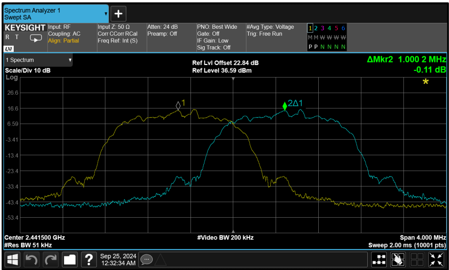
Figure 93 - 8-DPSK - 2441 MHz (CH39)
