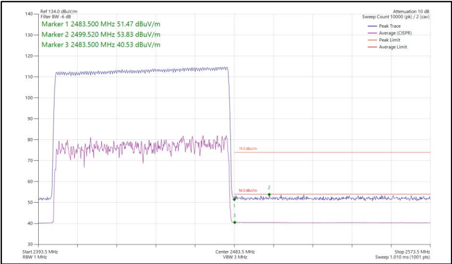
Figure 72 - Bluetooth 3DH5, MIMO, Core 0-1 - Hopping Band Edge Frequency 2483.5 MHz
