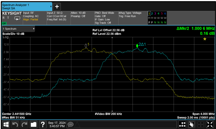
Figure 90 - \pi/4 DQPSK - 2441 MHz (CH39)
