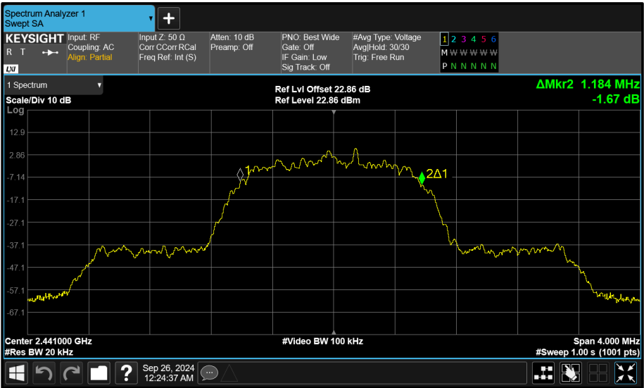
Figure 139 - Core 2 (C) 2441 MHz (CH39) 99% Bandwidth
