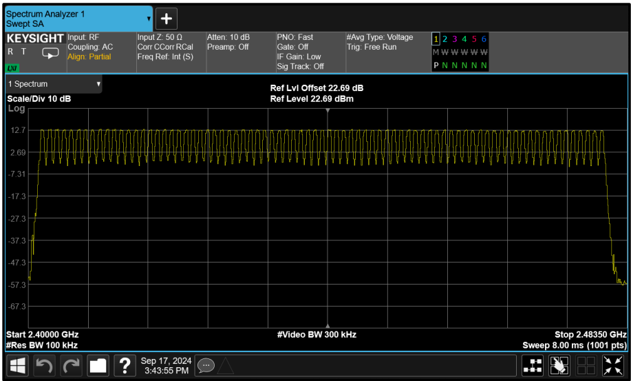
Figure 102 - GFSK (DH5) - Number of Hopping Channels
