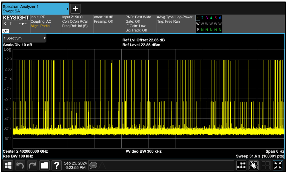
Figure 84 - \pi/4 DQPSK - 2402 MHz Accumulated Transmit Time
