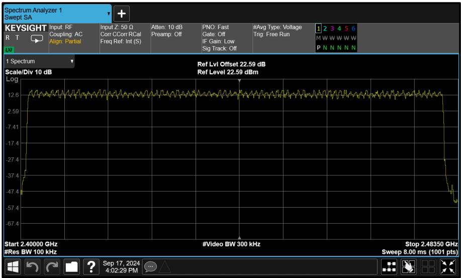
Figure 106 - 8-DPSK (3-DH5) - Number of Hopping Channels
