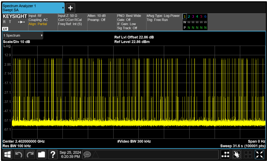
Figure 82 - \pi/4 DQPSK - 2402 MHz Accumulated Transmit Time
