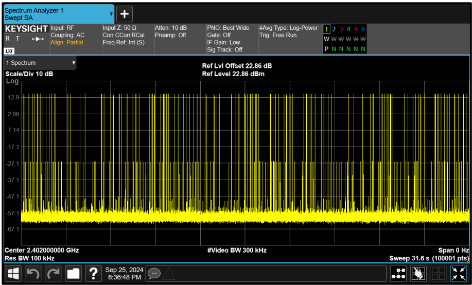
Figure 79 - \pi/4 DQPSK - 2402 MHz Accumulated Transmit Time
