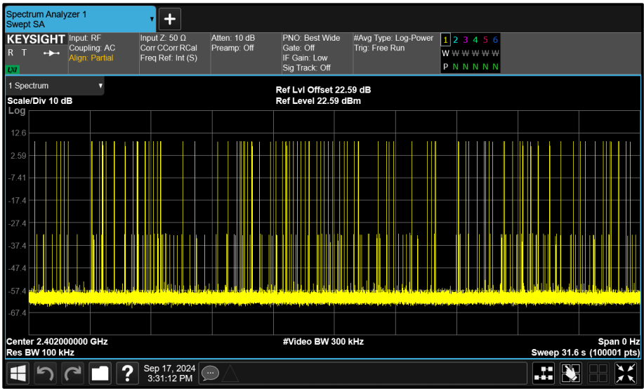
Figure 75 - 8-DPSK - 2402 MHz Accumulated Transmit Time
