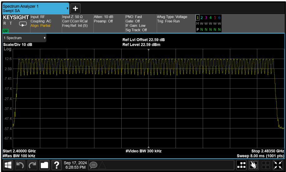
Figure 107 - GFSK (DH5) - Number of Hopping Channels
