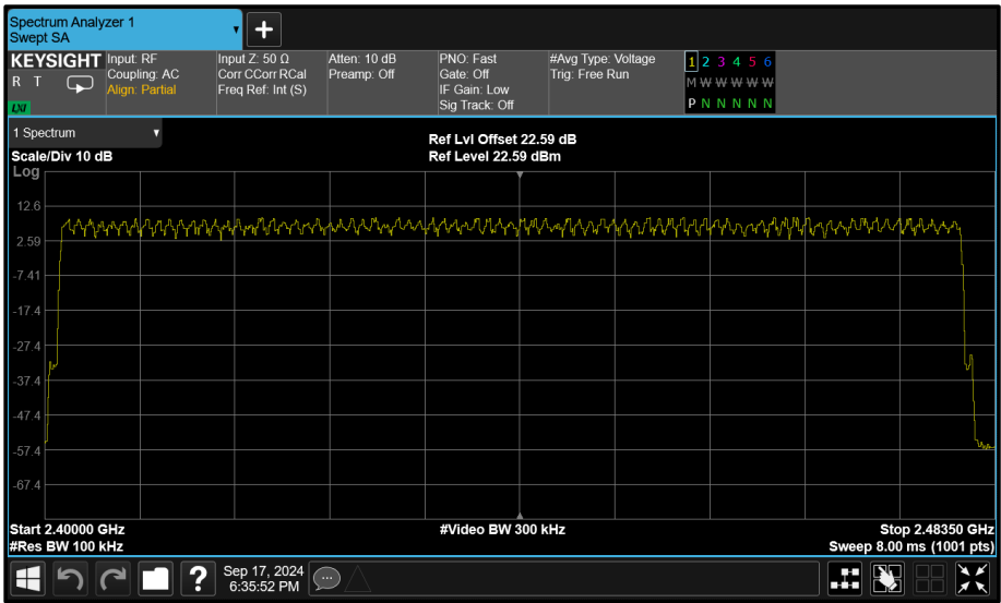
Figure 109 - 8-DPSK (3-DH5) - Number of Hopping Channels
