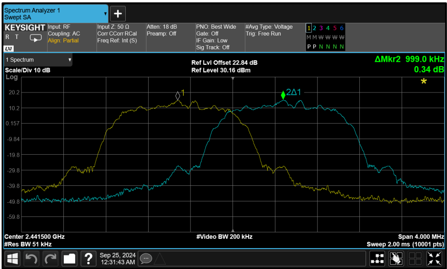
Figure 92 - \pi/4 DQPSK - 2441 MHz (CH39)
