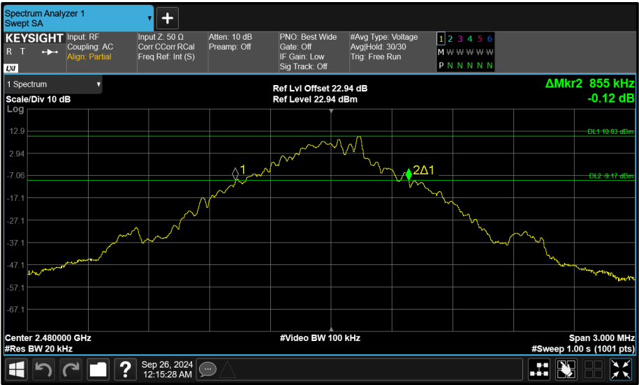
Figure 134 - Core 2 (C) 2480 MHz (CH78) 20 dB Bandwidth
