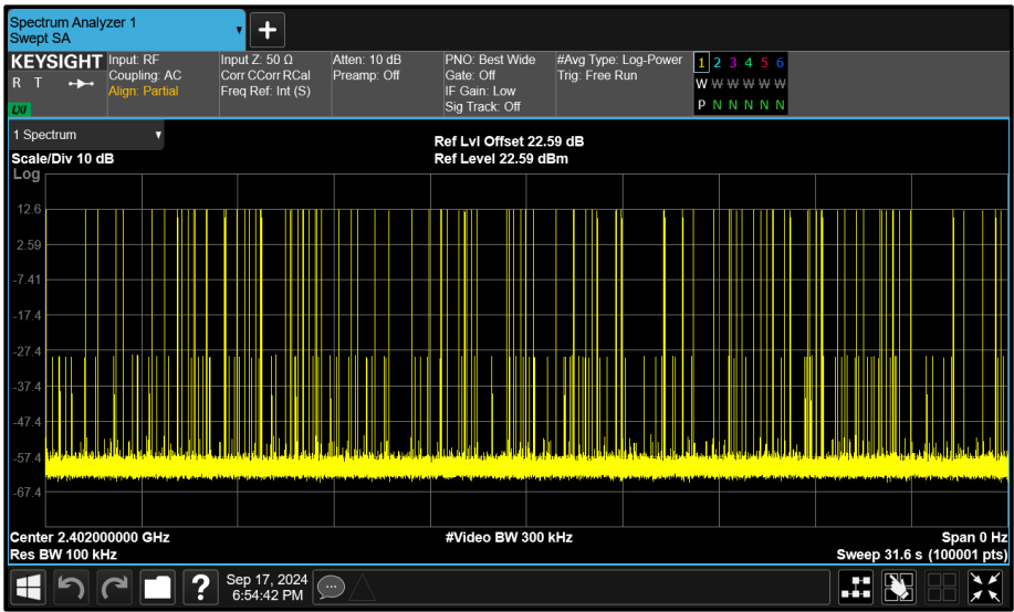
Figure 85 - 8-DPSK - 2402 MHz Accumulated Transmit Time
