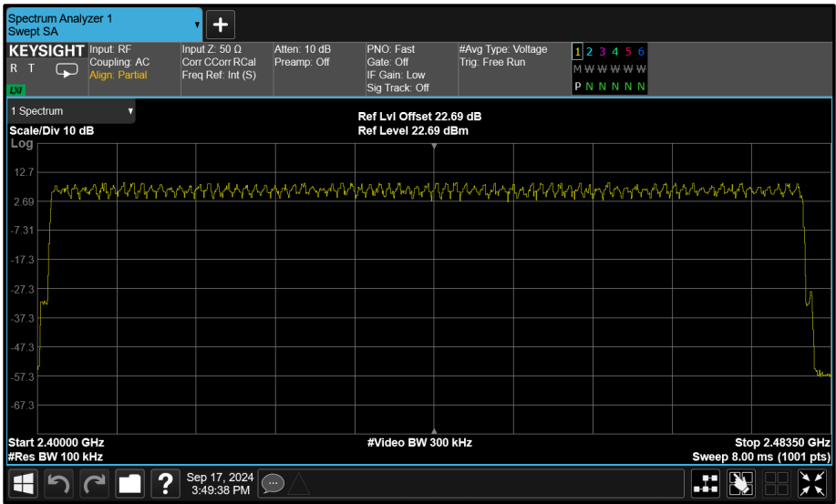
Figure 104 - 8-DPSK (3-DH5) - Number of Hopping Channels
