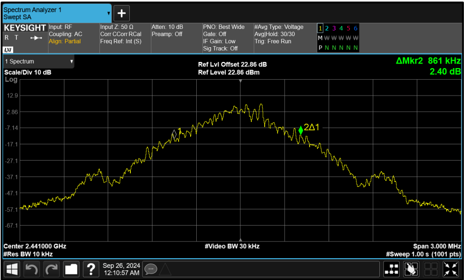
Figure 133 - Core 2 (C) 2441 MHz (CH39) 99% Bandwidth
