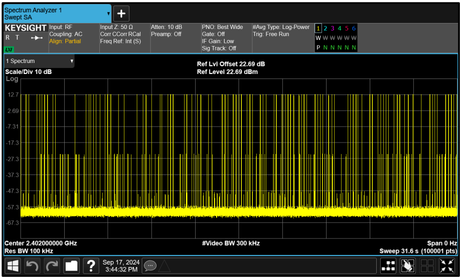
Figure 76 - GFSK - 2402 MHz Accumulated Transmit Time
