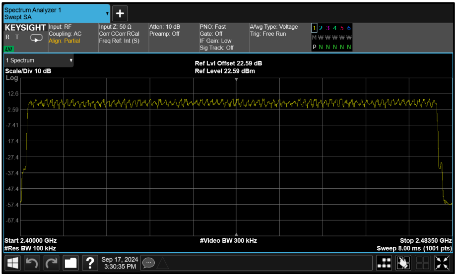
Figure 101 - 8-DPSK (3-DH5) - Number of Hopping Channels
