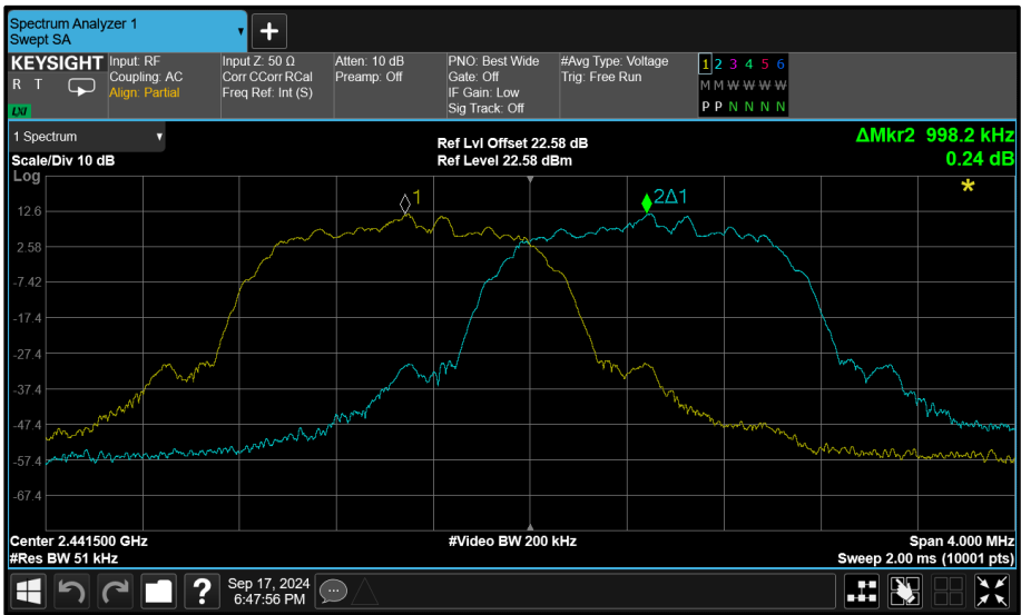
Figure 97 - \pi/4 DQPSK - 2441 MHz (CH39)
