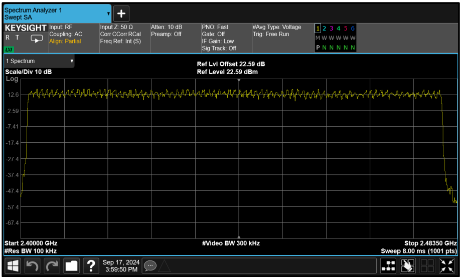
Figure 105 - \pi/4 DQPSK (2-DH5) - Number of Hopping Channels
