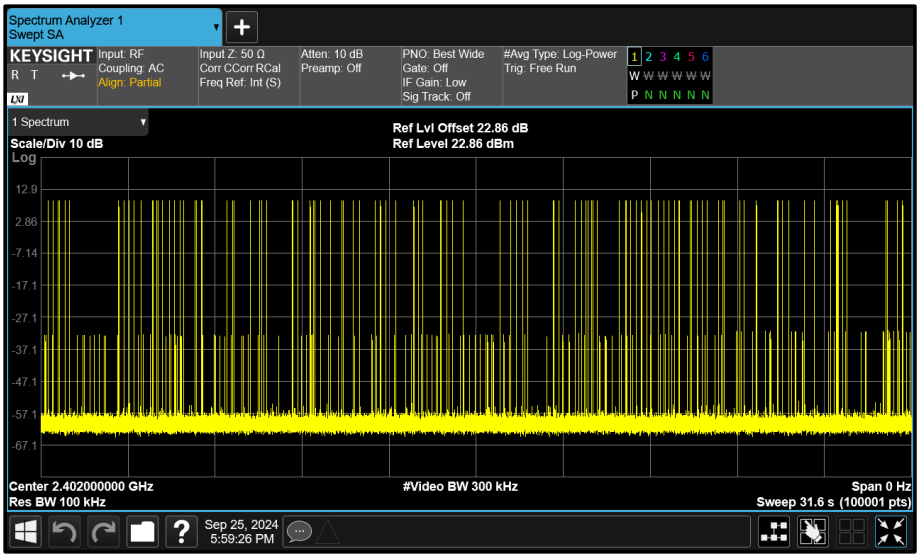
Figure 74 - \pi/4 DQPSK - 2402 MHz Accumulated Transmit Time
