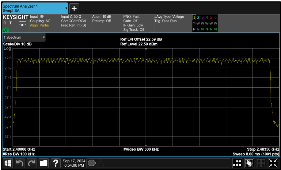
Figure 111 - 8-DPSK (3-DH5) - Number of Hopping Channels
