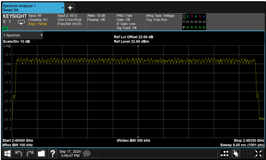
Figure 103 - \pi/4 DQPSK (2-DH5) - Number of Hopping Channels
