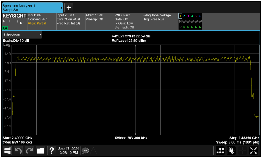
Figure 100 - \pi/4 DQPSK (2-DH5) - Number of Hopping Channels
