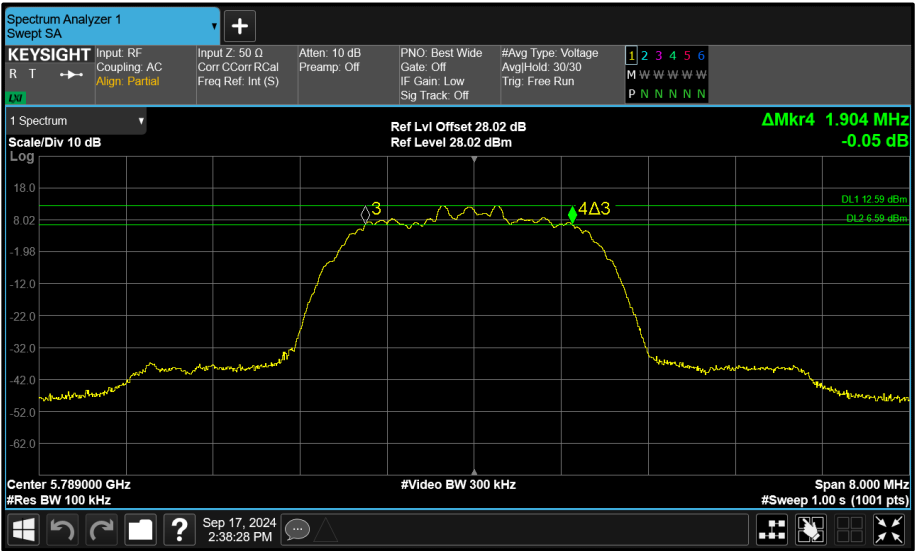
Figure 171 - Core 0 (A) 5789 MHz (CH64) 6 dB Bandwidth
