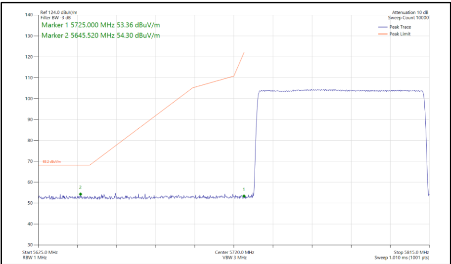
Figure 194 - Bluetooth HDR4, SISO, Core 0 - 5733-5811 MHz Band Edge Frequency 5725 MHz
