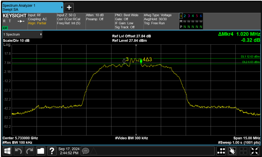
Figure 179 - Core 0 (A) 5733 MHz (CH8) 6 dB Bandwidth
