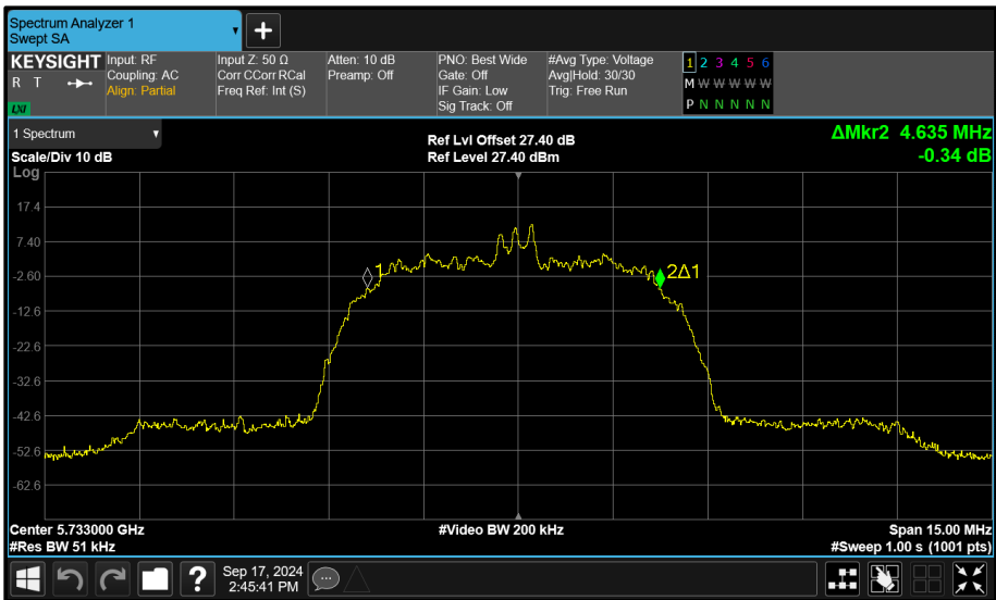
Figure 180 - Core 1 (B) 5733 MHz (CH8) 99% Bandwidth
