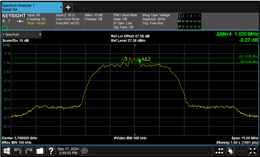
Figure 185 - Core 1 (B) 5789 MHz (CH64) 6 dB Bandwidth
