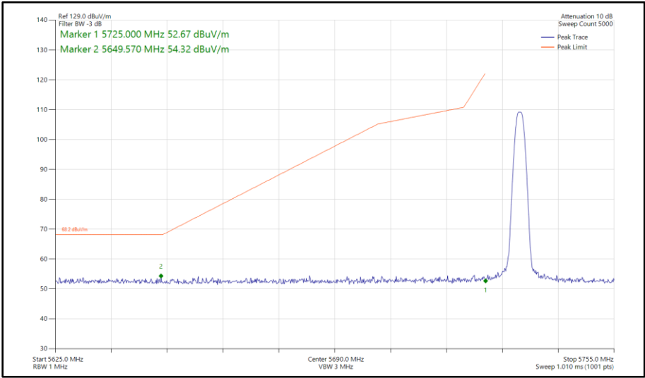
Figure 190 - Bluetooth DH5, SISO, Core 0 - 5733 MHz Band Edge Frequency 5725 MHz
