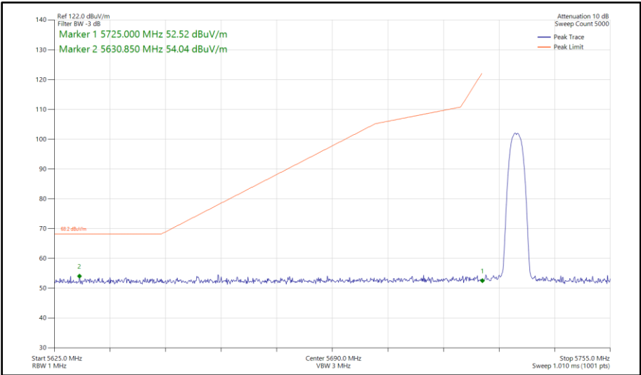
Figure 203 - Bluetooth HDR4, SISO, Core 1 - 5733 MHz Band Edge Frequency 5725 MHz
