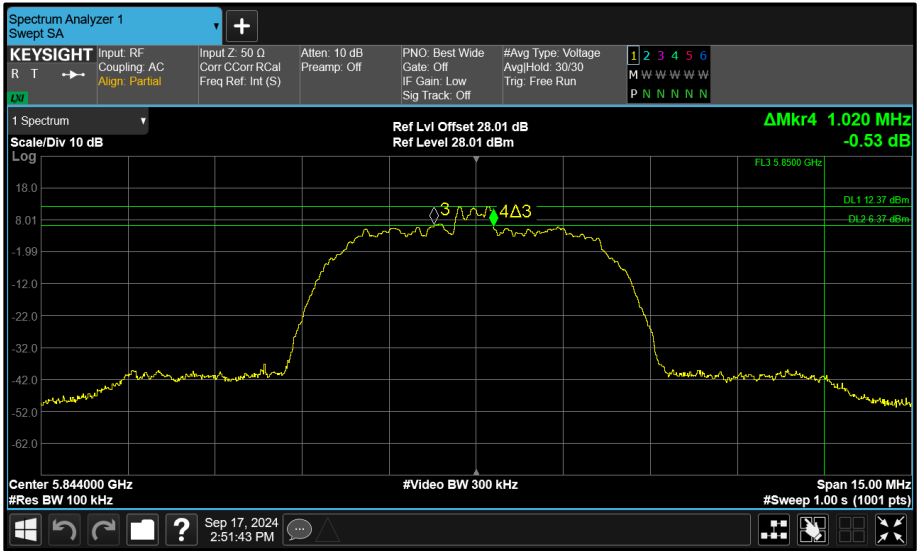
Figure 187 - Core 0 (A) 5844 MHz (CH119) 6 dB Bandwidth
