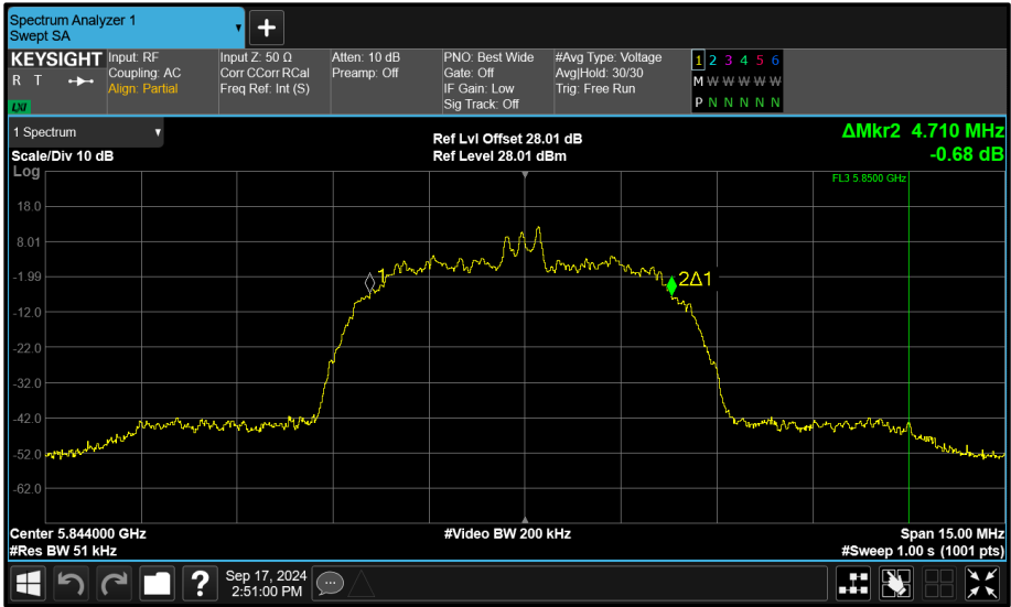
Figure 186 - Core 0 (A) 5844 MHz (CH119) 99% Bandwidth
