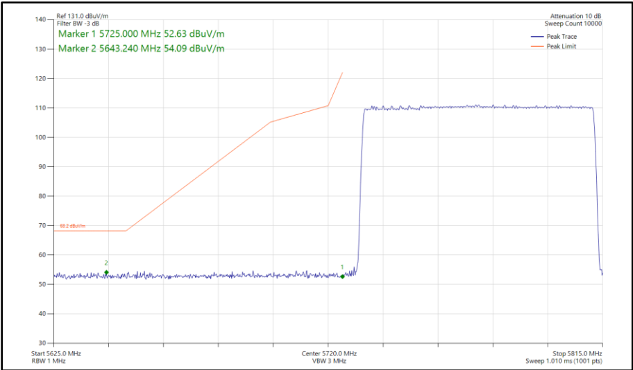
Figure 193 - Bluetooth DH5, SISO, Core 0 - 5733-5811 MHz Band Edge Frequency 5725 MHz
