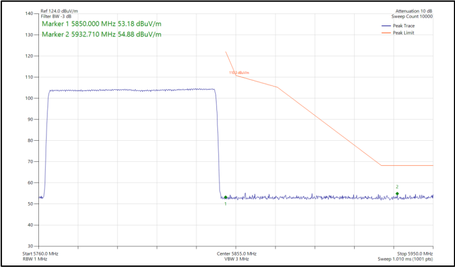
Figure 200 - Bluetooth HDR4, SISO, Core 0 - 5766-5844 MHz Band Edge Frequency 5850 MHz
