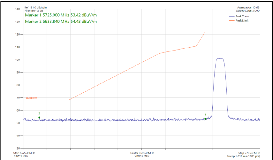
Figure 204 - Bluetooth HDR8, SISO, Core 1 - 5733 MHz Band Edge Frequency 5725 MHz
