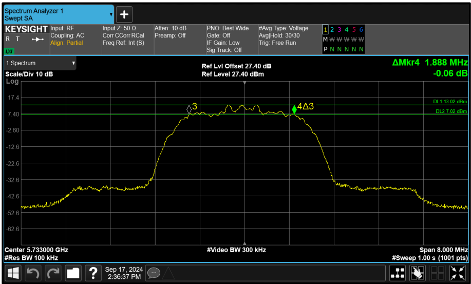
Figure 169 - Core 1 (B) 5733 MHz (CH8) 6 dB Bandwidth
