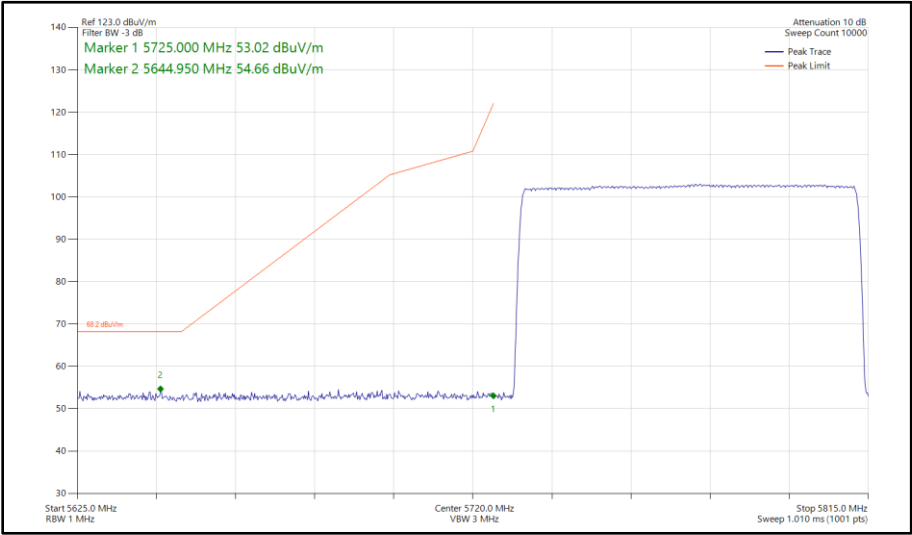
Figure 206 - Bluetooth HDR4, SISO, Core 1 - 5733-5811 MHz Band Edge Frequency 5725 MHz
