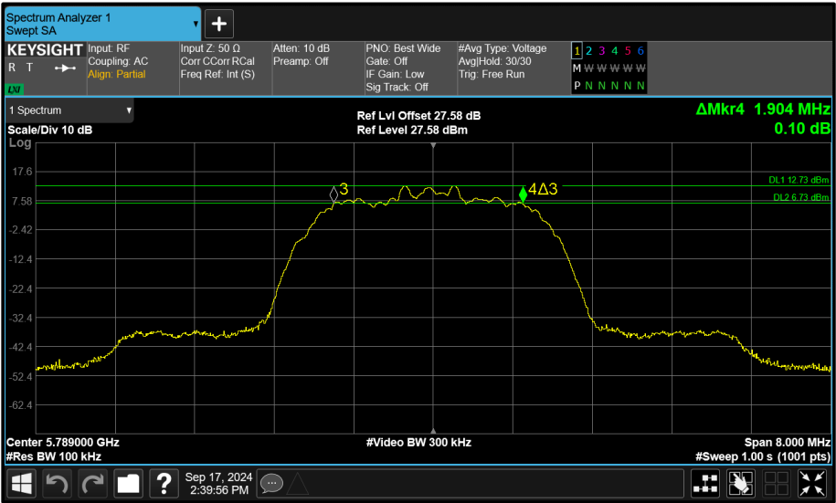
Figure 173 - Core 1 (B) 5789 MHz (CH64) 6 dB Bandwidth
