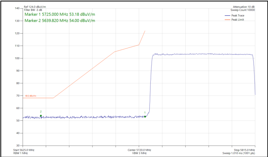
Figure 195 - Bluetooth HDR8, SISO, Core 0 - 5733-5811 MHz Band Edge Frequency 5725 MHz
