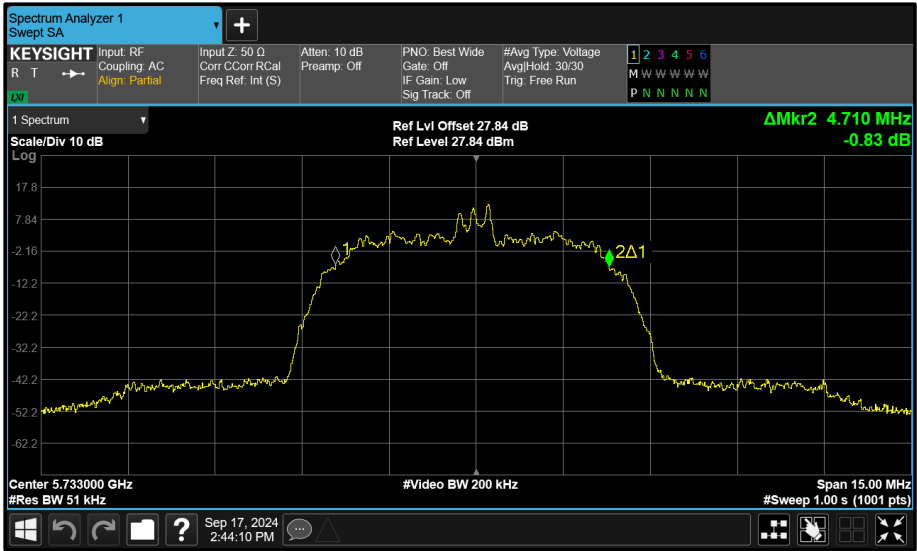
Figure 178 - Core 0 (A) 5733 MHz (CH8) 99% Bandwidth
