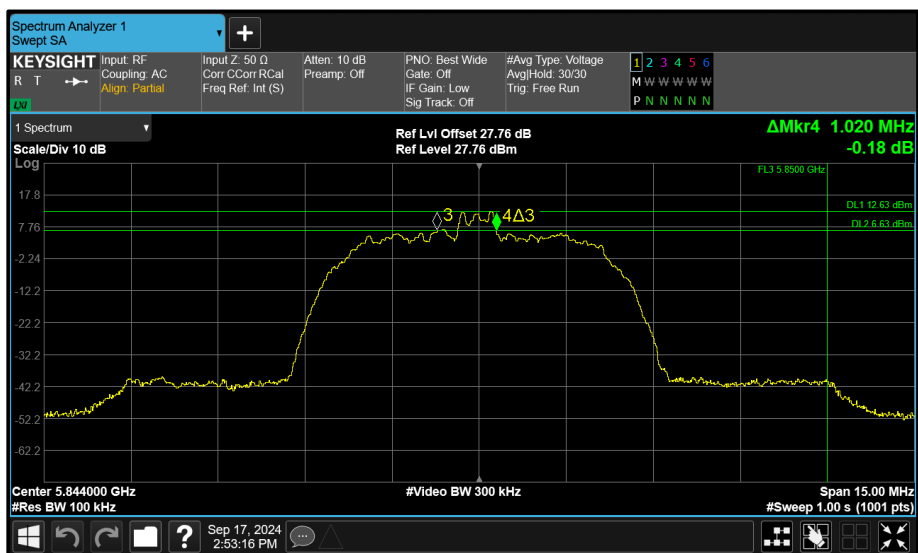
Figure 189 - Core 1 (B) 5844 MHz (CH119) 6 dB Bandwidth
