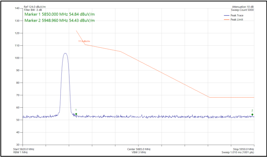
Figure 197 - Bluetooth HDR4, SISO, Core 0 - 5844 MHz Band Edge Frequency 5850 MHz
