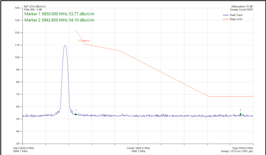
Figure 196 - Bluetooth DH5, SISO, Core 0 - 5844 MHz Band Edge Frequency 5850 MHz
