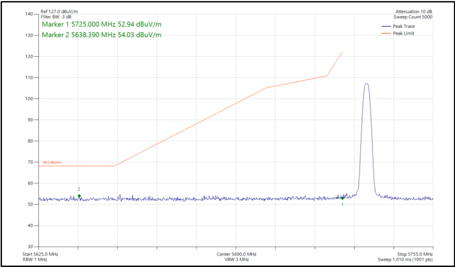
Figure 202 - Bluetooth DH5, SISO, Core 1 - 5733 MHz Band Edge Frequency 5725 MHz
