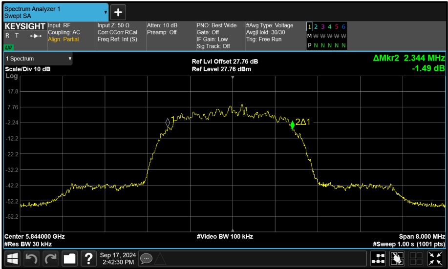
Figure 176 - Core 1 (B) 5844 MHz (CH119) 99% Bandwidth
