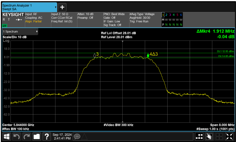
Figure 175 - Core 0 (A) 5844 MHz (CH119) 6 dB Bandwidth
