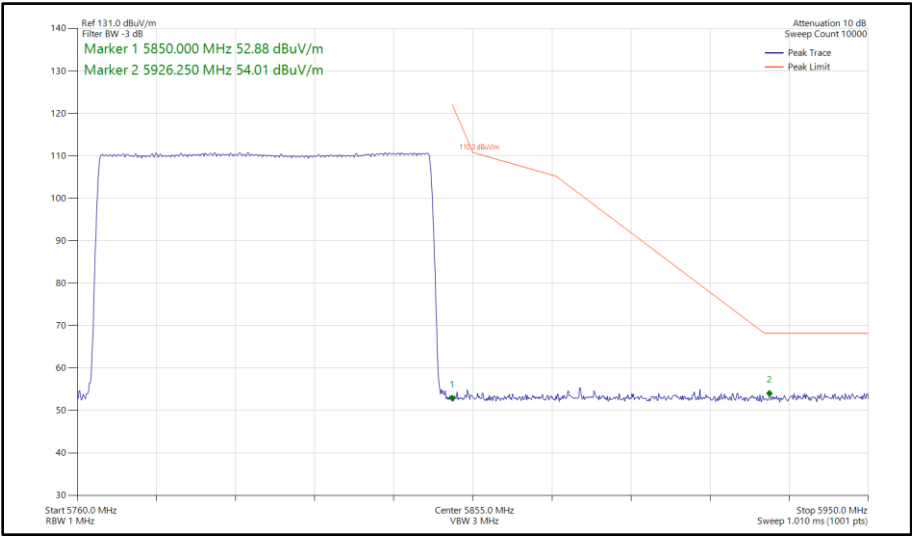
Figure 199 - Bluetooth DH5, SISO, Core 0 - 5766-5844 MHz Band Edge Frequency 5850 MHz
