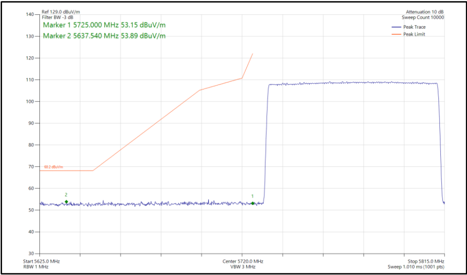
Figure 205 - Bluetooth DH5, SISO, Core 1 - 5733-5811 MHz Band Edge Frequency 5725 MHz
