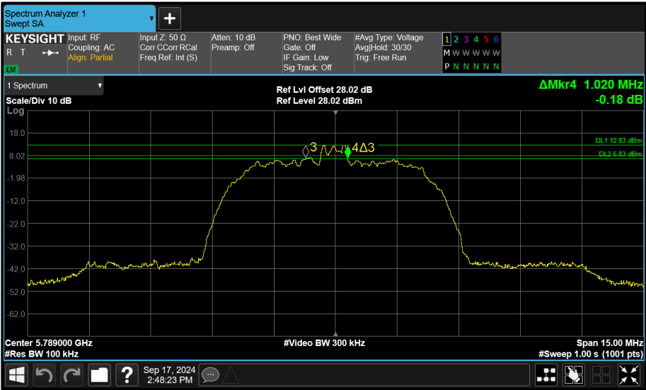
Figure 183 - Core 0 (A) 5789 MHz (CH64) 6 dB Bandwidth
