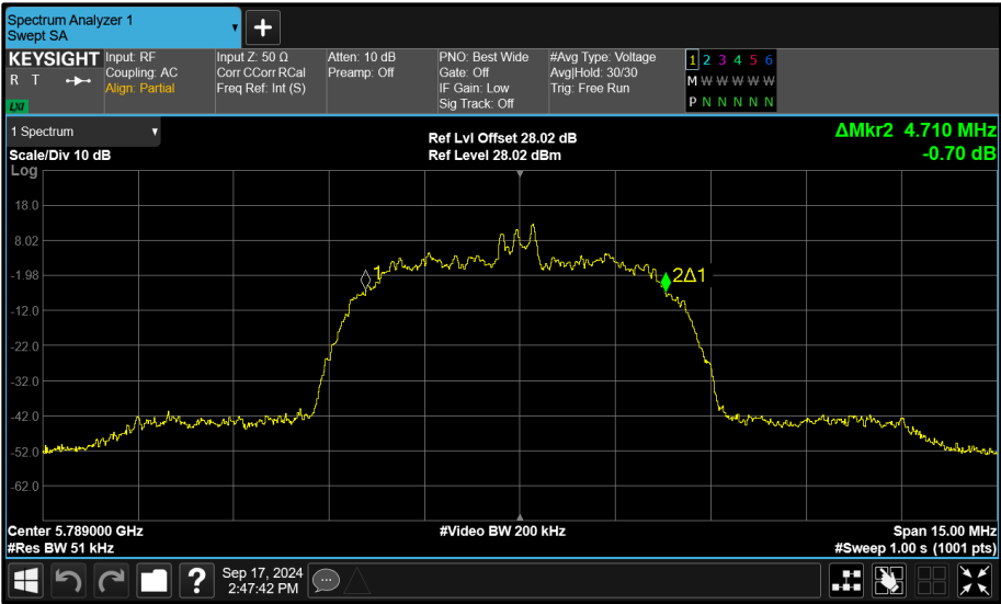
Figure 182 - Core 0 (A) 5789 MHz (CH64) 99% Bandwidth
