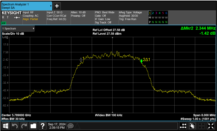
Figure 172 - Core 1 (B) 5789 MHz (CH64) 99% Bandwidth
