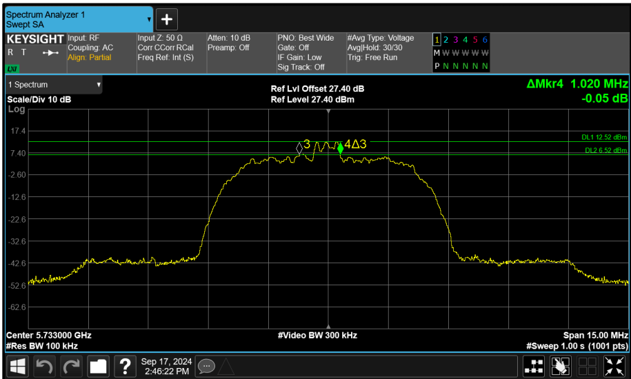
Figure 181 - Core 1 (B) 5733 MHz (CH8) 6 dB Bandwidth
