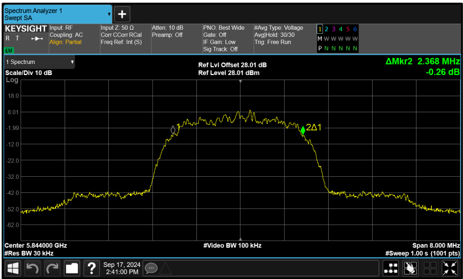
Figure 174 - Core 0 (A) 5844 MHz (CH119) 99% Bandwidth
