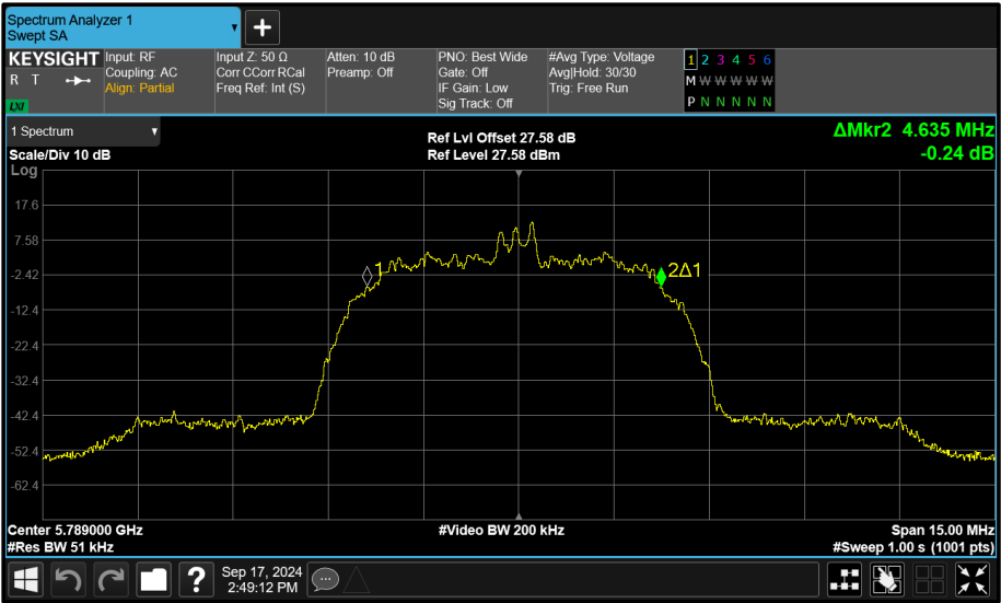
Figure 184 - Core 1 (B) 5789 MHz (CH64) 99% Bandwidth
