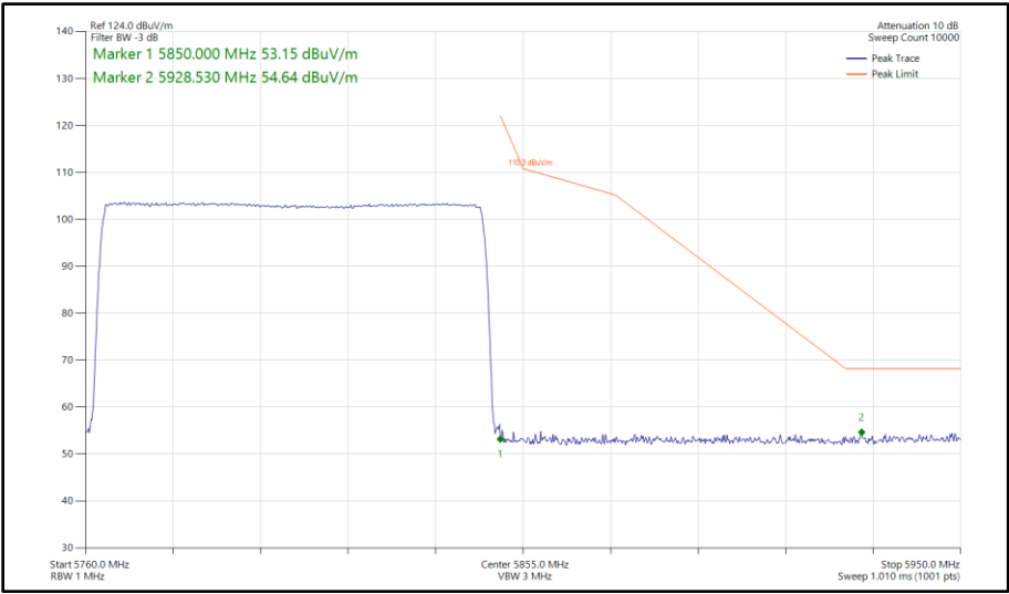
Figure 201 - Bluetooth HDR8, SISO, Core 0 - 5766-5844 MHz Band Edge Frequency 5850 MHz
