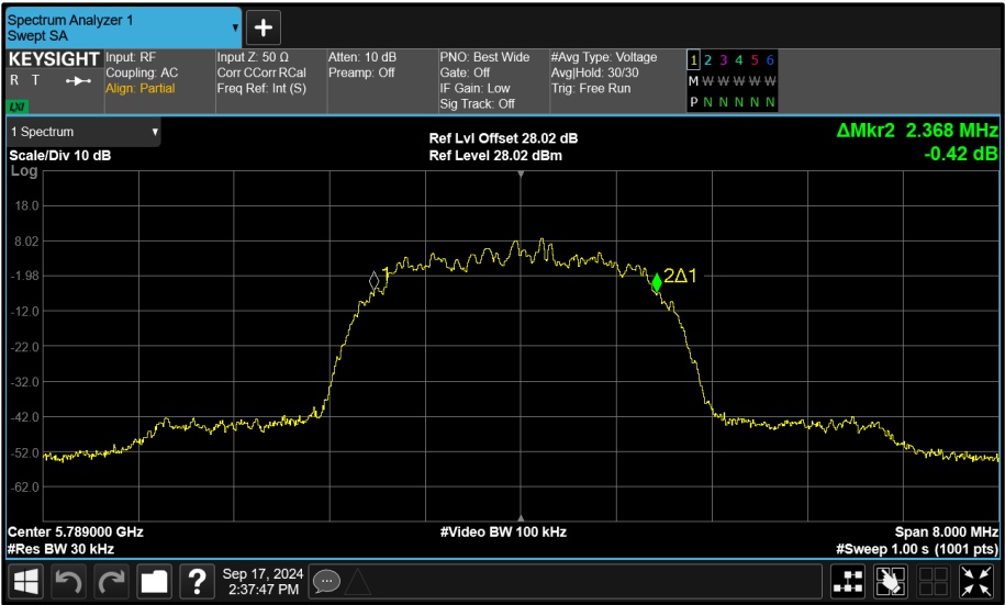
Figure 170 - Core 0 (A) 5789 MHz (CH64) 99% Bandwidth
