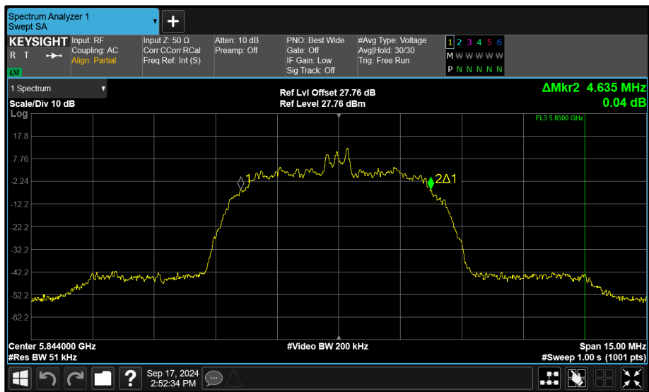
Figure 188 - Core 1 (B) 5844 MHz (CH119) 99% Bandwidth
