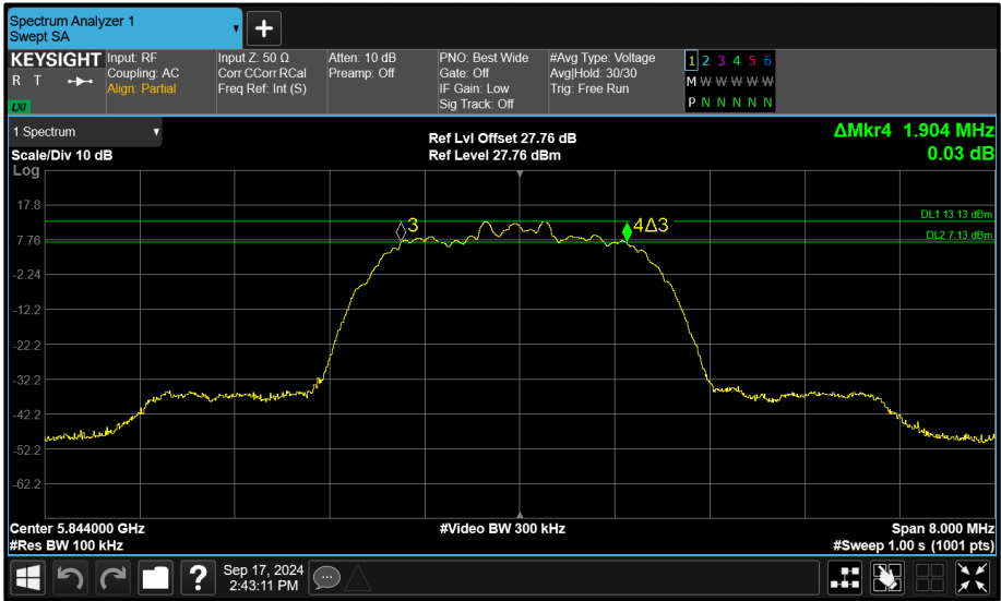
Figure 177 - Core 1 (B) 5844 MHz (CH119) 6 dB Bandwidth
