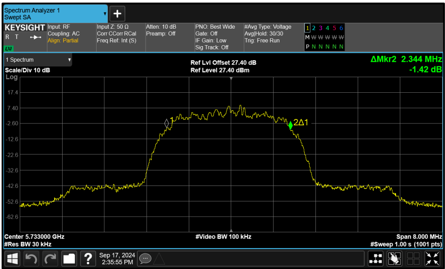
Figure 168 - Core 1 (B) 5733 MHz (CH8) 99% Bandwidth
