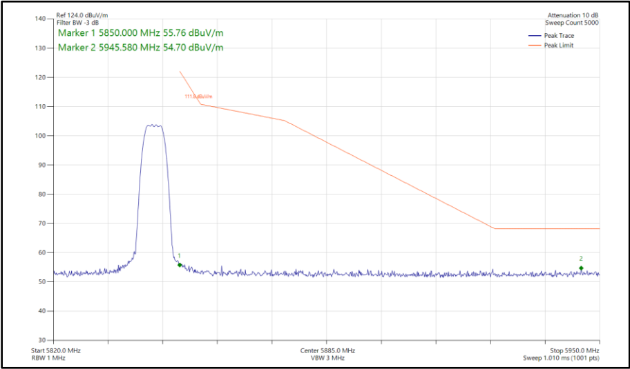
Figure 198 - Bluetooth HDR8, SISO, Core 0 - 5844 MHz Band Edge Frequency 5850 MHz
