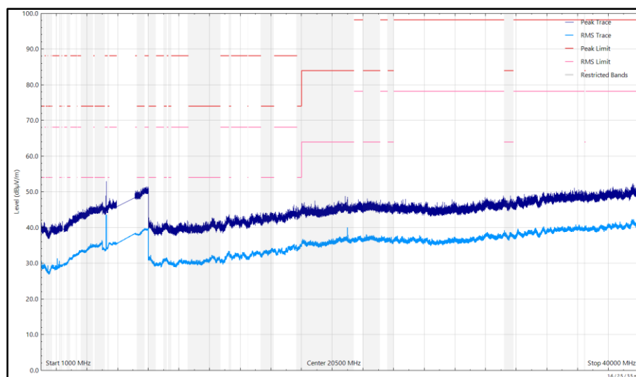
Figure 39 - 6995 MHz (CH209), HE20, SU, CDD, Core 0 + Core 1 and 2441 MHz (CH39), DH5, iPA, Core 2, 1 GHz to 40 GHz, Horizontal
