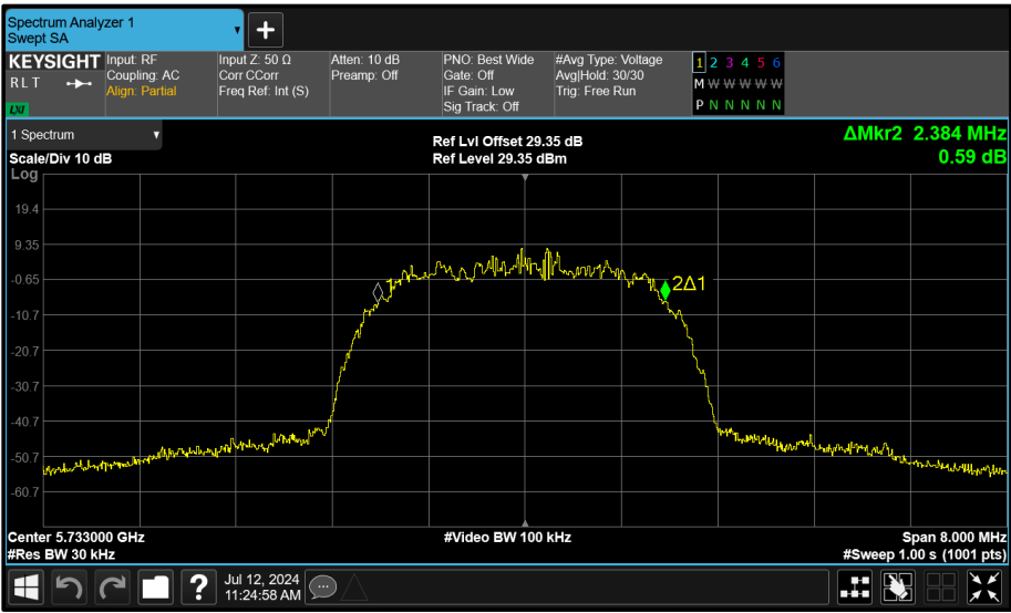
Figure 142 - Core 0 (A) 5733 MHz (CH8) 99% Bandwidth
