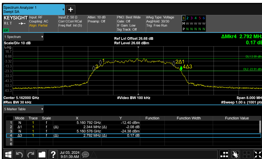
Figure 131 - Core 1 (B) 5162 MHz (CH12) 26 dB and 99% Bandwidth
