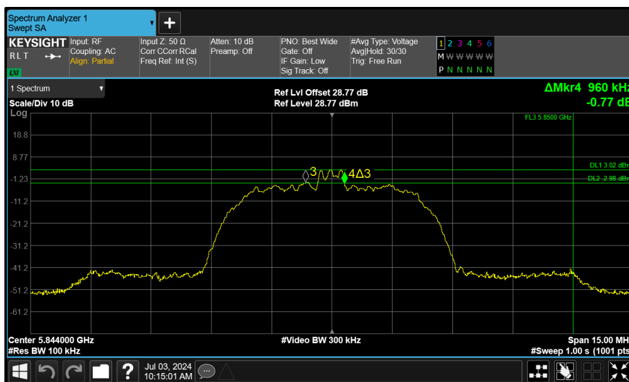
Figure 127 - Core 0 (A) 5844 MHz (CH119) 6 dB Bandwidth
