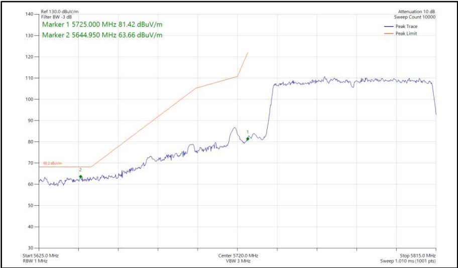
Figure 526 - 802.11ac VHT80, SISO, Core 0 - 5775 MHz Band Edge Frequency 5725 MHz
