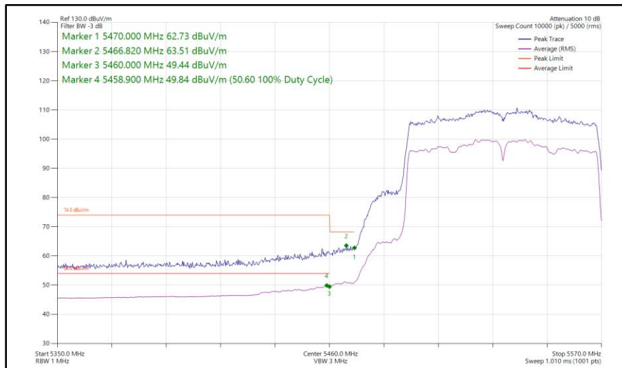
Figure 553 - 802.11ac VHT80, CDD, Core 0 - Core 1 - 5530 MHz Band Edge Frequency 5470 MHz
