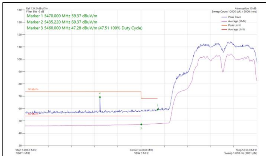
Figure 516 - 802.11ac VHT40, TxBF, Core 0 - Core 1 - 5510 MHz Band Edge Frequency 5470 MHz
