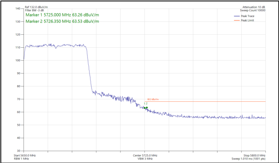
Figure 508 - 802.11ax HE40, SU, SDM, Core 0 - Core 1 - 5670 MHz Band Edge Frequency 5725 MHz
