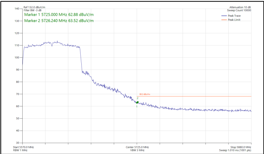
Figure 544 - 802.11ac VHT80, SISO, Core 1 - 5610 MHz Band Edge Frequency 5725 MHz
