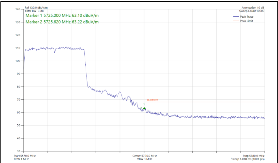
Figure 559 - 802.11ac VHT80, CDD, Core 0 - Core 1 - 5610 MHz Band Edge Frequency 5725 MHz
