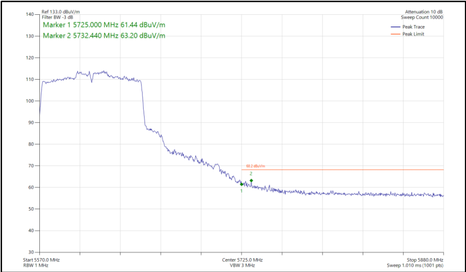
Figure 574 - 802.11ac VHT80, SDM, Core 0 - Core 1 - 5610 MHz Band Edge Frequency 5725 MHz
