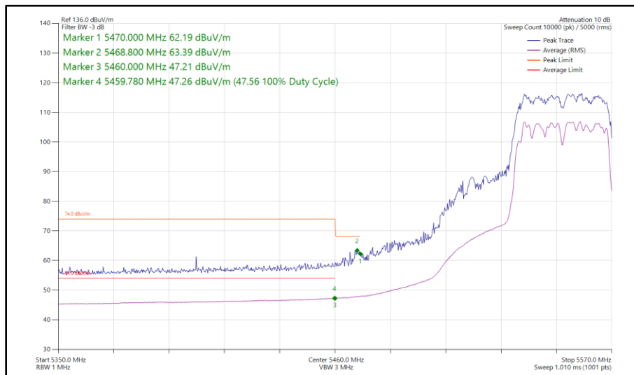
Figure 517 - 802.11ac VHT40, TxBF, Core 0 - Core 1 - 5550 MHz Band Edge Frequency 5470 MHz
