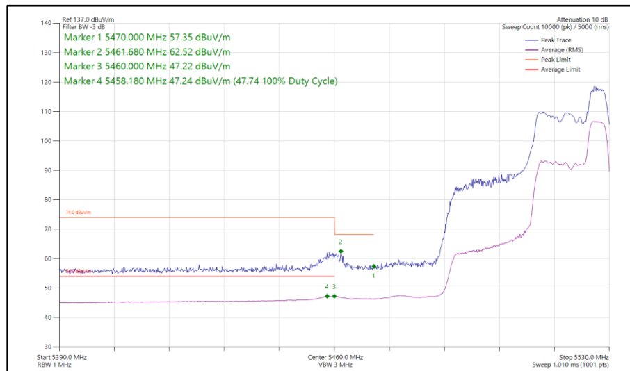
Figure 498 - 802.11ax HE40, RU 52-44, SDM, Core 0 - Core 1 - 5510 MHz Band Edge Frequency 5470 MHz
