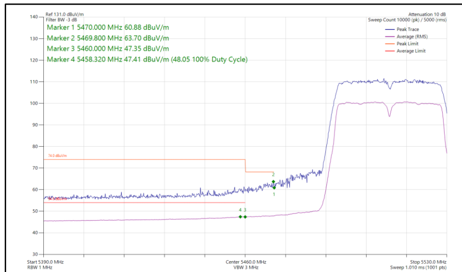
Figure 494 - 802.11n HT40, SDM, Core 0 - Core 1 - 5510 MHz Band Edge Frequency 5470 MHz
