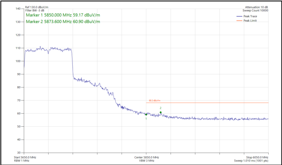
Figure 532 - 802.11ac VHT80, SISO, Core 0 - 5690 MHz Band Edge Frequency 5850 MHz
