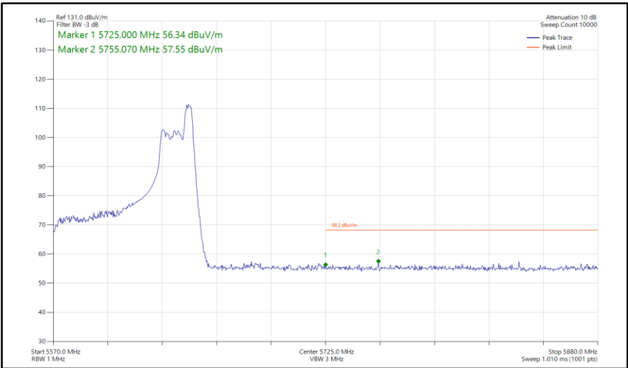
Figure 531 - 802.11ax HE80, RU 52-52, SISO, Core 0 - 5610 MHz Band Edge Frequency 5725 MHz
