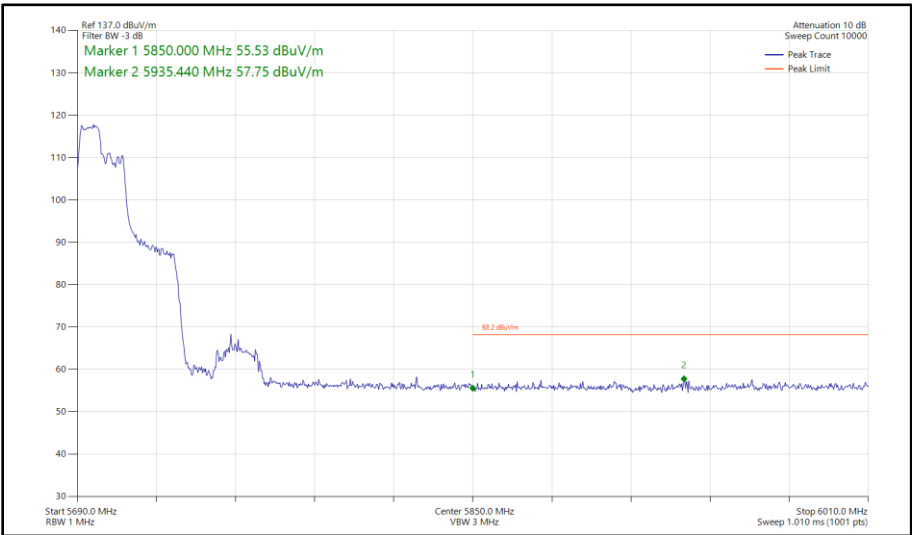
Figure 513 - 802.11ax HE40, RU 106-53, SDM, Core 0 - Core 1 - 5710 MHz Band Edge Frequency 5850 MHz
