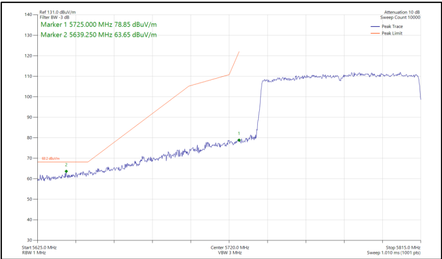
Figure 542 - 802.11ax HE80, SU, SISO, Core 1 - 5775 MHz Band Edge Frequency 5725 MHz
