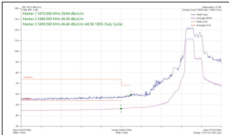
Figure 500 - 802.11ax HE40, RU 106-53, SDM, Core 0 - Core 1 - 5550 MHz Band Edge Frequency 5470 MHz
