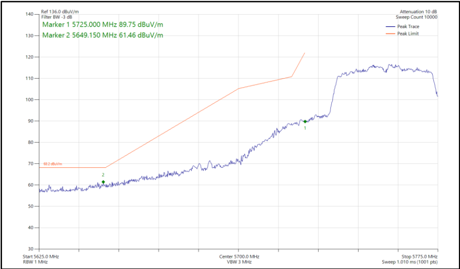
Figure 502 - 802.11n HT40, SDM, Core 0 - Core 1 - 5755 MHz Band Edge Frequency 5725 MHz
