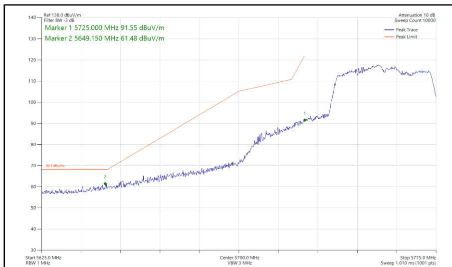
Figure 518 - 802.11ac VHT40, TxBF, Core 0 - Core 1 - 5755 MHz Band Edge Frequency 5725 MHz
