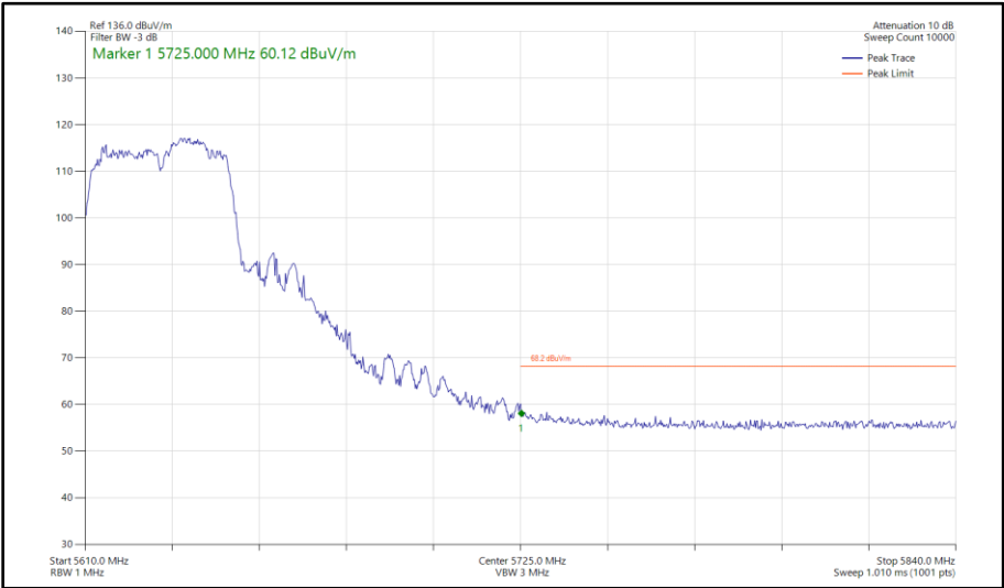
Figure 519 - 802.11ac VHT40, TxBF, Core 0 - Core 1 - 5630 MHz Band Edge Frequency 5725 MHz
