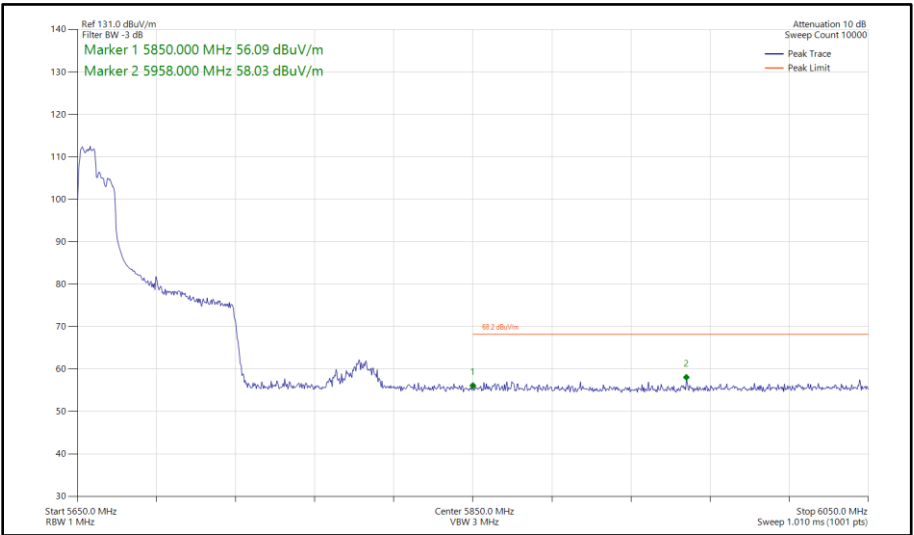
Figure 535 - 802.11ax HE80, RU 106-53, SISO, Core 0 - 5690 MHz Band Edge Frequency 5850 MHz
