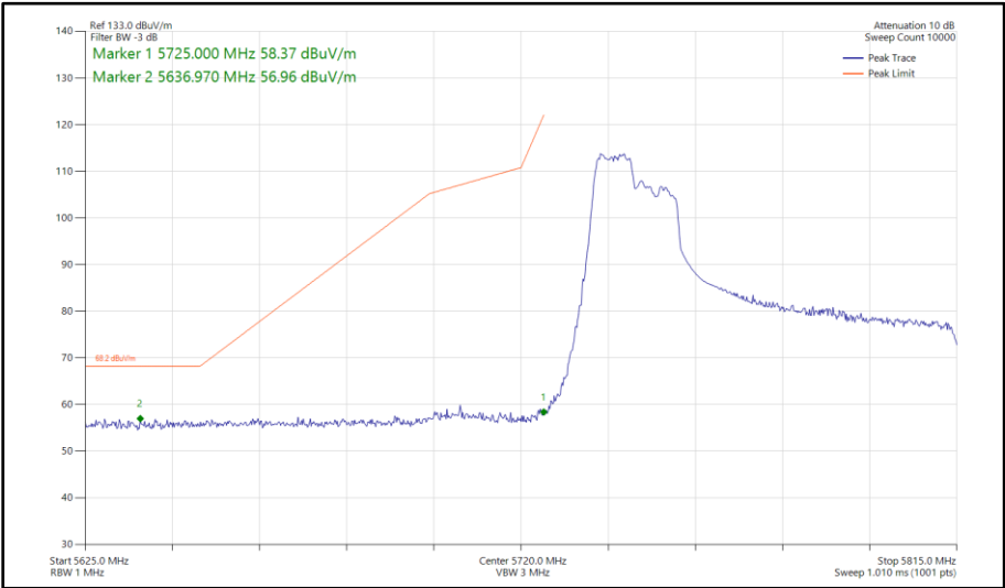
Figure 543 - 802.11ax HE80, RU 106-53, SISO, Core 1 - 5775 MHz Band Edge Frequency 5725 MHz
