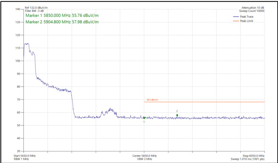
Figure 565 - 802.11ax HE80, RU 106-53, CDD, Core 0 - Core 1 - 5690 MHz Band Edge Frequency 5850 MHz
