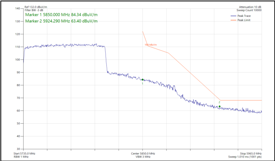
Figure 536 - 802.11ax HE80, SU, SISO, Core 0 - 5775 MHz Band Edge Frequency 5850 MHz
