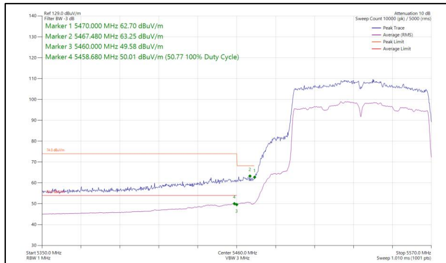
Figure 523 - 802.11ac VHT80, SISO, Core 0 - 5530 MHz Band Edge Frequency 5470 MHz
