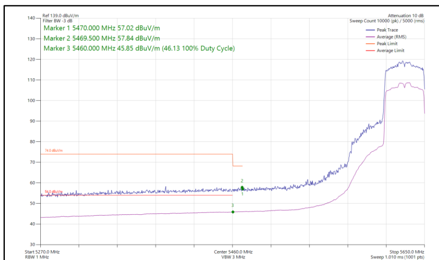
Figure 501 - 802.11ax HE40, SU, SDM, Core 0 - Core 1 - 5630 MHz Band Edge Frequency 5470 MHz
