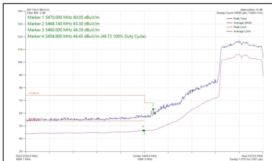
Figure 499 - 802.11ax HE40, SU, SDM, Core 0 - Core 1 - 5550 MHz Band Edge Frequency 5470 MHz
