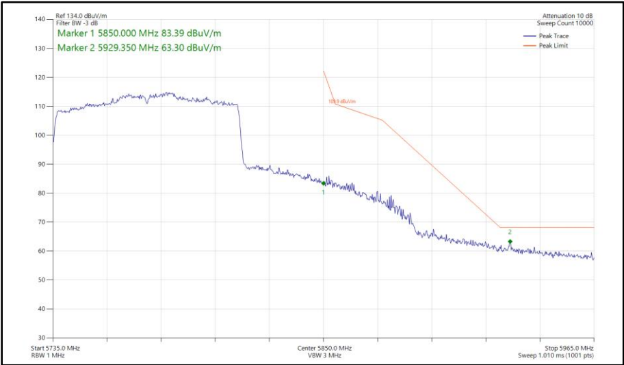
Figure 551 - 802.11ax HE80, SU, SISO, Core 1 - 5775 MHz Band Edge Frequency 5850 MHz
