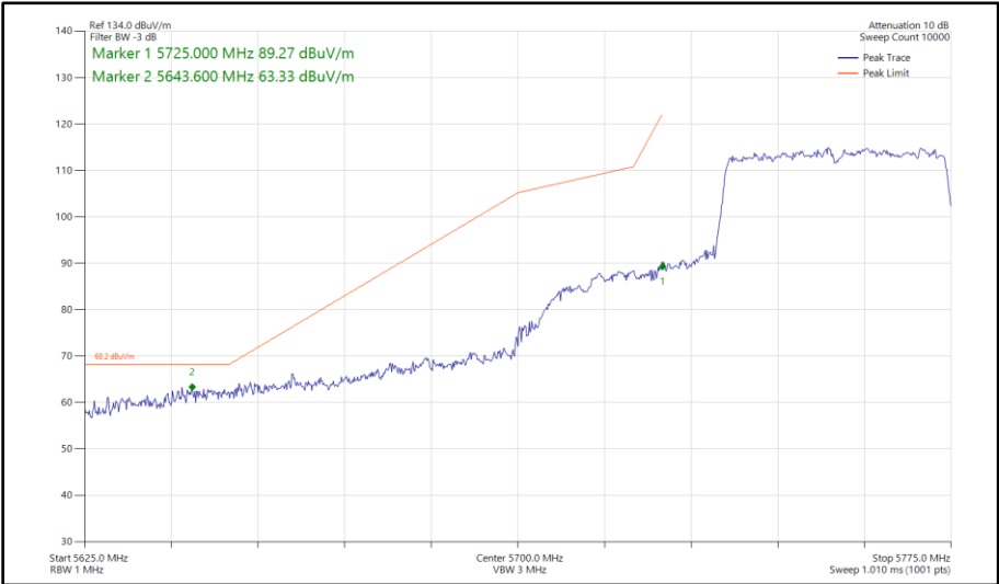
Figure 503 - 802.11ax HE40, SU, SDM, Core 0 - Core 1 - 5755 MHz Band Edge Frequency 5725 MHz
