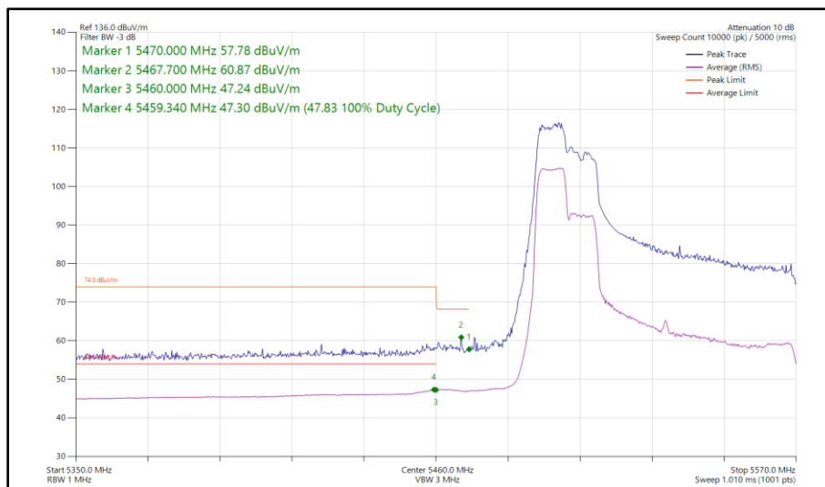
Figure 540 - 802.11ax HE80, RU 106-53, SISO, Core 1 - 5530 MHz Band Edge Frequency 5470 MHz
