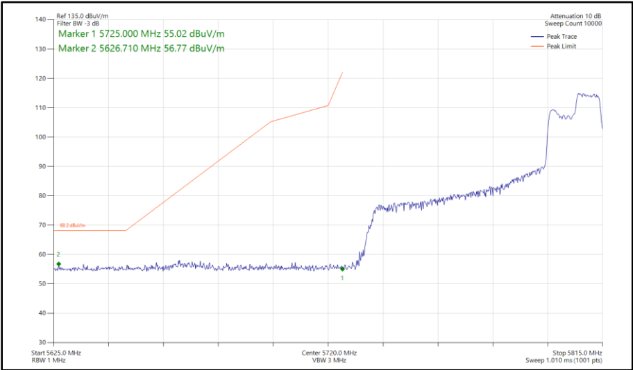
Figure 558 - 802.11ax HE80, RU 106-60, CDD, Core 0 - Core 1 - 5775 MHz Band Edge Frequency 5725 MHz
