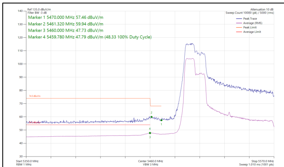
Figure 570 - 802.11ax HE80, RU 106-53, SDM, Core 0 - Core 1 - 5530 MHz Band Edge Frequency 5470 MHz
