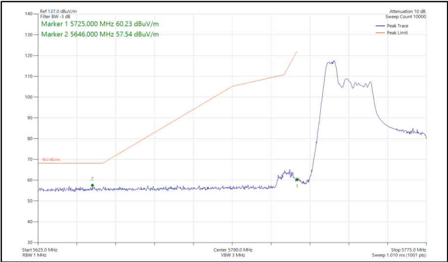
Figure 504 - 802.11ax HE40, RU 52-37, SDM, Core 0 - Core 1 - 5755 MHz Band Edge Frequency 5725 MHz
