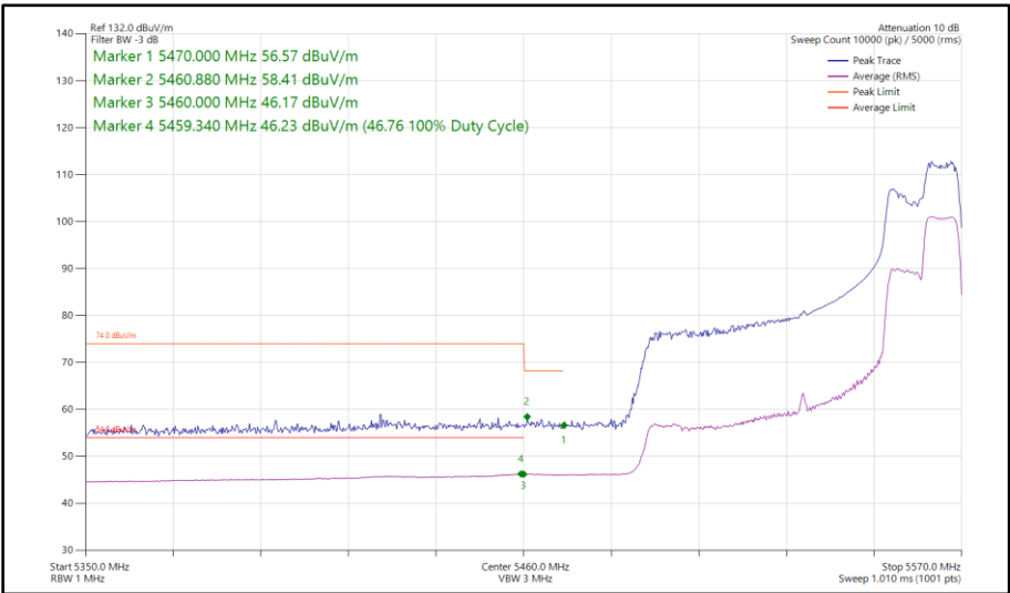
Figure 525 - 802.11ax HE80, RU 106-60, SISO, Core 0 - 5530 MHz Band Edge Frequency 5470 MHz
