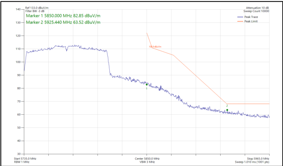
Figure 533 - 802.11ac VHT80, SISO, Core 0 - 5775 MHz Band Edge Frequency 5850 MHz
