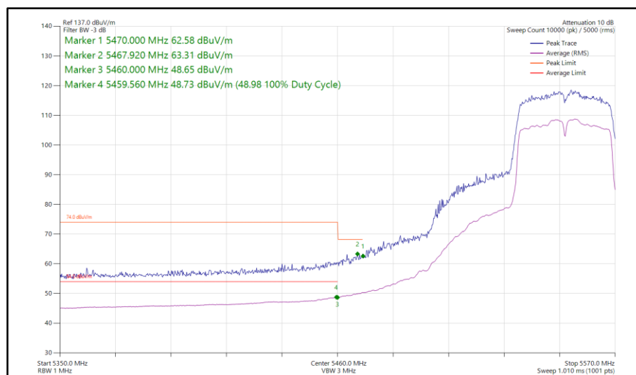
Figure 495 - 802.11n HT40, SDM, Core 0 - Core 1 - 5550 MHz Band Edge Frequency 5470 MHz
