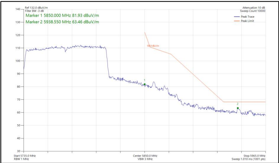
Figure 563 - 802.11ac VHT80, CDD, Core 0 - Core 1 - 5775 MHz Band Edge Frequency 5850 MHz
