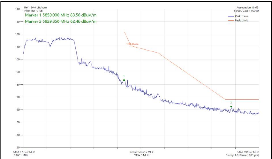
Figure 522 - 802.11ac VHT40, TxBF, Core 0 - Core 1 - 5795 MHz Band Edge Frequency 5850 MHz
