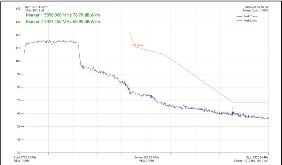
Figure 514 - 802.11ax HE40, SU, SDM, Core 0 - Core 1 - 5795 MHz Band Edge Frequency 5850 MHz
