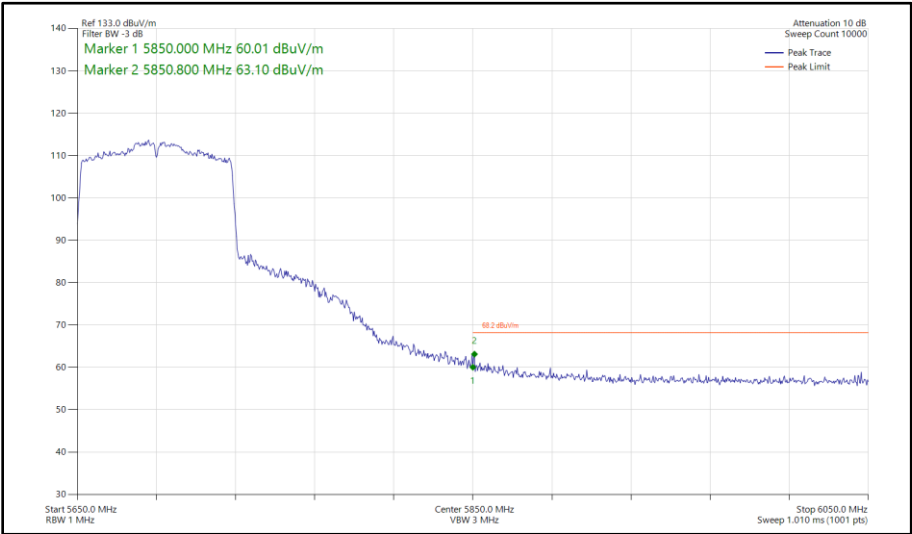
Figure 547 - 802.11ac VHT80, SISO, Core 1 - 5690 MHz Band Edge Frequency 5850 MHz
