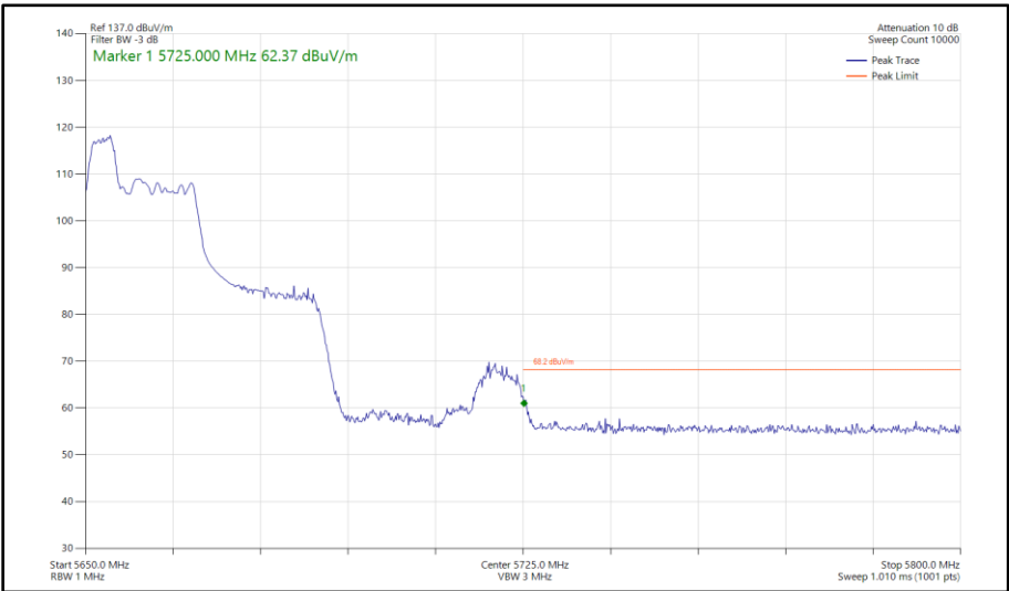
Figure 509 - 802.11ax HE40, RU 52-37, SDM, Core 0 - Core 1 - 5670 MHz Band Edge Frequency 5725 MHz
