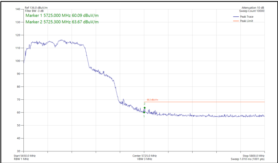
Figure 520 - 802.11ac VHT40, TxBF, Core 0 - Core 1 - 5670 MHz Band Edge Frequency 5725 MHz
