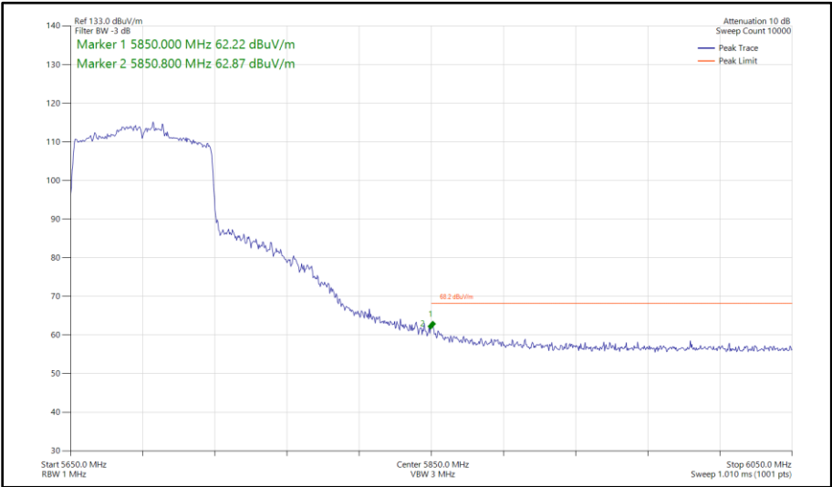
Figure 562 - 802.11ac VHT80, CDD, Core 0 - Core 1 - 5690 MHz Band Edge Frequency 5850 MHz
