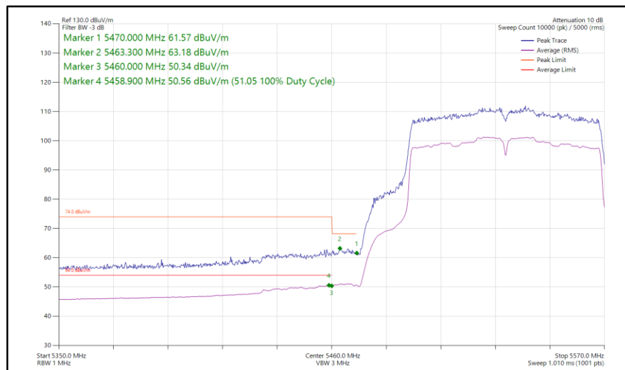
Figure 538 - 802.11ac VHT80, SISO, Core 1 - 5530 MHz Band Edge Frequency 5470 MHz
