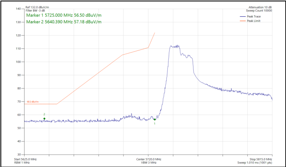
Figure 528 - 802.11ax HE80, RU 106-53, SISO, Core 0 - 5775 MHz Band Edge Frequency 5725 MHz
