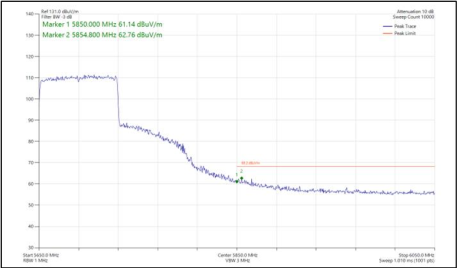
Figure 534 - 802.11ax HE80, SU, SISO, Core 0 - 5690 MHz Band Edge Frequency 5850 MHz
