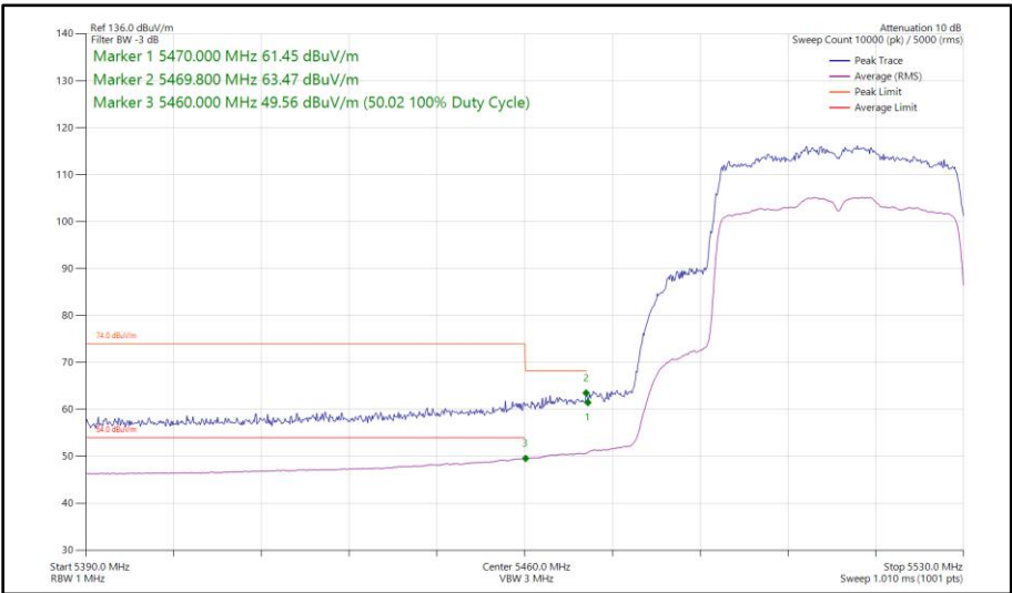
Figure 497 - 802.11ax HE40, SU, SDM, Core 0 - Core 1 - 5510 MHz Band Edge Frequency 5470 MHz
