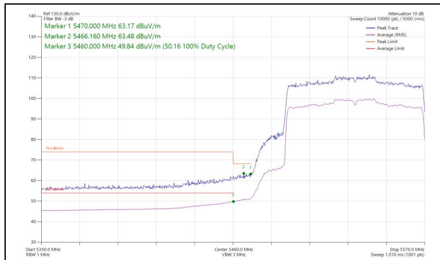
Figure 554 - 802.11ax HE80, SU, CDD, Core 0 - Core 1 - 5530 MHz Band Edge Frequency 5470 MHz
