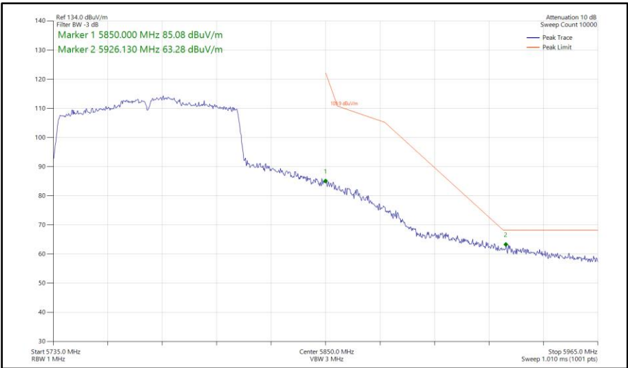
Figure 548 - 802.11ac VHT80, SISO, Core 1 - 5775 MHz Band Edge Frequency 5850 MHz
