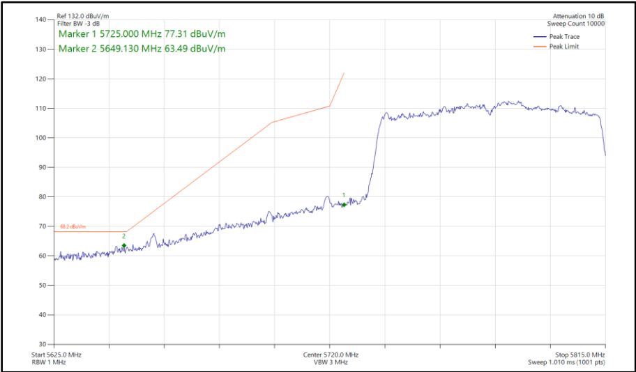
Figure 571 - 802.11ac VHT80, SDM, Core 0 - Core 1 - 5775 MHz Band Edge Frequency 5725 MHz
