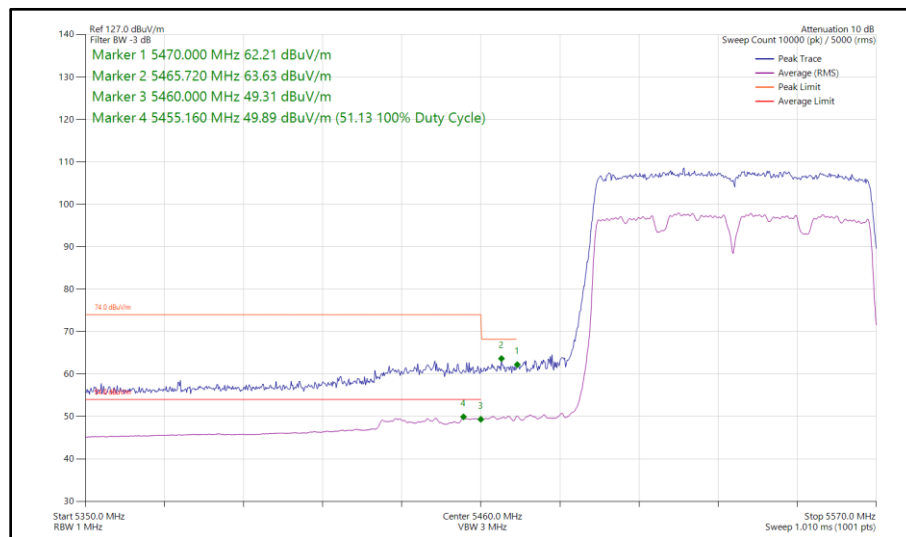
Figure 568 - 802.11ac VHT80, SDM, Core 0 - Core 1 - 5530 MHz Band Edge Frequency 5470 MHz
