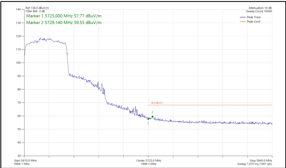
Figure 507 - 802.11ax HE40, SU, SDM, Core 0 - Core 1 - 5630 MHz Band Edge Frequency 5725 MHz
