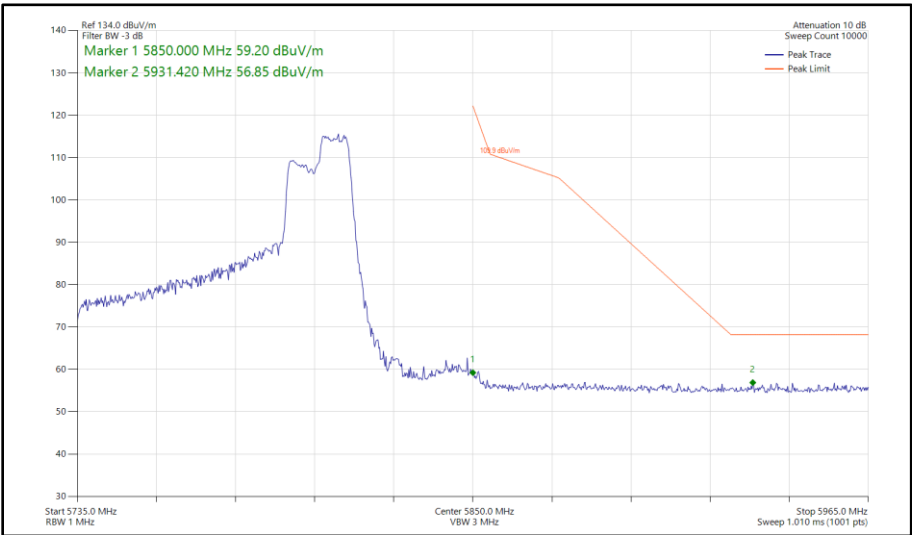
Figure 567 - 802.11ax HE80, RU 106-60, CDD, Core 0 - Core 1 - 5775 MHz Band Edge Frequency 5850 MHz
