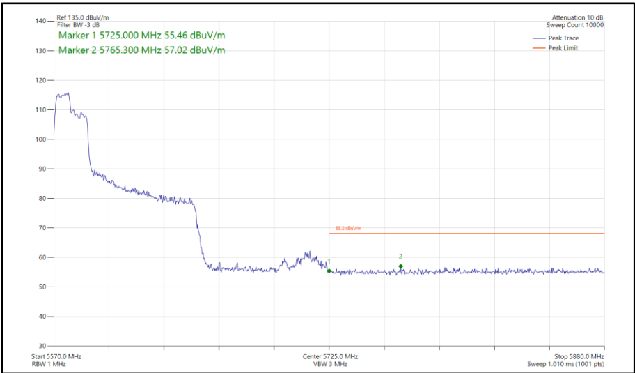
Figure 561 - 802.11ax HE80, RU 106-53, CDD, Core 0 - Core 1 - 5610 MHz Band Edge Frequency 5725 MHz
