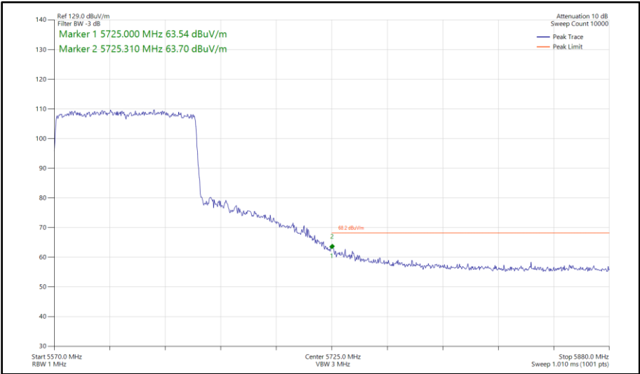
Figure 530 - 802.11ax HE80, SU, SISO, Core 0 - 5610 MHz Band Edge Frequency 5725 MHz
