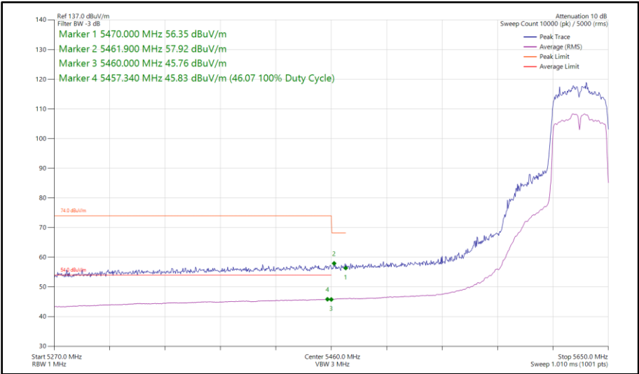
Figure 496 - 802.11n HT40, SDM, Core 0 - Core 1 - 5630 MHz Band Edge Frequency 5470 MHz
