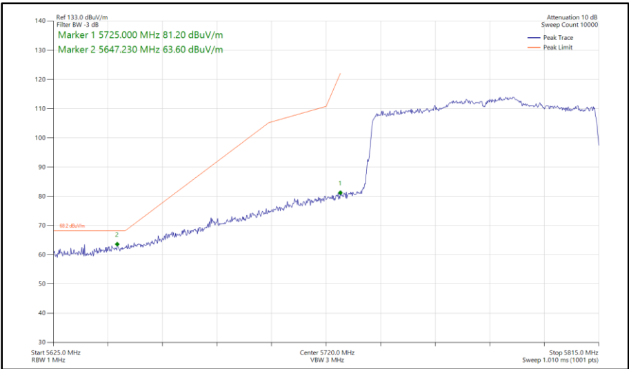
Figure 572 - 802.11ax HE80, SU, SDM, Core 0 - Core 1 - 5775 MHz Band Edge Frequency 5725 MHz
