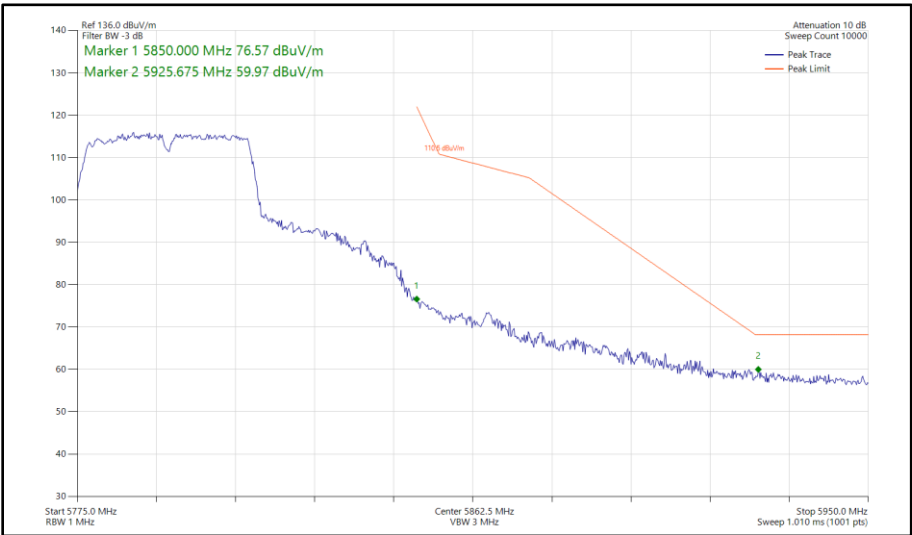
Figure 511 - 802.11n HT40, SDM, Core 0 - Core 1 - 5795 MHz Band Edge Frequency 5850 MHz
