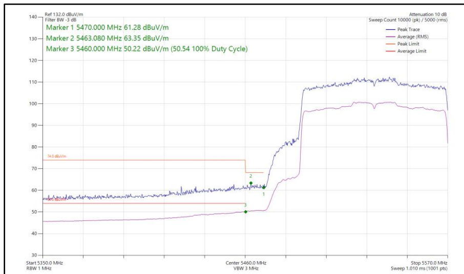
Figure 539 - 802.11ax HE80, SU, SISO, Core 1 - 5530 MHz Band Edge Frequency 5470 MHz
