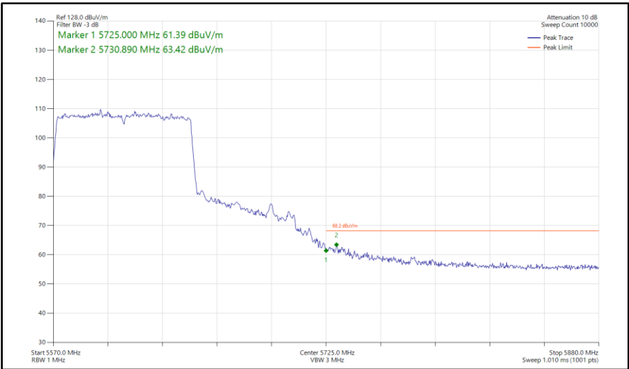
Figure 529 - 802.11ac VHT80, SISO, Core 0 - 5610 MHz Band Edge Frequency 5725 MHz
