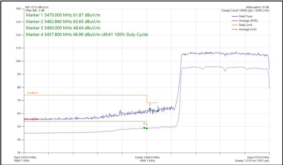
Figure 524 - 802.11ax HE80, SU, SISO, Core 0 - 5530 MHz Band Edge Frequency 5470 MHz
