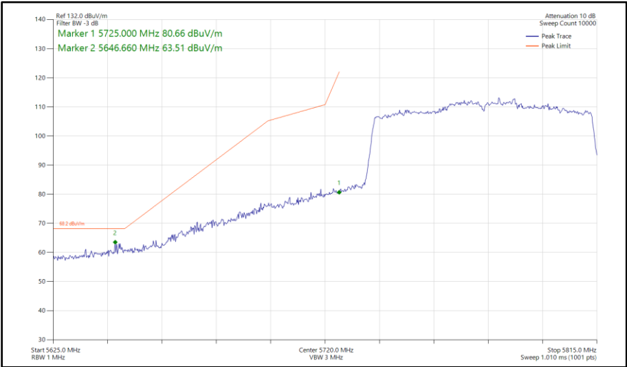
Figure 556 - 802.11ac VHT80, CDD, Core 0 - Core 1 - 5775 MHz Band Edge Frequency 5725 MHz
