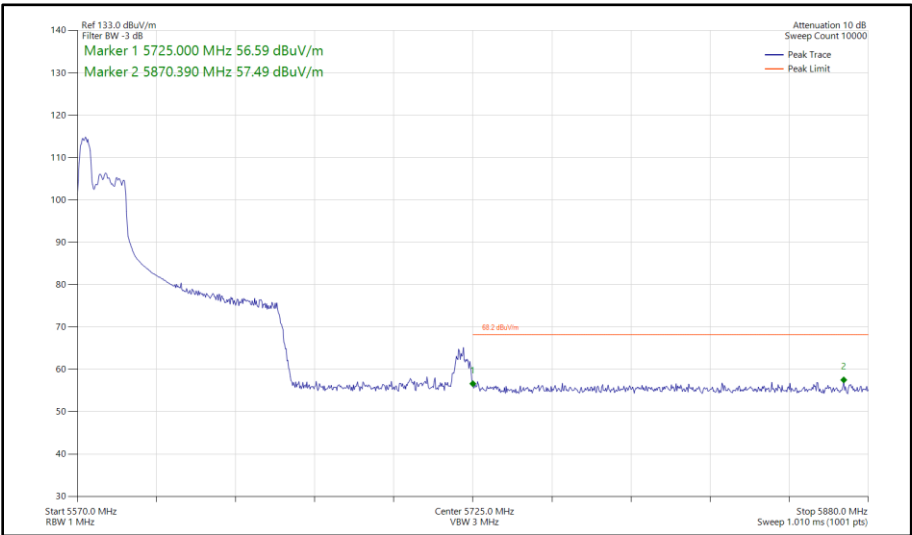
Figure 546 - 802.11ax HE80, RU 52-37, SISO, Core 1 - 5610 MHz Band Edge Frequency 5725 MHz
