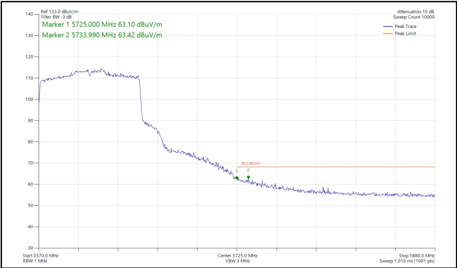
Figure 560 - 802.11ax HE80, SU, CDD, Core 0 - Core 1 - 5610 MHz Band Edge Frequency 5725 MHz
