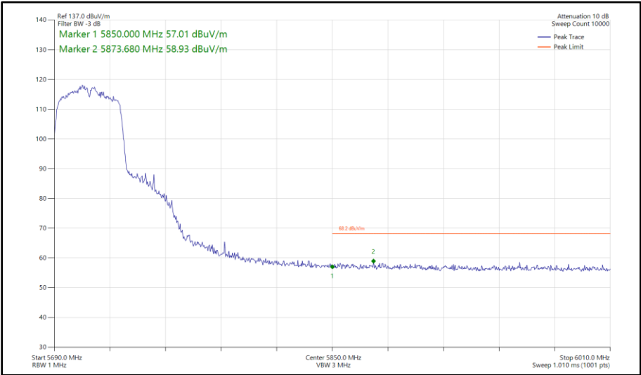
Figure 521 - 802.11ac VHT40, TxBF, Core 0 - Core 1 - 5710 MHz Band Edge Frequency 5850 MHz
