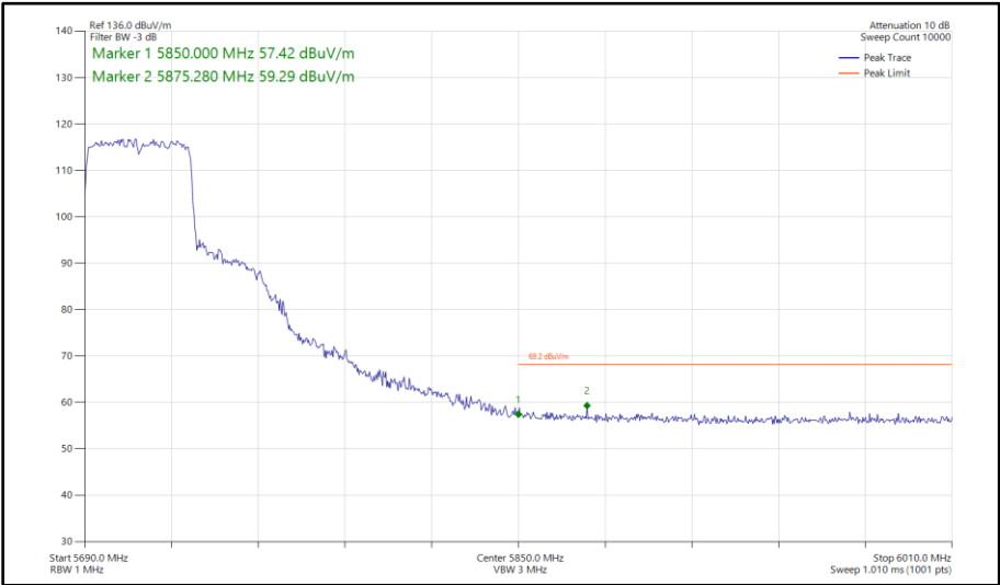
Figure 512 - 802.11ax HE40, SU, SDM, Core 0 - Core 1 - 5710 MHz Band Edge Frequency 5850 MHz
