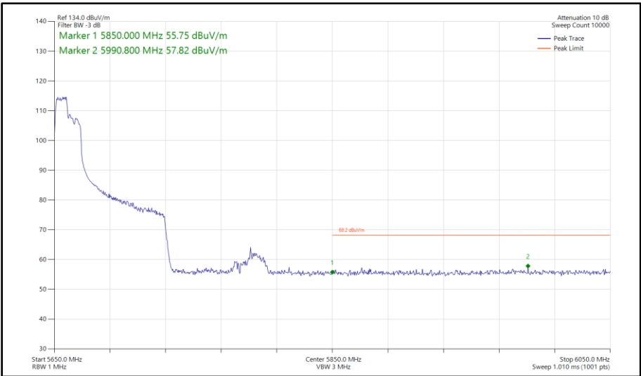
Figure 550 - 802.11ax HE80, RU 106-53, SISO, Core 1 - 5690 MHz Band Edge Frequency 5850 MHz
