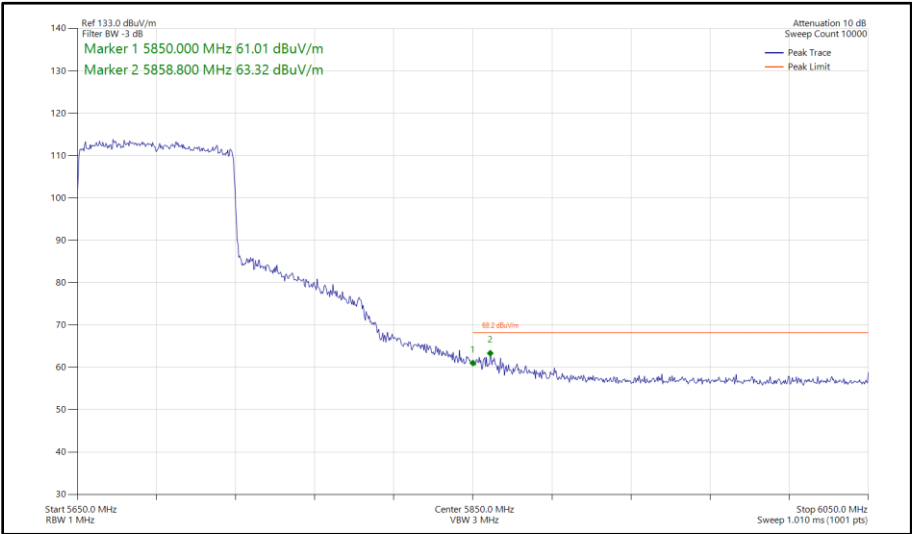
Figure 549 - 802.11ax HE80, SU, SISO, Core 1 - 5690 MHz Band Edge Frequency 5850 MHz
