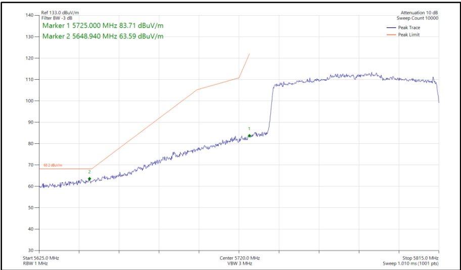
Figure 527 - 802.11ax HE80, SU, SISO, Core 0 - 5775 MHz Band Edge Frequency 5725 MHz
