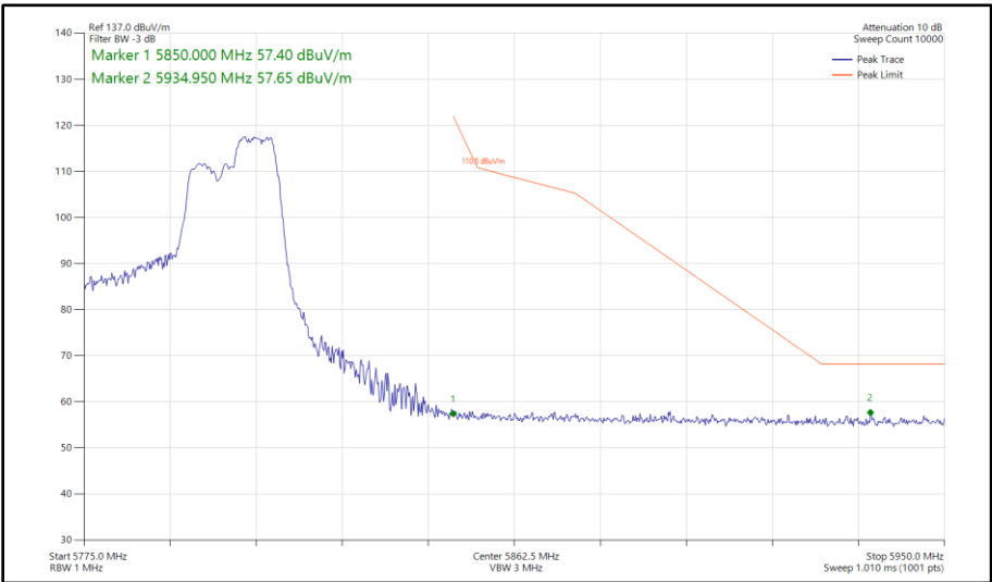
Figure 515 - 802.11ax HE40, RU 106-56, SDM, Core 0 - Core 1 - 5795 MHz Band Edge Frequency 5850 MHz
