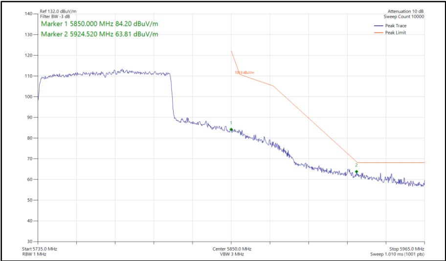
Figure 566 - 802.11ax HE80, SU, CDD, Core 0 - Core 1 - 5775 MHz Band Edge Frequency 5850 MHz
