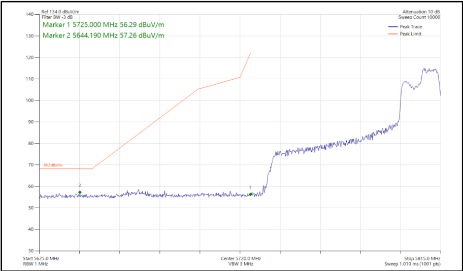
Figure 573 - 802.11ax HE80, RU 106-60, SDM, Core 0 - Core 1 - 5775 MHz Band Edge Frequency 5725 MHz
