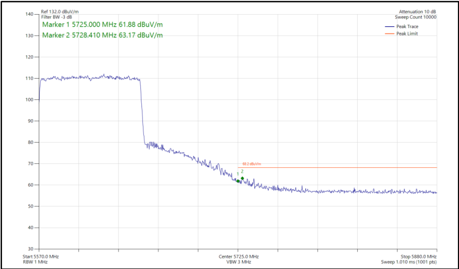
Figure 545 - 802.11ax HE80, SU, SISO, Core 1 - 5610 MHz Band Edge Frequency 5725 MHz
