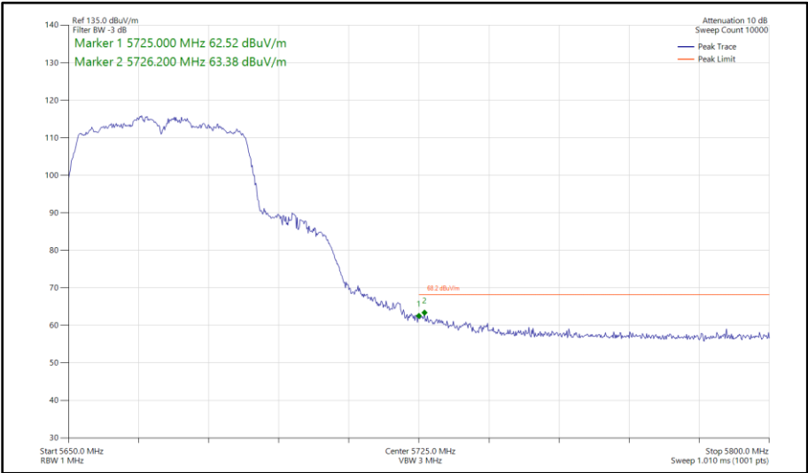
Figure 506 - 802.11n HT40, SDM, Core 0 - Core 1 - 5670 MHz Band Edge Frequency 5725 MHz
