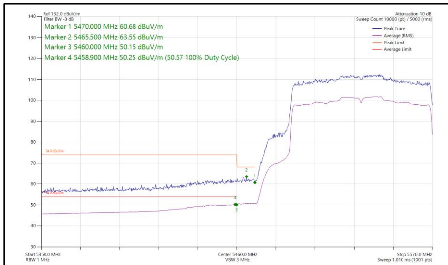
Figure 569 - 802.11ax HE80, SU, SDM, Core 0 - Core 1 - 5530 MHz Band Edge Frequency 5470 MHz
