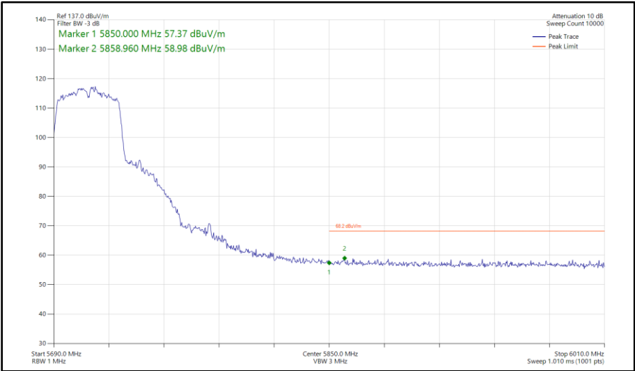
Figure 510 - 802.11n HT40, SDM, Core 0 - Core 1 - 5710 MHz Band Edge Frequency 5850 MHz
