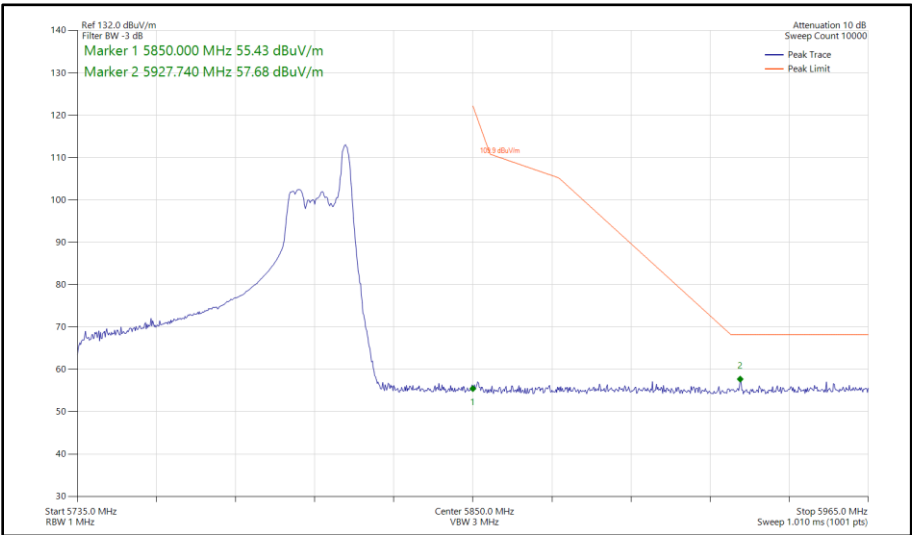
Figure 552 - 802.11ax HE80, RU 26-36, SISO, Core 1 - 5775 MHz Band Edge Frequency 5850 MHz
