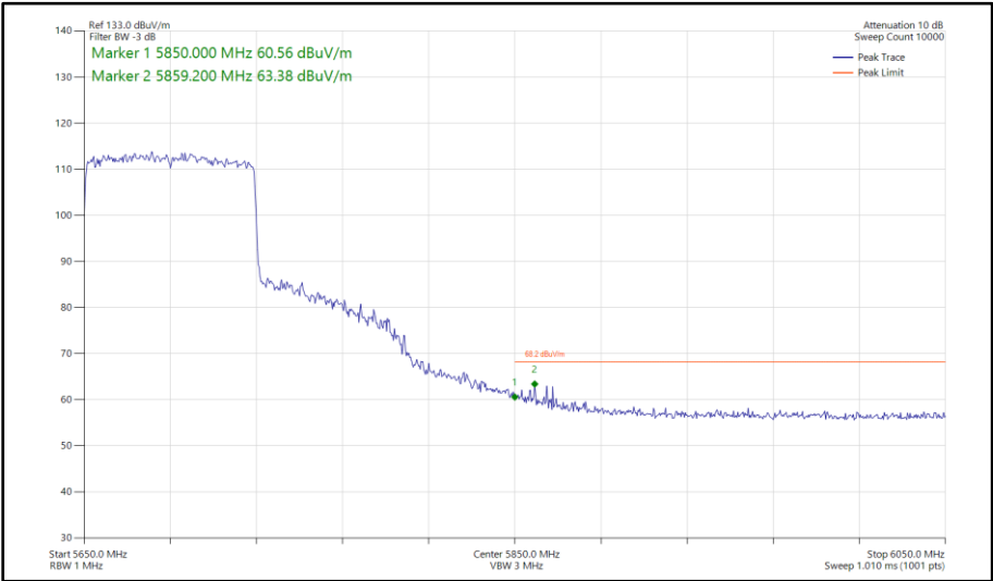
Figure 564 - 802.11ax HE80, SU, CDD, Core 0 - Core 1 - 5690 MHz Band Edge Frequency 5850 MHz
