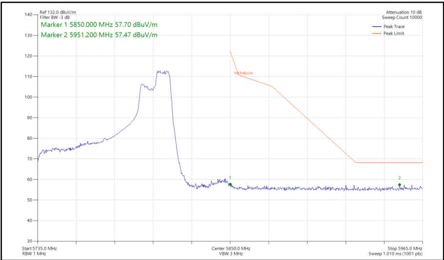
Figure 537 - 802.11ax HE80, RU 106-60, SISO, Core 0 - 5775 MHz Band Edge Frequency 5850 MHz
