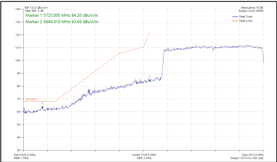
Figure 557 - 802.11ax HE80, SU, CDD, Core 0 - Core 1 - 5775 MHz Band Edge Frequency 5725 MHz
