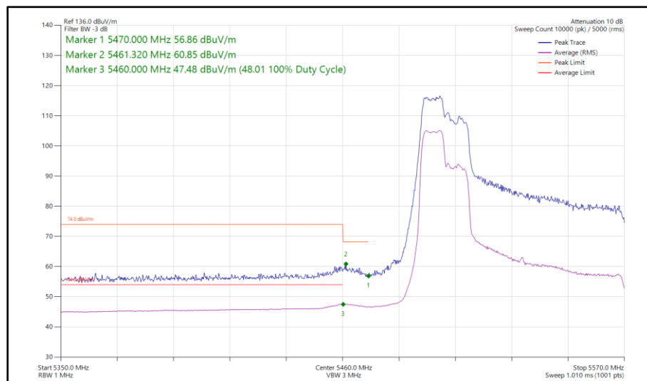
Figure 555 - 802.11ax HE80, RU 106-53, CDD, Core 0 - Core 1 - 5530 MHz Band Edge Frequency 5470 MHz
