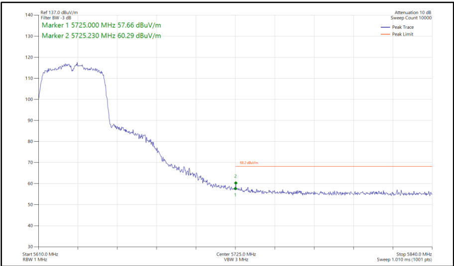
Figure 505 - 802.11n HT40, SDM, Core 0 - Core 1 - 5630 MHz Band Edge Frequency 5725 MHz
