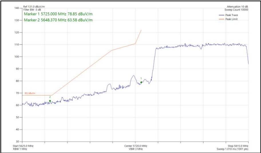
Figure 541 - 802.11ac VHT80, SISO, Core 1 - 5775 MHz Band Edge Frequency 5725 MHz
