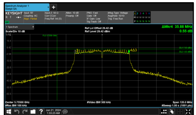
Figure 291 - 802.11n HT40 Maximum 6 dB EBW
