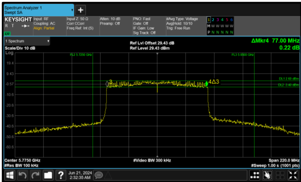
Figure 298 - 802.11ax HE80 SU Minimum 6 dB EBW
