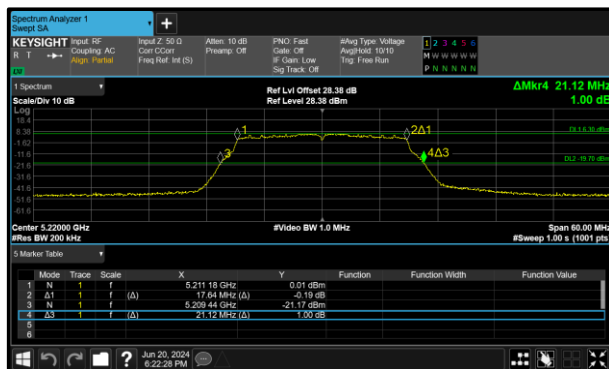
Figure 300 - 802.11n HT20 Minimum 99% OBW
