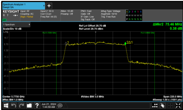
Figure 304 - 802.11ac VHT80 Minimum 99% OBW
