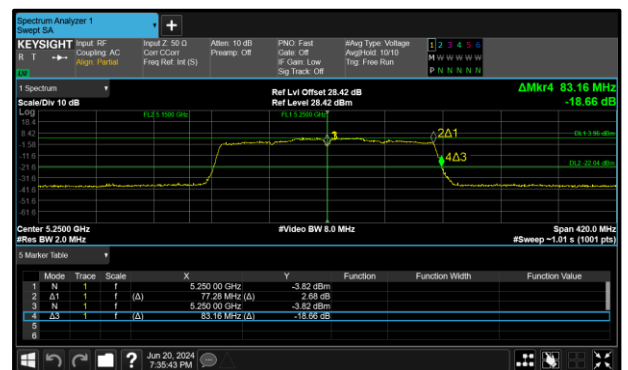
Figure 279 - 802.11ac VHT160 Maximum 99% OBW
