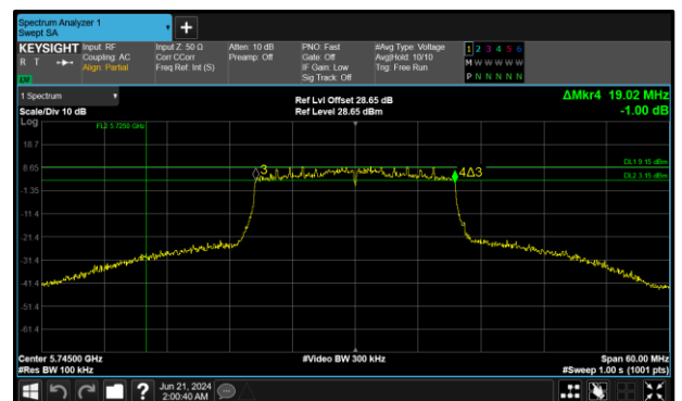
Figure 295 - 802.11ax HE20 SU Maximum 6 dB EBW
