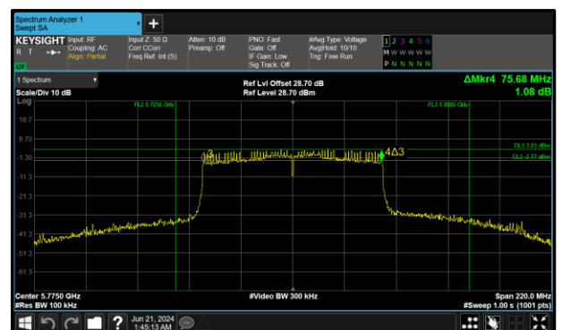
Figure 293 - 802.11ac VHT80 Maximum 6 dB EBW
