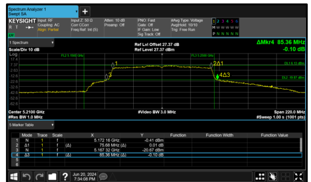
Figure 277 - 802.11ac VHT80 Maximum 99% OBW
