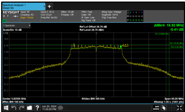
Figure 260 - 802.11n HT20 Minimum 6 dB EBW
