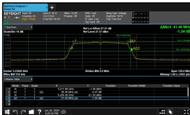
Figure 302 - 802.11n HT40 Minimum 99% OBW
