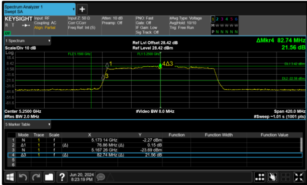
Figure 306 - 802.11ac VHT160 Minimum 99% OBW
