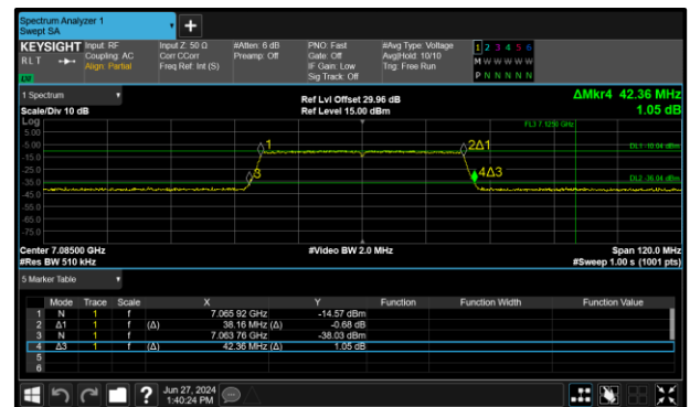
Figure 34 - 802.11ax HE40 SU LPI Maximum and 99% OBW
