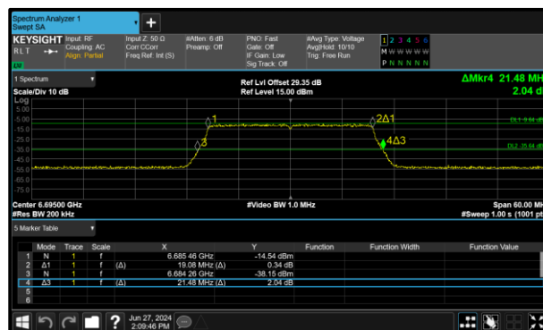
Figure 44 - 802.11ax HE20 SU VLP Maximum 26 dB EBW
