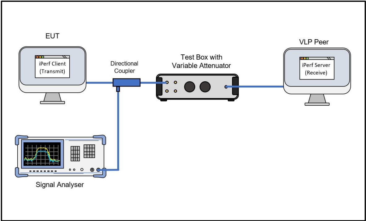
Figure 88 - Test Equipment Setup Diagram
