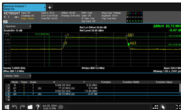
Figure 83 - 802.11ax HE80 SU SP Minimum 99% OBW
