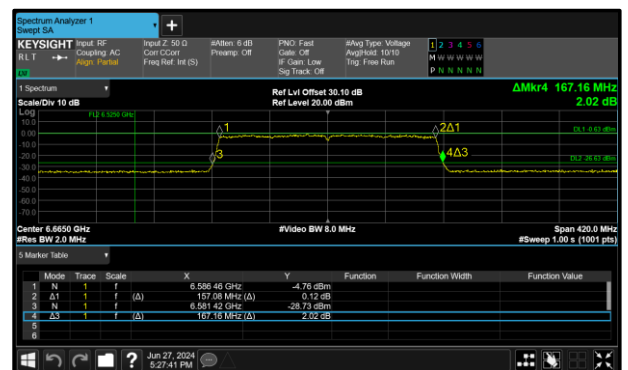
Figure 76 - 802.11ax HE160 SU VLP Maximum 99% OBW
