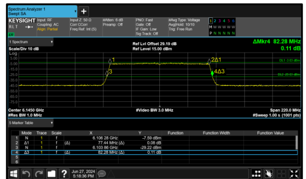
Figure 74 - 802.11ax HE80 SU VLP Maximum 99% OBW
