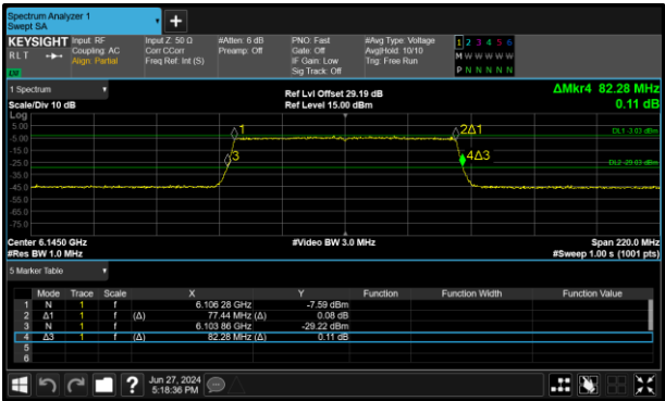
Figure 141 - 802.11ax HE80 SU VLP Minimum 26 dB EBW
