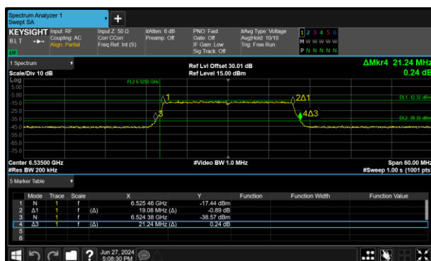
Figure 137 - 802.11ax HE20 SU VLP Minimum 26 dB EBW
